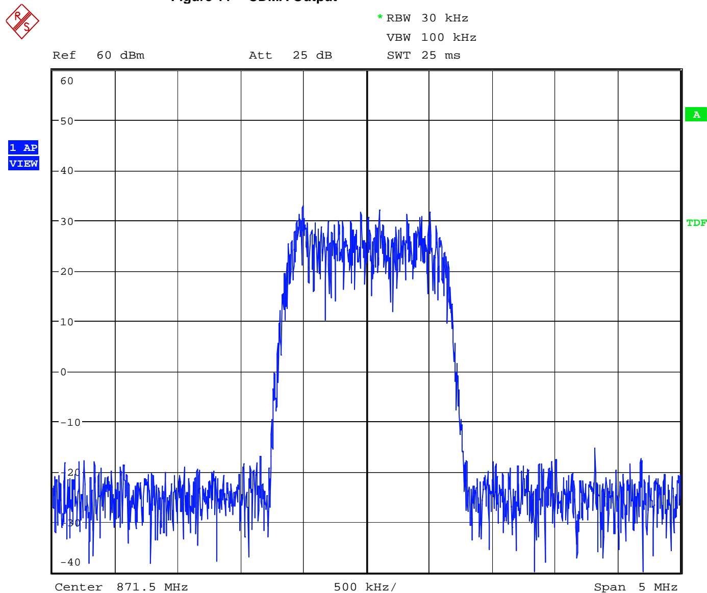
Figure 11 CDMA Output
