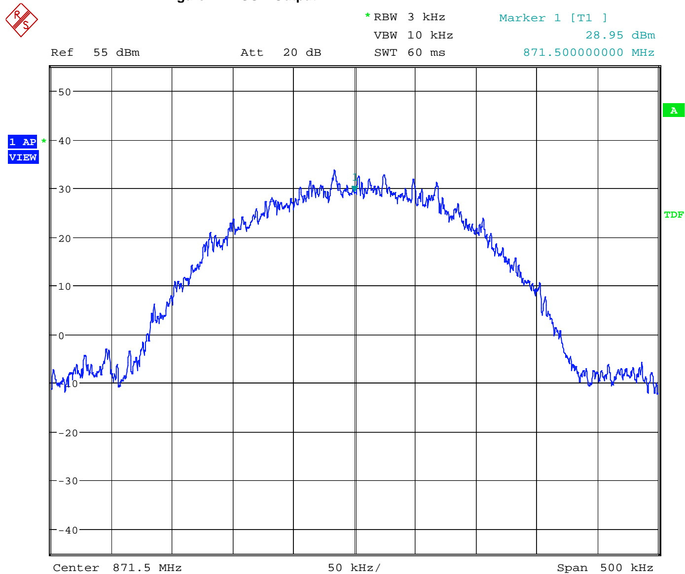
Figure 7 GSM Output
