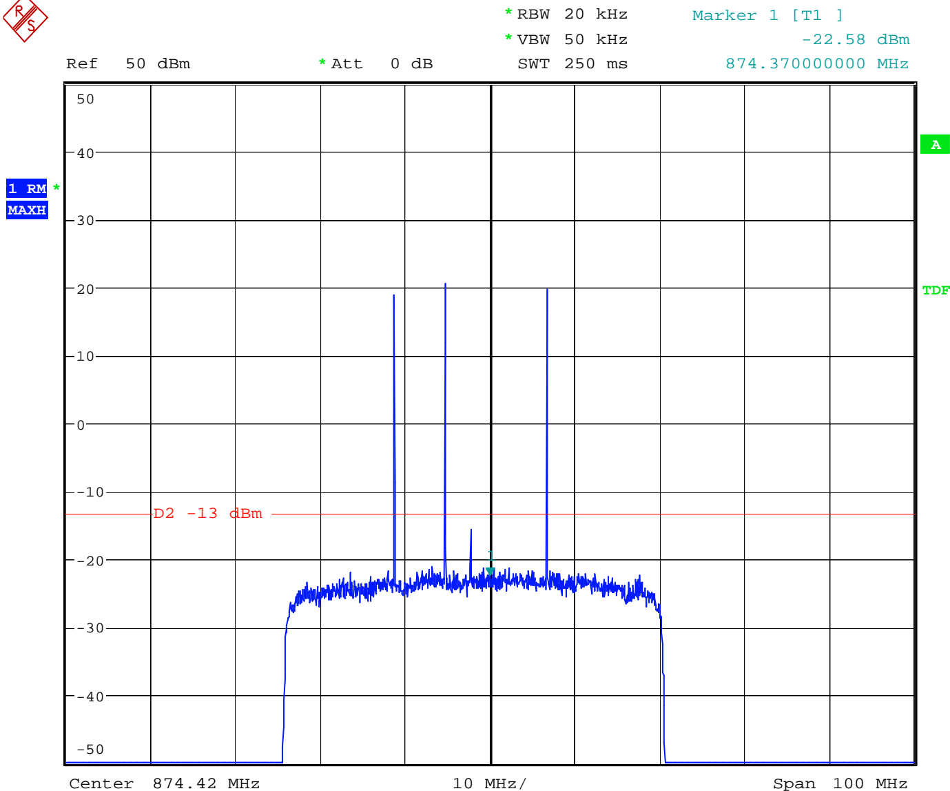
Figure 37 3 rd Order Inter-modulation Spurious - Downlink – IDEN
