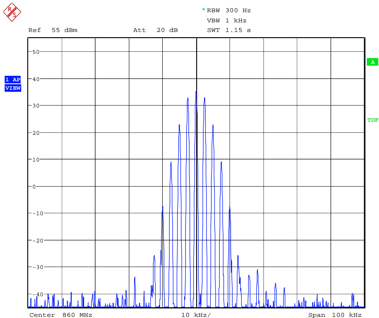
Figure 1 Analog Output
