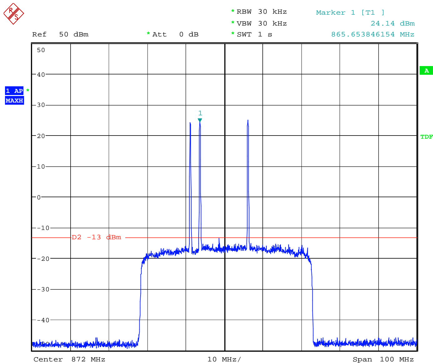
Figure 34 3rd Order Inter-modulation Spurious - Downlink – GSM
