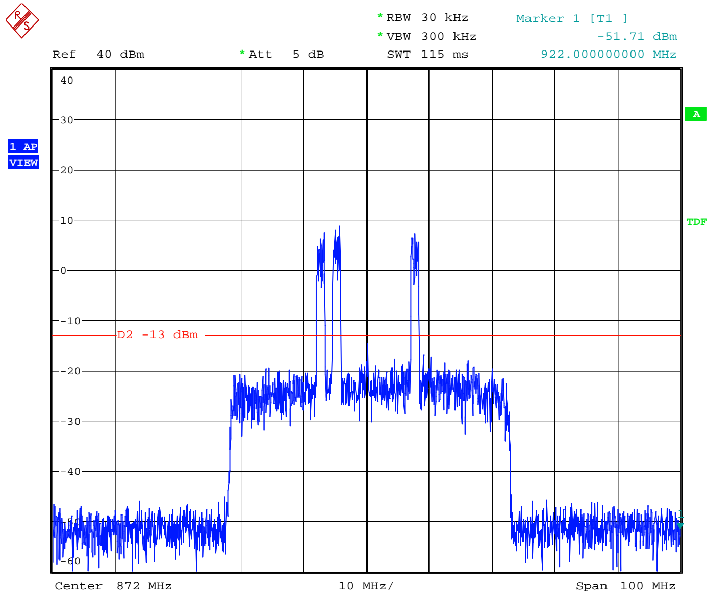
Figure 29 3 rd Order Inter-modulation Spurious - Downlink – IS-95 CDMA
