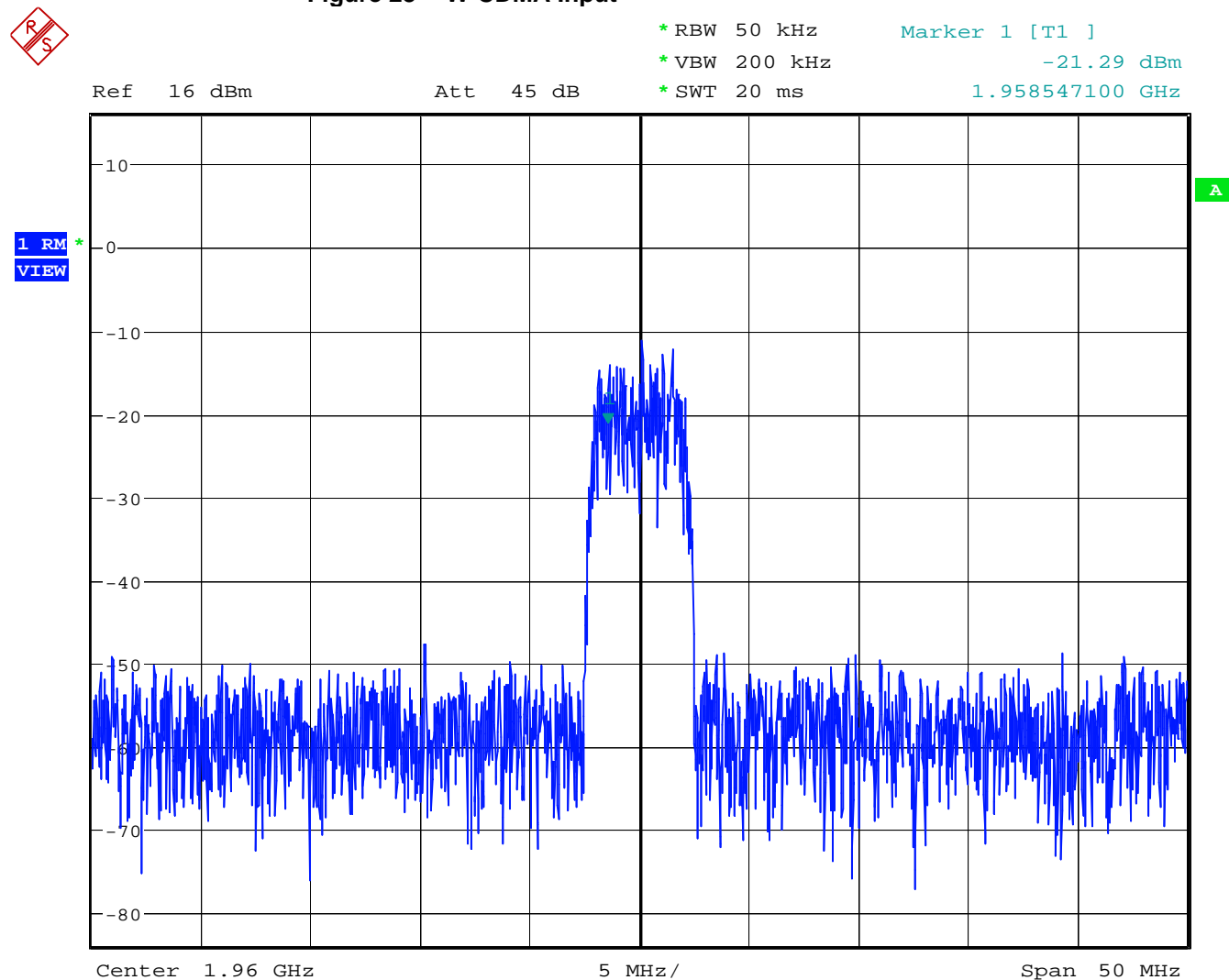
Figure 28 W-CDMA Input
