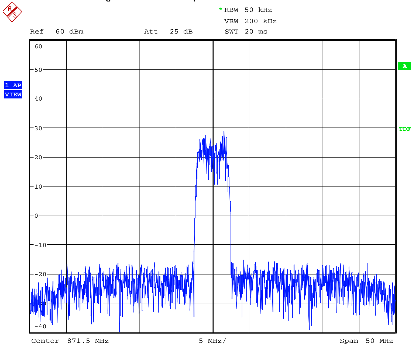
Figure 15 W-CDMA Output
