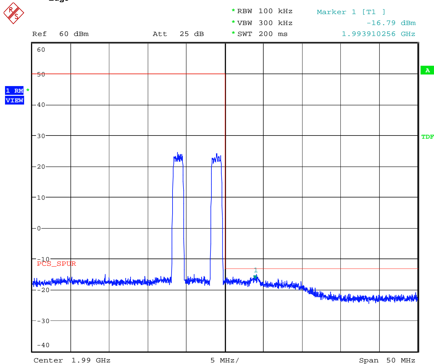
Figure 39 3 rd Order Inter-modulation Spurious - Downlink – IS-95 CDMA Upper Edge
