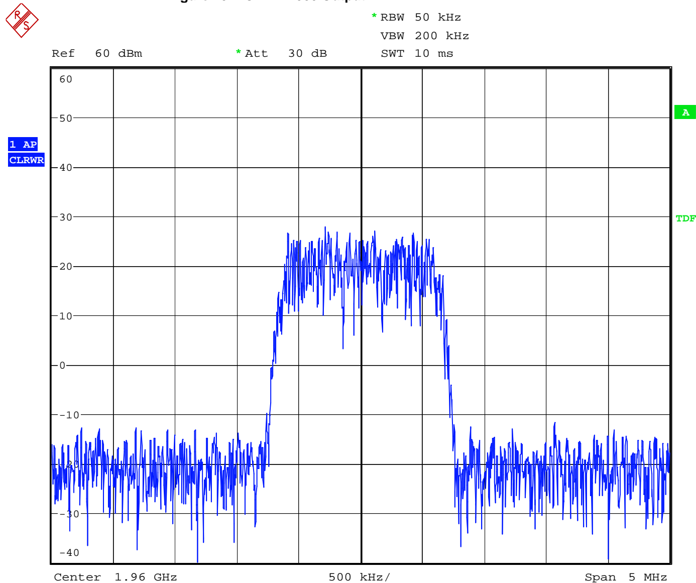
Figure 25 CDMA 2000 Output
