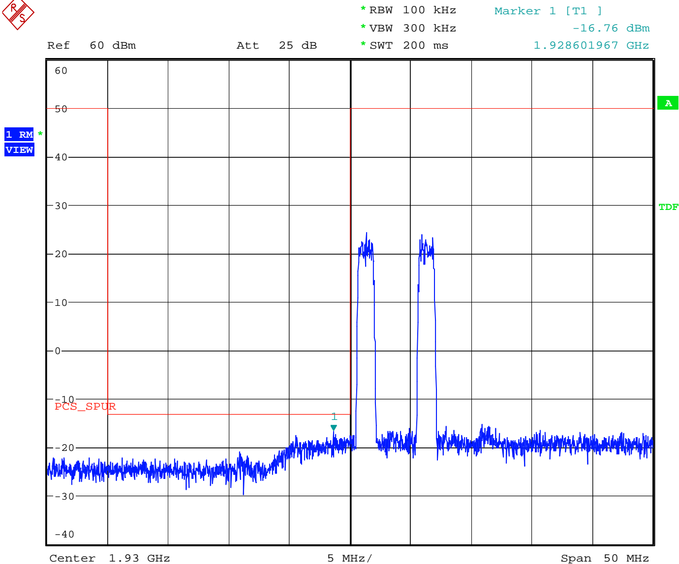
Figure 40 3 rd Order Inter-modulation Spurious - Downlink – IS-95 CDMA Lower Edge Edge
