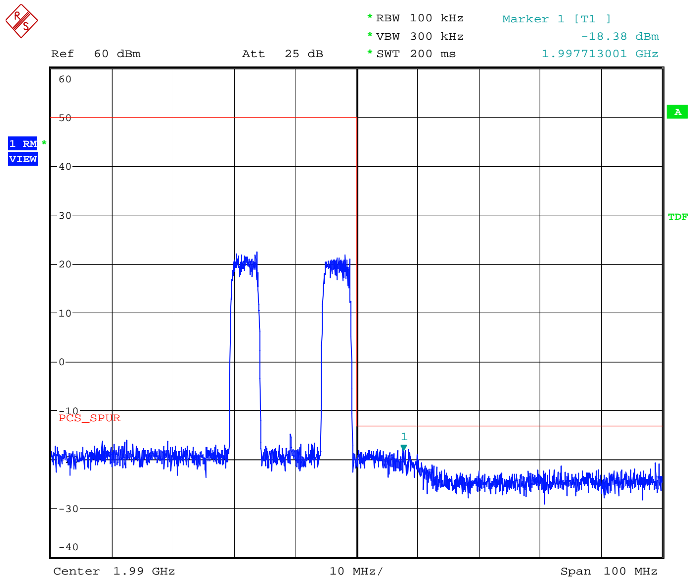
Figure 42 3rd Order Inter-modulation Spurious - Downlink - W-CDMA Upper Edge
