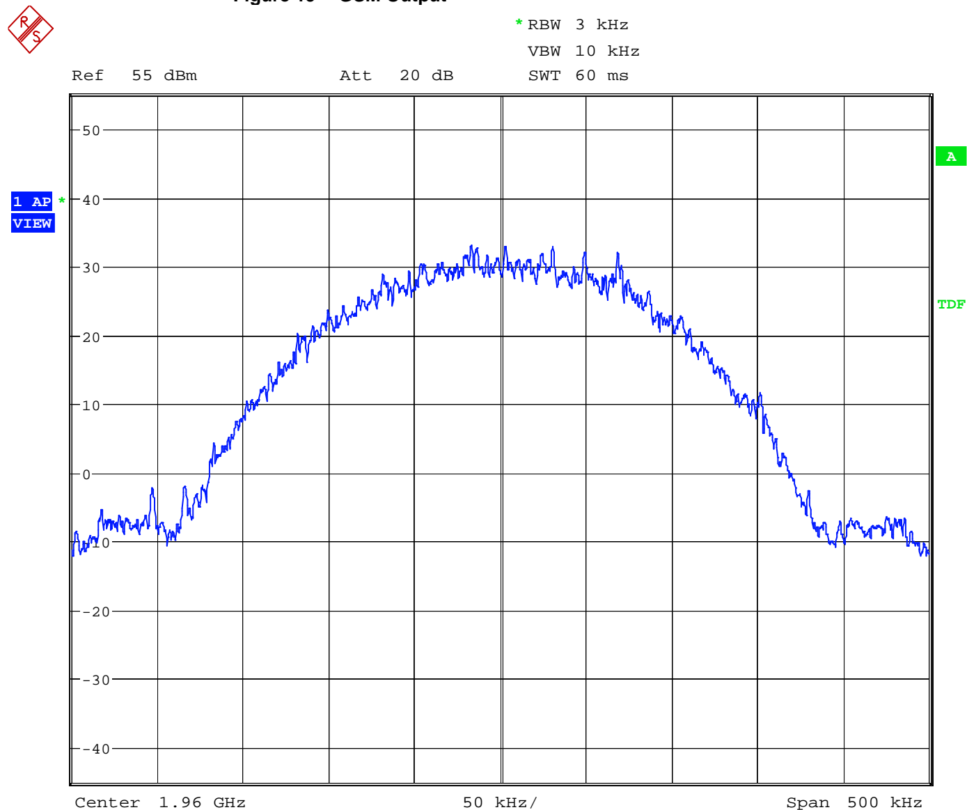
Figure 19 GSM Output
