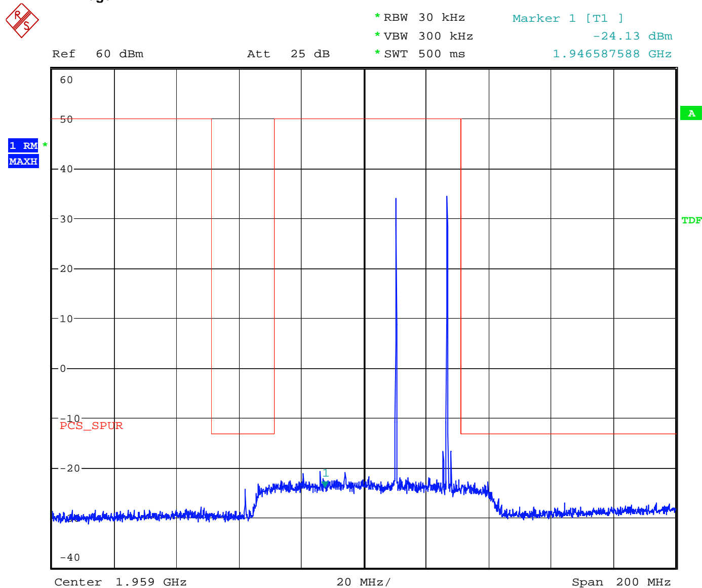
Figure 50 3 rd Order Inter-modulation Spurious - Downlink – GSM Edge Upper Edge
