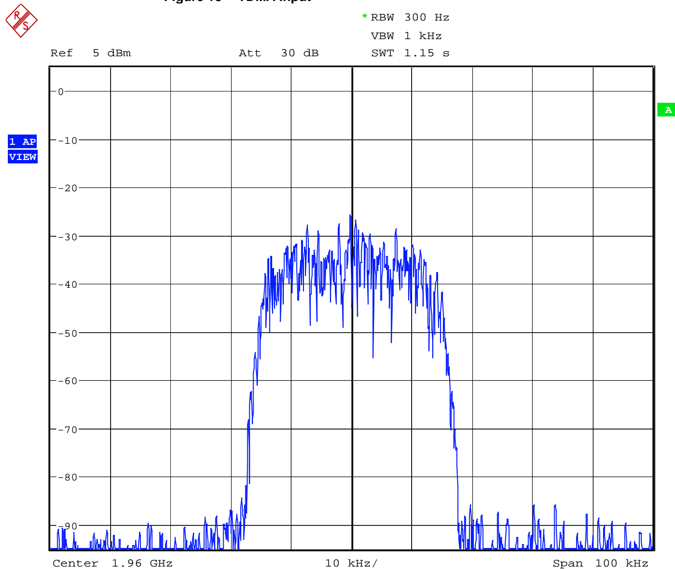
Figure 18 TDMA Input
