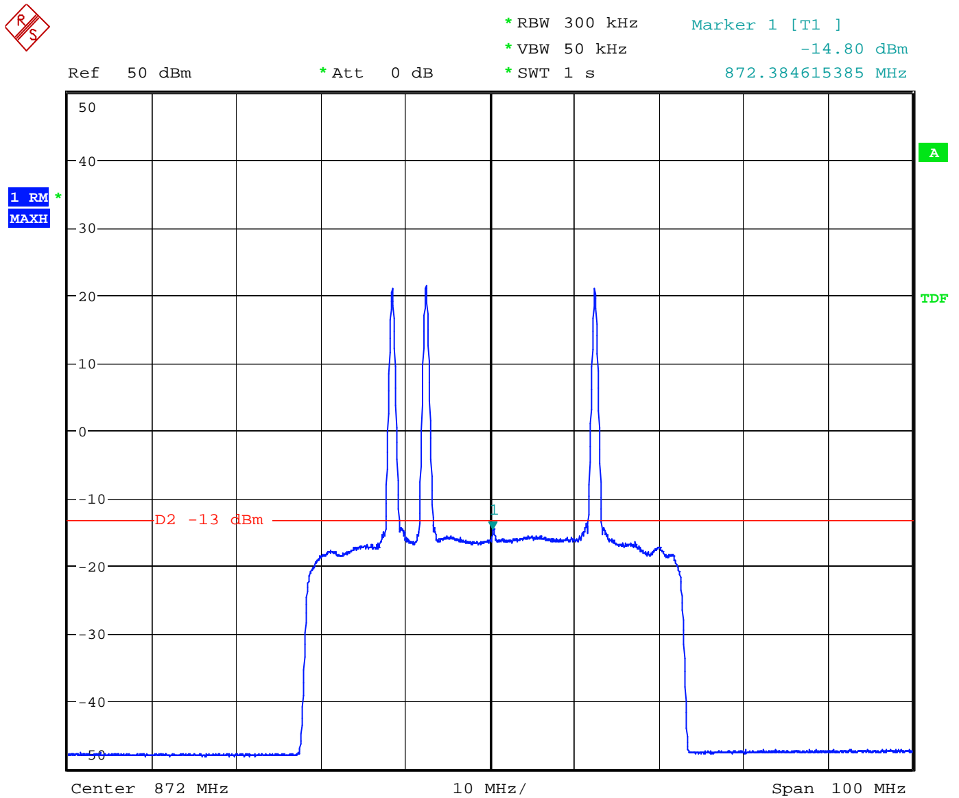
Figure 35 3 rd Order Inter-modulation Spurious - Downlink – GSM Edge
