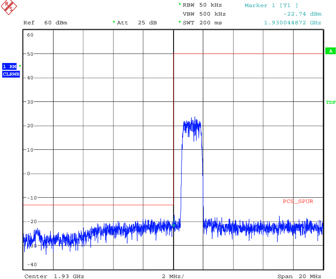
Figure 45 3 rd Order Inter-modulation Spurious - Downlink – CDMA 2000 Lower Edge
