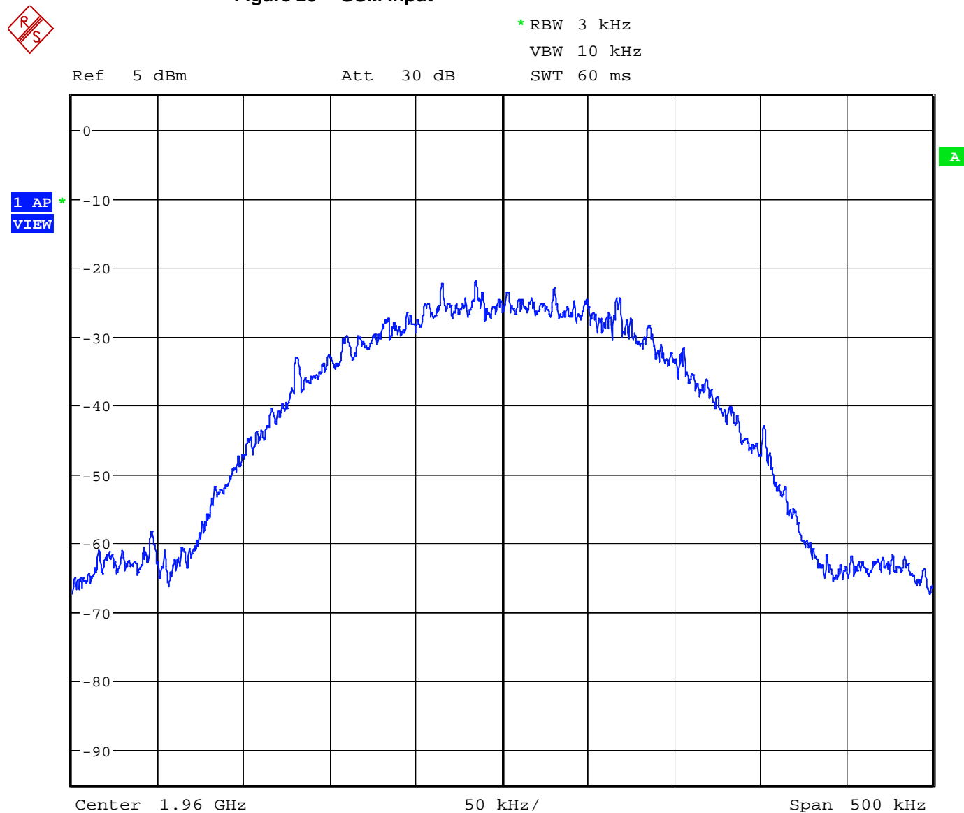
Figure 20 GSM Input
