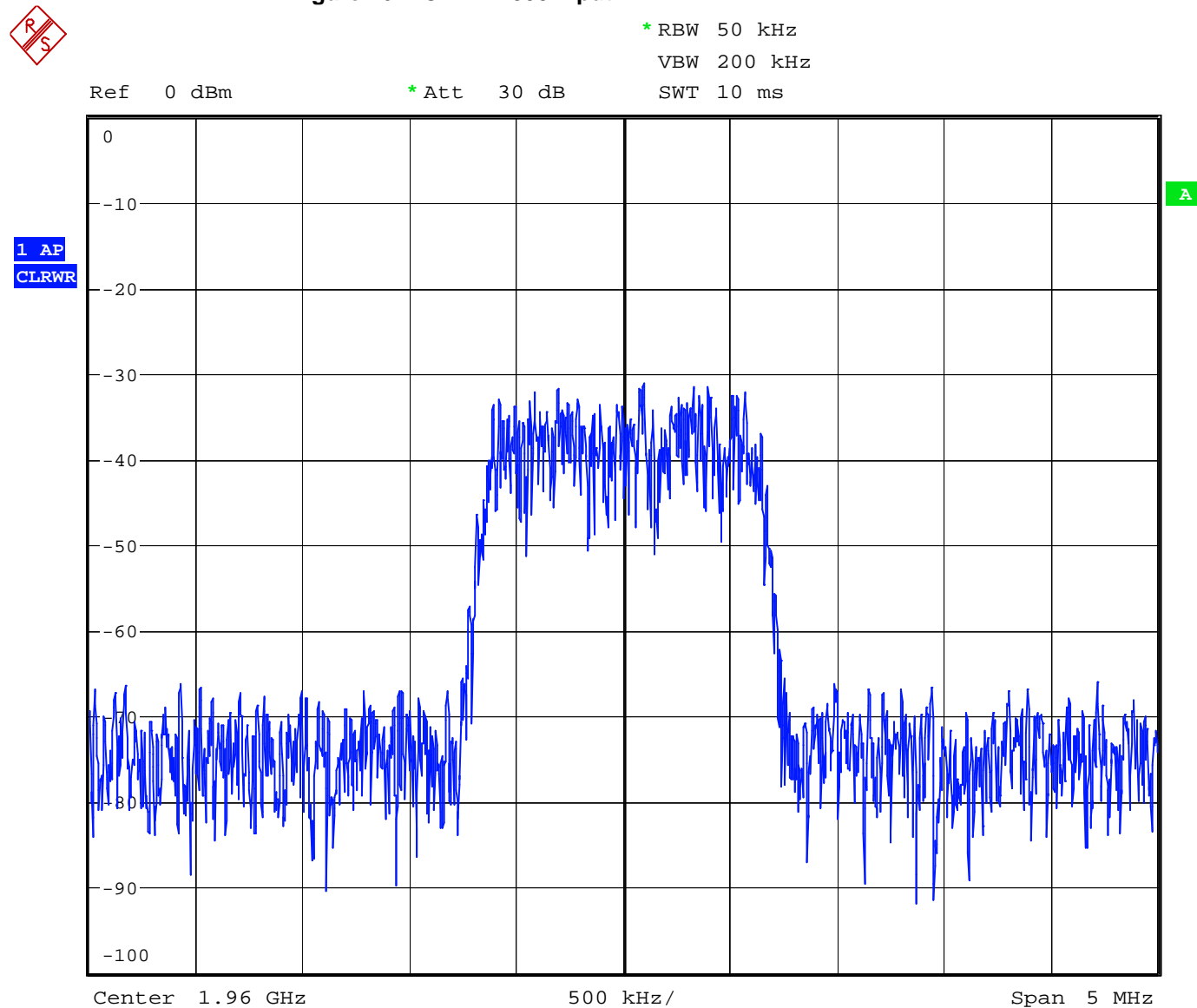
Figure 26 CDMA 2000 Input
