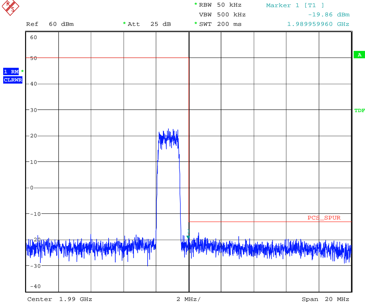
Figure 44 3 rd Order Inter-modulation Spurious - Downlink – CDMA 2000 Upper Edge
