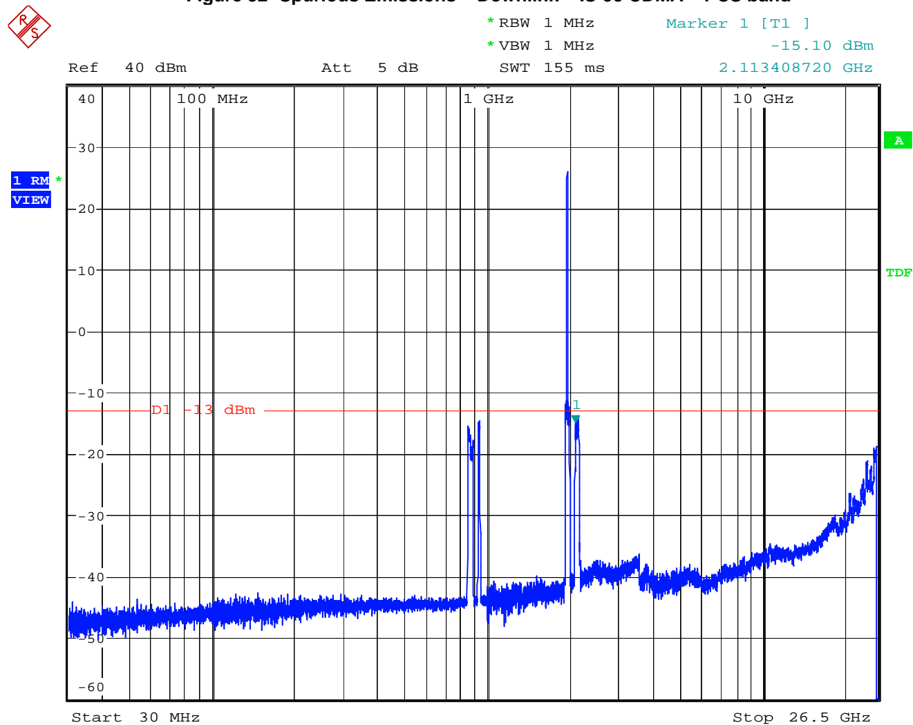
Figure 52 Spurious Emissions – Downlink – IS-95 CDMA – PCS band
