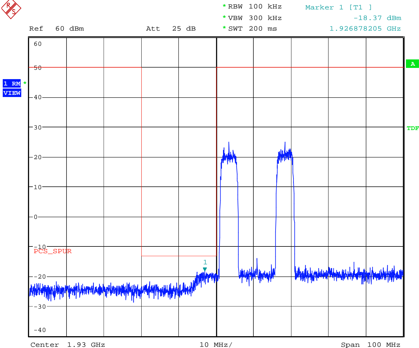
Figure 41 3rd Order Inter-modulation Spurious - Downlink - W-CDMA Lower Edge
