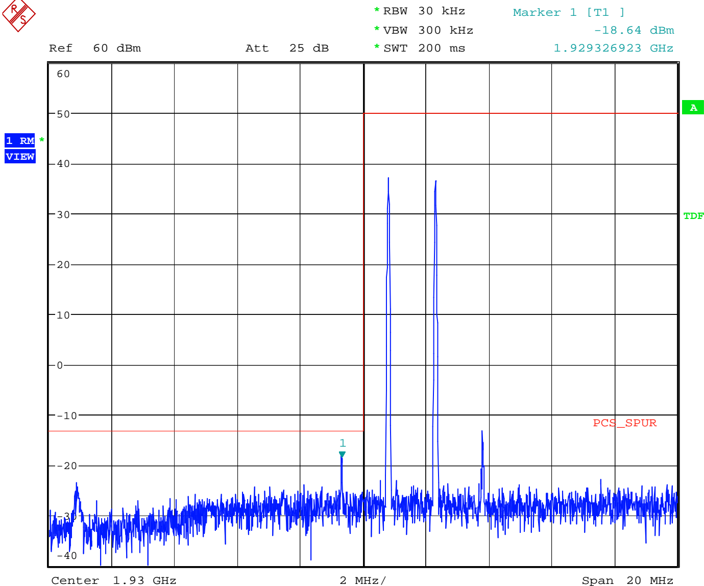
Figure 46 3 rd Order Inter-modulation Spurious - Downlink – TDMA Lower Edge
