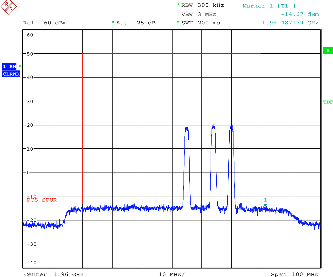
Figure 43 3 rd Order Inter-modulation Spurious - Downlink – CDMA 2000
