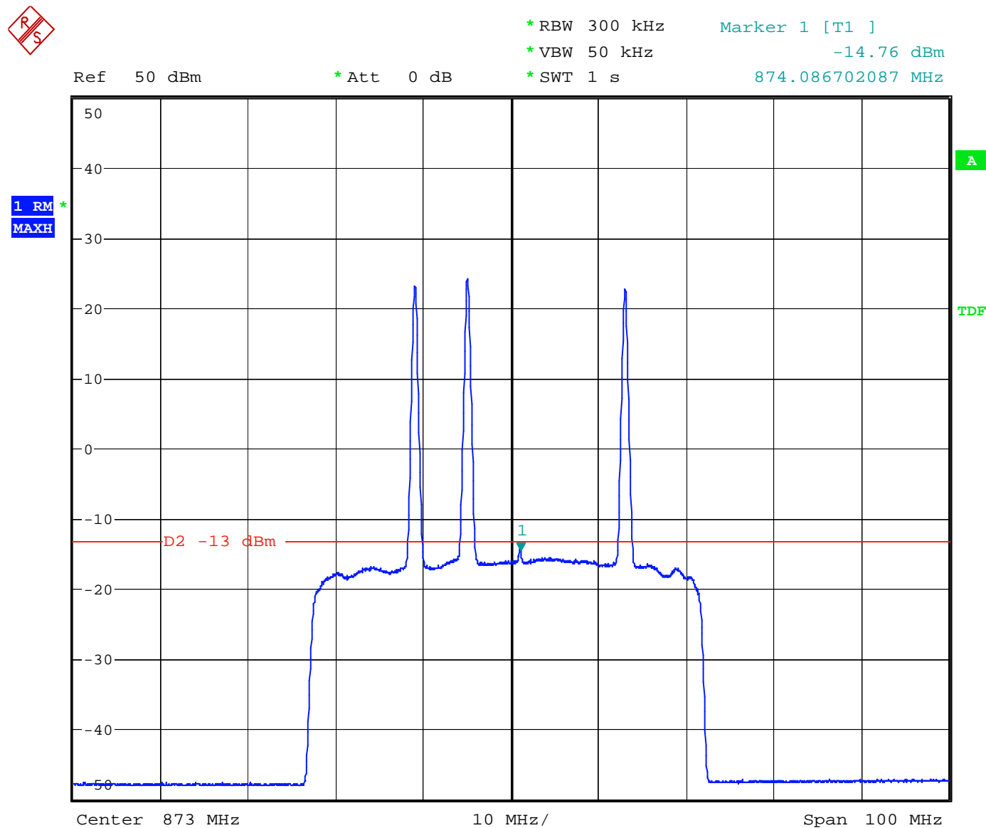
Figure 36 3 rd Order Inter-modulation Spurious - Downlink – TDMA
