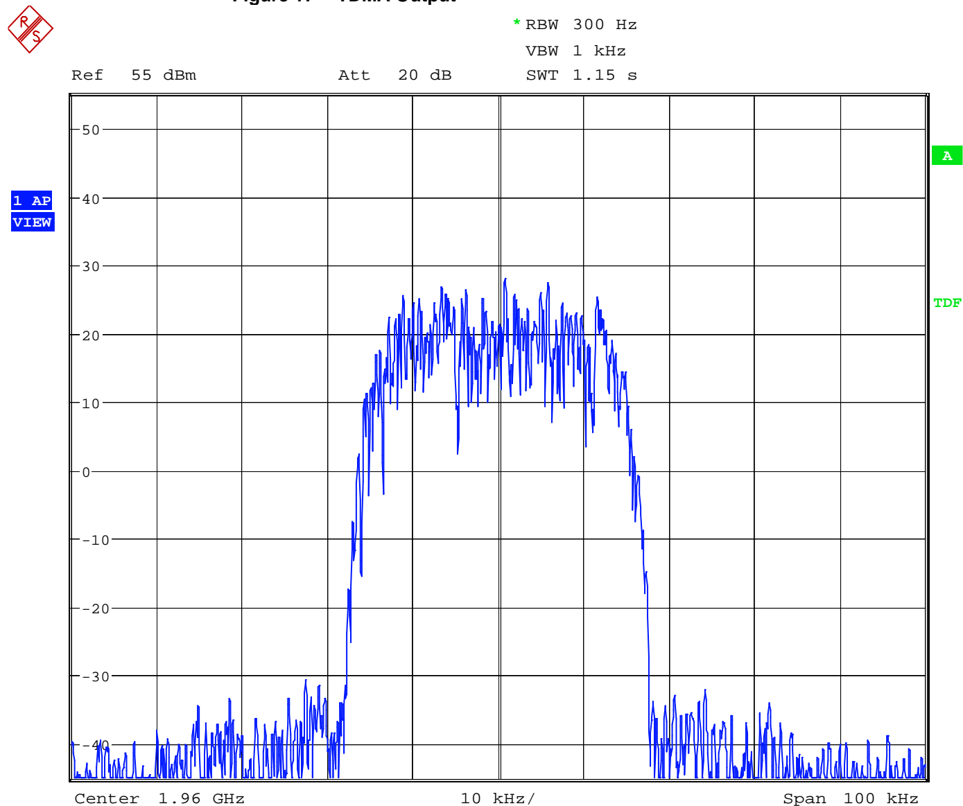
Figure 17 TDMA Output
