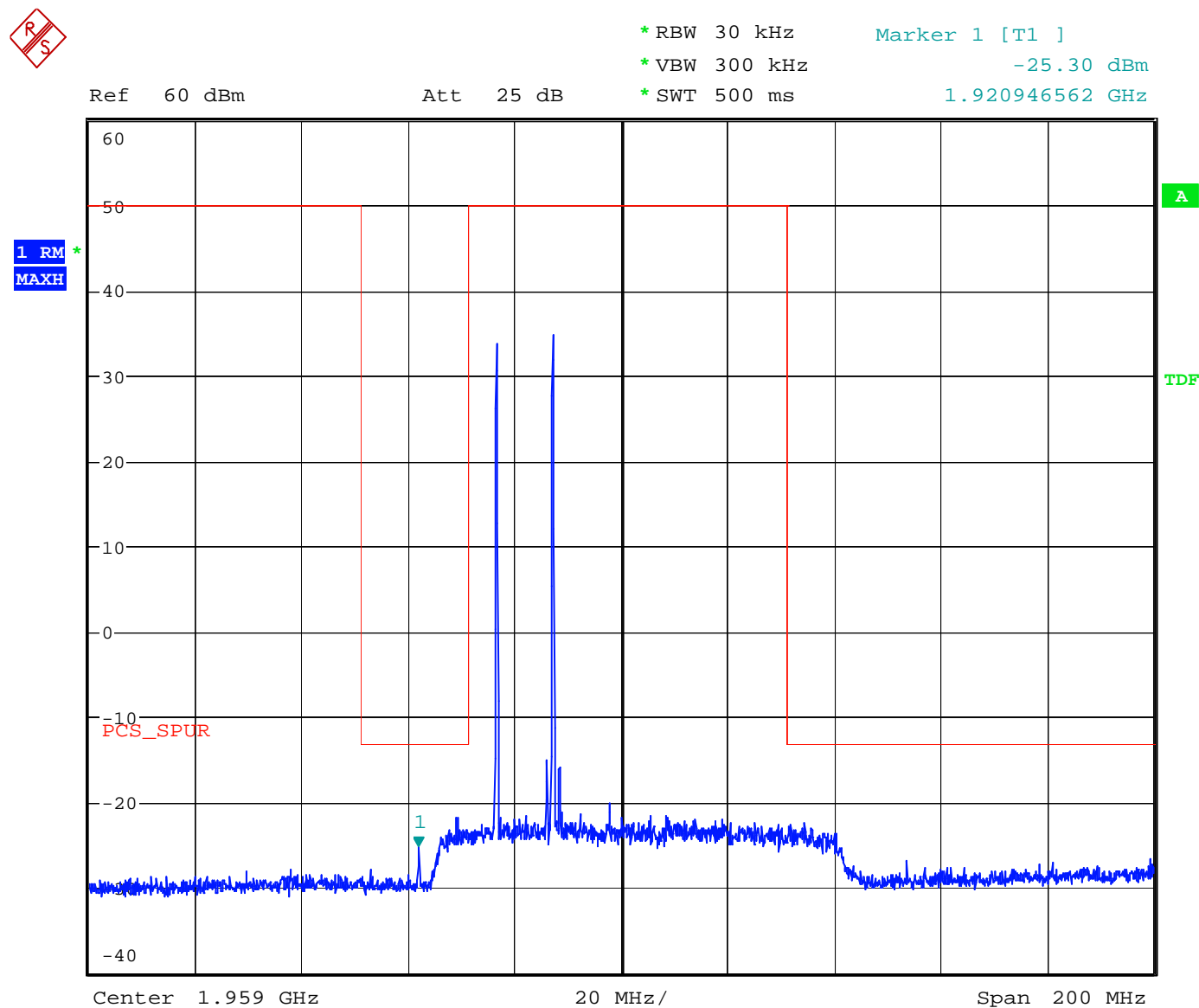
Figure 49 3 rd Order Inter-modulation Spurious - Downlink – GSM Edge Lower Edge
