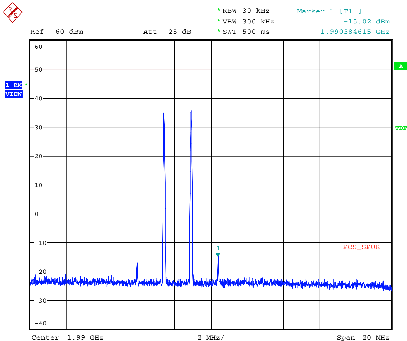
Figure 47 3 rd Order Inter-modulation Spurious - Downlink – TDMA Upper Edge
