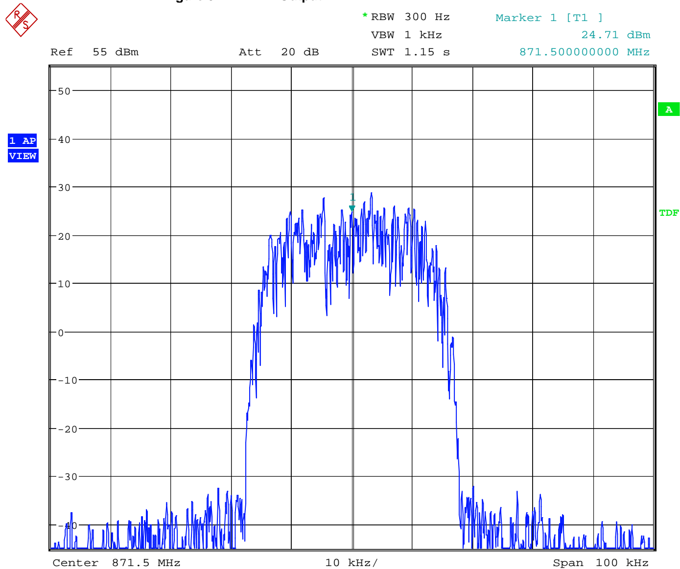
Figure 5 TDMA Output
