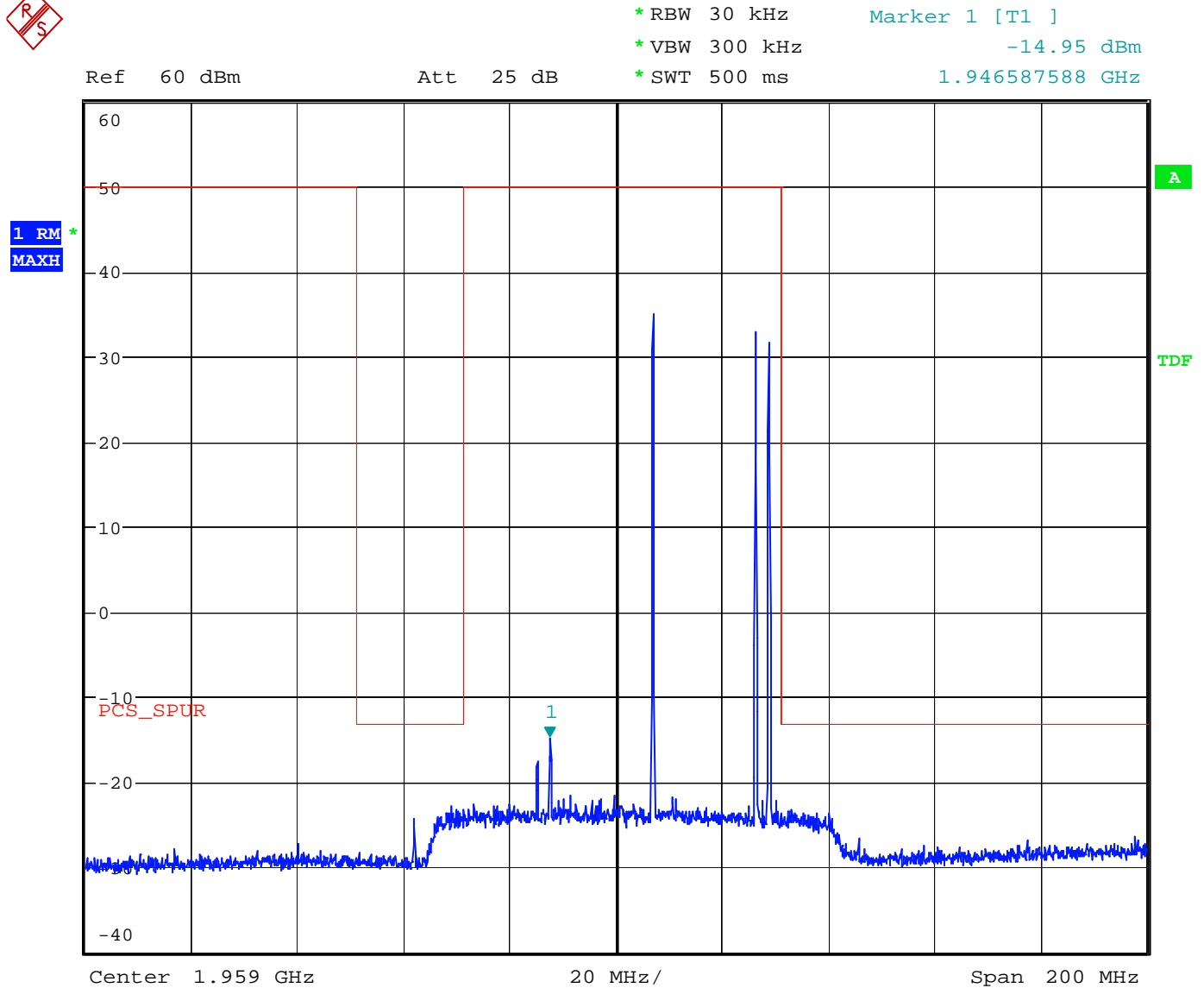
Figure 48 3 rd Order Inter-modulation Spurious - Downlink – GSM
