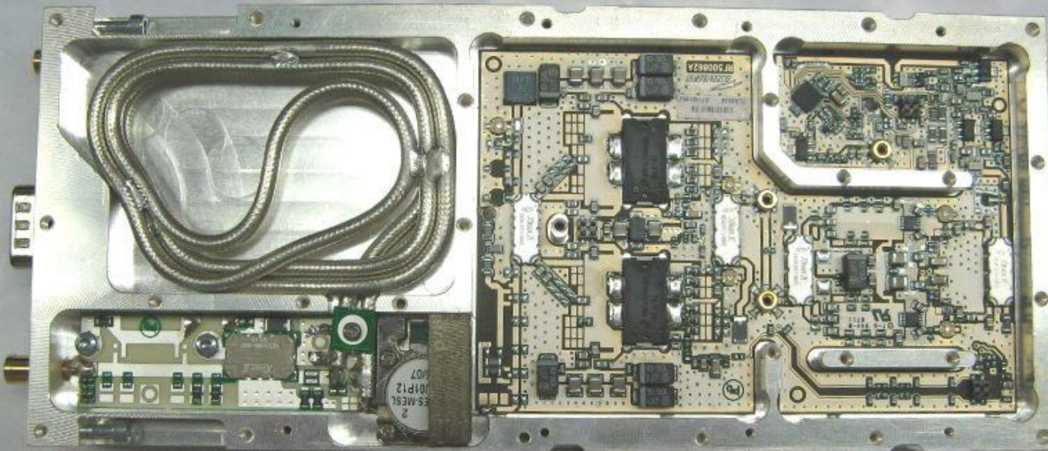
1900 MHz Main RF Board
