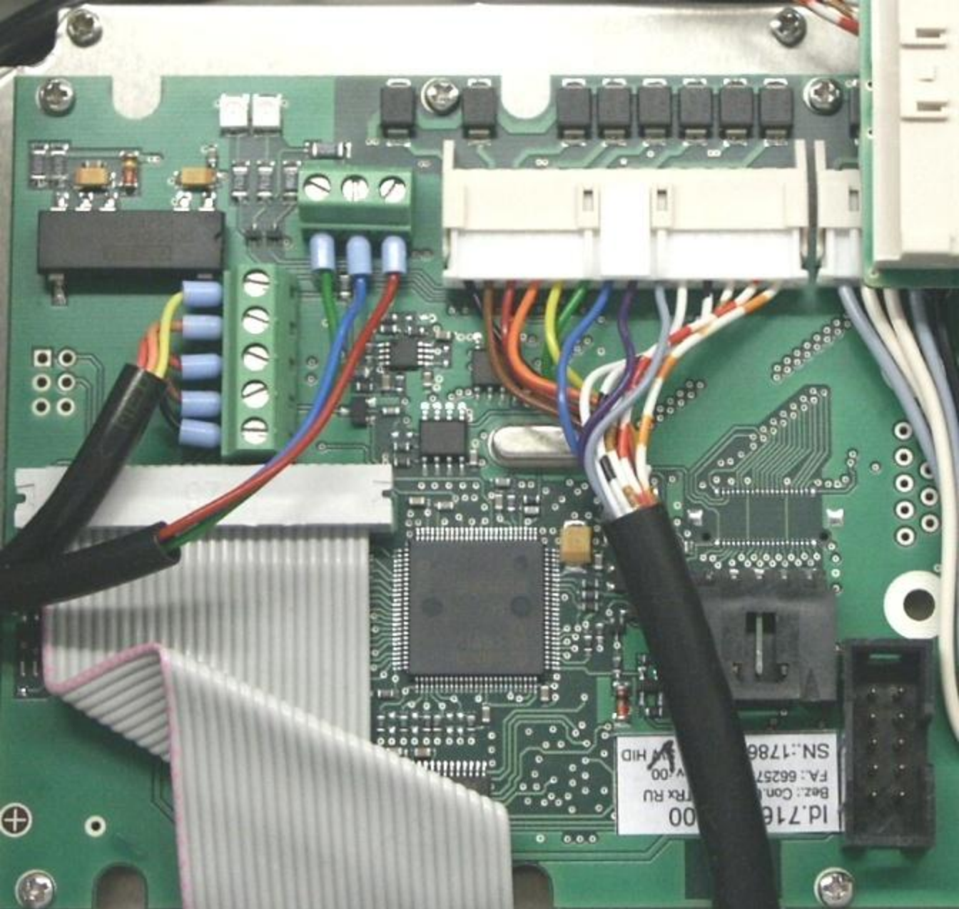
Main Unit - Control Board
