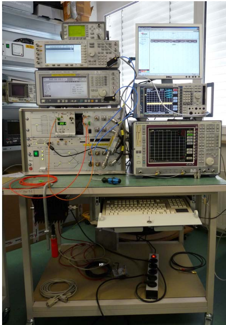
Figure 3. Measurement Equipment
