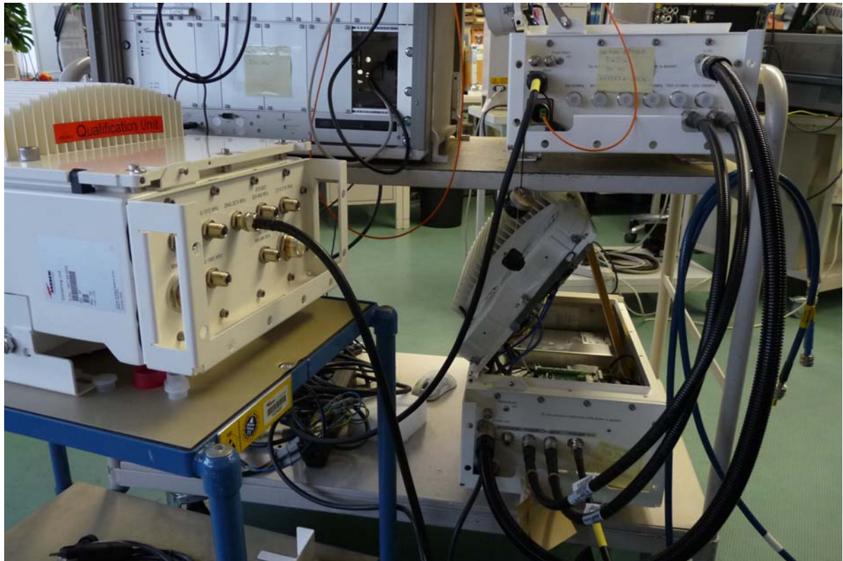
Figure 1. Whole measurement: Remote Unit, Extension Unit and Combining Unit
