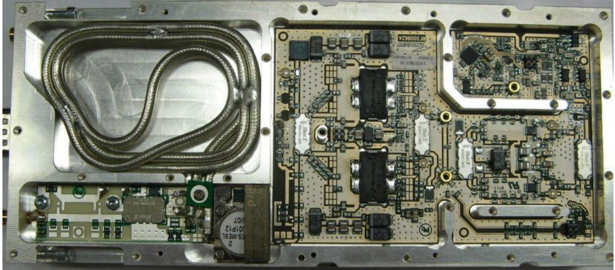
2100 MHz PA - Bottom
