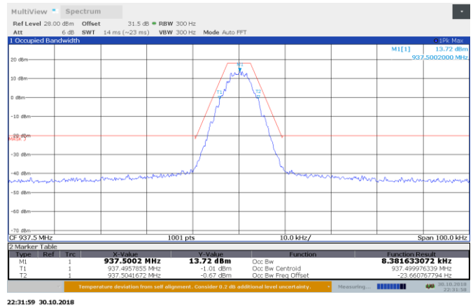
Figure 8.3-2: 8K10F1D AGC-0.5 dB 937.5 MHz output 99% BW Emission Mask J
