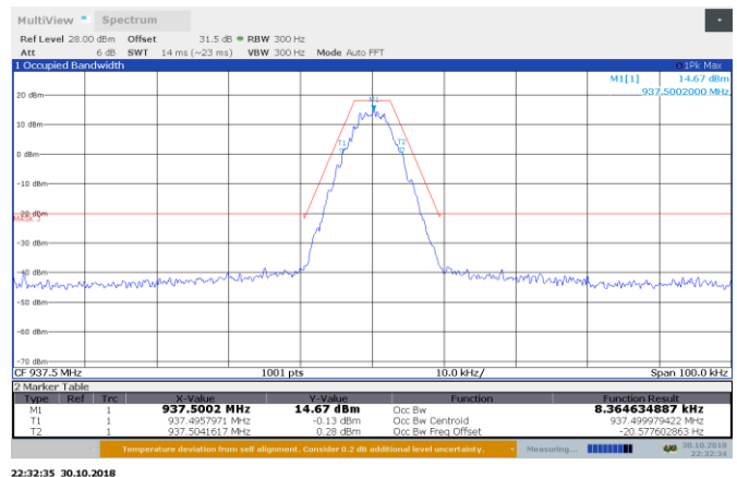
Figure 8.3-4: 8K10F1D AGC +3 dB 937.5 MHz output 99% BW Emission Mask J
