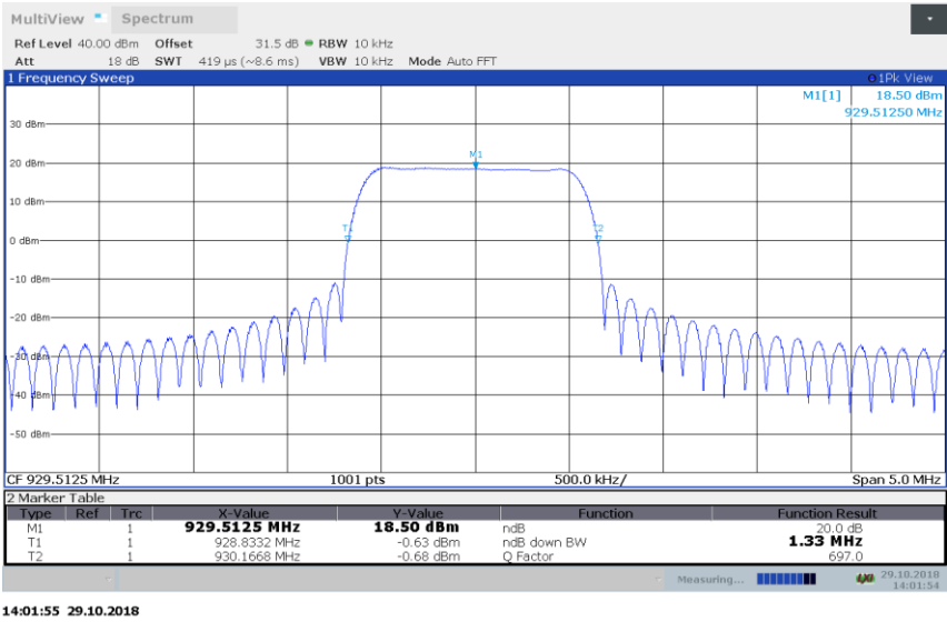
Figure 8.2-1: Passband
