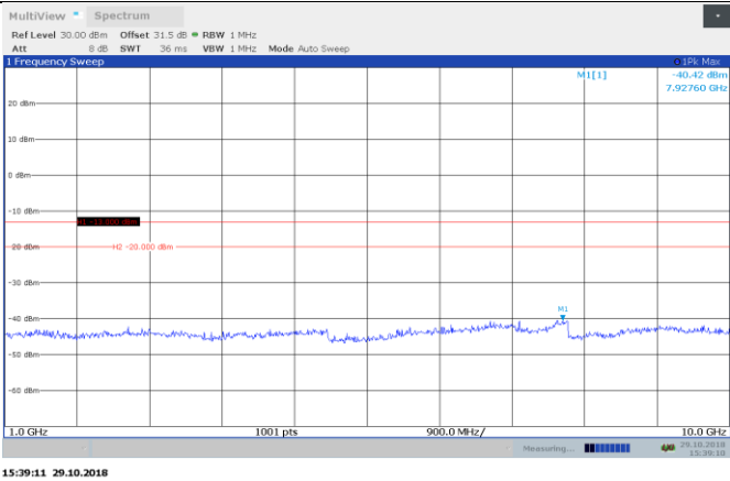
Figure 8.6-2: 929.5125 MHz 1-10 GHz conducted emission
