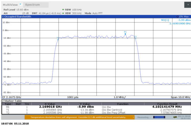
Figure 8.3-1: Input signal AGC -0.5dB 2167.5 MHz input 99% BW
