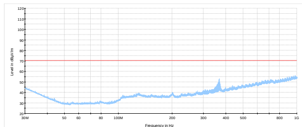
Figure 8.7-1: 30 MHz to 1 GHz Radiated
