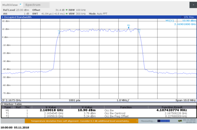
Figure 8.3-2: Output signal AGC -0.5dB 2167.5 MHz Output 99% BW
