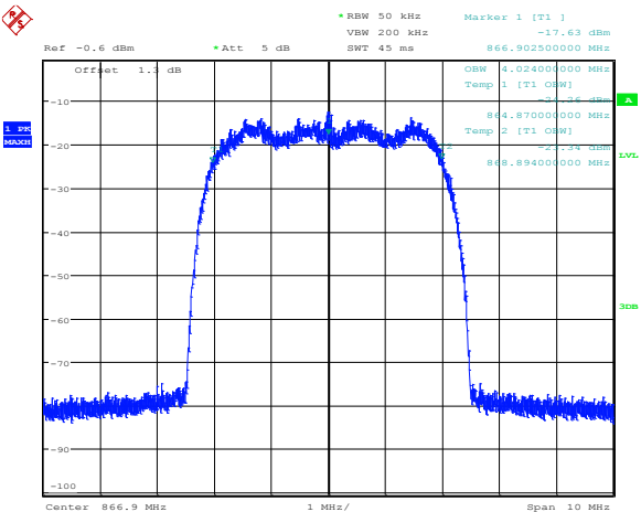
Figure 8.5-6: CDMA output
