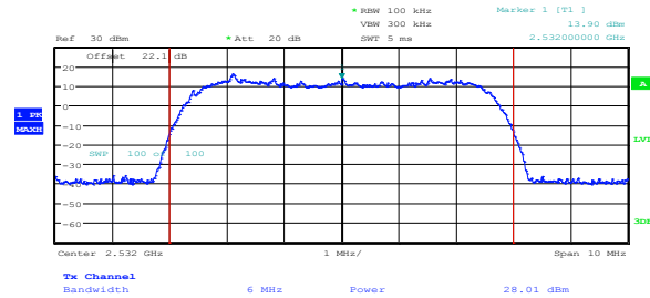
Figure 8.1-2: Conducted Peak power example
