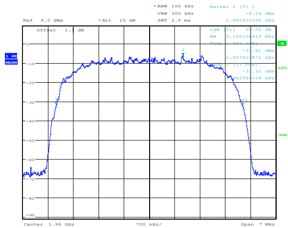
Figure 8.5-18: UMTS output
