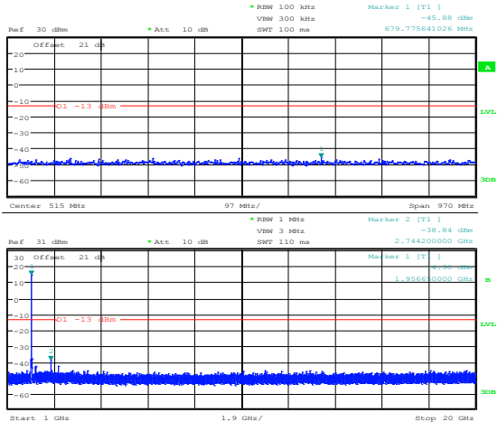
Figure 8.2-6: 5 MHz LTE QPSK 30 MHz – 20 GHz
