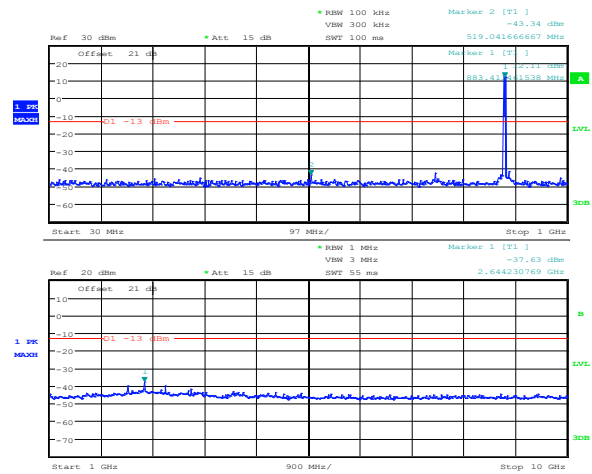
Figure 8.2-2: 1.4 MHz LTE QPSK 30 MHz –10 GHz
