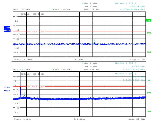
Figure 8.2-6: 5 MHz LTE QPSK 30 MHz – 22 GHz
