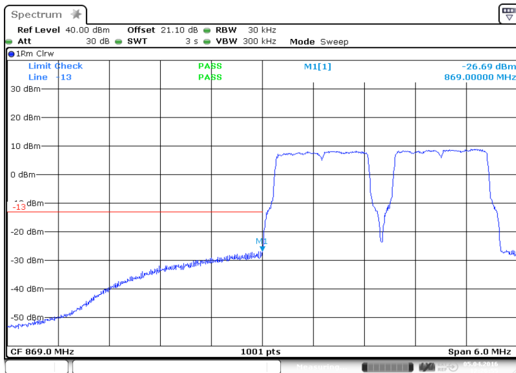
plot 8.3.2.1-#1 Intermodulation: §22.917, §2.1051; Test results; Uplink; Downlink LTE Lower Band Edge
