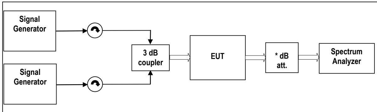
figure 8-#1 Test setup: Intermodulation: §22.917, §2.1051
