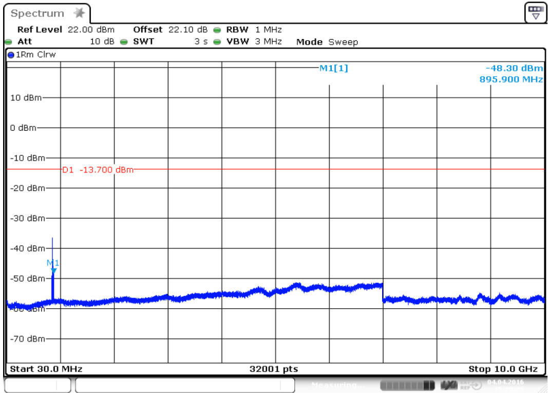
plot 7.3.2.1-#1 Spurious Emissions at Antenna Terminals: §22.917, §2.1051; Test results; Uplink; Downlink LTE; carrier (881.5MHz) notched
