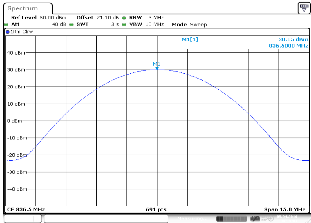
plot 5.3.2.2-#1 RF Power Out: §22.913, §2.1046; Test results; Uplink; LTE Uplink Middle
