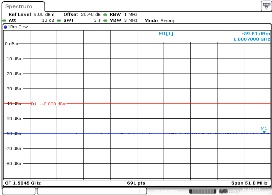
plot 7.3.2.3-#1 Spurious Emissions at Antenna Terminals: §27.53, §2.1051; Test results; Downlink Measurement in the band of 1559 MHz – 1610 MHz acc. to 27.53(f); LTE band 12
