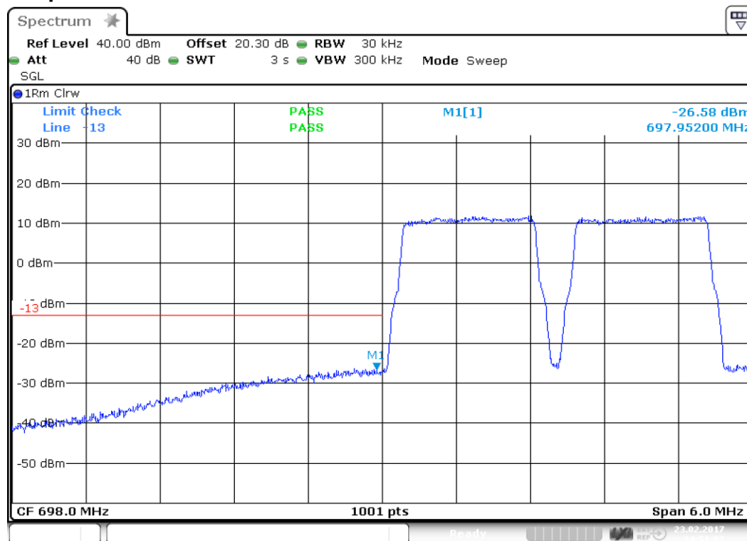
plot 8.3.2.3-#1 Intermodulation: §27.53, §2.1051; Test results; Uplink LTE 698 – 716MHz Lower Band Edge
