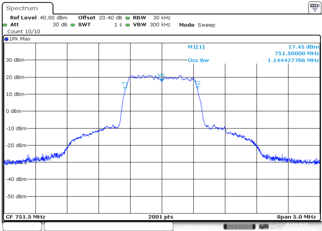
plot 6.3.2.2-#1 Occupied Bandwidth: $2.1049; Test results; Downlink LTE 746 – 757MHz Output
