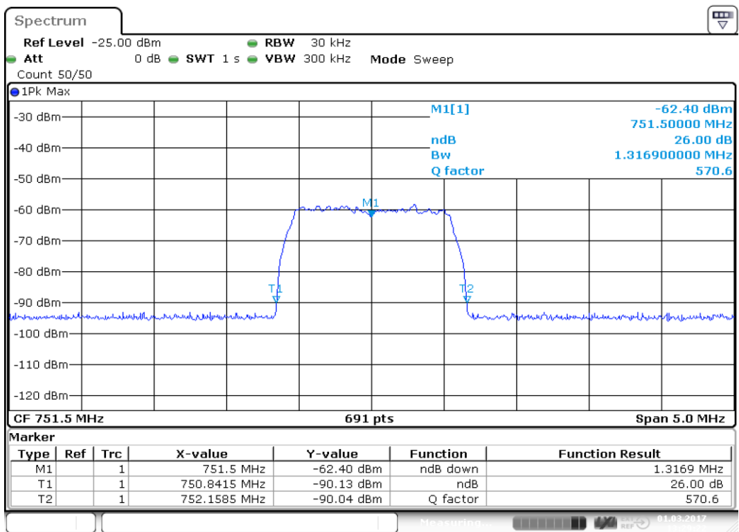
plot 6.3.3.2-#1 Occupied Bandwidth: $2.1049; Test results; 26 dB Bandwidth; Downlink LTE 746 – 757MHz Output
