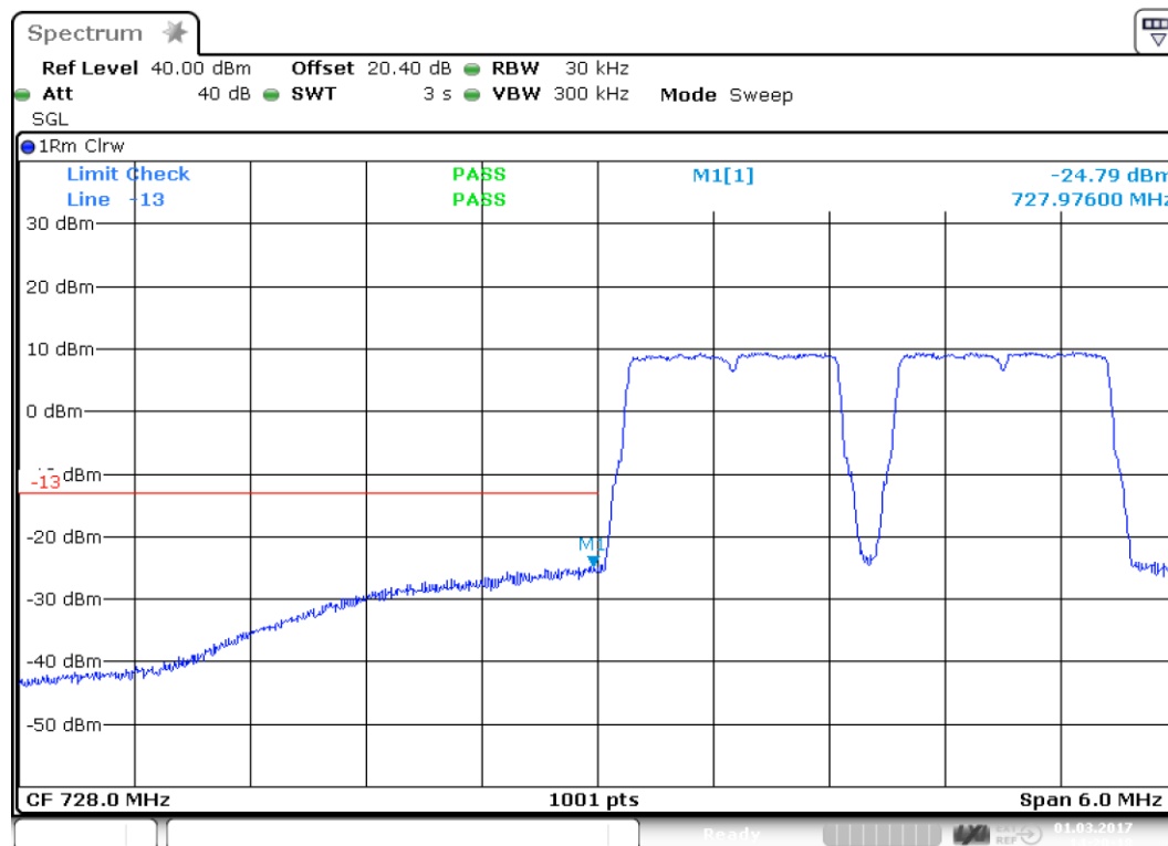
plot 8.3.2.1-#1 Intermodulation: §27.53, §2.1051; Test results; Downlink LTE 728 – 746MHz Lower Band Edge
