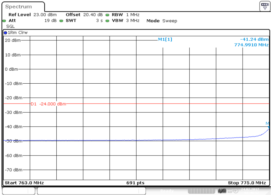
plot 7.3.2.5-#2 Spurious Emissions at Antenna Terminals: §27.53, §2.1051; Test results; Uplink LTE 776 – 787MHz; 763 MHz – 775 MHz
