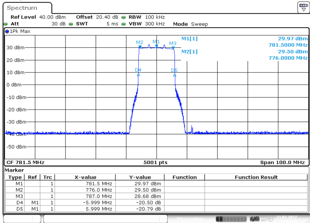
plot 8.3.2-#1 Out of Band Rejection; Test results;Uplink 776 – 787MHz;
