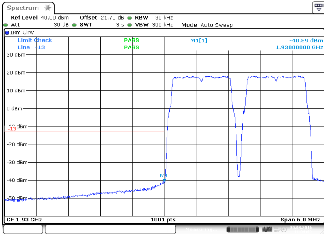
plot 8.3.2.1-#1 Intermodulation: §24.238, §2.1051; Test results; Uplink; Downlink LTE Lower Band Edge
