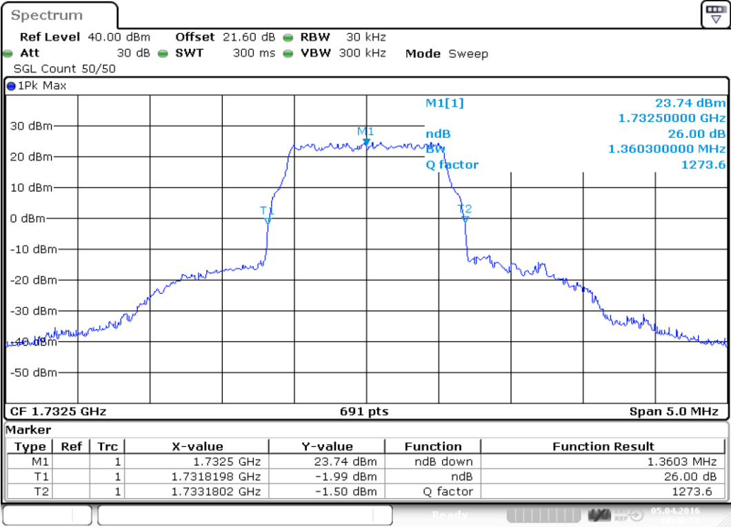
plot 6.3.3.2-#1 Occupied Bandwidth: $2.1049; Test results; 26dB Bandwidth; Uplink LTE Output
