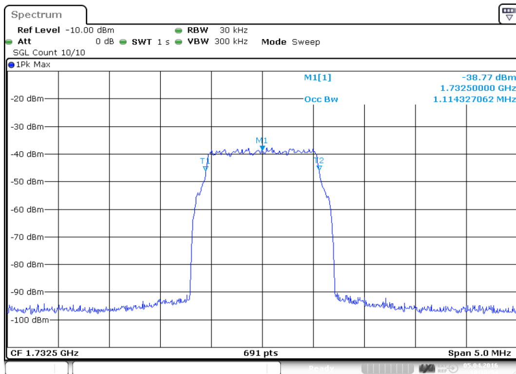
plot 6.3.2.2-#1 Occupied Bandwidth: $2.1049; Test results; Uplink; Uplink LTE Output
