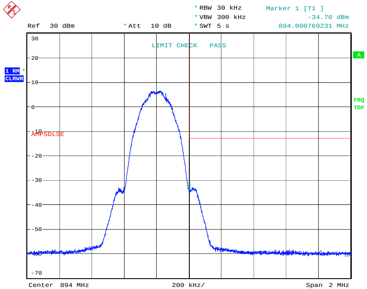
Figure 46 Band Edge Spurious with Single Carrier - EDGE - Downlink
