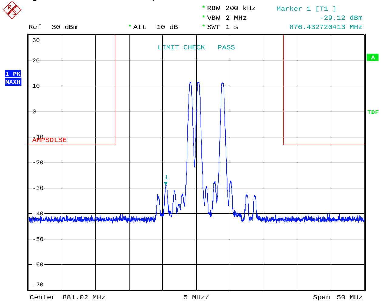
Figure 29 Intermodulation Spurious - EDGE - Downlink
