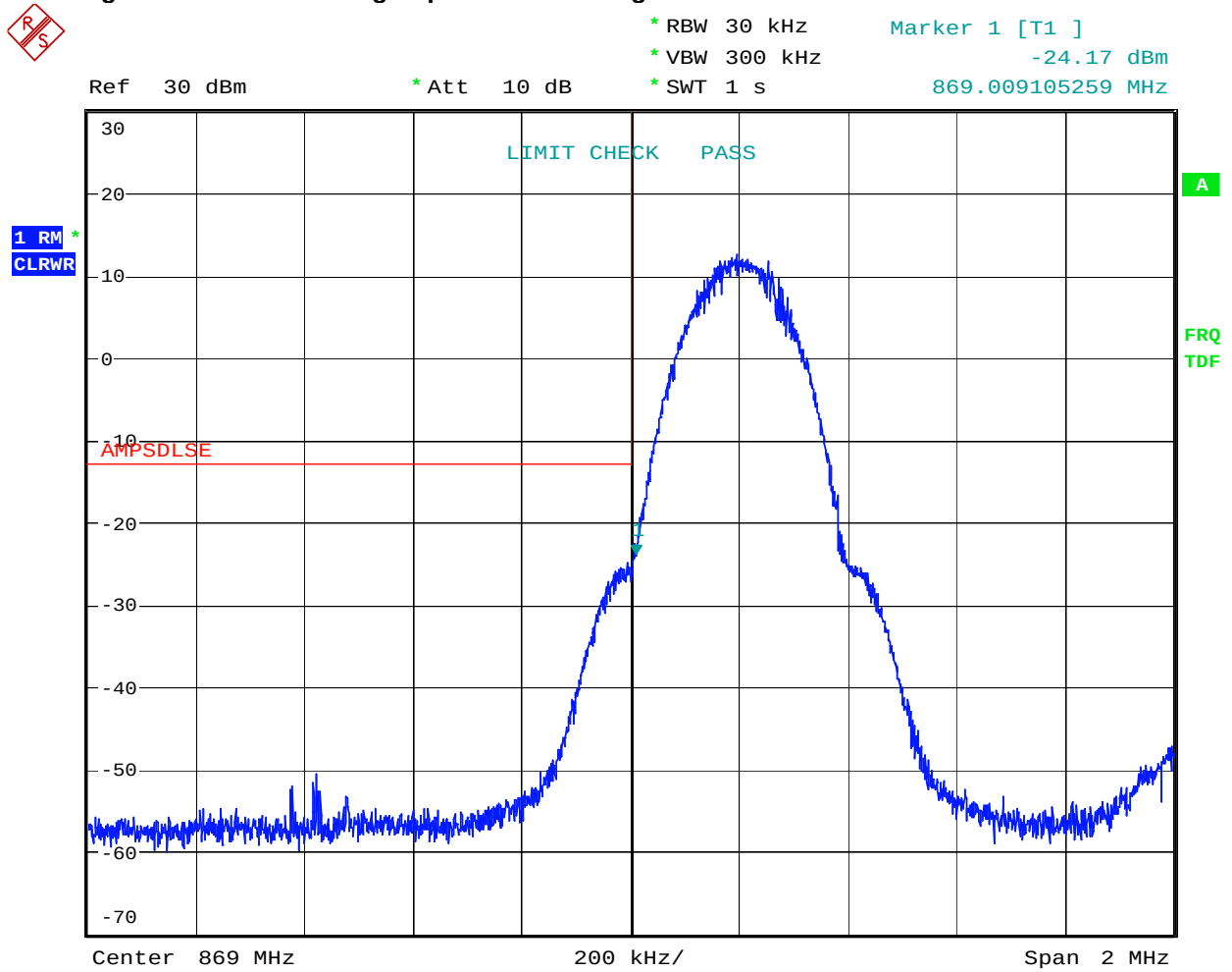
Figure 41 Band Edge Spurious with Single Carrier - GSM - Downlink
