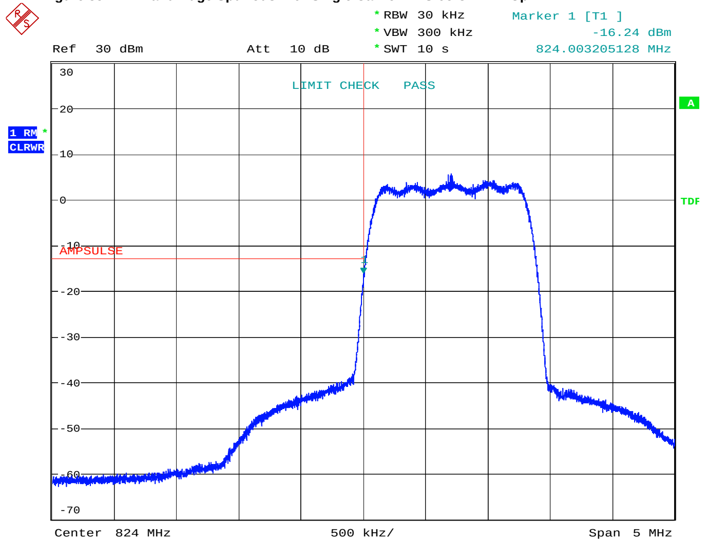
Figure 35 Band Edge Spurious with Single Carrier - IS-95 CDMA - Uplink
