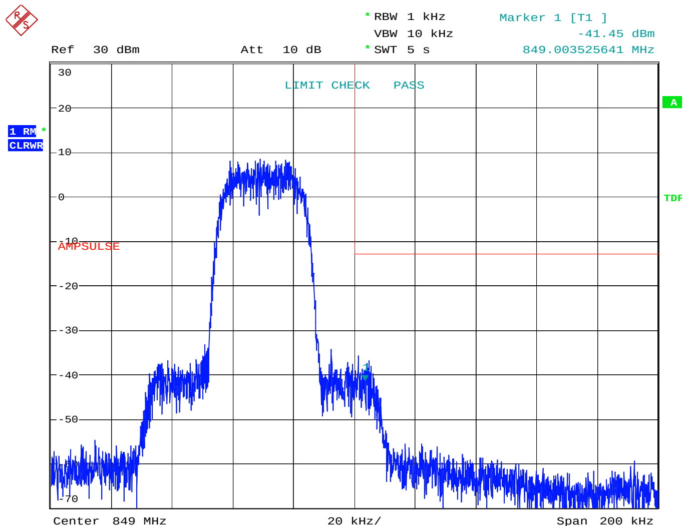
Figure 52 Band Edge Spurious with Single Carrier - TDMA - Uplink
