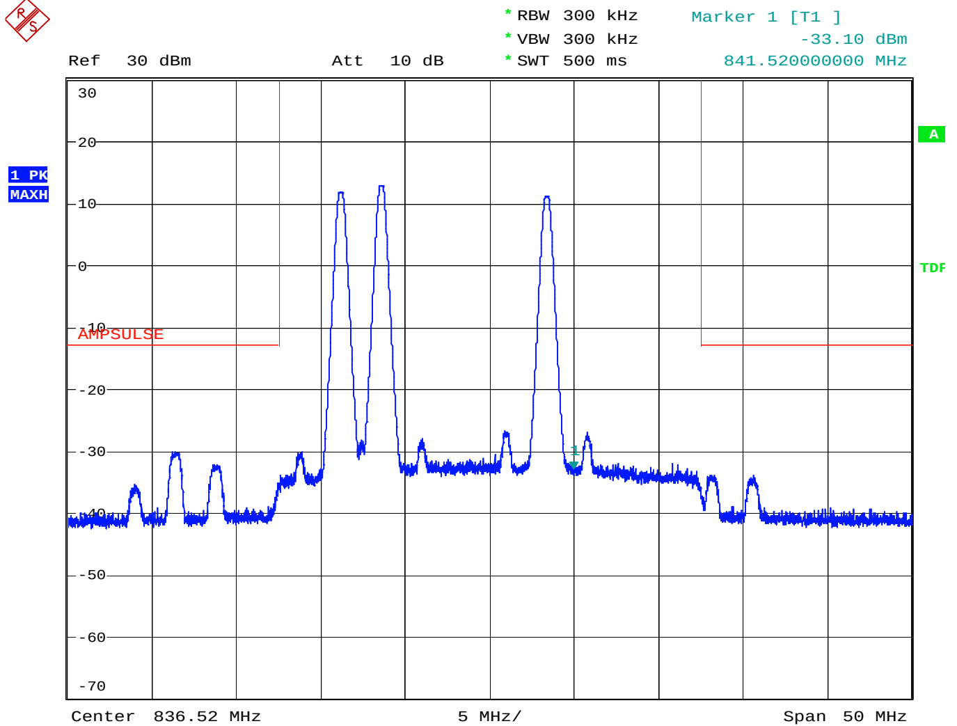
Figure 30 Intermodulation Spurious - EDGE - Uplink
