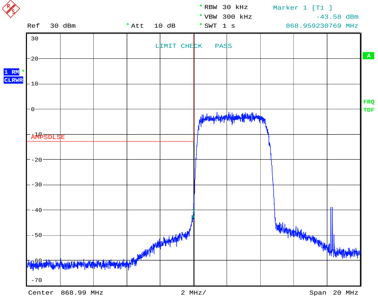
Figure 37 Band Edge Spurious with Single Carrier - W-CDMA - Downlink
