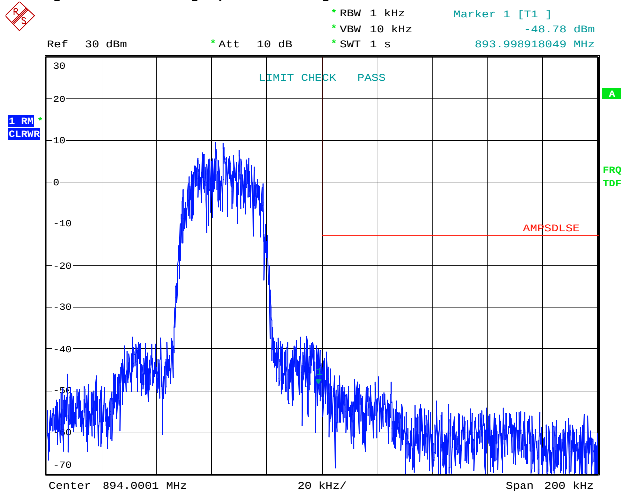
Figure 50 Band Edge Spurious with Single Carrier - TDMA - Downlink
