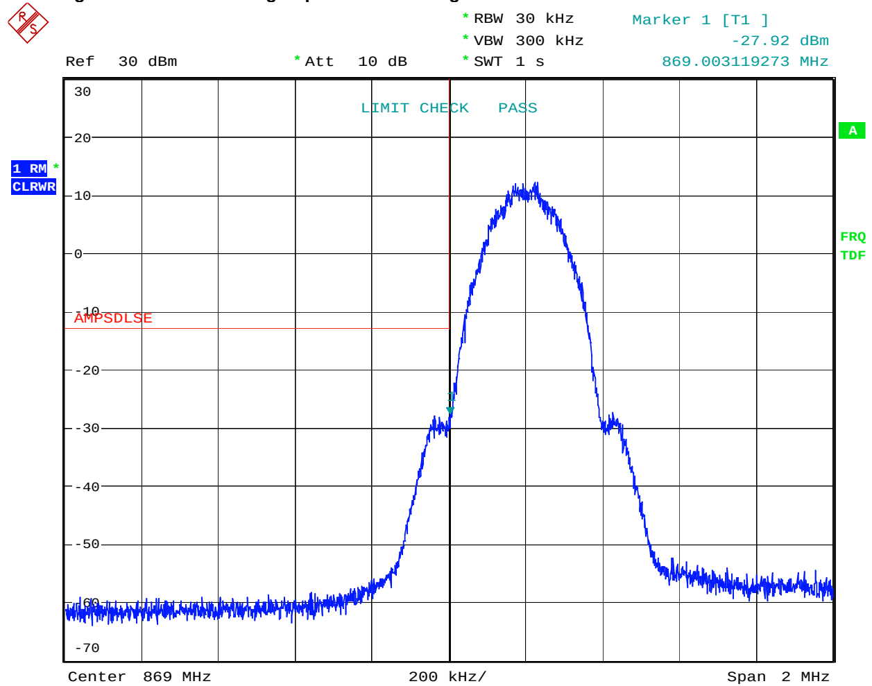
Figure 45 Band Edge Spurious with Single Carrier - EDGE - Downlink
