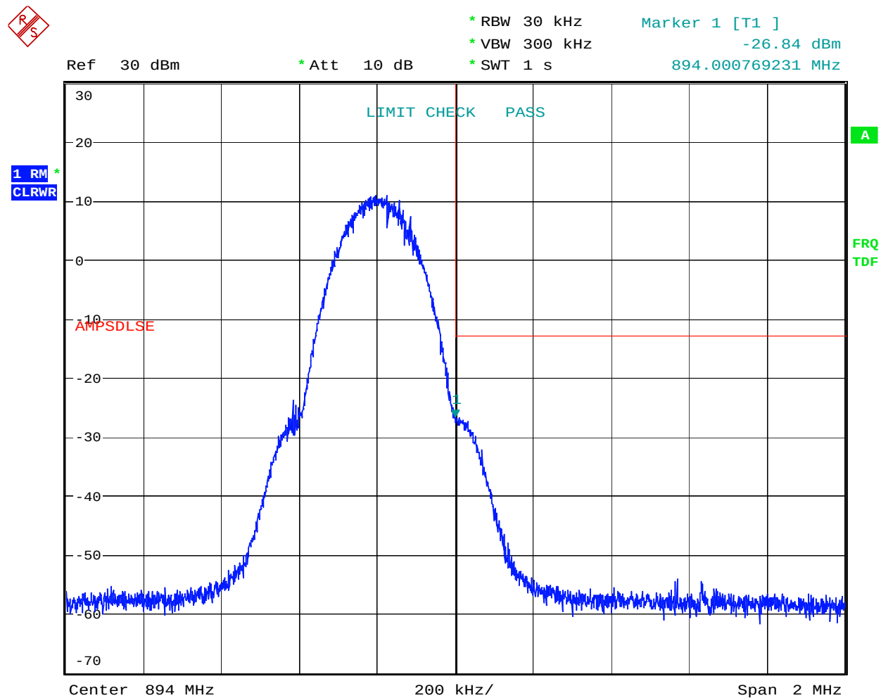
Figure 42 Band Edge Spurious with Single Carrier - GSM - Downlink
