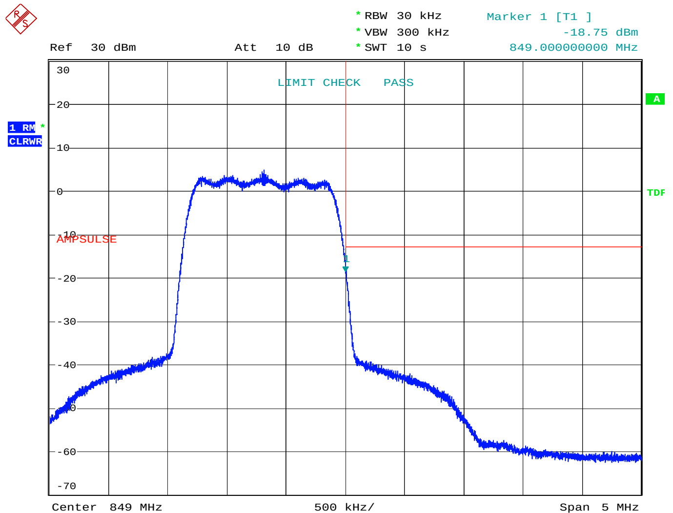
Figure 36 Band Edge Spurious with Single Carrier - IS-95 CDMA - Uplink
