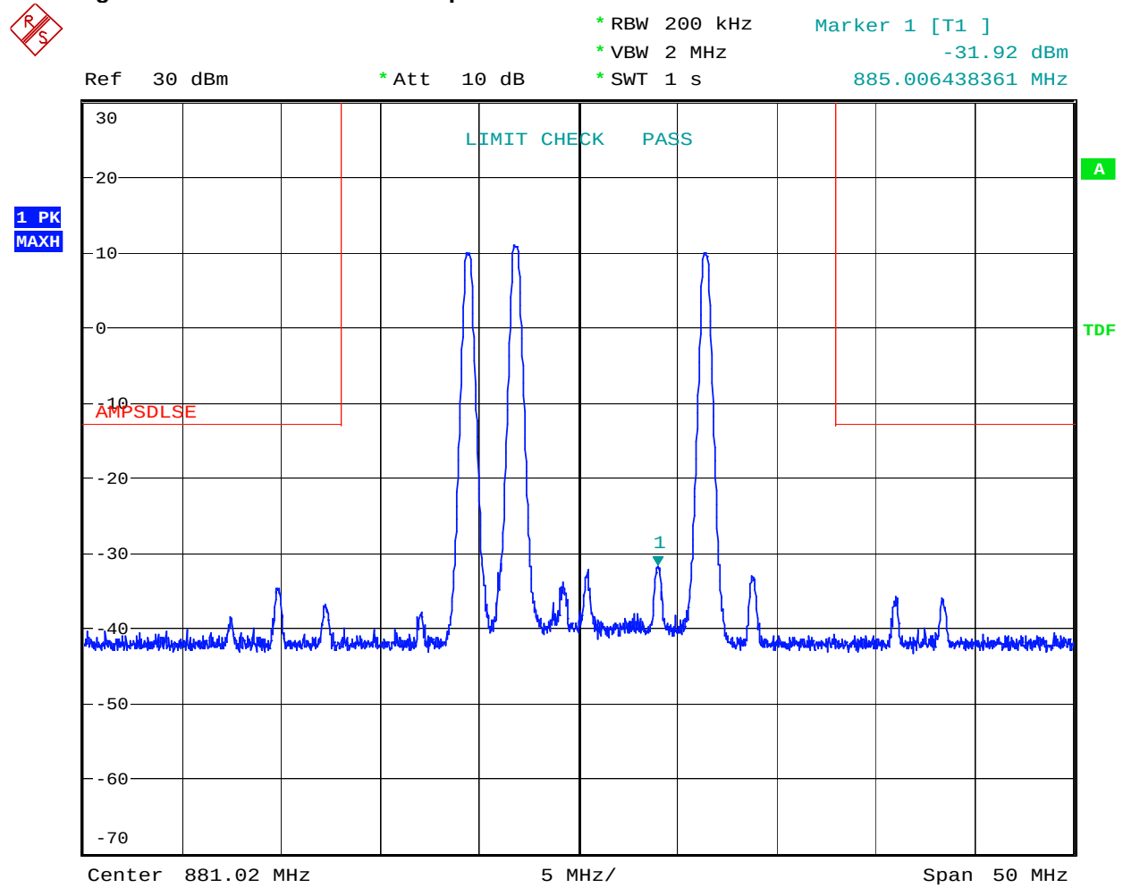
Figure 31 Intermodulation Spurious - TDMA - Downlink
