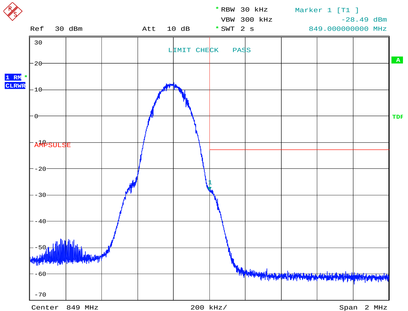
Figure 44 Band Edge Spurious with Single Carrier - GSM - Uplink
