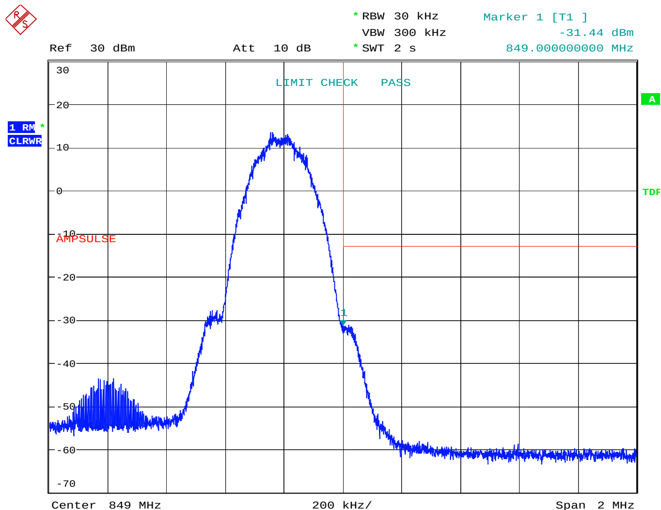
Figure 48 Band Edge Spurious with Single Carrier - EDGE - Uplink
