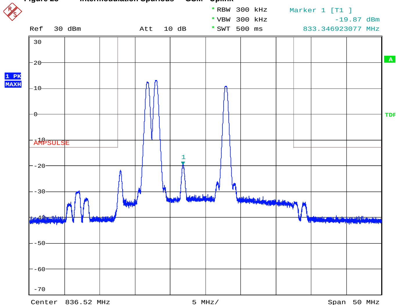
Figure 28 Intermodulation Spurious - GSM - Uplink
