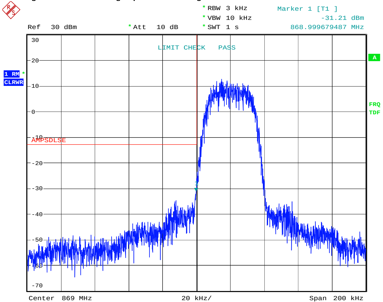
Figure 49 Band Edge Spurious with Single Carrier - TDMA - Downlink
