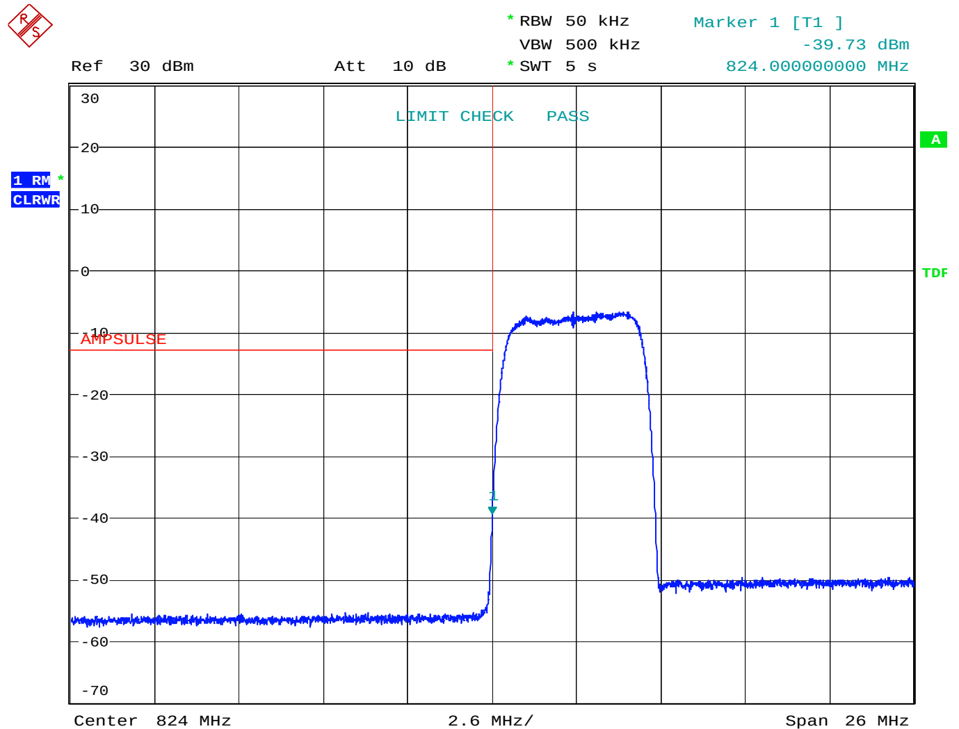
Figure 39 Band Edge Spurious with Single Carrier - W-CDMA – Uplink
