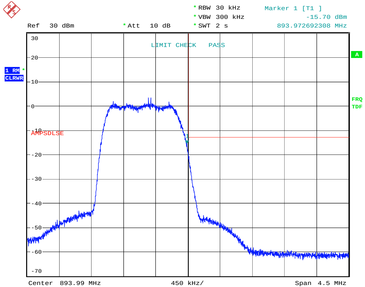
Figure 34 Band Edge Spurious with Single Carrier - IS-95 CDMA - Downlink
