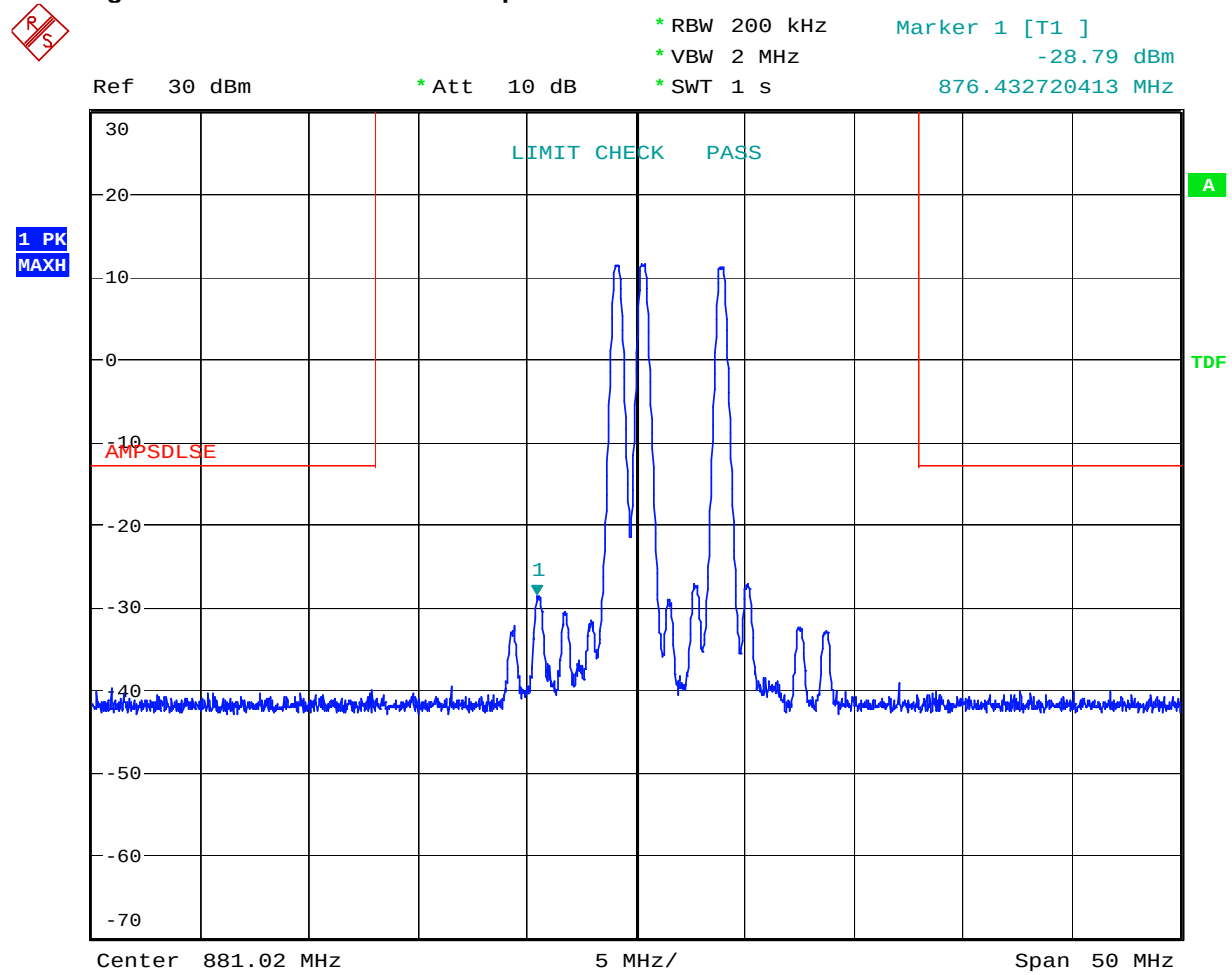
Figure 27 Intermodulation Spurious - GSM - Downlink
