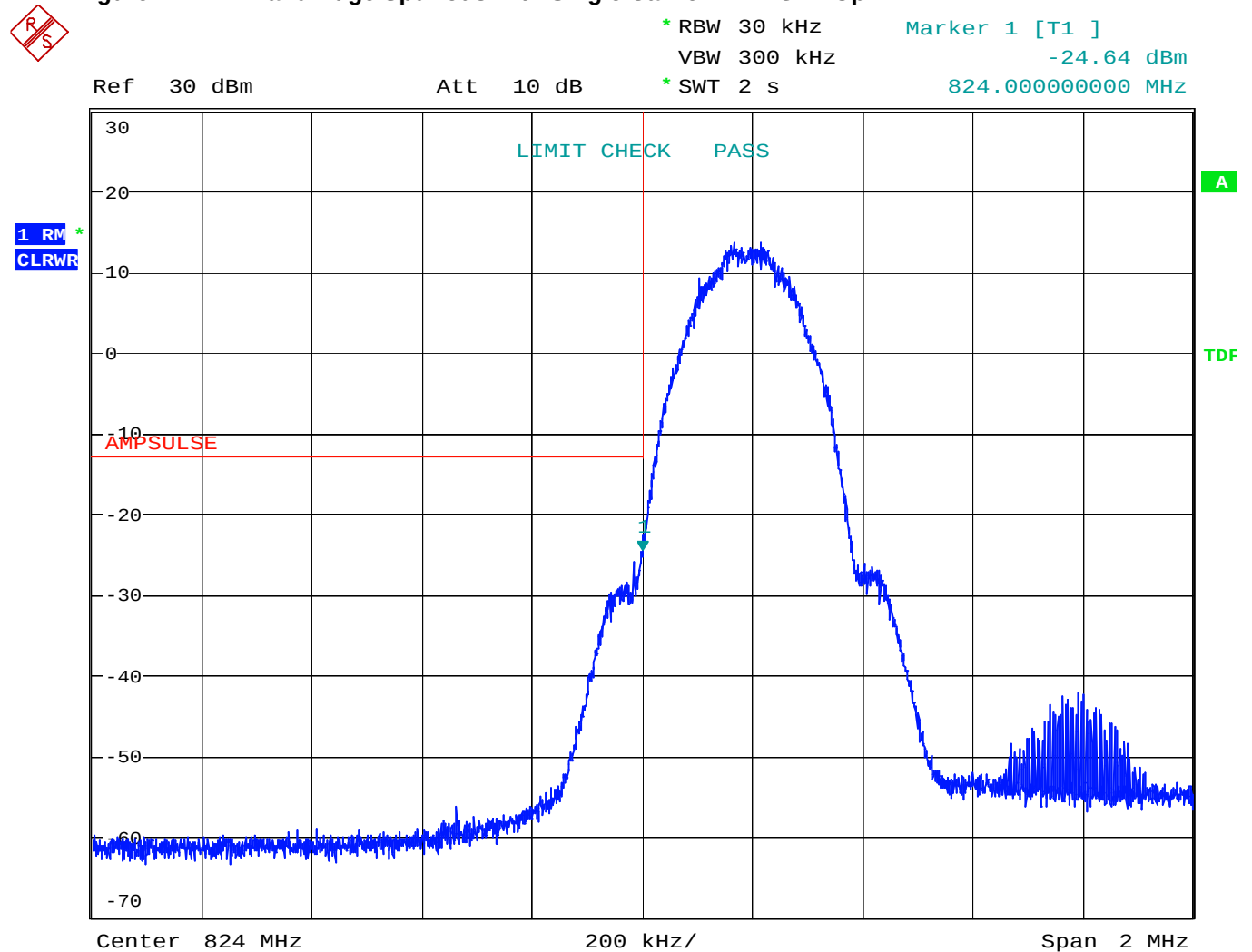
Figure 47 Band Edge Spurious with Single Carrier - EDGE - Uplink
