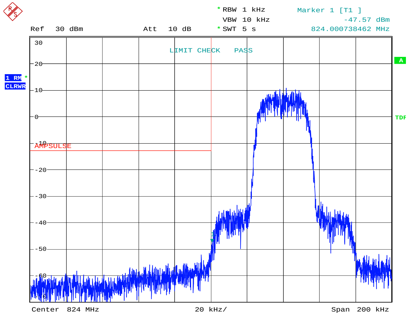
Figure 51 Band Edge Spurious with Single Carrier - TDMA - Uplink
