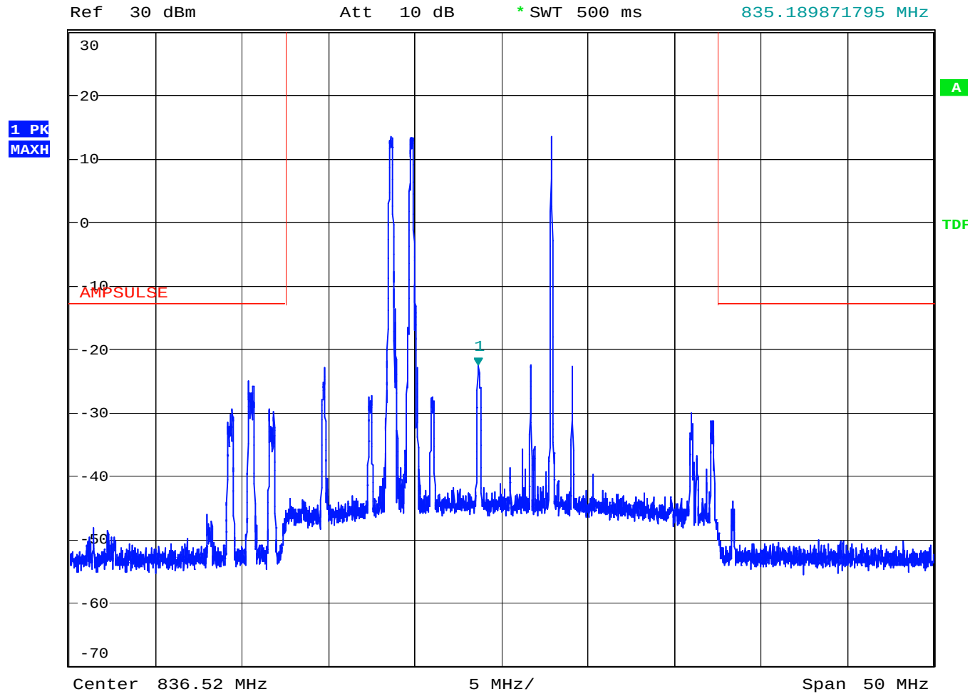
Figure 32 Intermodulation Spurious - TDMA - Uplink
