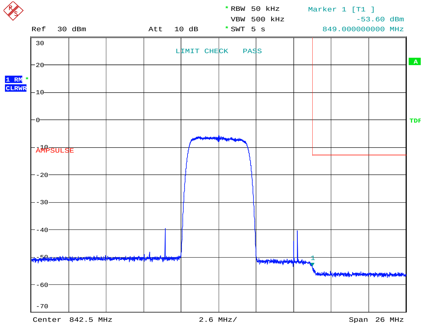
Figure 40 Band Edge Spurious with Single Carrier - W-CDMA – Uplink
