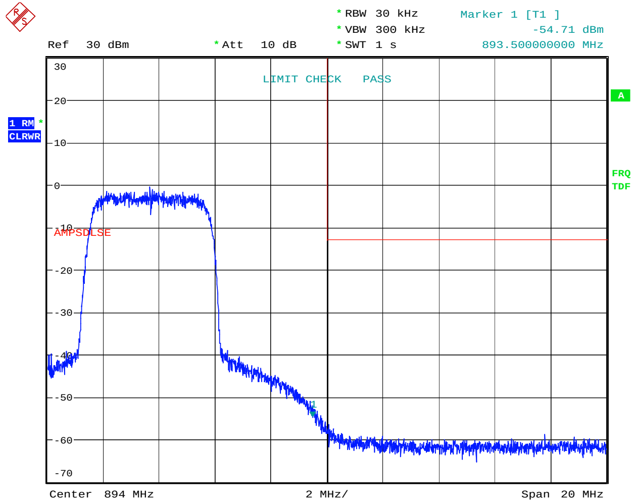
Figure 38 Band Edge Spurious with Single Carrier - W-CDMA - Downlink
