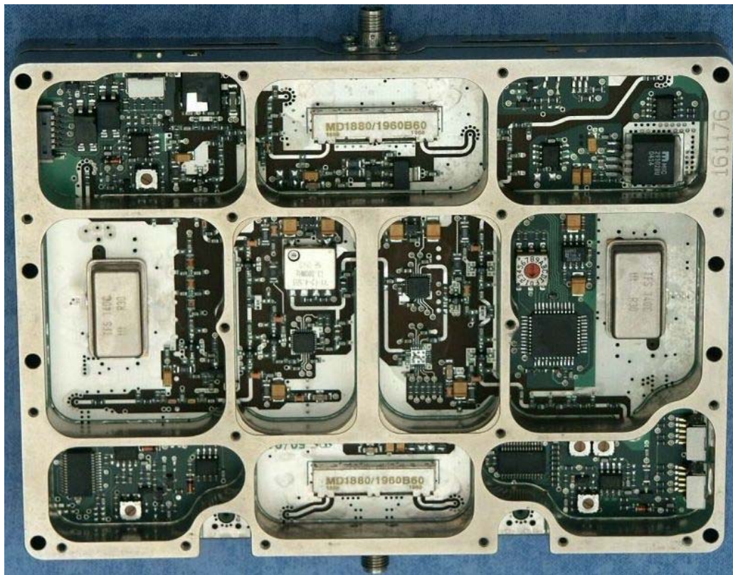
PCB – Top
