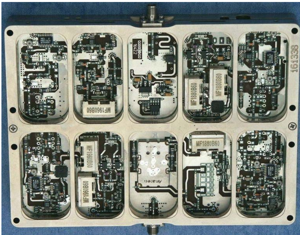
PCB – Bottom
