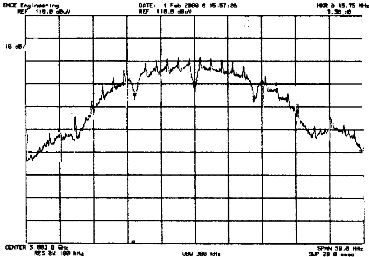
FIGURE 1 BANDWIDTH
