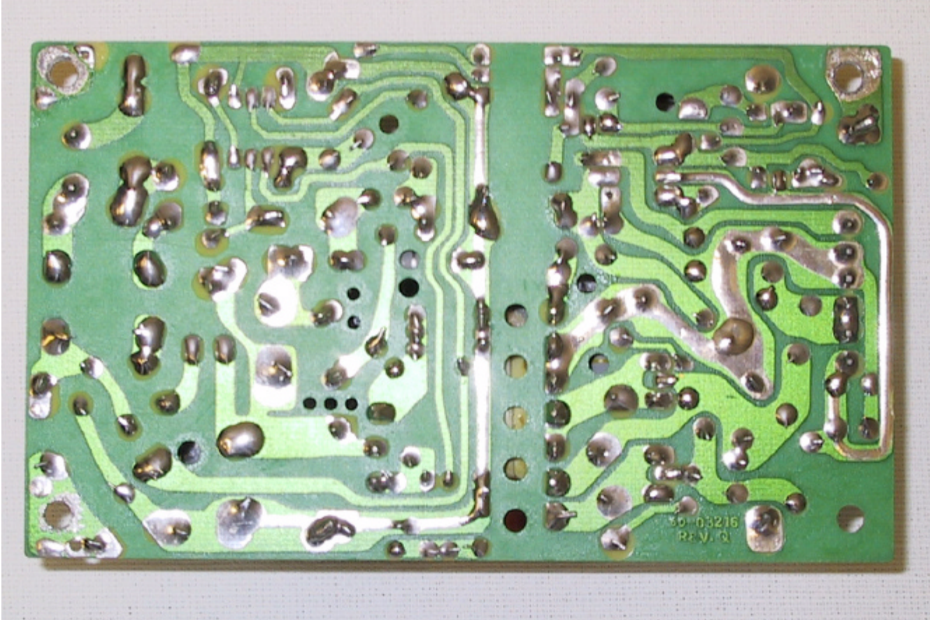
BOTTOM VIEW
