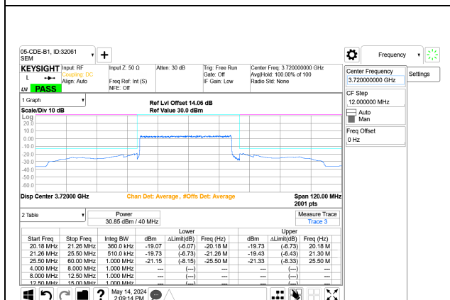
5G NR n77 40MHz BPSK Low Channel RB105-0 Port A+B
