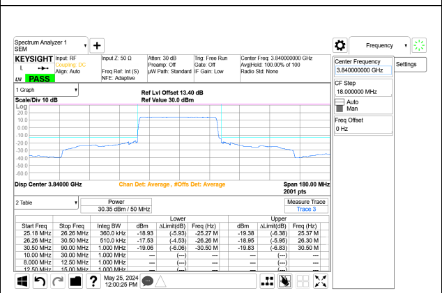
5G NR n77 50MHz BPSK Mid Channel RB128-0 Port A+B, ID: 32546
