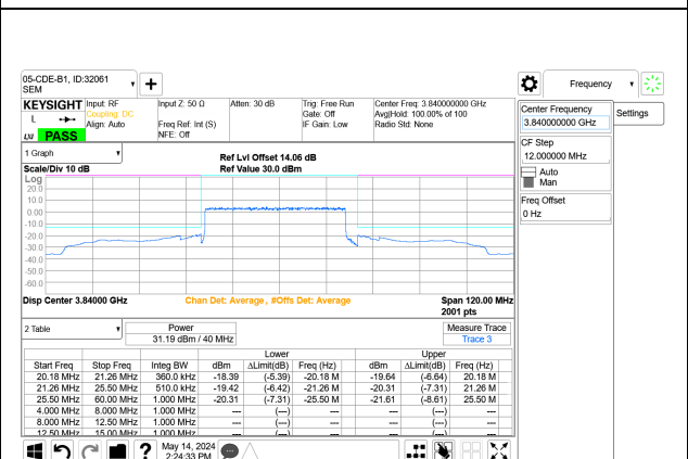
5G NR n77 40MHz BPSK Mid Channel RB105-0 Port A+B
