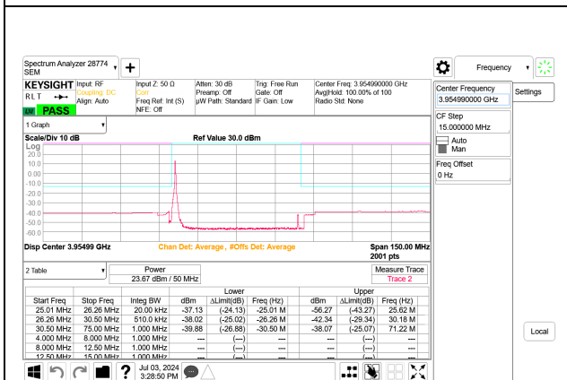
5G NR n77 50MHz BPSK High Channel RB1-0 Port B
