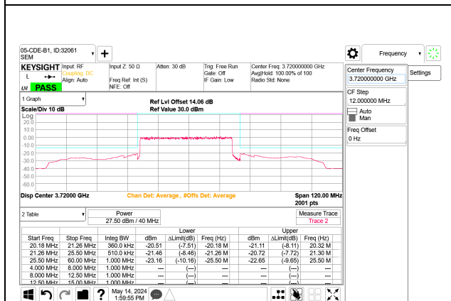
5G NR n77 40MHz BPSK Low Channel RB105-0 Port B
