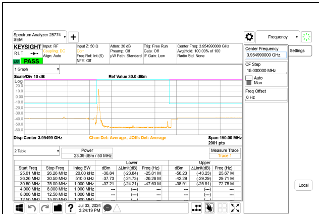
5G NR n77 50MHz BPSK High Channel RB1-0 Port A
