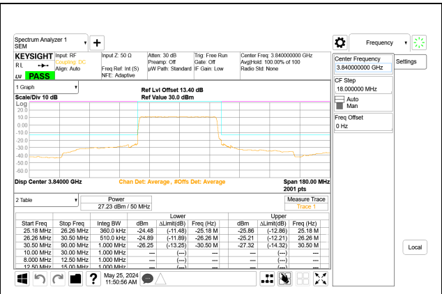
5G NR n77 50MHz BPSK Mid Channel RB128-0 Port A, ID: 32546
