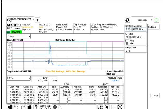
5G NR n77 50MHz BPSK High Channel RB1-0 Port A+B
