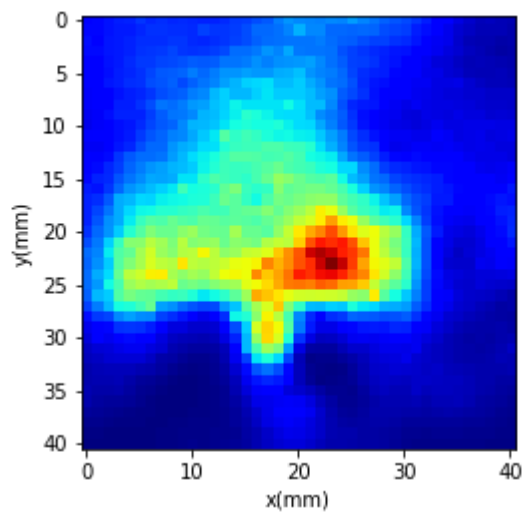
Power Density Plots for Beam ID:149
