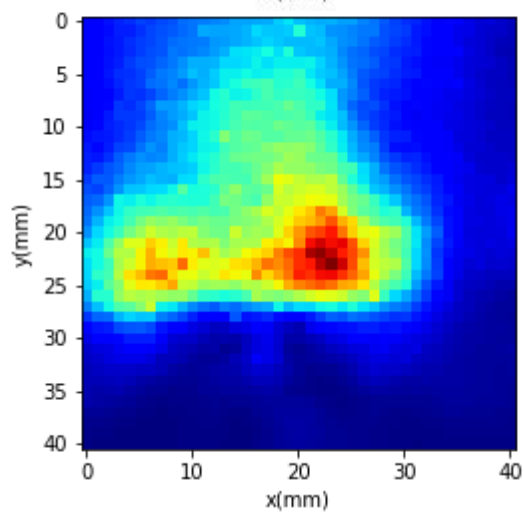
Power Density Plots for Beam ID:141
