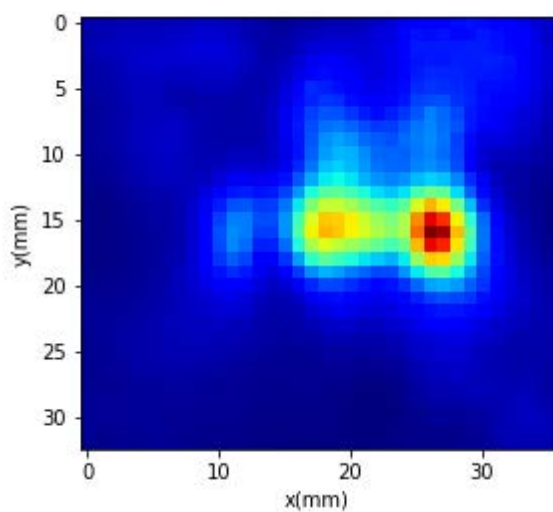
Power Density Plots for Beam ID:18
