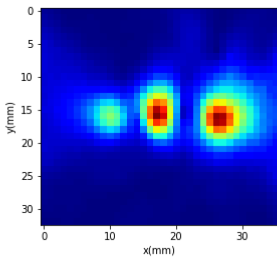
Power Density Plots for Beam ID:157
