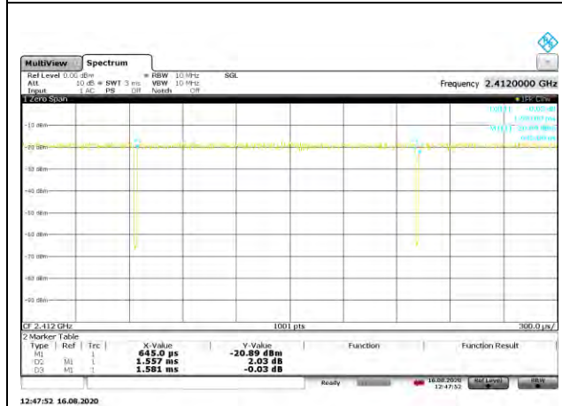
DUTY CYCLE 802.11ax HE20 2Tx MCS0
