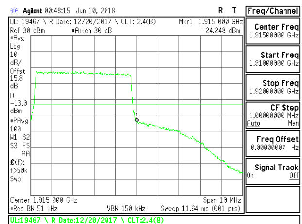
LTE B25 5MHz 16QAM High Channel RB25-0
