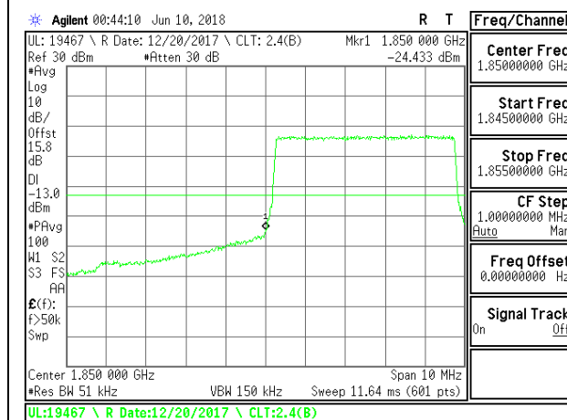
LTE B25 5MHz 16QAM Low Channel RB25-0
