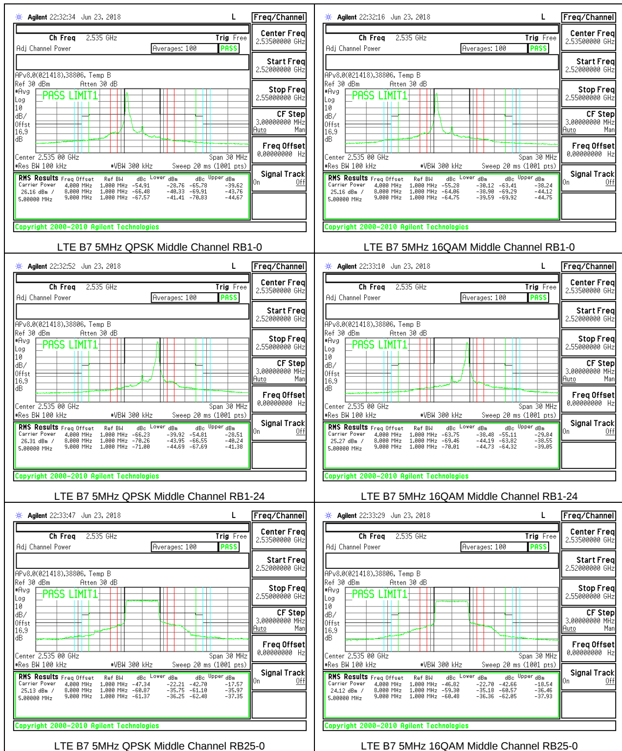
LTE B7 5MHz QPSK Middle Channel RB25-0
