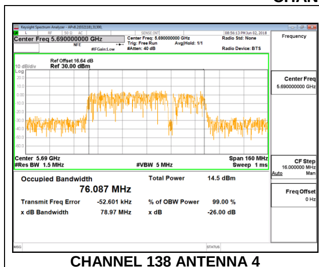
HIGH CHANNEL ANTENNA 4
