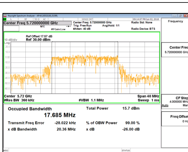
CHANNEL 144 ANTENNA 5
