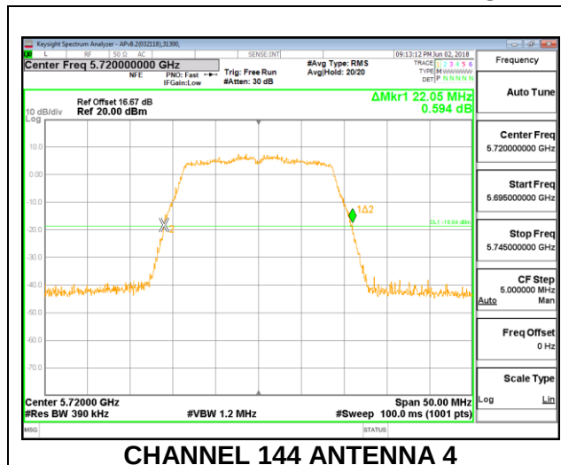
CHANNEL 144 ANTENNA 4
