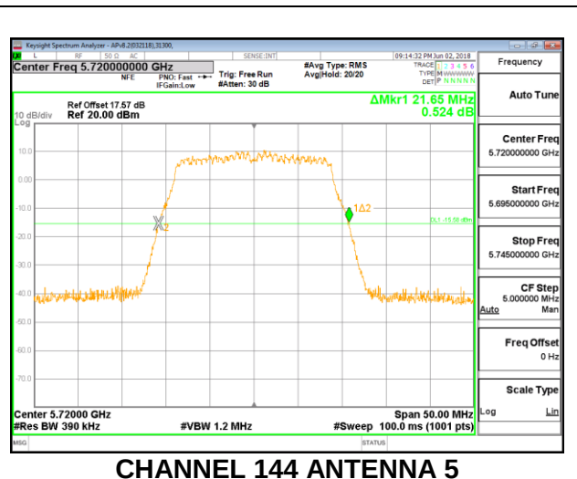
CHANNEL 144 ANTENNA 5
