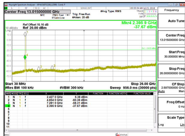
OUT-OF-BAND LOW CHANNEL 4 ANTENNA 5
