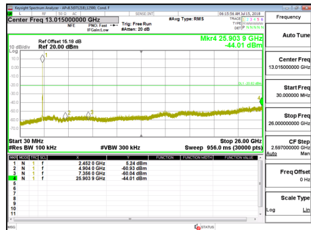
OUT-OF-BAND HIGH CHANNEL 9 ANTENNA 5
