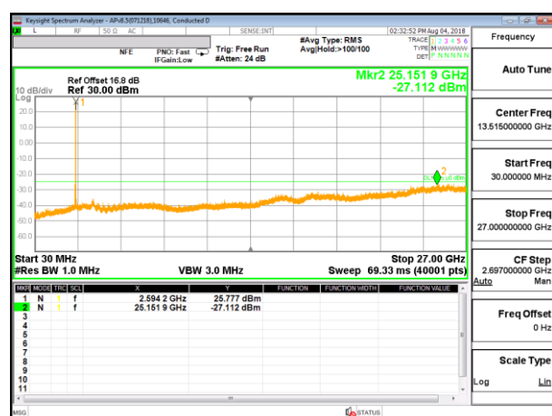
LTE B41 20MHz + 20MHz 16OAM Middle Ch RB1-99 + RB1-0
