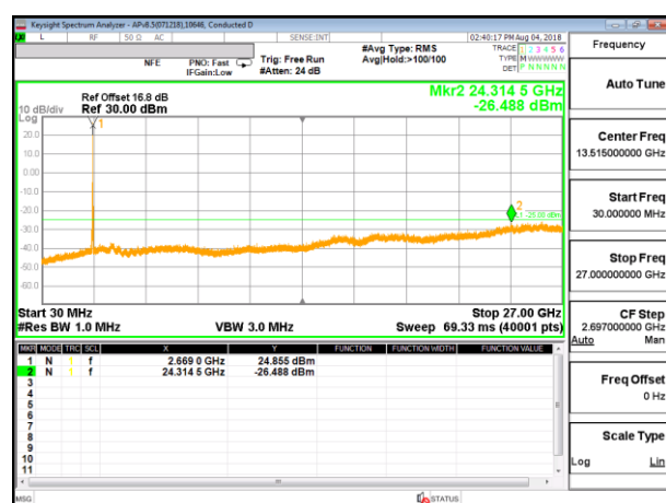
LTE B41 20MHz + 20MHz 16OAM High Ch RB1-99 + RB1-0
