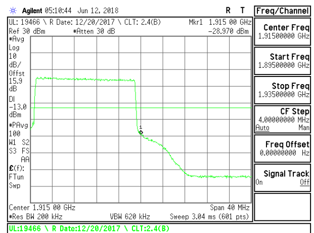
LTE B25 20MHz 16QAM High Channel RB100-0
