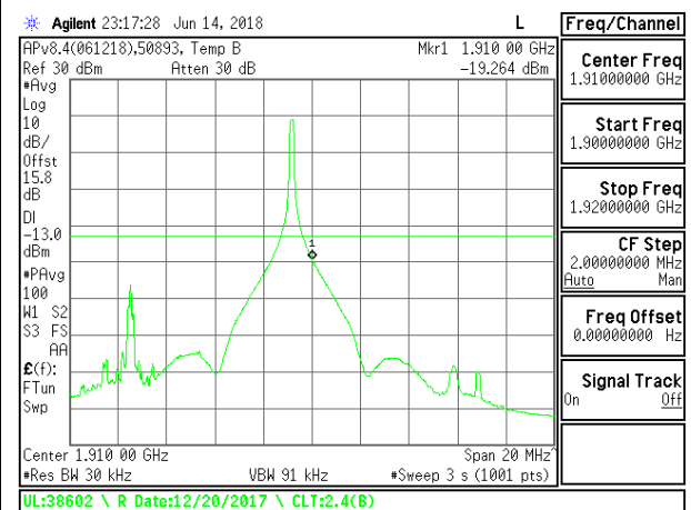
LTE B2 15MHz QPSK High Channel RB1-74
