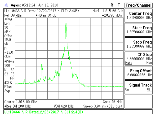
LTE B25 20MHz 16QAM High Channel RB1-99
