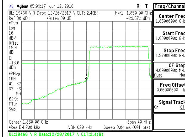
LTE B25 20MHz 16QAM Low Channel RB100-0
