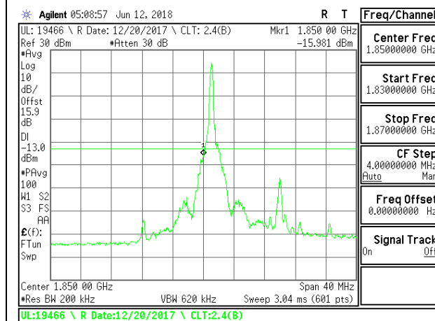
LTE B25 20MHz 16QAM Low Channel RB1-0
