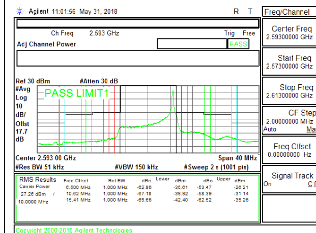
LTE B41 10MHz QPSK Middle Channel RB1-49
