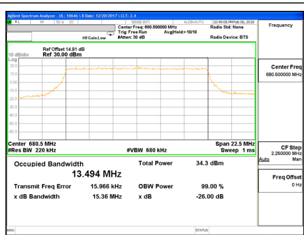
LTE B71 15MHz 16QAM Middle Channel RB75-0
