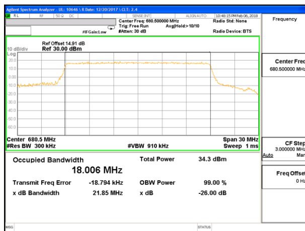
LTE B71 20MHz 16QAM Middle Channel RB100-0
