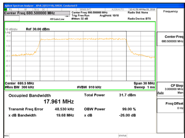
LTE B71 20MHz 64QAM Middle Channel RB100-0
