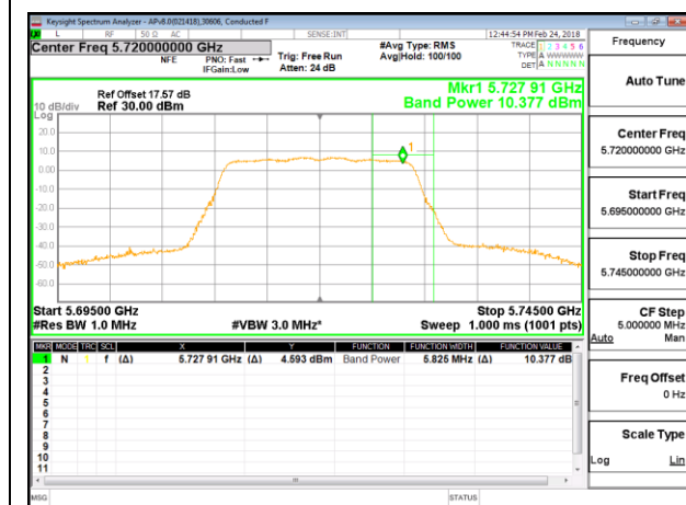
CHANNEL 144 ANT 5 POWER
