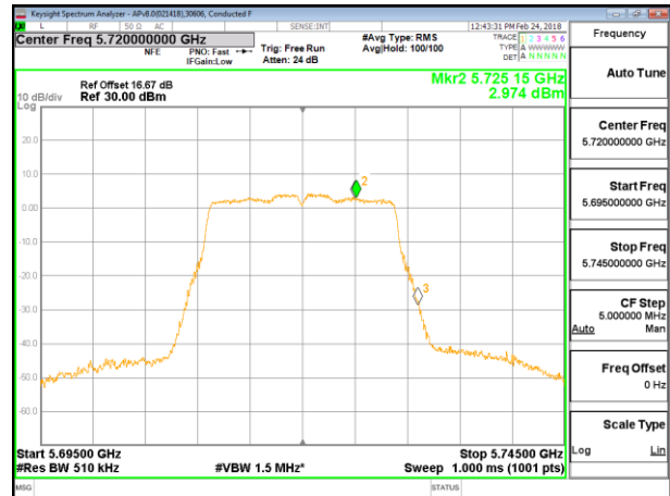
CHANNEL 144 ANT 6 PSD
