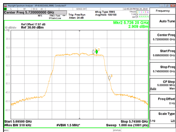
CHANNEL POWER ANT 5 PSD
