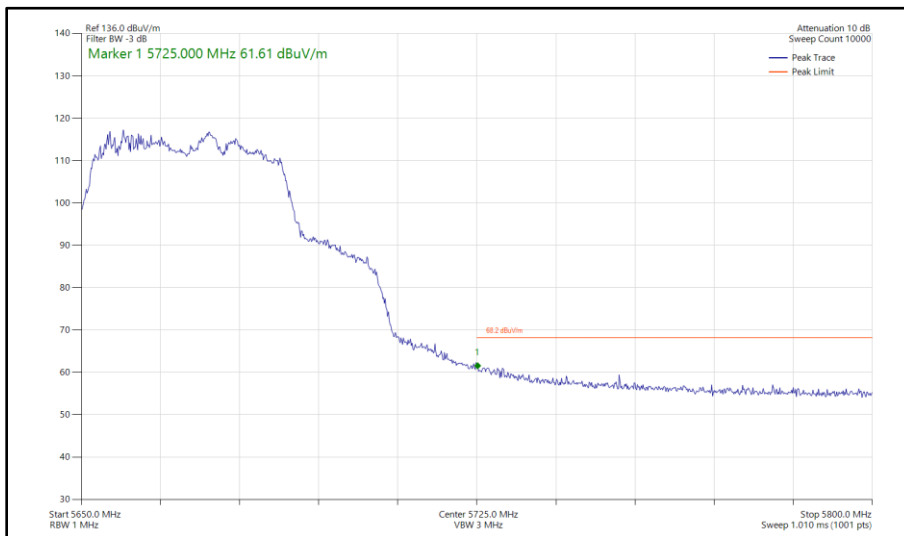
Figure 372 - 802.11ac VHT40, TxBF, Core 0 - Core 1 - 5670 MHz Band Edge Frequency 5725 MHz
