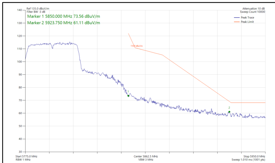
Figure 341 - 802.11n HT40, SISO, Core 1 - 5795 MHz Band Edge Frequency 5850 MHz
