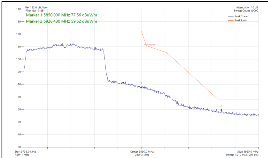
Figure 385 - 802.11ac VHT80, SISO, Core 0 - 5775 MHz Band Edge Frequency 5850 MHz
