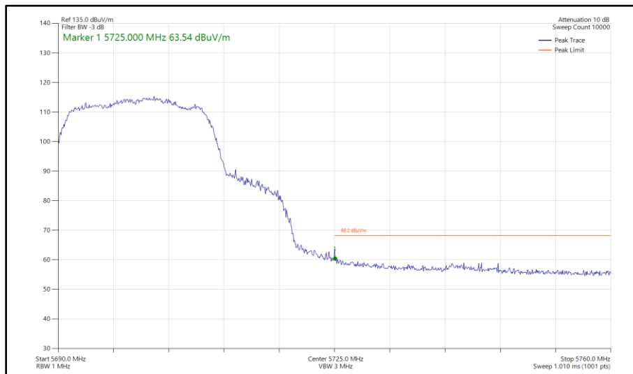
Figure 318 - 802.11ac VHT20, TxBF, Core 0 - Core 1 - 5700 MHz Band Edge Frequency 5725 MHz
