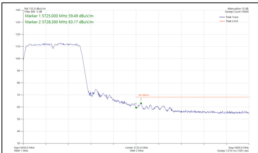
Figure 362 - 802.11n HT40, SDM, Core 0 - Core 1 - 5670 MHz Band Edge Frequency 5725 MHz
