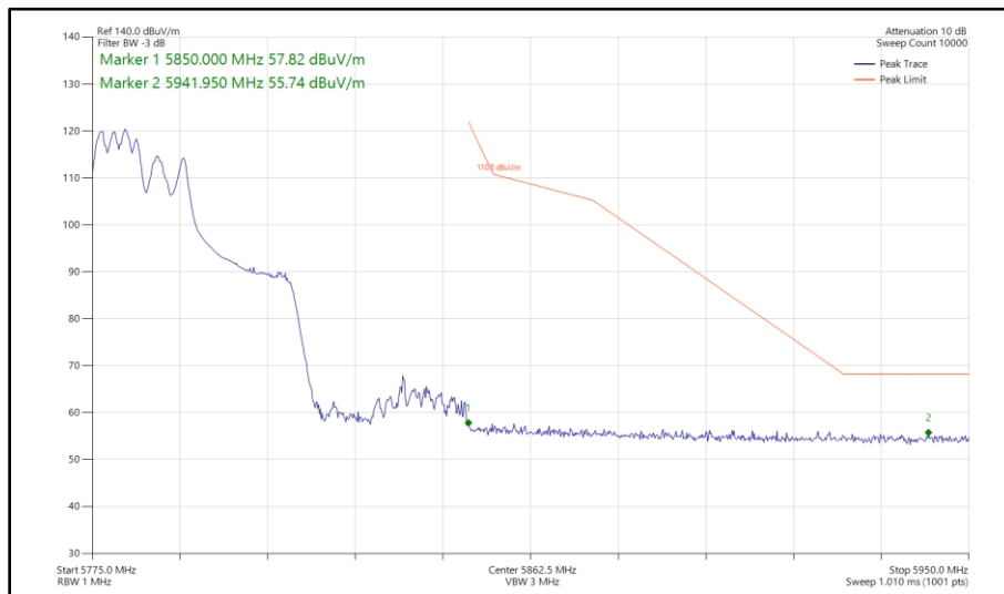
Figure 367 - 802.11ax HE40, RU 106-53, SDM, Core 0 - Core 1 - 5795 MHz Band Edge Frequency 5850 MHz
