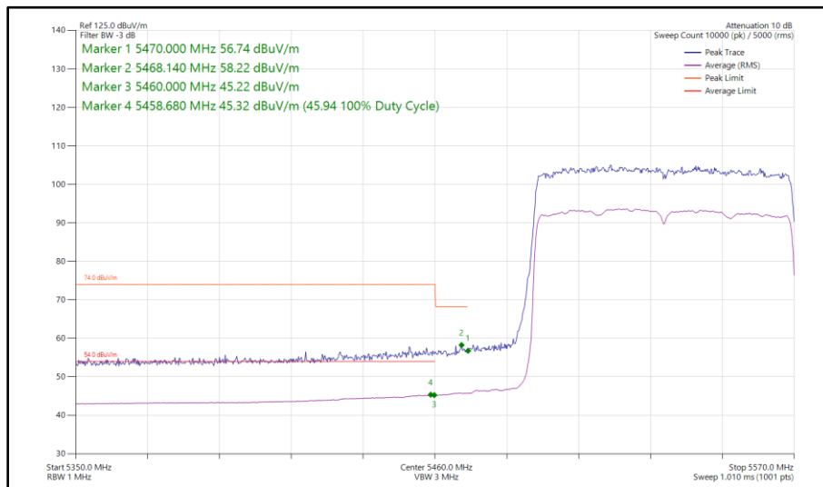
Figure 389 - 802.11ax HE80, SU, SISO, Core 1 - 5530 MHz Band Edge Frequency 5470 MHz
