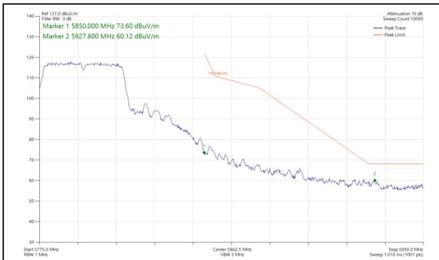
Figure 365 - 802.11n HT40, SDM, Core 0 - Core 1 - 5795 MHz Band Edge Frequency 5850 MHz
