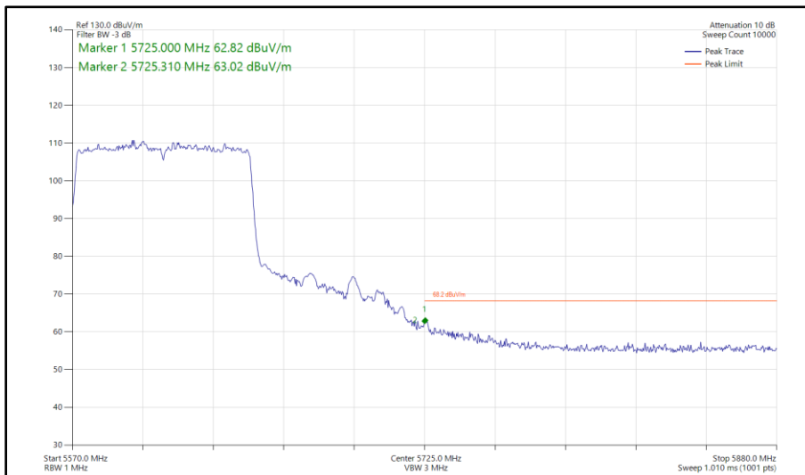
Figure 394 - 802.11ac VHT80, SISO, Core 1 - 5610 MHz Band Edge Frequency 5725 MHz
