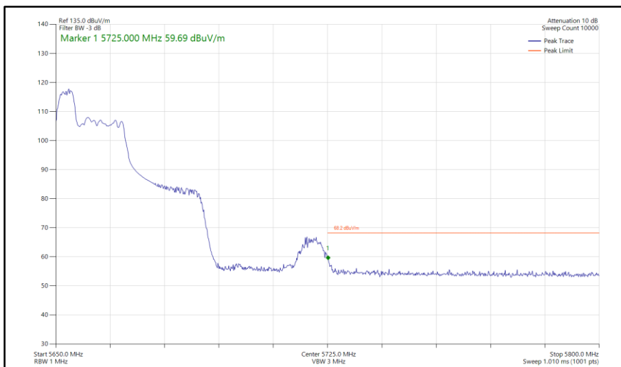
Figure 328 - 802.11ax HE40, RU 52-37, SISO, Core 0 - 5670 MHz Band Edge Frequency 5725 MHz
