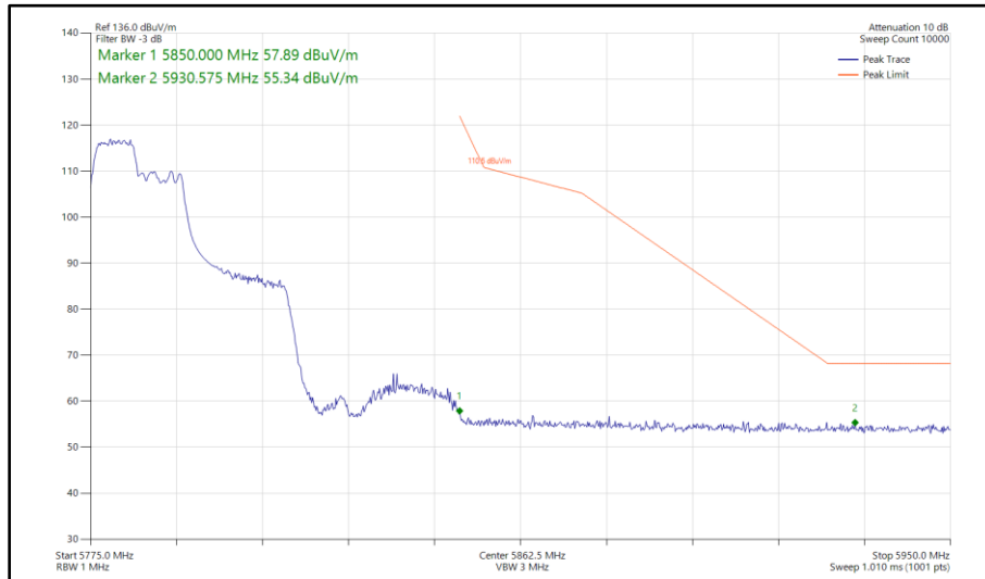
Figure 331 - 802.11ax HE40, RU 106-53, SISO, Core 0 - 5795 MHz Band Edge Frequency 5850 MHz
