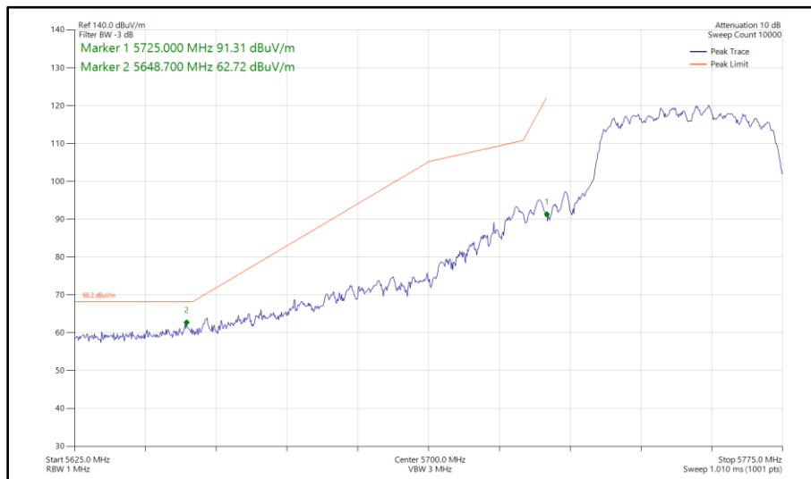
Figure 347 - 802.11n HT40, CDD, Core 0 - Core 1 - 5755 MHz Band Edge Frequency 5725 MHz
