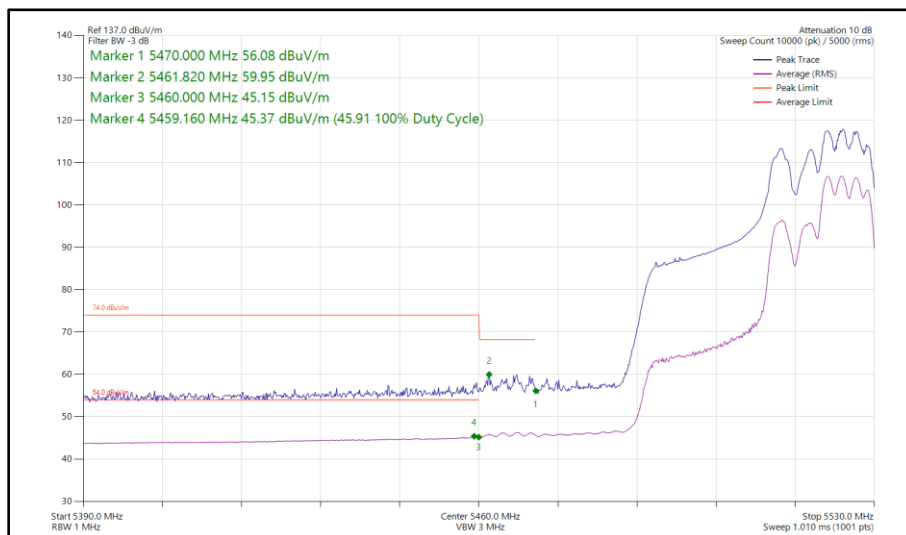
Figure 346 - 802.11ax HE40, RU 106-56, CDD, Core 0 - Core 1 - 5510 MHz Band Edge Frequency 5470 MHz
