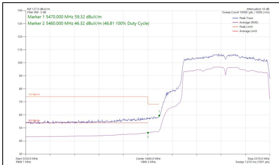
Figure 376 - 802.11ac VHT80, SISO, Core 0 - 5530 MHz Band Edge Frequency 5470 MHz
