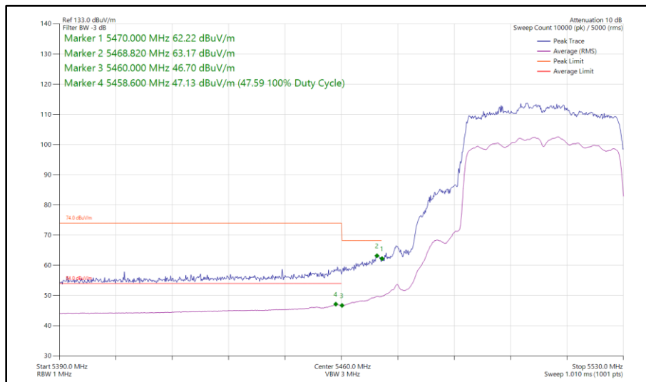
Figure 357 - 802.11ax HE40, SU, SDM, Core 0 - Core 1 - 5510 MHz Band Edge Frequency 5470 MHz
