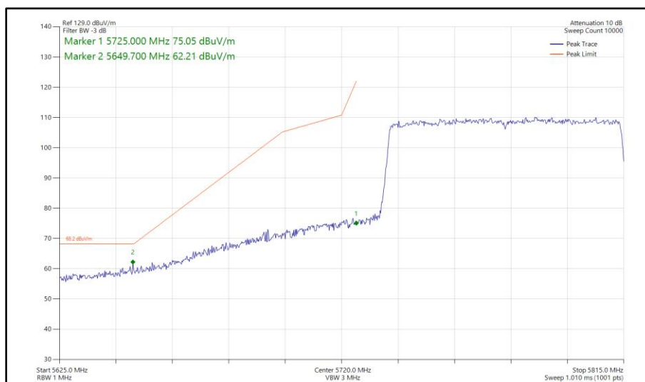
Figure 392 - 802.11ax HE80, SU, SISO, Core 1 - 5775 MHz Band Edge Frequency 5725 MHz
