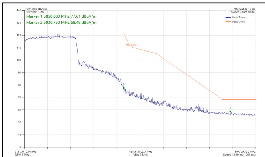
Figure 375 - 802.11ax HE40, SU, TxBF, Core 0 - Core 1 - 5795 MHz Band Edge Frequency 5850 MHz
