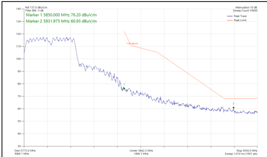
Figure 353 - 802.11n HT40, CDD, Core 0 - Core 1 - 5795 MHz Band Edge Frequency 5850 MHz
