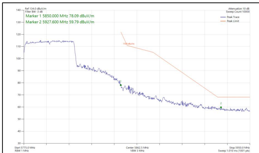
Figure 342 - 802.11ax HE40, SU, SISO, Core 1 - 5795 MHz Band Edge Frequency 5850 MHz
