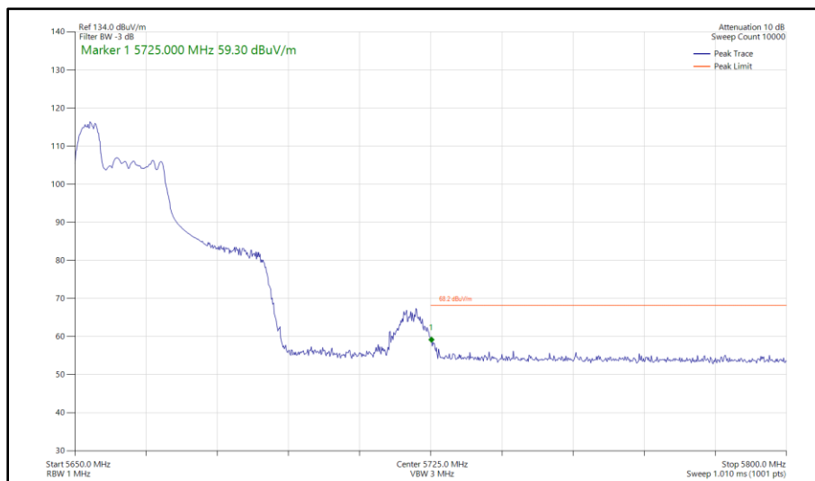
Figure 340 - 802.11ax HE40, RU 52-37, SISO, Core 1 - 5670 MHz Band Edge Frequency 5725 MHz
