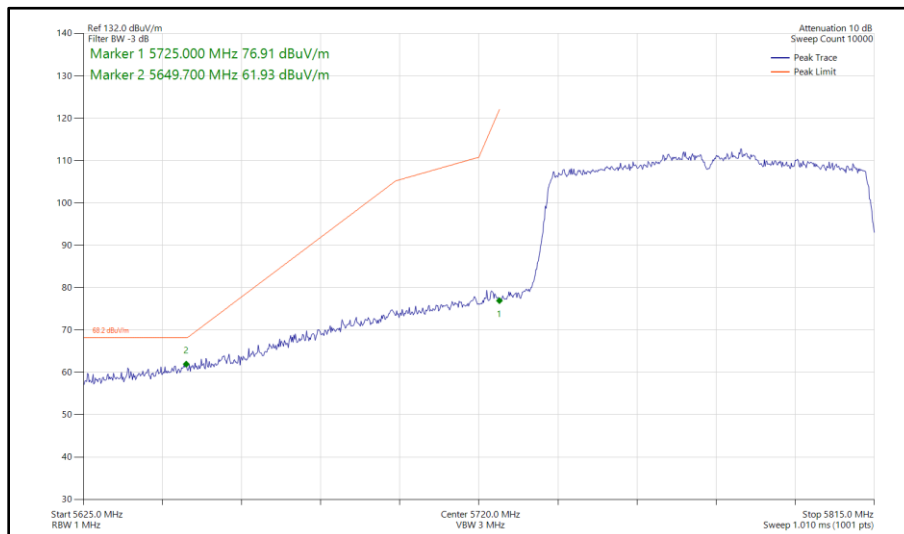
Figure 391 - 802.11ac VHT80, SISO, Core 1 - 5775 MHz Band Edge Frequency 5725 MHz
