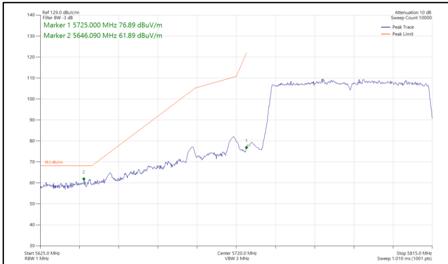
Figure 379 - 802.11ac VHT80, SISO, Core 0 - 5775 MHz Band Edge Frequency 5725 MHz
