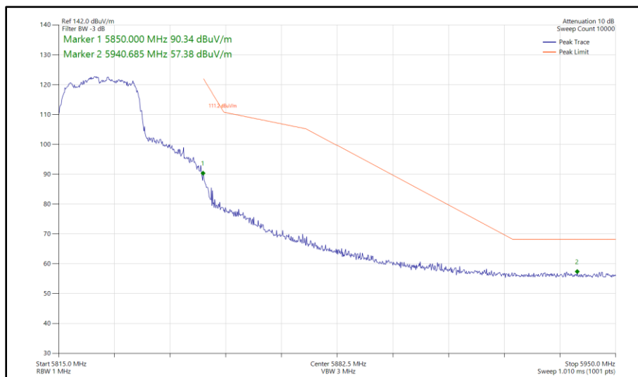
Figure 319 - 802.11ac VHT20, TxBF, Core 0 - Core 1 - 5825 MHz Band Edge Frequency 5850 MHz
