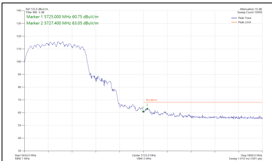
Figure 350 - 802.11n HT40, CDD, Core 0 - Core 1 - 5670 MHz Band Edge Frequency 5725 MHz
