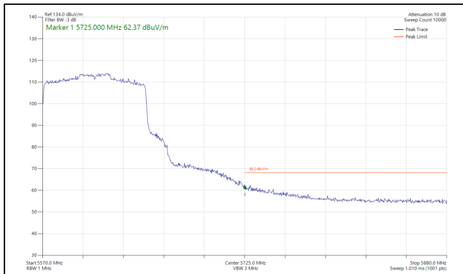
Figure 383 - 802.11ax HE80, SU, SISO, Core 0 - 5610 MHz Band Edge Frequency 5725 MHz
