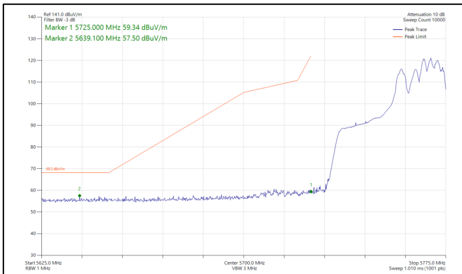
Figure 361 - 802.11ax HE40, RU 106-56, SDM, Core 0 - Core 1 - 5755 MHz Band Edge Frequency 5725 MHz
