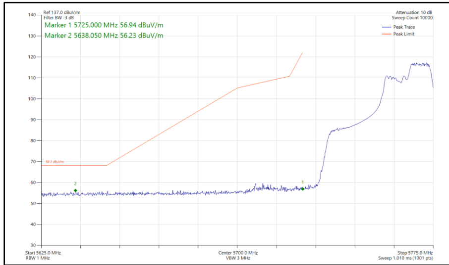
Figure 337 - 802.11ax HE40, RU 106-56, SISO, Core 1 - 5755 MHz Band Edge Frequency 5725 MHz
