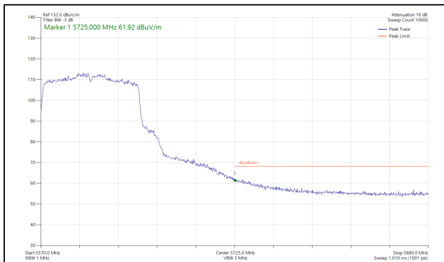
Figure 382 - 802.11ac VHT80, SISO, Core 0 - 5610 MHz Band Edge Frequency 5725 MHz
