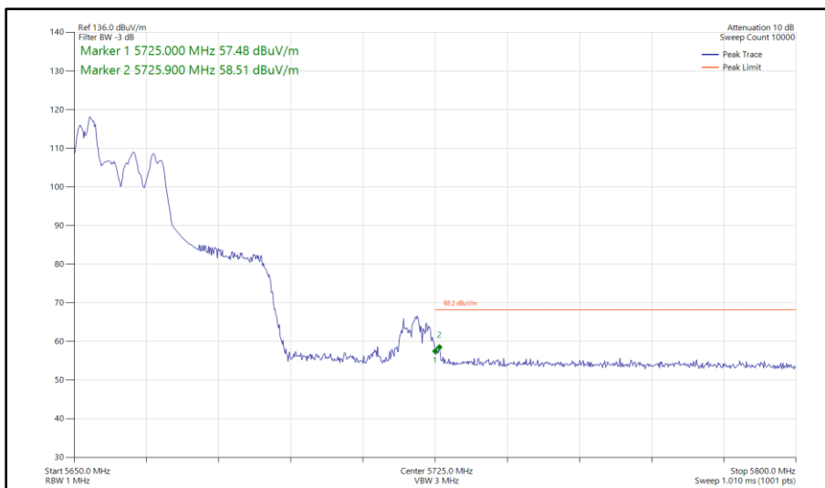
Figure 352 - 802.11ax HE40, RU 52-37, CDD, Core 0 - Core 1 - 5670 MHz Band Edge Frequency 5725 MHz
