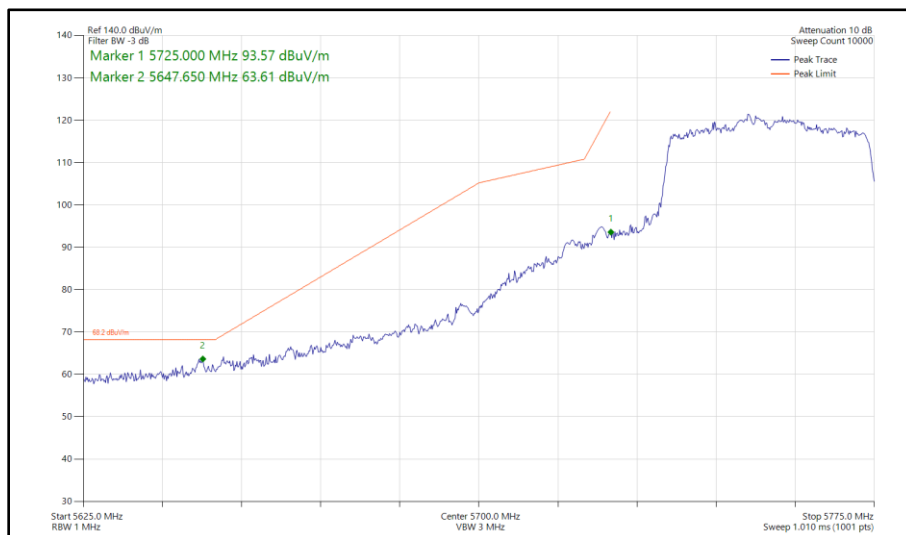
Figure 360 - 802.11ax HE40, SU, SDM, Core 0 - Core 1 - 5755 MHz Band Edge Frequency 5725 MHz
