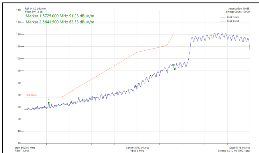
Figure 348 - 802.11ax HE40, SU, CDD, Core 0 - Core 1 - 5755 MHz Band Edge Frequency 5725 MHz
