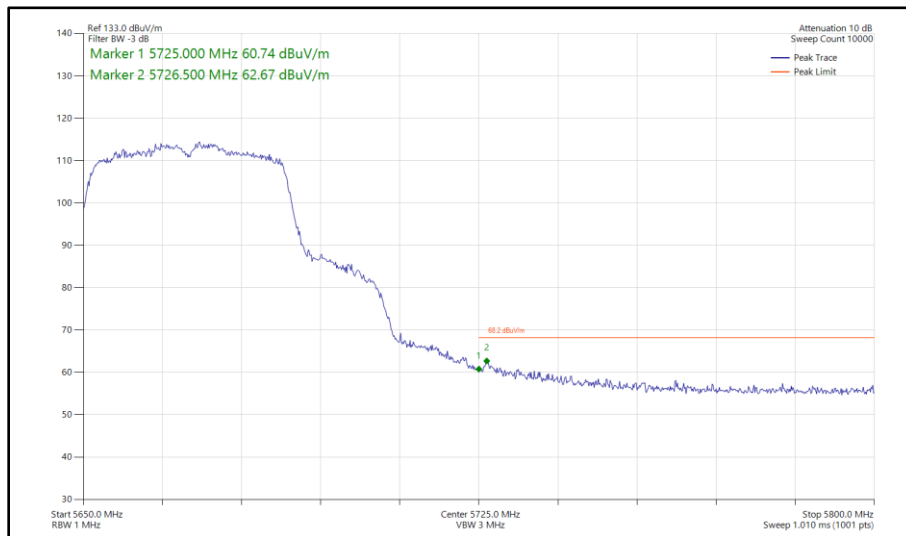
Figure 338 - 802.11n HT40, SISO, Core 1 - 5670 MHz Band Edge Frequency 5725 MHz
