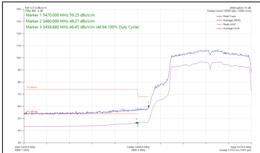
Figure 388 - 802.11ac VHT80, SISO, Core 1 - 5530 MHz Band Edge Frequency 5470 MHz
