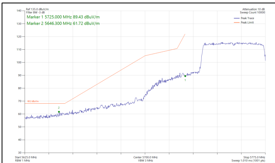
Figure 324 - 802.11ax HE40, SU, SISO, Core 0 - 5755 MHz Band Edge Frequency 5725 MHz
