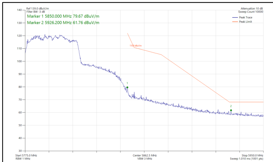
Figure 374 - 802.11ac VHT40, TxBF, Core 0 - Core 1 - 5795 MHz Band Edge Frequency 5850 MHz
