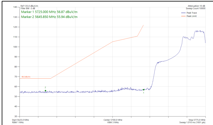
Figure 325 - 802.11ax HE40, RU 106-56, SISO, Core 0 - 5755 MHz Band Edge Frequency 5725 MHz
