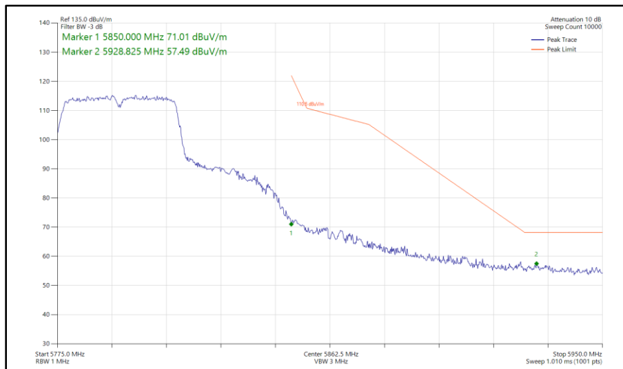
Figure 329 - 802.11n HT40, SISO, Core 0 - 5795 MHz Band Edge Frequency 5850 MHz
