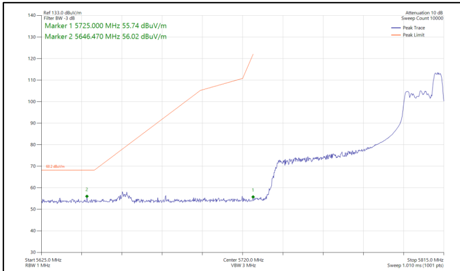
Figure 393 - 802.11ax HE80, RU 52-52, SISO, Core 1 - 5775 MHz Band Edge Frequency 5725 MHz
