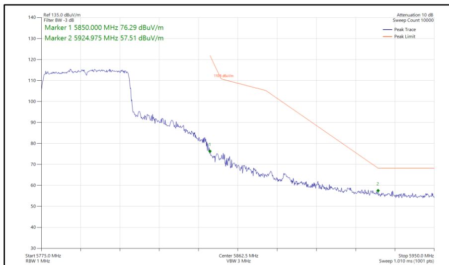
Figure 330 - 802.11ax HE40, SU, SISO, Core 0 - 5795 MHz Band Edge Frequency 5850 MHz
