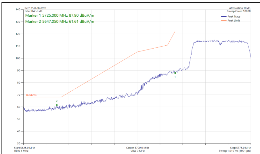
Figure 323 - 802.11n HT40, SISO, Core 0 - 5755 MHz Band Edge Frequency 5725 MHz
