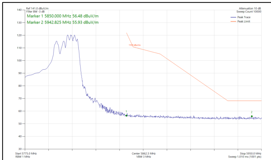
Figure 355 - 802.11ax HE40, RU 106-56, CDD, Core 0 - Core 1 - 5795 MHz Band Edge Frequency 5850 MHz
