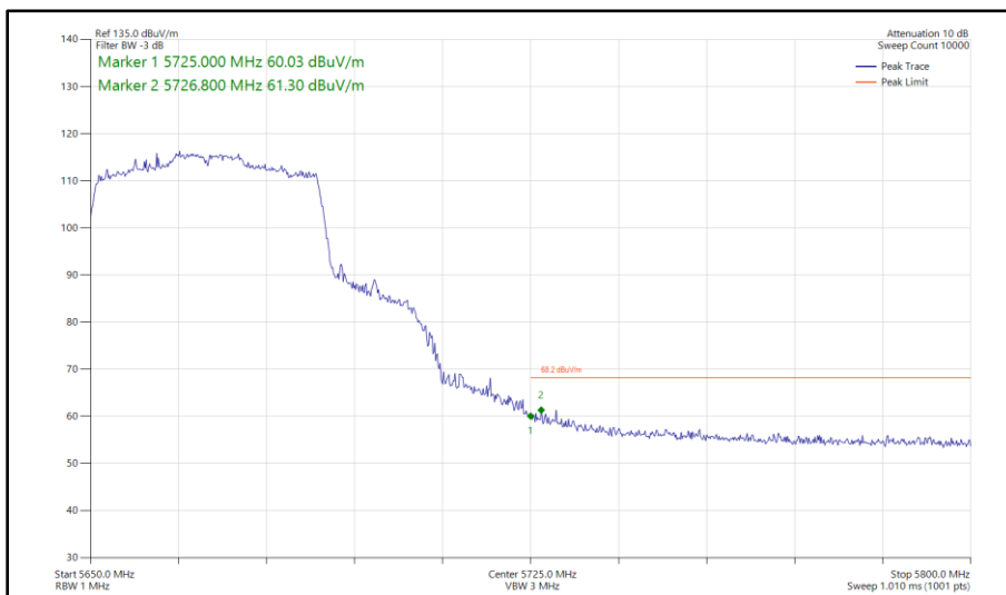
Figure 373 - 802.11ax HE40, SU, TxBF, Core 0 - Core 1 - 5670 MHz Band Edge Frequency 5725 MHz
