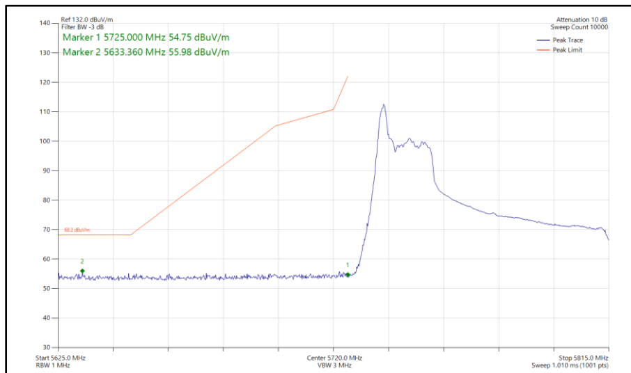
Figure 381 - 802.11ax HE80, RU 26-0, SISO, Core 0 - 5775 MHz Band Edge Frequency 5725 MHz
