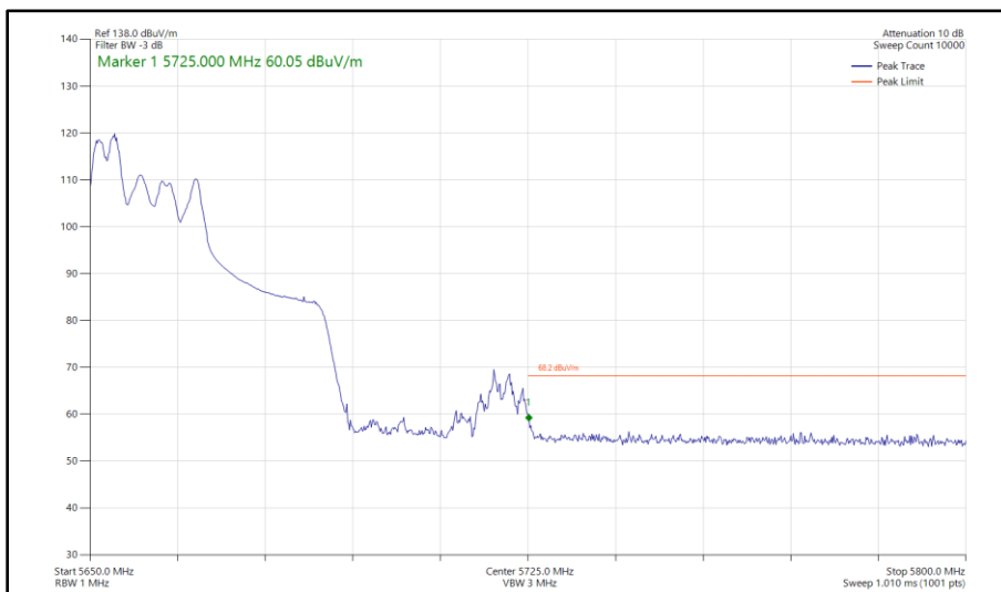
Figure 364 - 802.11ax HE40, RU 52-37, SDM, Core 0 - Core 1 - 5670 MHz Band Edge Frequency 5725 MHz
