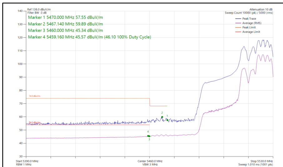
Figure 358 - 802.11ax HE40, RU 106-56, SDM, Core 0 - Core 1 - 5510 MHz Band Edge Frequency 5470 MHz
