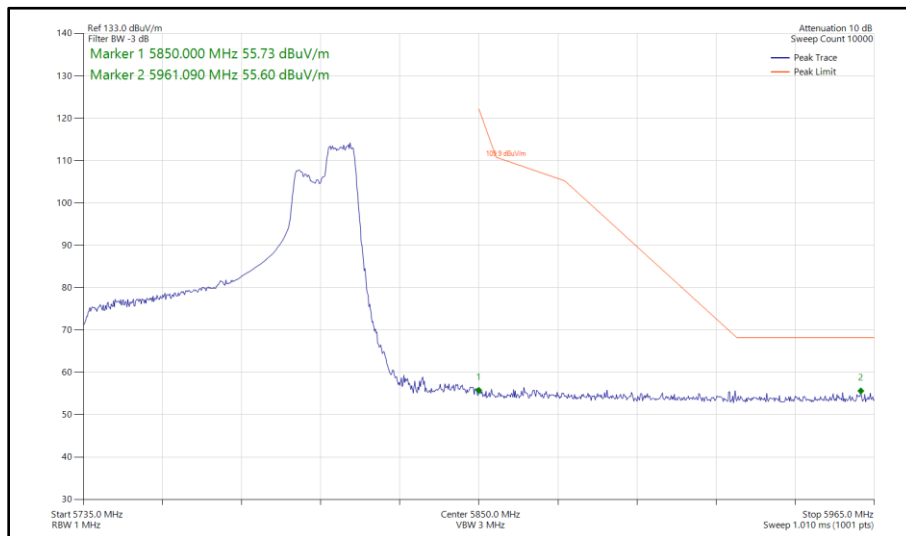
Figure 387 - 802.11ax HE80, RU 106-60, SISO, Core 0 - 5775 MHz Band Edge Frequency 5850 MHz
