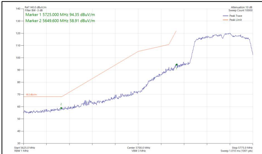
Figure 370 - 802.11ac VHT40, TxBF, Core 0 - Core 1 - 5755 MHz Band Edge Frequency 5725 MHz
