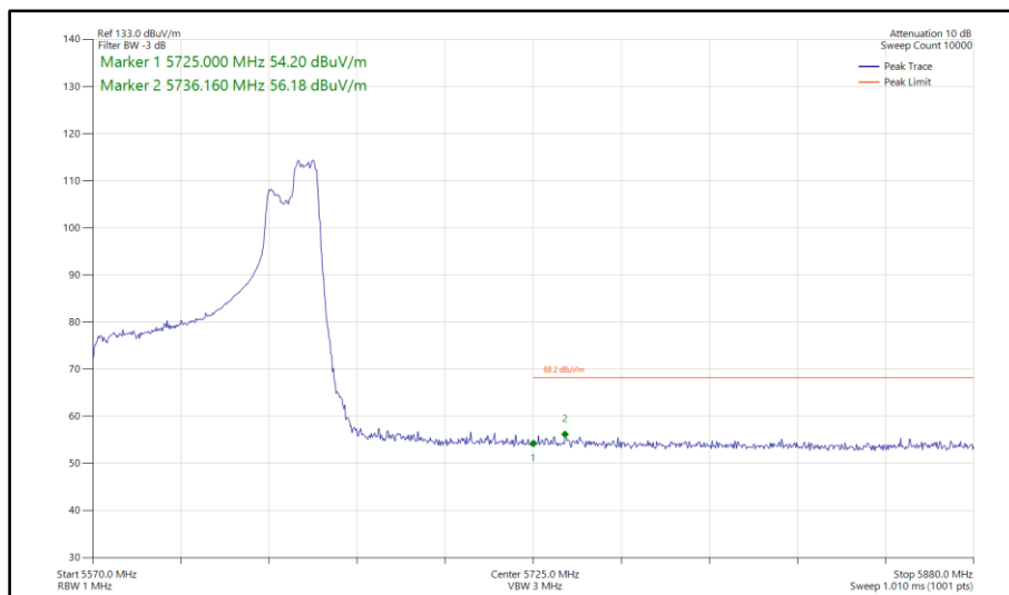
Figure 384 - 802.11ax HE80, RU 106-60, SISO, Core 0 - 5610 MHz Band Edge Frequency 5725 MHz
