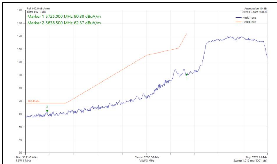
Figure 359 - 802.11n HT40, SDM, Core 0 - Core 1 - 5755 MHz Band Edge Frequency 5725 MHz
