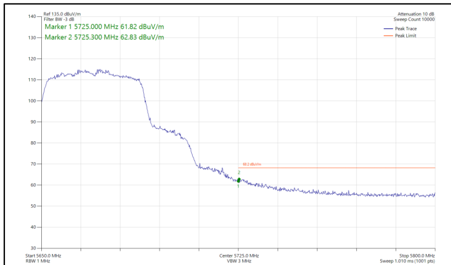
Figure 326 - 802.11n HT40, SISO, Core 0 - 5670 MHz Band Edge Frequency 5725 MHz
