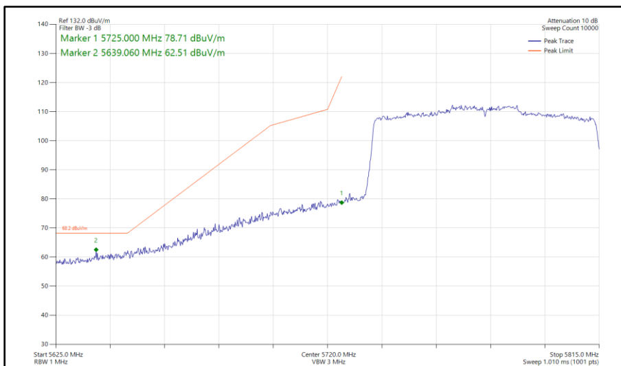
Figure 380 - 802.11ax HE80, SU, SISO, Core 0 - 5775 MHz Band Edge Frequency 5725 MHz
