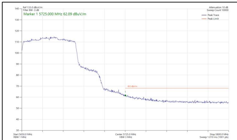
Figure 339 - 802.11ax HE40, SU, SISO, Core 1 - 5670 MHz Band Edge Frequency 5725 MHz
