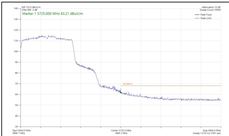
Figure 327 - 802.11ax HE40, SU, SISO, Core 0 - 5670 MHz Band Edge Frequency 5725 MHz
