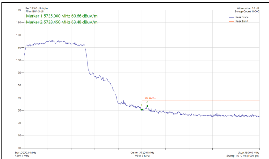
Figure 363 - 802.11ax HE40, SU, SDM, Core 0 - Core 1 - 5670 MHz Band Edge Frequency 5725 MHz
