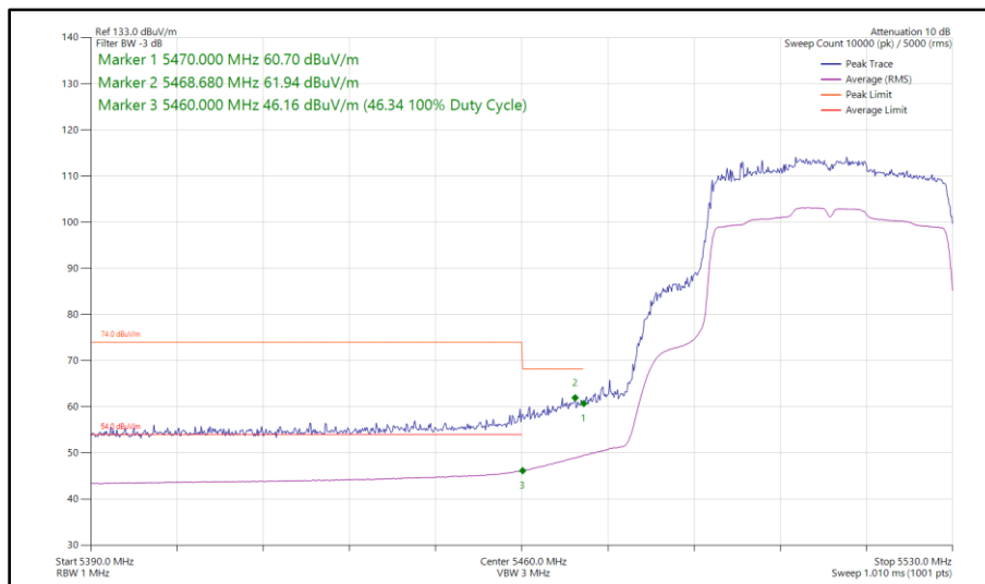
Figure 369 - 802.11ax HE40, SU, TxBF, Core 0 - Core 1 - 5510 MHz Band Edge Frequency 5470 MHz
