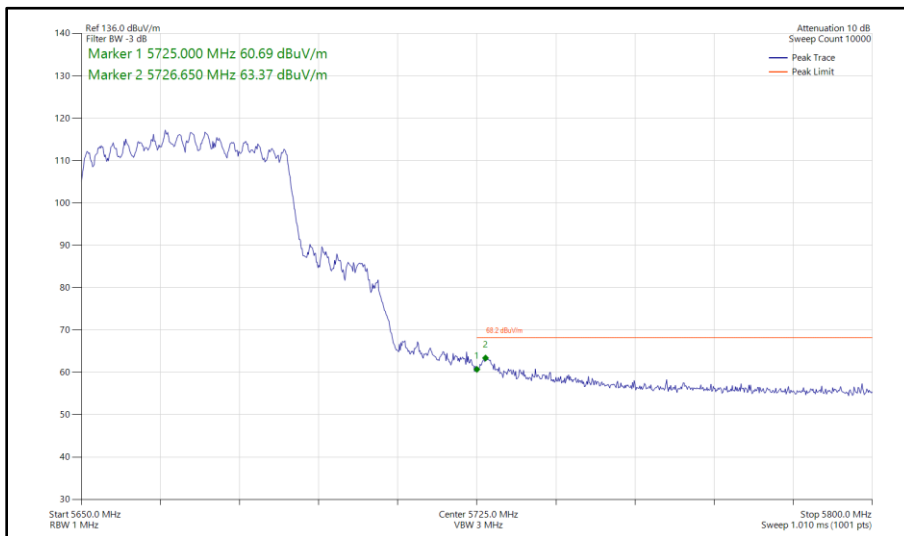
Figure 351 - 802.11ax HE40, SU, CDD, Core 0 - Core 1 - 5670 MHz Band Edge Frequency 5725 MHz
