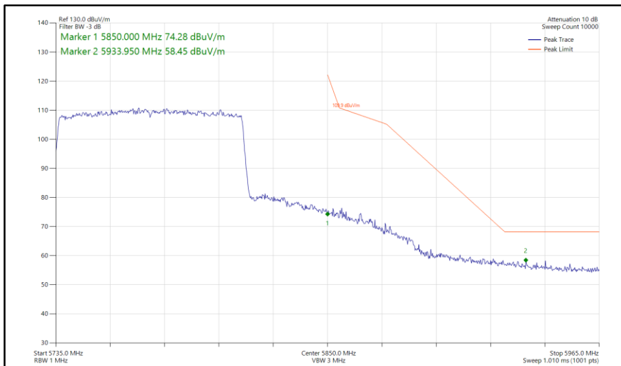
Figure 386 - 802.11ax HE80, SU, SISO, Core 0 - 5775 MHz Band Edge Frequency 5850 MHz
