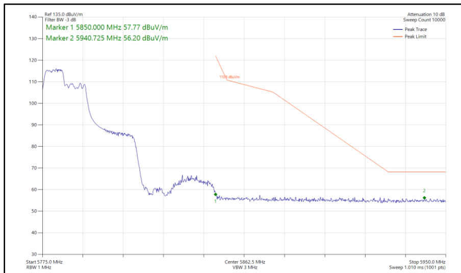
Figure 343 - 802.11ax HE40, RU 106-53, SISO, Core 1 - 5795 MHz Band Edge Frequency 5850 MHz
