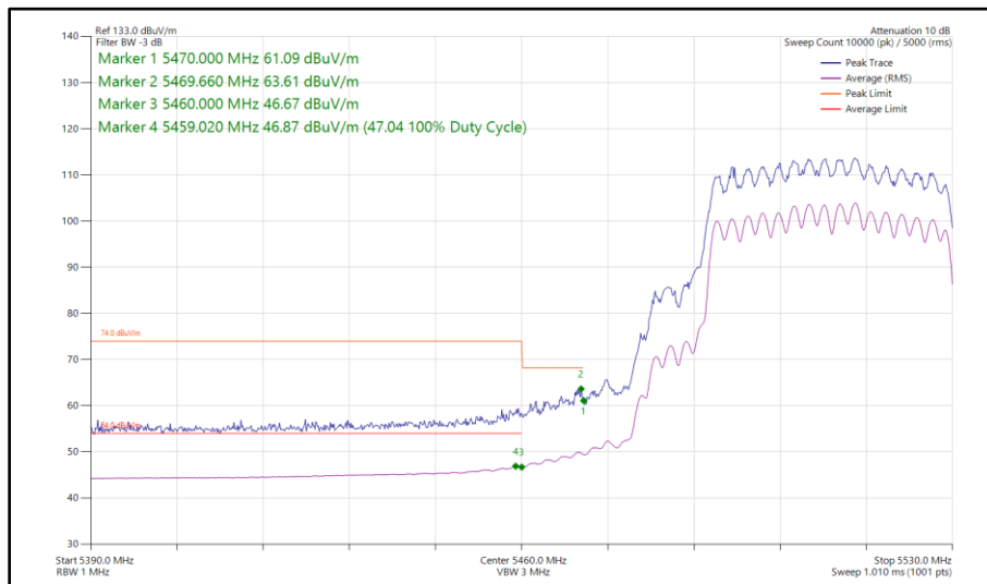
Figure 345 - 802.11ax HE40, SU, CDD, Core 0 - Core 1 - 5510 MHz Band Edge Frequency 5470 MHz
