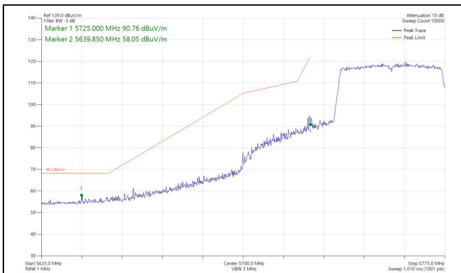
Figure 371 - 802.11ax HE40, SU, TxBF, Core 0 - Core 1 - 5755 MHz Band Edge Frequency 5725 MHz
