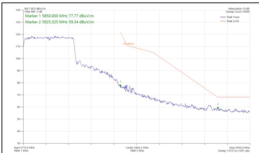
Figure 366 - 802.11ax HE40, SU, SDM, Core 0 - Core 1 - 5795 MHz Band Edge Frequency 5850 MHz
