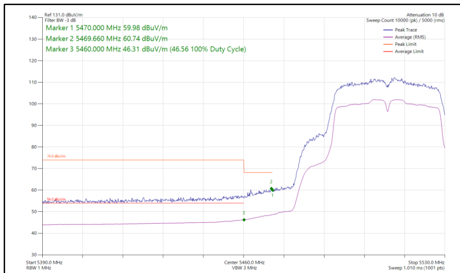
Figure 320 - 802.11n HT40, SISO, Core 0 - 5510 MHz Band Edge Frequency 5470 MHz
