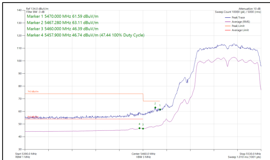
Figure 356 - 802.11n HT40, SDM, Core 0 - Core 1 - 5510 MHz Band Edge Frequency 5470 MHz
