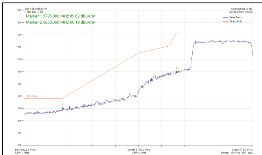
Figure 336 - 802.11ax HE40, SU, SISO, Core 1 - 5755 MHz Band Edge Frequency 5725 MHz
