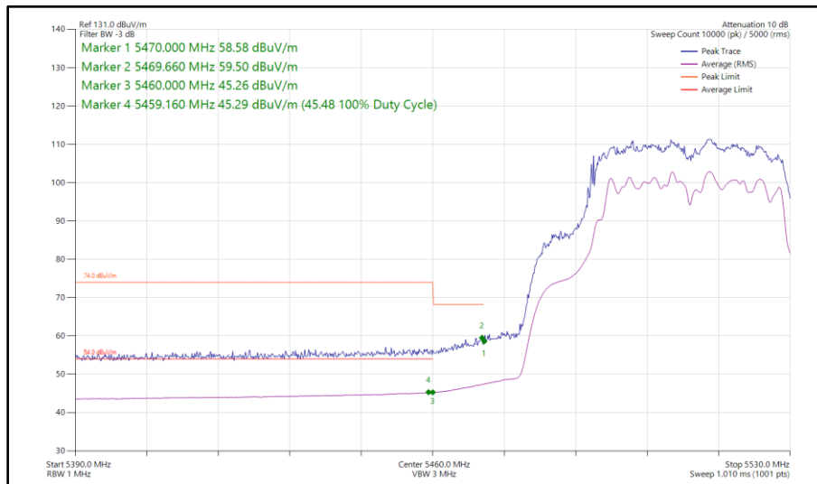
Figure 368 - 802.11ac VHT40, TxBF, Core 0 - Core 1 - 5510 MHz Band Edge Frequency 5470 MHz
