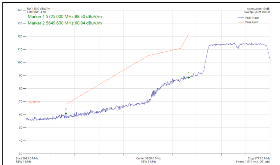
Figure 335 - 802.11n HT40, SISO, Core 1 - 5755 MHz Band Edge Frequency 5725 MHz
