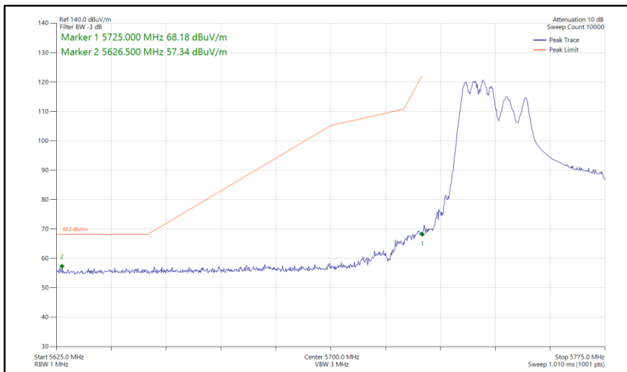
Figure 349 - 802.11ax HE40, RU 106-53, CDD, Core 0 - Core 1 - 5755 MHz Band Edge Frequency 5725 MHz
