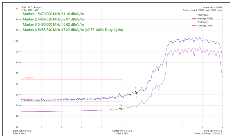
Figure 344 - 802.11n HT40, CDD, Core 0 - Core 1 - 5510 MHz Band Edge Frequency 5470 MHz
