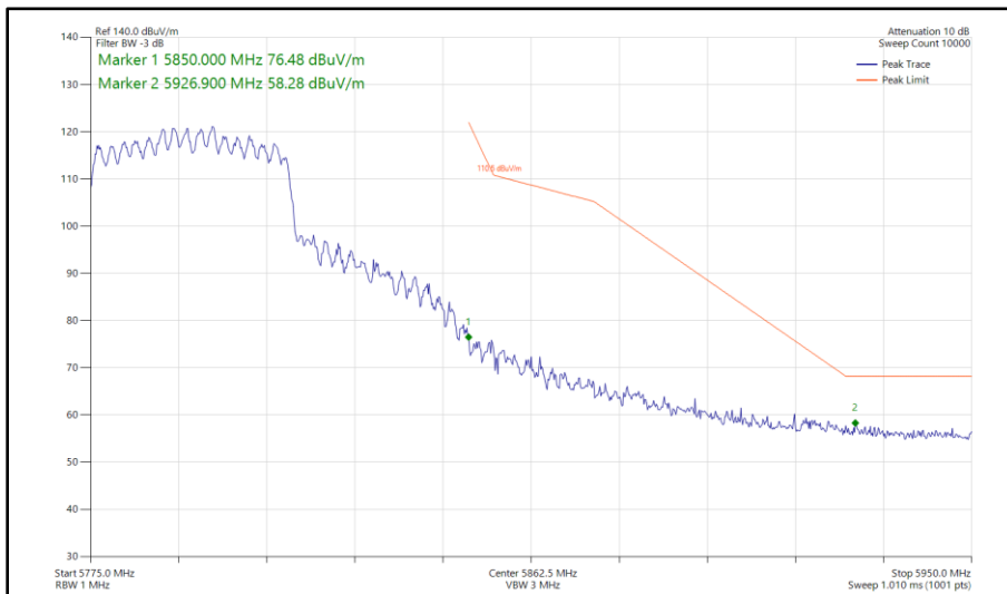
Figure 354 - 802.11ax HE40, SU, CDD, Core 0 - Core 1 - 5795 MHz Band Edge Frequency 5850 MHz
