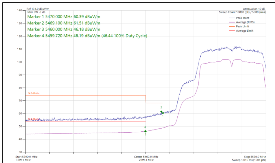
Figure 332 - 802.11n HT40, SISO, Core 1 - 5510 MHz Band Edge Frequency 5470 MHz
