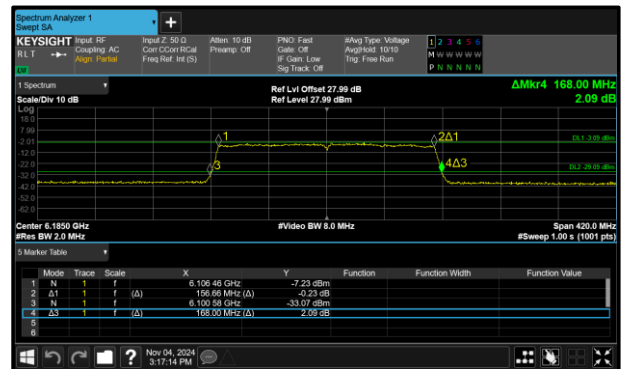
Figure 82 - 802.11ax HE160 SU VLP Maximum 26 dB EBW
