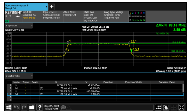
Figure 126 - 802.11ax HE80 SU VLP Maximum 26 dB EBW
