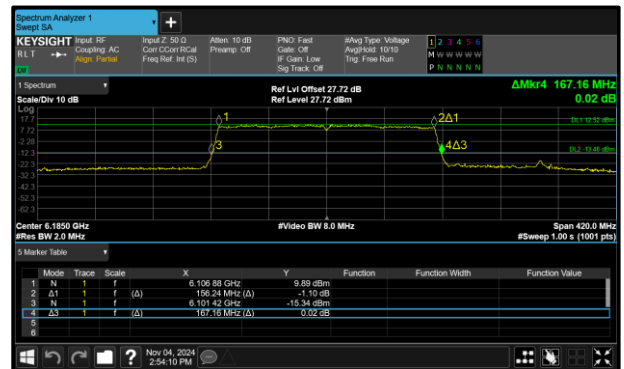
Figure 120 - 802.11ax HE160 SU SP Maximum 26 dB EBW
