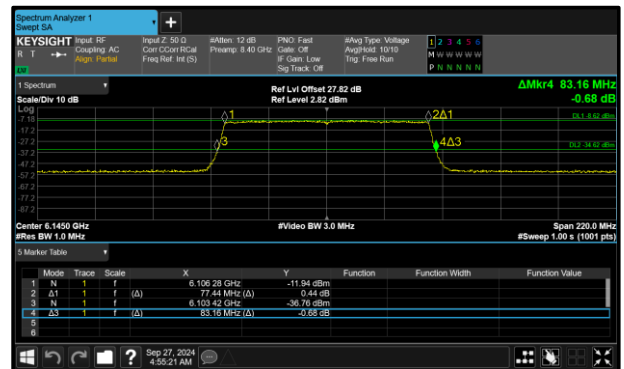
Figure 80 - 802.11ax HE80 SU VLP Maximum 26 dB EBW
