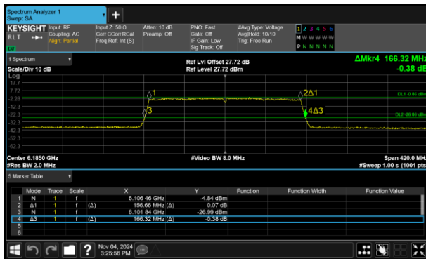
Figure 127 - 802.11ax HE160 SU VLP Minimum 26 dB EBW
