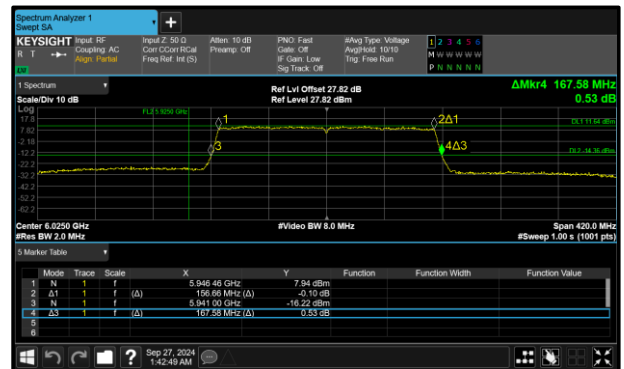
Figure 98 - 802.11ax HE160 SU SP Maximum 99% OBW
