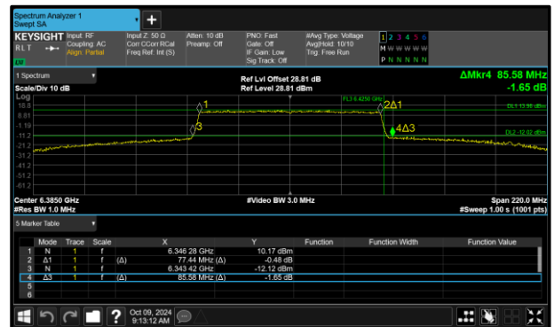
Figure 118 - 802.11ax HE80 SU SP Maximum 26 dB EBW
