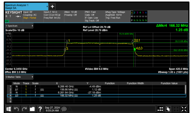
Figure 152 - 802.11ax HE160 SU VLP Maximum 99% OBW
