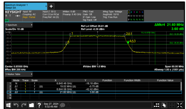
Figure 122 - 802.11ax HE20 SU VLP Maximum 26 dB EBW
