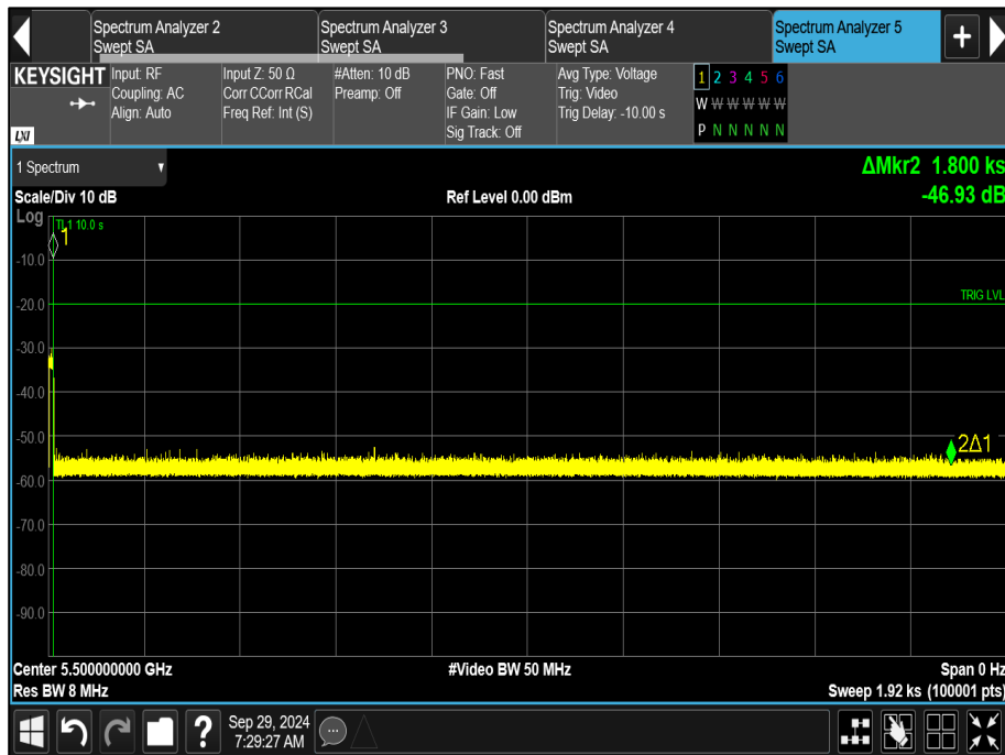
Figure 518 - 30 minute Non-Occupancy Period
