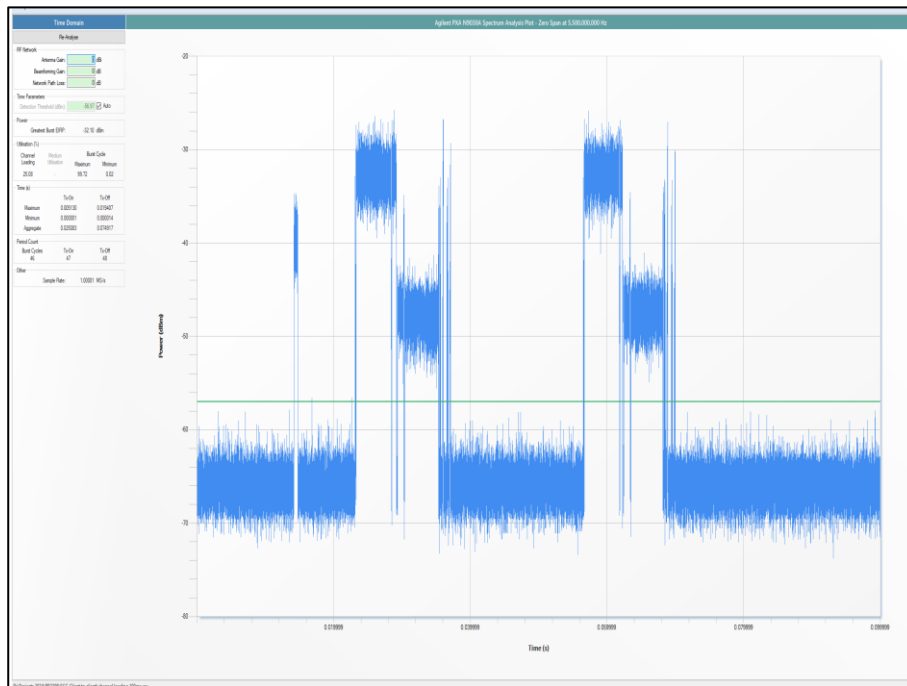
Figure 521 - Channel Loading
