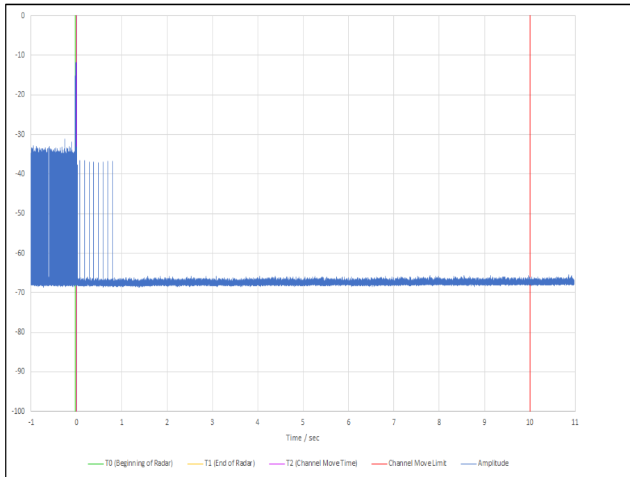
Figure 517 - First 12 s of Channel Shutdown Period
