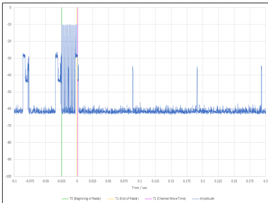
Figure 522 - First 200 ms of Channel Shutdown Period
