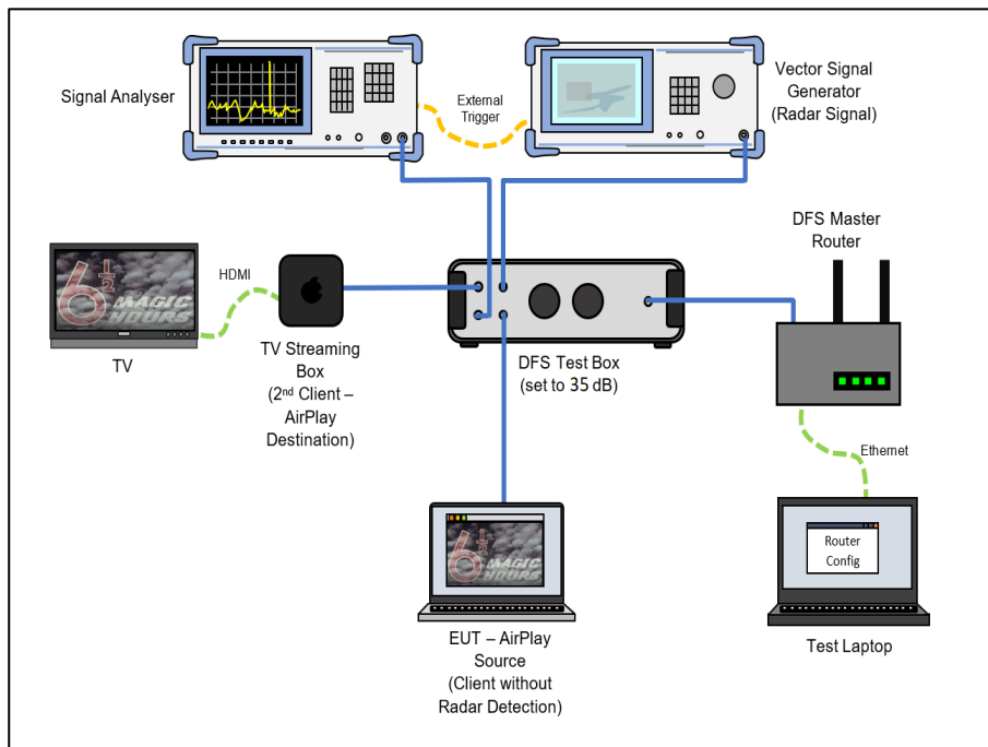
Figure 519 - Test Equipment Setup Diagram for Client without Radar Detection with Injection at the Master
