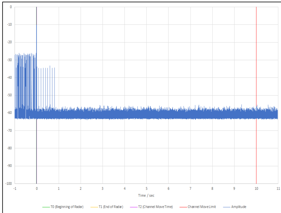
Figure 523 - First 12 s of Channel Shutdown Period
