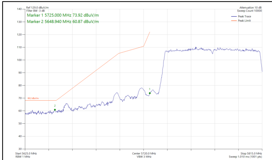
Figure 387 - 802.11ac VHT80, SISO, Core 1 - 5775 MHz Band Edge Frequency 5725 MHz
