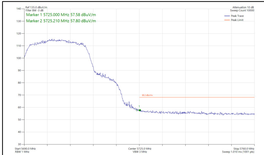
Figure 318 - 802.11ac VHT20, TxBF, Core 0 - Core 1 - 5700 MHz Band Edge Frequency 5725 MHz
