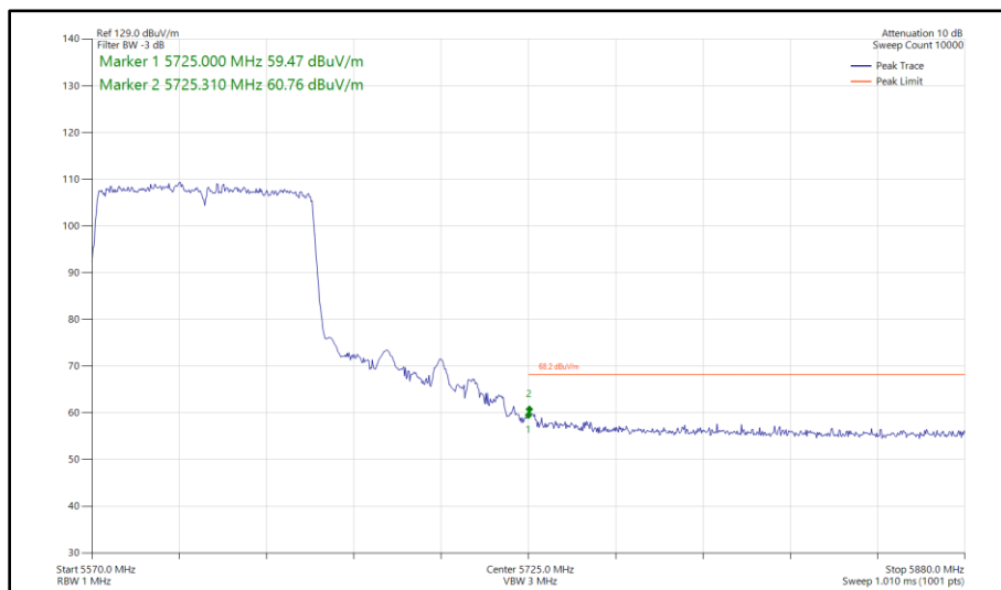
Figure 378 - 802.11ac VHT80, SISO, Core 0 - 5610 MHz Band Edge Frequency 5725 MHz
