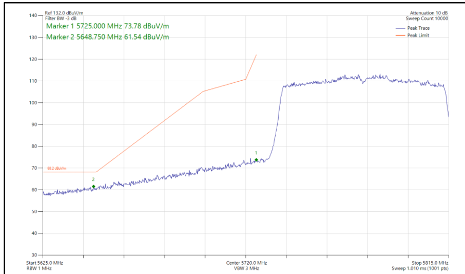
Figure 375 - 802.11ac VHT80, SISO, Core 0 - 5775 MHz Band Edge Frequency 5725 MHz
