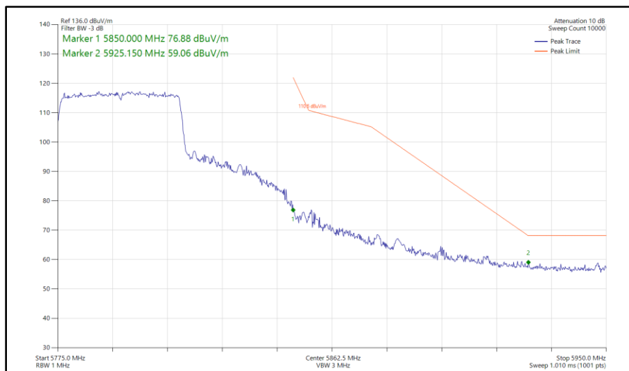
Figure 330 - 802.11ax HE40, SU, SISO, Core 0 - 5795 MHz Band Edge Frequency 5850 MHz
