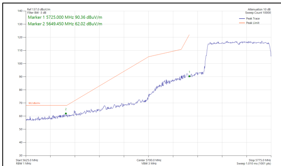
Figure 324 - 802.11ax HE40, SU, SISO, Core 0 - 5755 MHz Band Edge Frequency 5725 MHz
