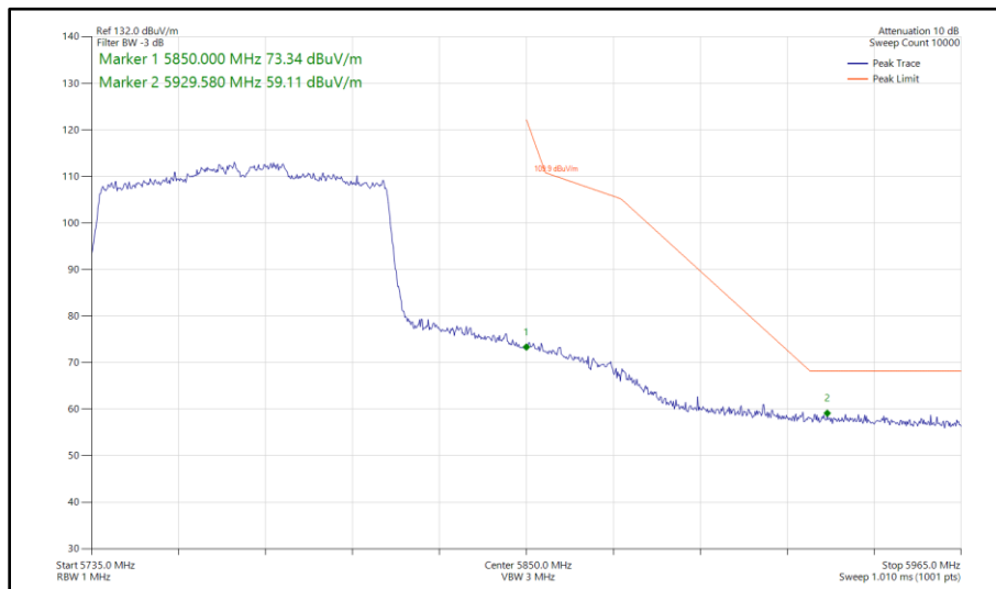
Figure 381 - 802.11ac VHT80, SISO, Core 0 - 5775 MHz Band Edge Frequency 5850 MHz
