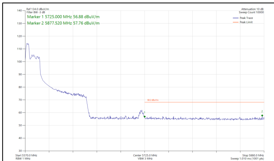
Figure 380 - 802.11ax HE80, RU 52-37, SISO, Core 0 - 5610 MHz Band Edge Frequency 5725 MHz
