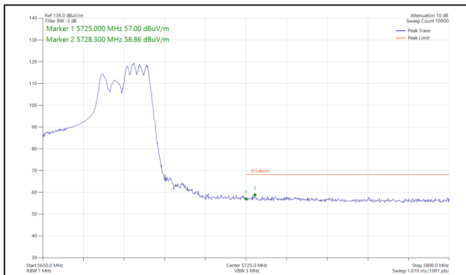
Figure 352 - 802.11ax HE40, RU 106-56, CDD, Core 0 - Core 1 - 5670 MHz Band Edge Frequency 5725 MHz
