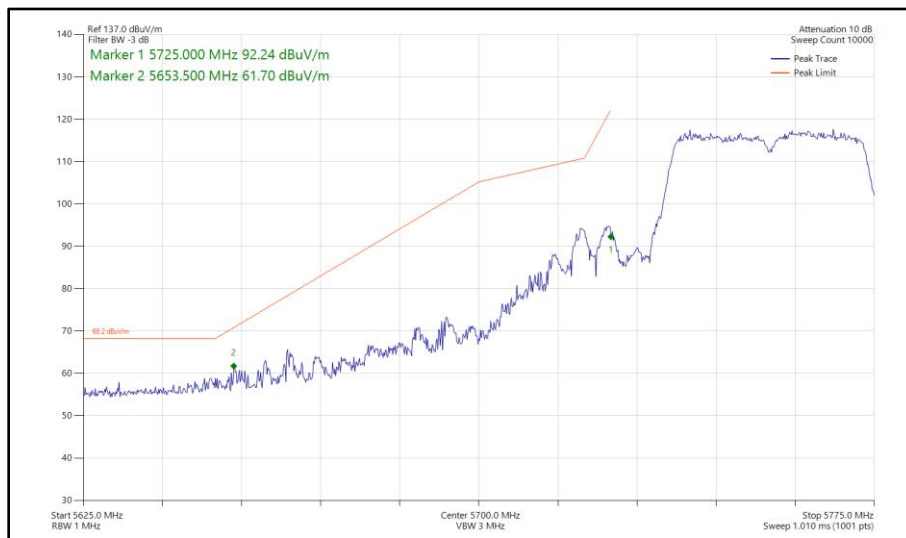
Figure 369 - 802.11ac VHT40, TxBF, Core 0 - Core 1 - 5755 MHz Band Edge Frequency 5725 MHz
