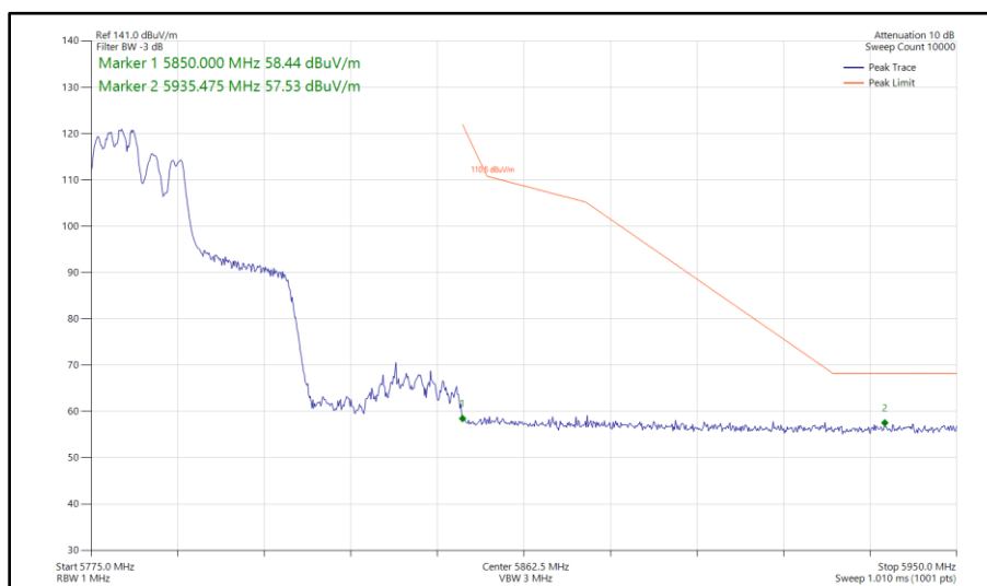
Figure 355 - 802.11ax HE40, RU 106-53, CDD, Core 0 - Core 1 - 5795 MHz Band Edge Frequency 5850 MHz
