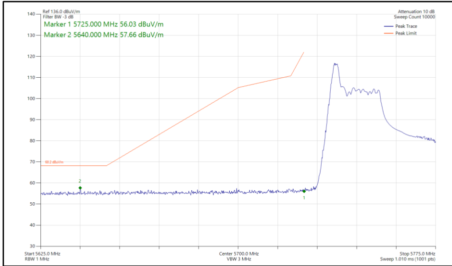
Figure 325 - 802.11ax HE40, RU 26-0, SISO, Core 0 - 5755 MHz Band Edge Frequency 5725 MHz
