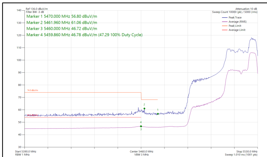
Figure 334 - 802.11ax HE40, RU 52-44, SISO, Core 1 - 5510 MHz Band Edge Frequency 5470 MHz
