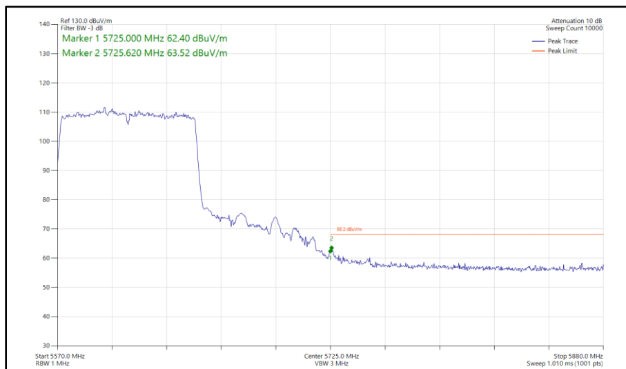
Figure 390 - 802.11ac VHT80, SISO, Core 1 - 5610 MHz Band Edge Frequency 5725 MHz
