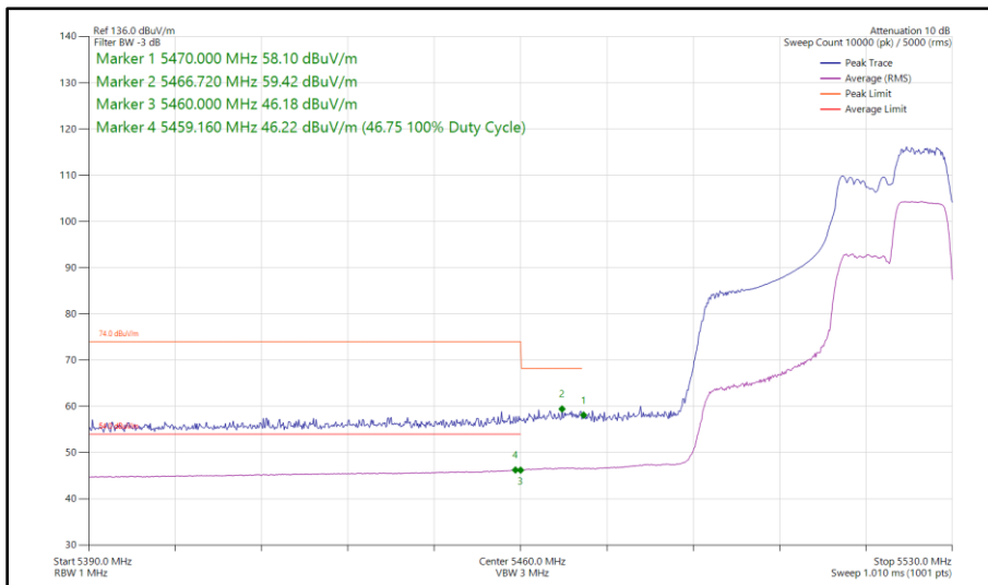
Figure 322 - 802.11ax HE40, RU 106-56, SISO, Core 0 - 5510 MHz Band Edge Frequency 5470 MHz
