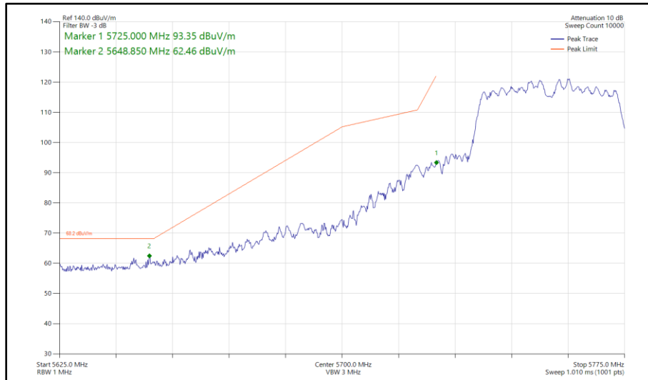
Figure 347 - 802.11n HT40, CDD, Core 0 - Core 1 - 5755 MHz Band Edge Frequency 5725 MHz
