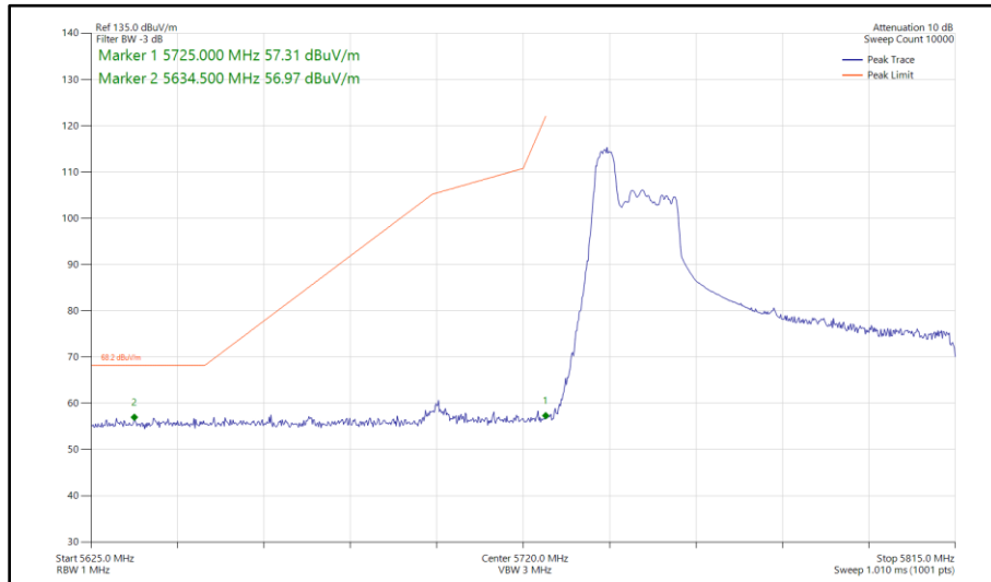
Figure 389 - 802.11ax HE80, RU 52-37, SISO, Core 1 - 5775 MHz Band Edge Frequency 5725 MHz
