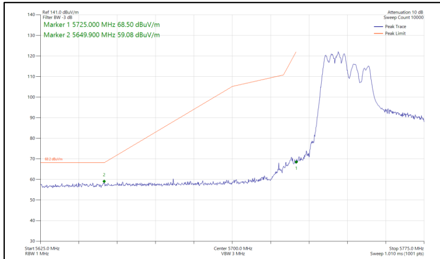
Figure 361 - 802.11ax HE40, RU 106-53, SDM, Core 0 - Core 1 - 5755 MHz Band Edge Frequency 5725 MHz
