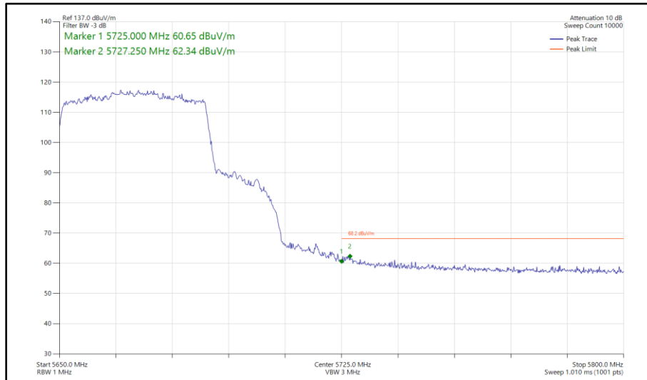
Figure 363 - 802.11ax HE40, SU, SDM, Core 0 - Core 1 - 5670 MHz Band Edge Frequency 5725 MHz
