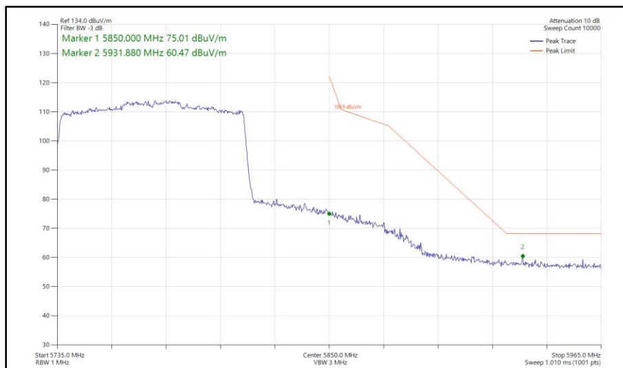
Figure 382 - 802.11ax HE80, SU, SISO, Core 0 - 5775 MHz Band Edge Frequency 5850 MHz
