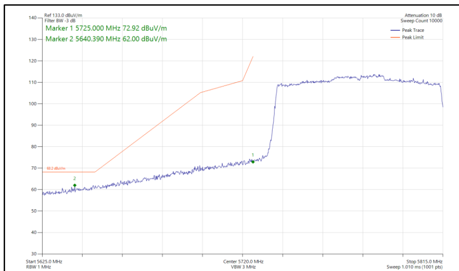
Figure 376 - 802.11ax HE80, SU, SISO, Core 0 - 5775 MHz Band Edge Frequency 5725 MHz
