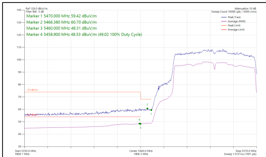
Figure 372 - 802.11ac VHT80, SISO, Core 0 - 5530 MHz Band Edge Frequency 5470 MHz
