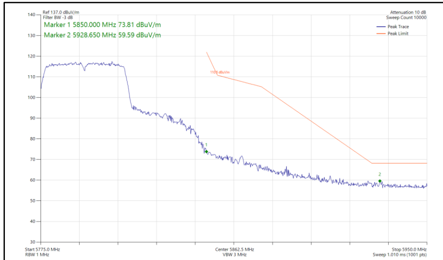
Figure 329 - 802.11n HT40, SISO, Core 0 - 5795 MHz Band Edge Frequency 5850 MHz
