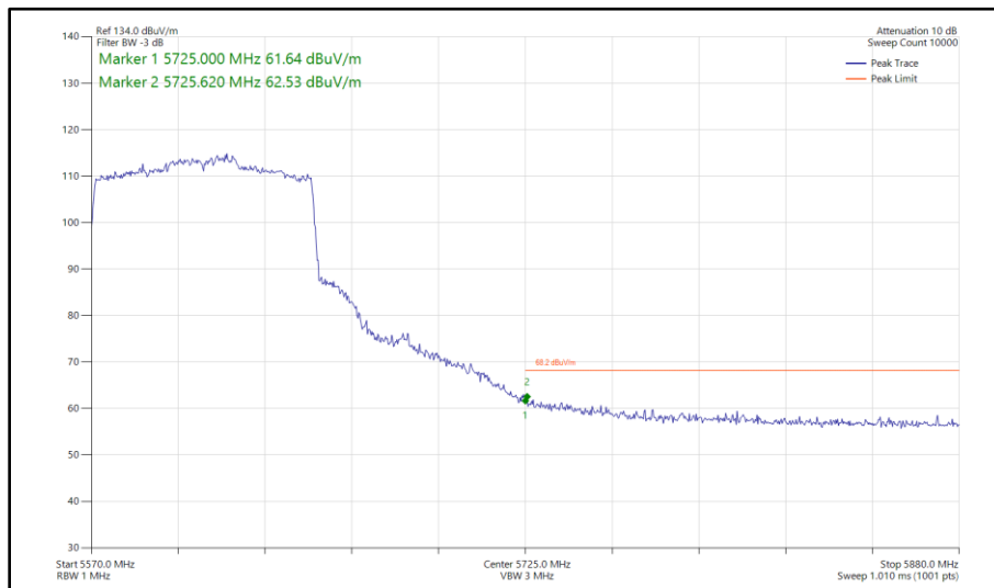
Figure 391 - 802.11ax HE80, SU, SISO, Core 1 - 5610 MHz Band Edge Frequency 5725 MHz
