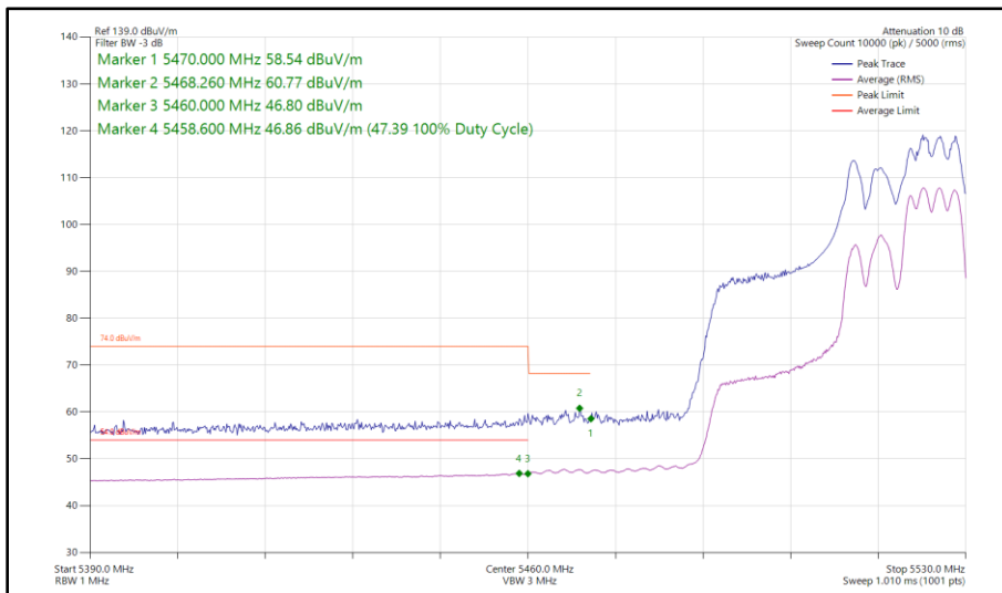
Figure 346 - 802.11ax HE40, RU 106-56, CDD, Core 0 - Core 1 - 5510 MHz Band Edge Frequency 5470 MHz
