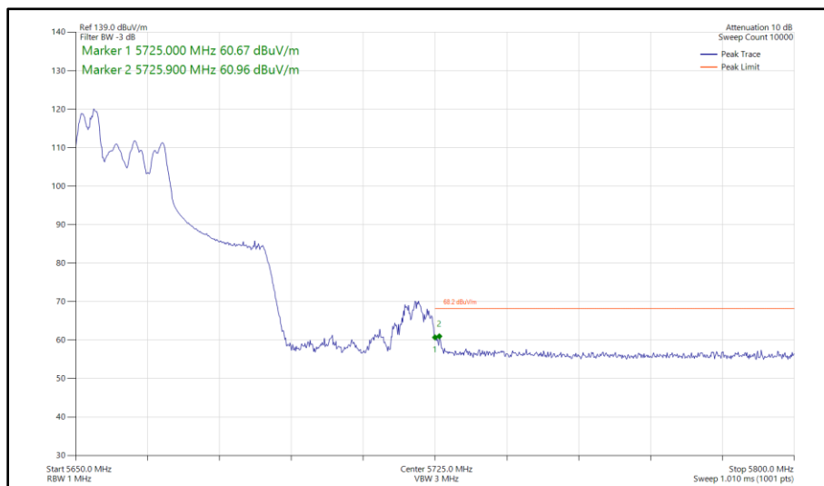
Figure 364 - 802.11ax HE40, RU 52-37, SDM, Core 0 - Core 1 - 5670 MHz Band Edge Frequency 5725 MHz
