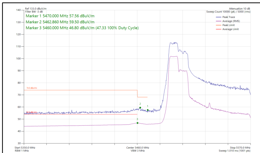
Figure 374 - 802.11ax HE80, RU 106-53, SISO, Core 0 - 5530 MHz Band Edge Frequency 5470 MHz
