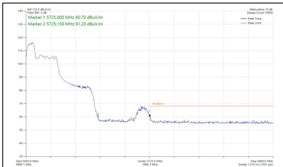
Figure 328 - 802.11ax HE40, RU 52-37, SISO, Core 0 - 5670 MHz Band Edge Frequency 5725 MHz
