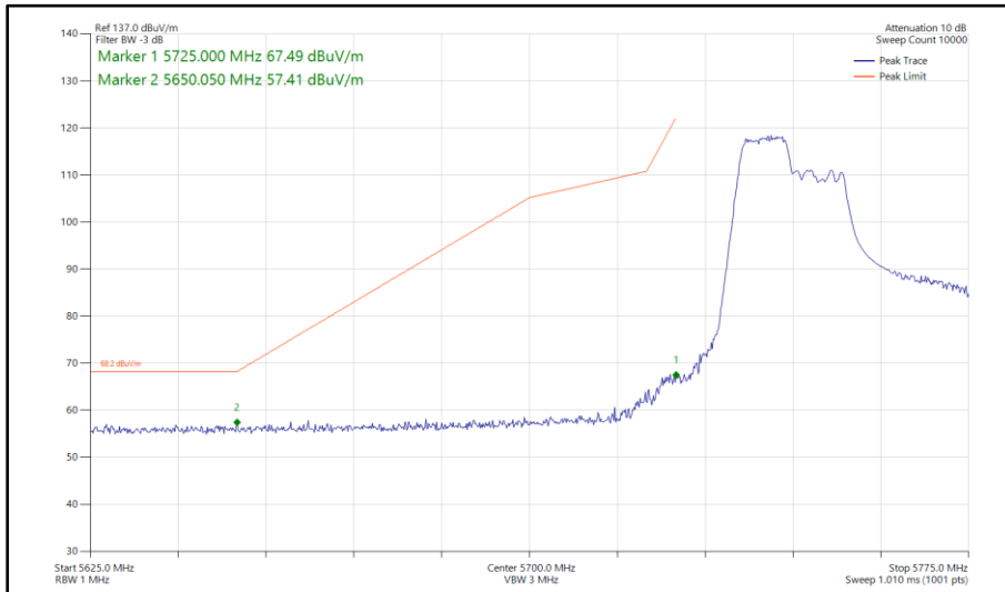
Figure 337 - 802.11ax HE40, RU 106-53, SISO, Core 1 - 5755 MHz Band Edge Frequency 5725 MHz
