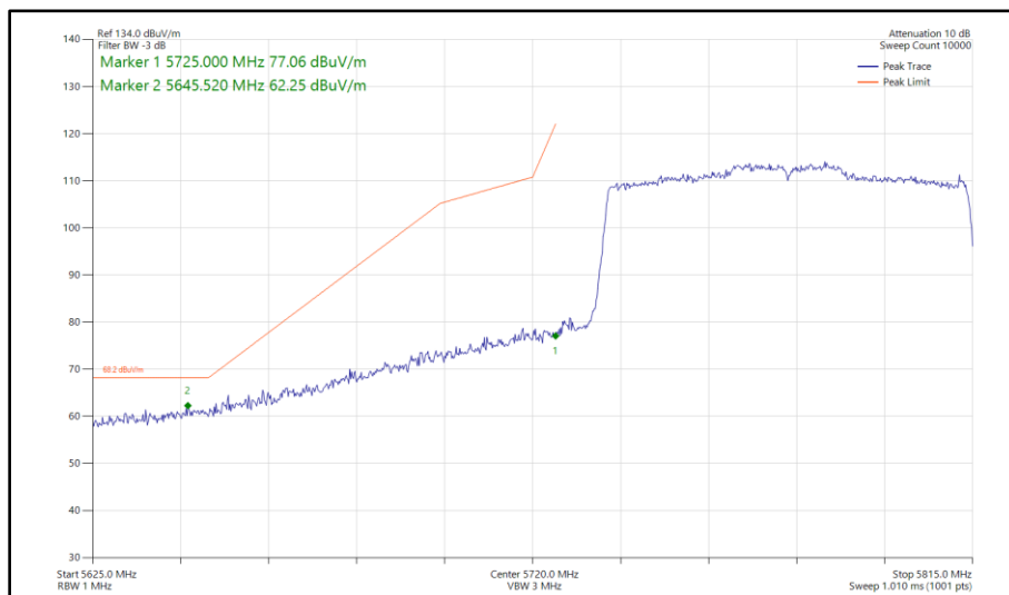
Figure 388 - 802.11ax HE80, SU, SISO, Core 1 - 5775 MHz Band Edge Frequency 5725 MHz
