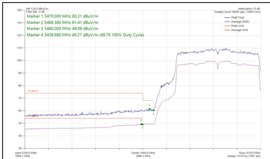
Figure 384 - 802.11ac VHT80, SISO, Core 1 - 5530 MHz Band Edge Frequency 5470 MHz
