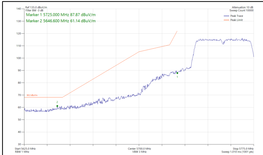
Figure 323 - 802.11n HT40, SISO, Core 0 - 5755 MHz Band Edge Frequency 5725 MHz
