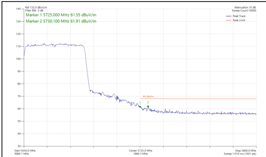
Figure 339 - 802.11ax HE40, SU, SISO, Core 1 - 5670 MHz Band Edge Frequency 5725 MHz
