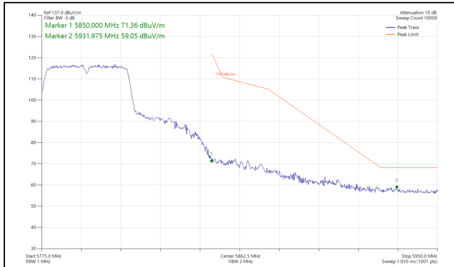
Figure 341 - 802.11n HT40, SISO, Core 1 - 5795 MHz Band Edge Frequency 5850 MHz
