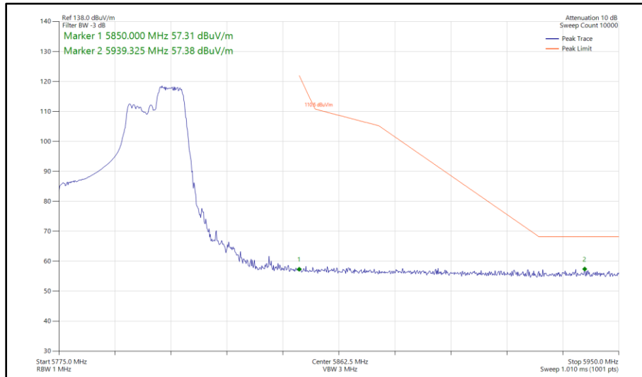
Figure 331 - 802.11ax HE40, RU 106-56, SISO, Core 0 - 5795 MHz Band Edge Frequency 5850 MHz
