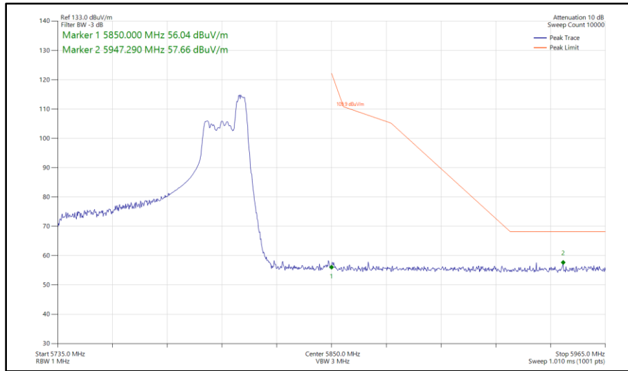
Figure 383 - 802.11ax HE80, RU 52-52, SISO, Core 0 - 5775 MHz Band Edge Frequency 5850 MHz
