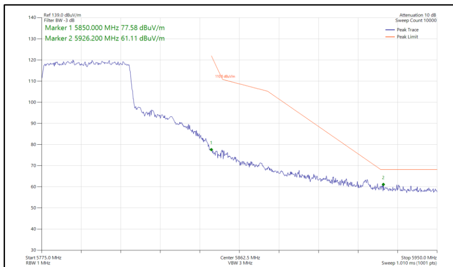
Figure 366 - 802.11ax HE40, SU, SDM, Core 0 - Core 1 - 5795 MHz Band Edge Frequency 5850 MHz
