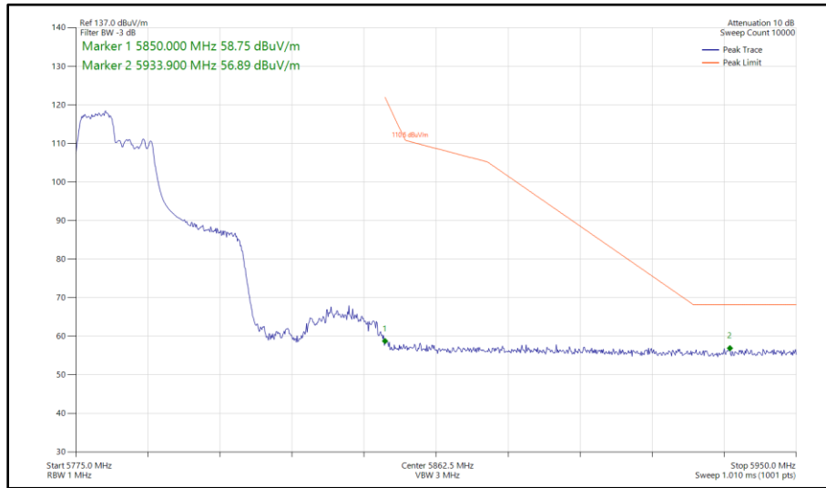
Figure 343 - 802.11ax HE40, RU 106-53, SISO, Core 1 - 5795 MHz Band Edge Frequency 5850 MHz
