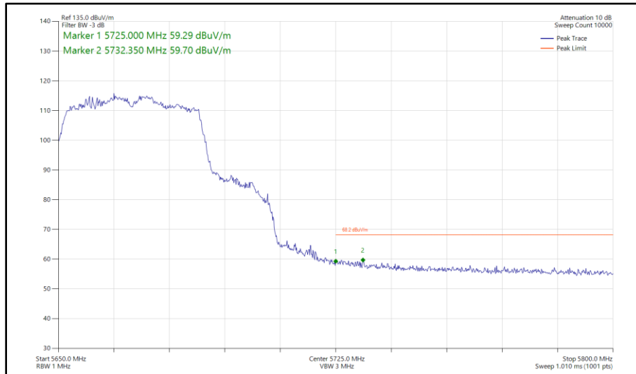
Figure 370 - 802.11ac VHT40, TxBF, Core 0 - Core 1 - 5670 MHz Band Edge Frequency 5725 MHz
