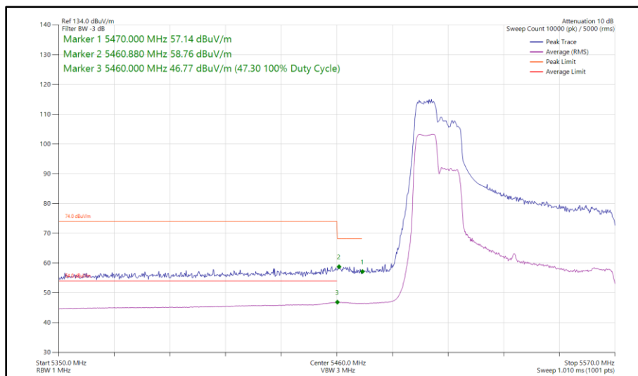
Figure 386 - 802.11ax HE80, RU 106-53, SISO, Core 1 - 5530 MHz Band Edge Frequency 5470 MHz
