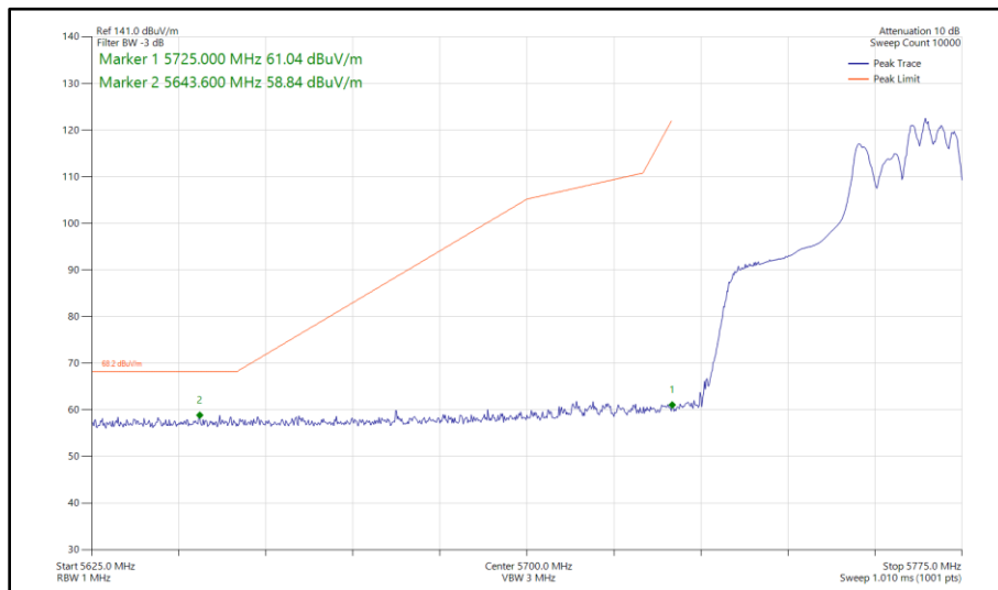
Figure 349 - 802.11ax HE40, RU 106-56, CDD, Core 0 - Core 1 - 5755 MHz Band Edge Frequency 5725 MHz
