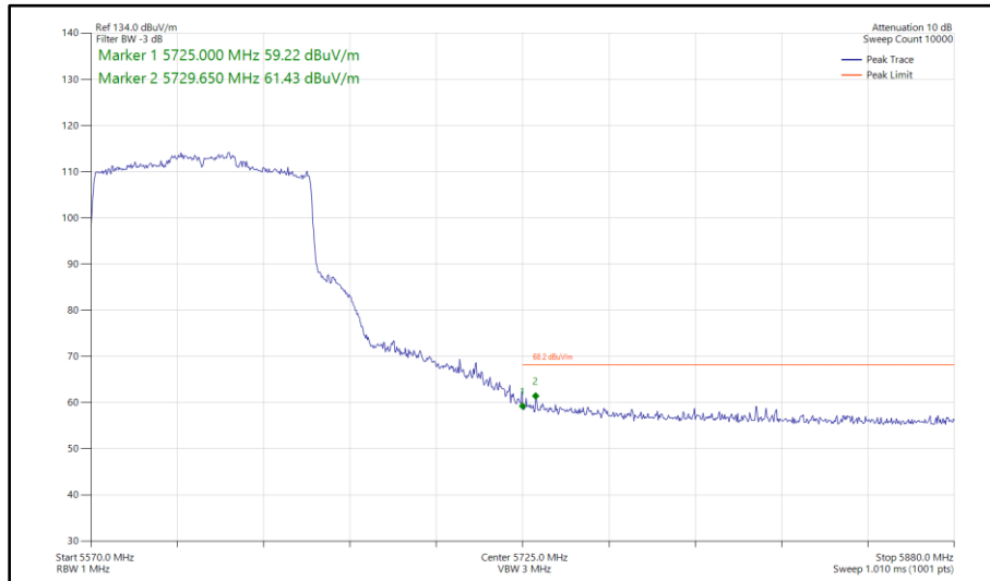
Figure 379 - 802.11ax HE80, SU, SISO, Core 0 - 5610 MHz Band Edge Frequency 5725 MHz
