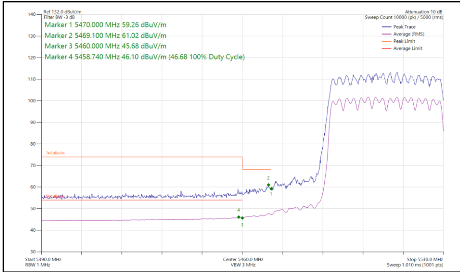
Figure 345 - 802.11ax HE40, SU, CDD, Core 0 - Core 1 - 5510 MHz Band Edge Frequency 5470 MHz
