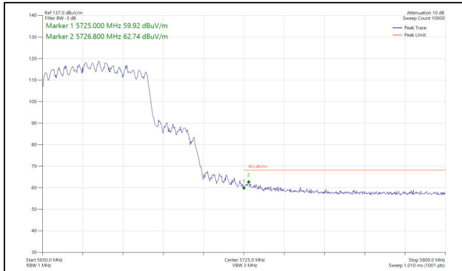
Figure 351 - 802.11ax HE40, SU, CDD, Core 0 - Core 1 - 5670 MHz Band Edge Frequency 5725 MHz
