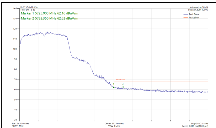
Figure 338 - 802.11n HT40, SISO, Core 1 - 5670 MHz Band Edge Frequency 5725 MHz
