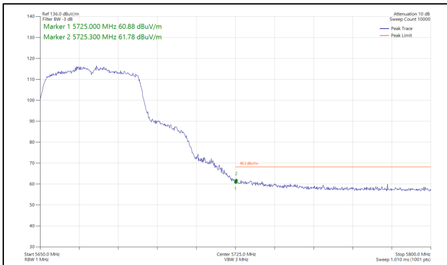
Figure 326 - 802.11n HT40, SISO, Core 0 - 5670 MHz Band Edge Frequency 5725 MHz
