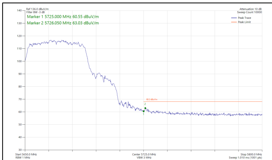
Figure 350 - 802.11n HT40, CDD, Core 0 - Core 1 - 5670 MHz Band Edge Frequency 5725 MHz
