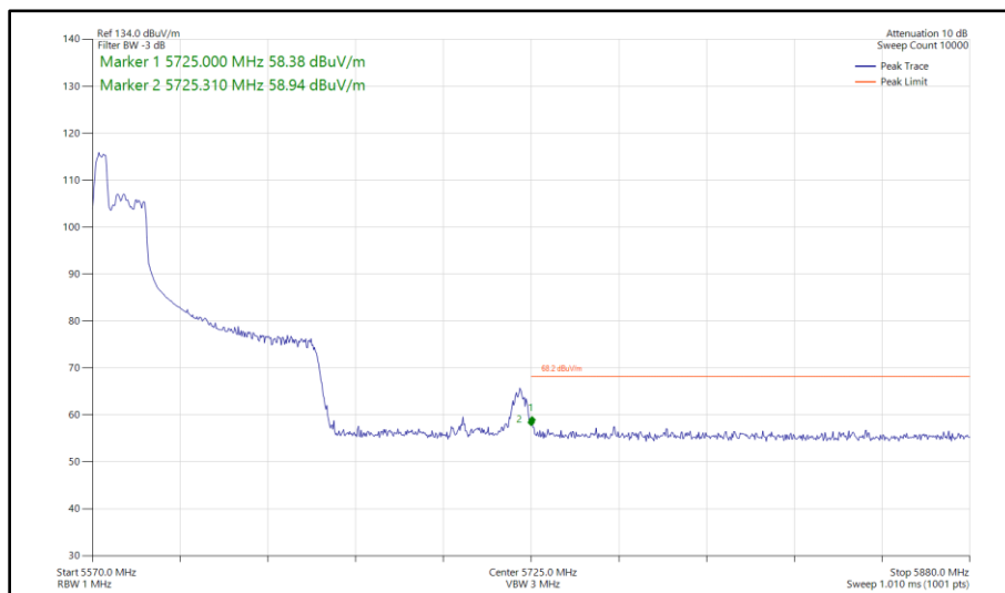
Figure 392 - 802.11ax HE80, RU 52-37, SISO, Core 1 - 5610 MHz Band Edge Frequency 5725 MHz
