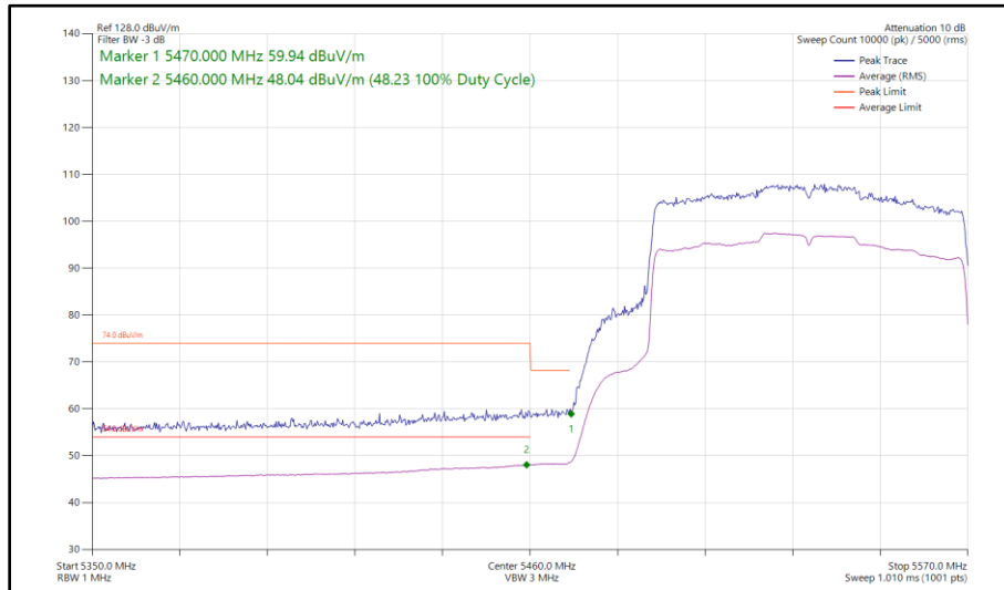
Figure 373 - 802.11ax HE80, SU, SISO, Core 0 - 5530 MHz Band Edge Frequency 5470 MHz
