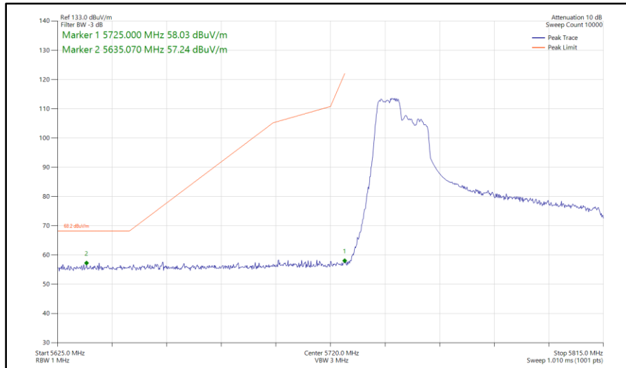
Figure 377 - 802.11ax HE80, RU 106-53, SISO, Core 0 - 5775 MHz Band Edge Frequency 5725 MHz
