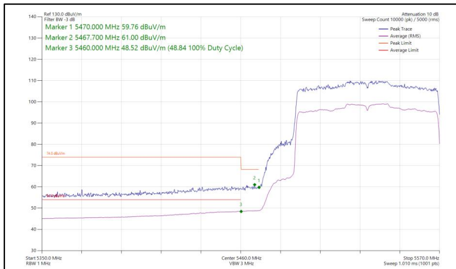
Figure 385 - 802.11ax HE80, SU, SISO, Core 1 - 5530 MHz Band Edge Frequency 5470 MHz
