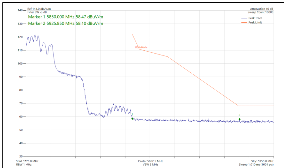
Figure 367 - 802.11ax HE40, RU 106-53, SDM, Core 0 - Core 1 - 5795 MHz Band Edge Frequency 5850 MHz
