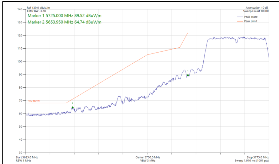
Figure 359 - 802.11n HT40, SDM, Core 0 - Core 1 - 5755 MHz Band Edge Frequency 5725 MHz
