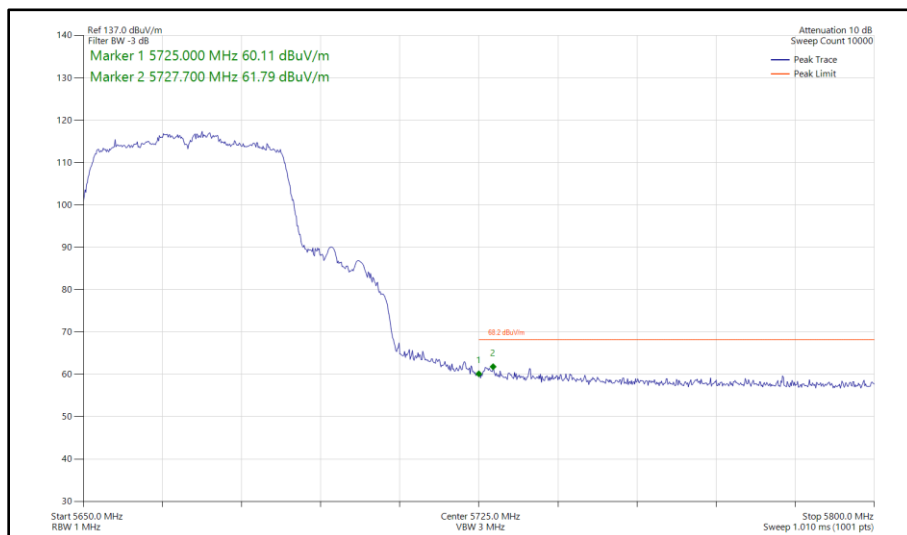
Figure 362 - 802.11n HT40, SDM, Core 0 - Core 1 - 5670 MHz Band Edge Frequency 5725 MHz
