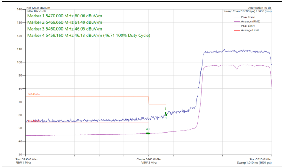
Figure 321 - 802.11ax HE40, SU, SISO, Core 0 - 5510 MHz Band Edge Frequency 5470 MHz
