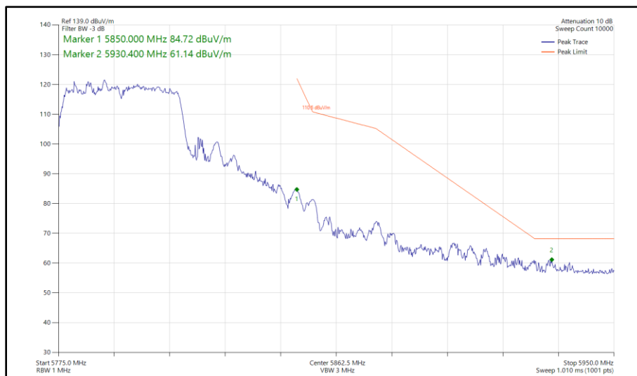
Figure 371 - 802.11ac VHT40, TxBF, Core 0 - Core 1 - 5795 MHz Band Edge Frequency 5850 MHz
