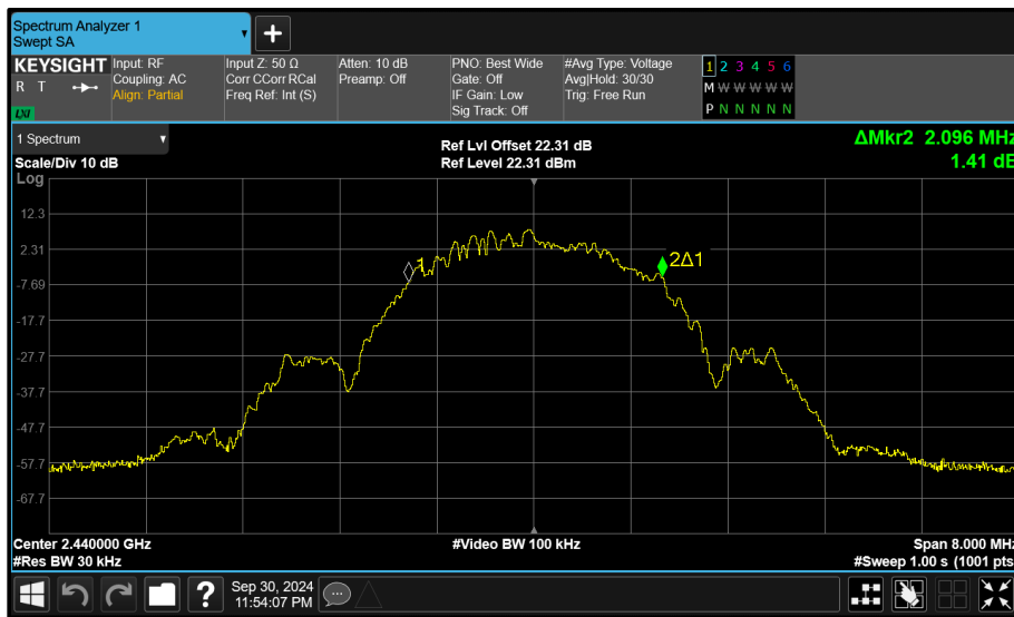
Figure 233 - Core 1 (B) 2440 MHz (CH17) 99% Bandwidth
