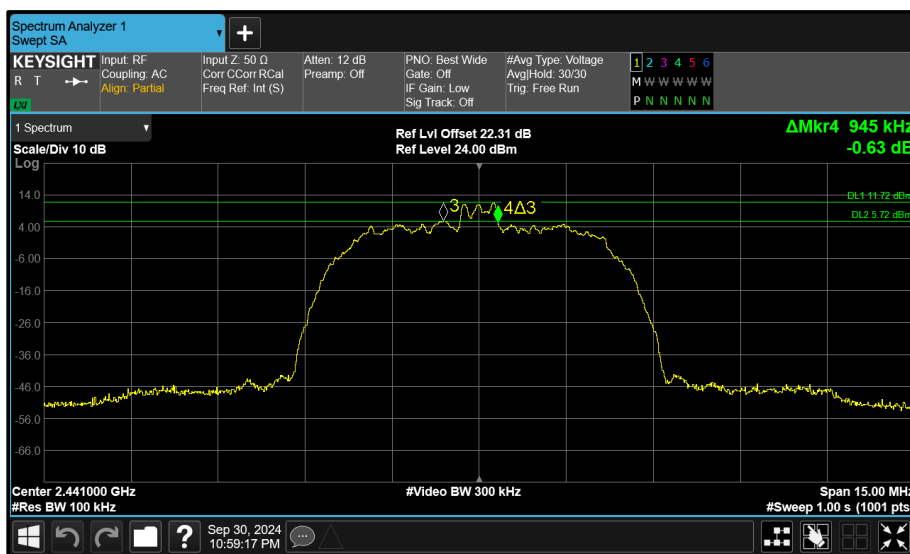
Figure 210 - Core 1 (B) 2441 MHz (CH39) 6 dB Bandwidth
