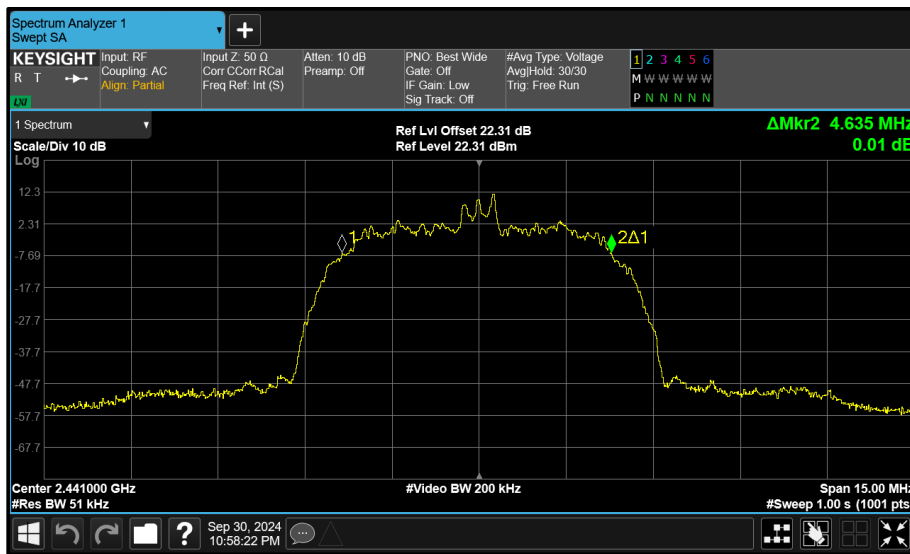
Figure 209 - Core 1 (B) 2441 MHz (CH39) 99% Bandwidth
