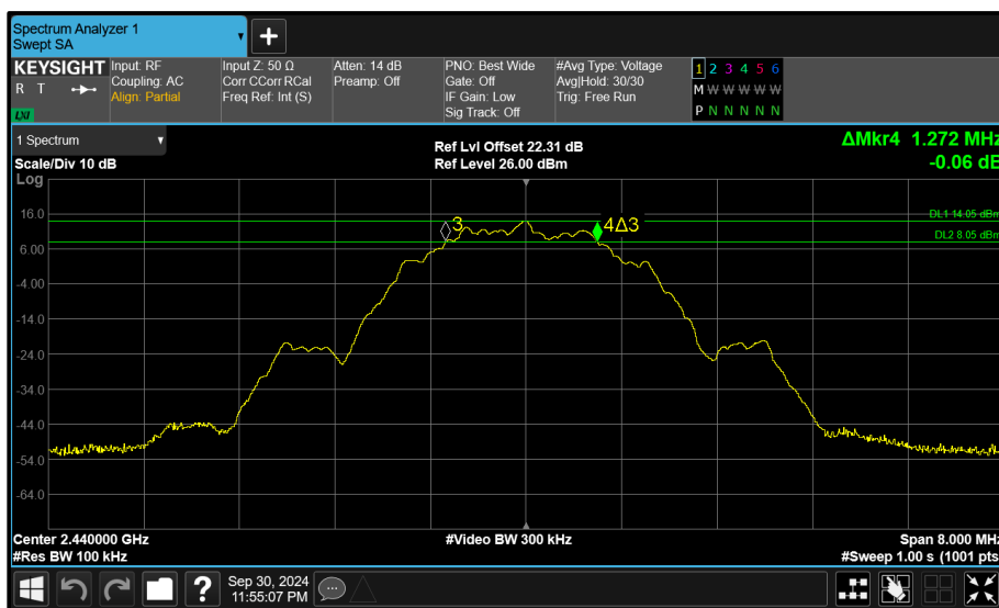
Figure 234 - Core 1 (B) 2440 MHz (CH17) 6 dB Bandwidth
