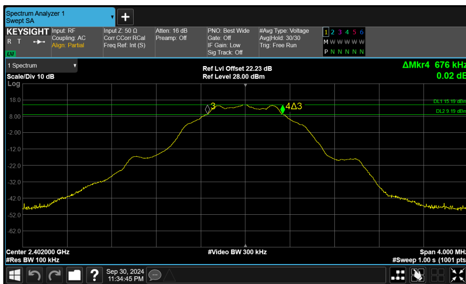
Figure 218 - Core 1 (B) 2402 MHz (CH37) 6 dB Bandwidth
