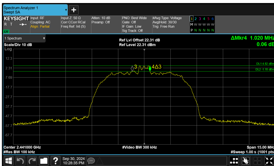
Figure 162 - Core 1 (B) 2441 MHz (CH39) 6 dB Bandwidth
