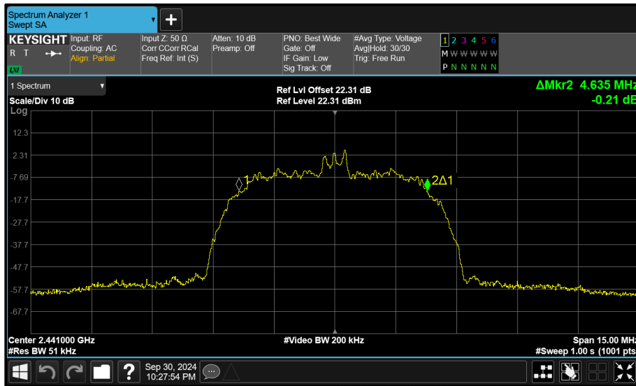
Figure 161 - Core 1 (B) 2441 MHz (CH39) 99% Bandwidth
