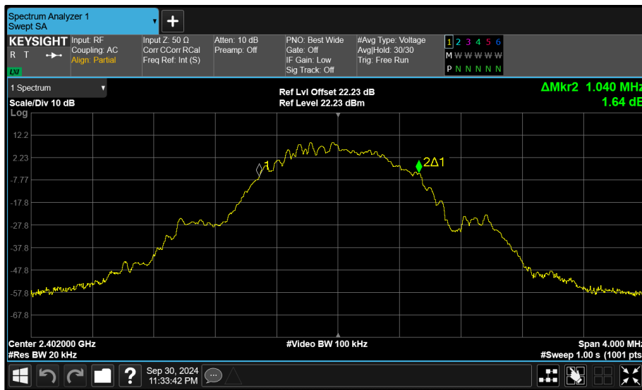
Figure 217 - Core 1 (B) 2402 MHz (CH37) 99% Bandwidth
