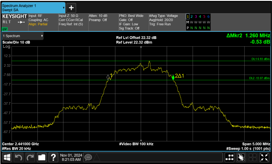
Figure 159 - Core 0 (A) 2441 MHz (CH39) 20 dB Bandwidth
