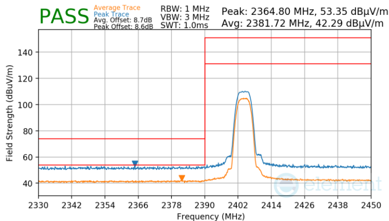
Plot 7-94. Radiated Restricted Lower Band Edge Measurement TxBF
