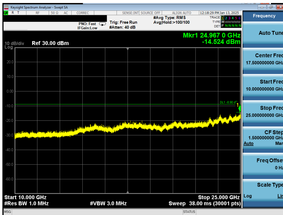
Plot 7-78. Conducted Spurious Plot Antenna 1a (Bluetooth (HDR4), 4 Mbps, ePA – Ch. 38)
