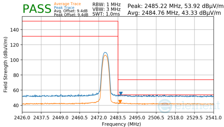
Plot 7-95. Radiated Restricted Upper Band Edge Measurement TxBF
