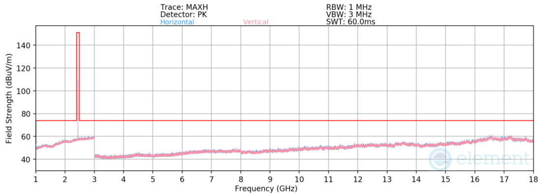
Plot 7-82. Radiated Spurious Emissions 1-18GHz TxBF (4Mbps, HDR4, ePA – Ch. 38)
