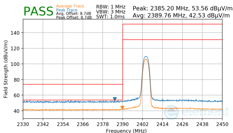
Plot 7-85. Radiated Restricted Lower Band Edge Measurement Antenna 3a
