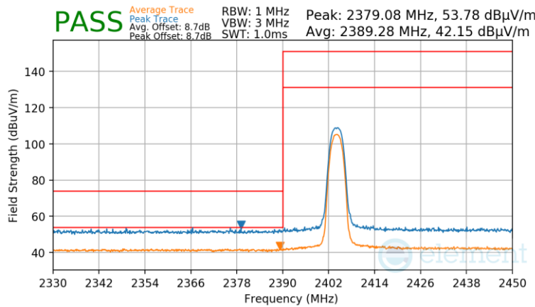
Plot 7-89. Radiated Restricted Lower Band Edge Measurement Antenna 1a
