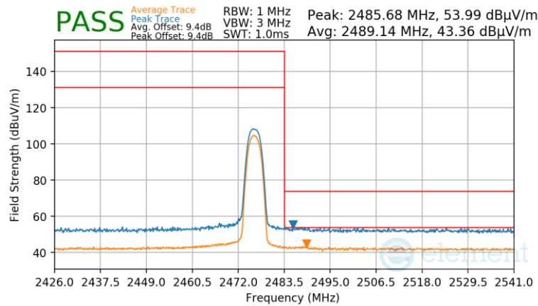
Plot 7-87. Radiated Restricted Upper Band Edge Measurement Antenna 3a
