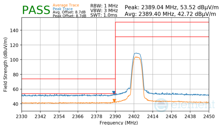
Plot 7-86. Radiated Restricted Lower Band Edge Measurement Antenna 3a
