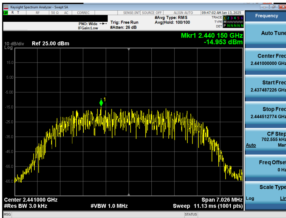
Plot 7-23. Power Spectral Density Plot Antenna 3a (Bluetooth (HDR8), 8Mbps, iPA – Ch. 38)
