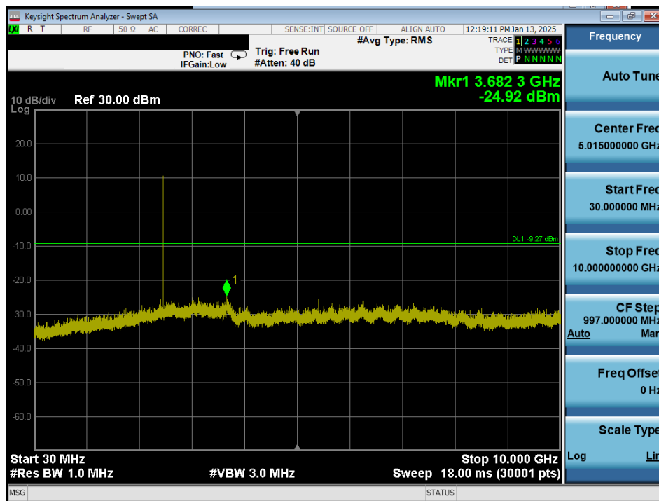
Plot 7-79. Conducted Spurious Plot Antenna 1a (Bluetooth (HDR4), 4 Mbps, ePA – Ch. 73)
