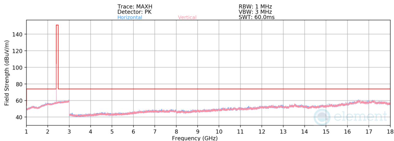
Plot 7-81. Radiated Spurious Emissions 1-18GHz TxBF (4Mbps, HDR4, ePA – Ch. 1)
