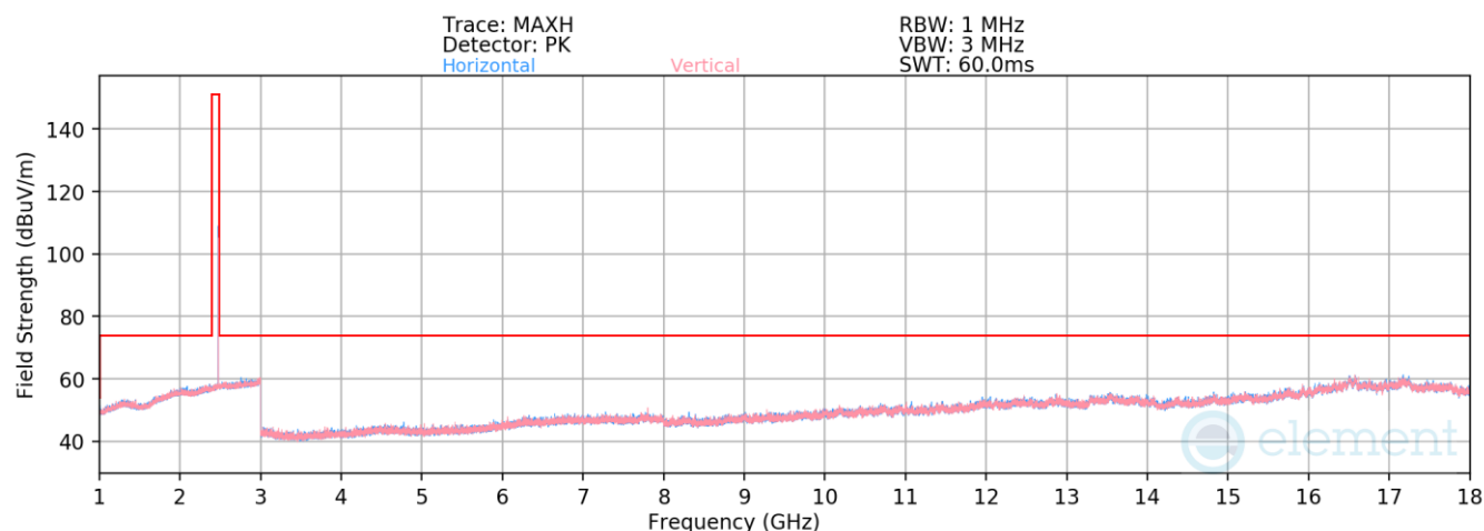
Plot 7-84. Radiated Spurious Emissions 1-18GHz TxBF (4Mbps, HDR4, ePA – Ch. 73)
