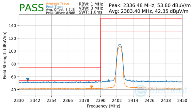
Plot 7-93. Radiated Restricted Lower Band Edge Measurement TxBF
