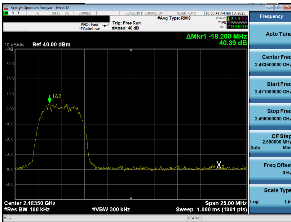
Plot 7-64. Band Edge Plot Antenna 3a (Bluetooth (HDR8), ePA – Ch. 73)
