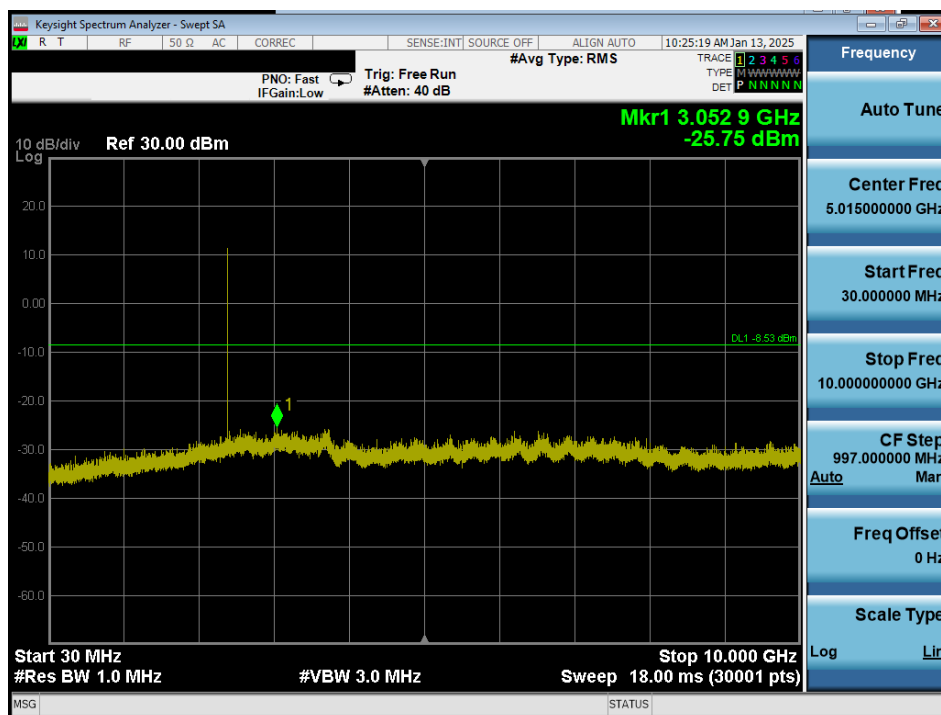
Plot 7-69. Conducted Spurious Plot Antenna 3a (Bluetooth (HDR4), 4 Mbps, ePA – Ch. 1)
