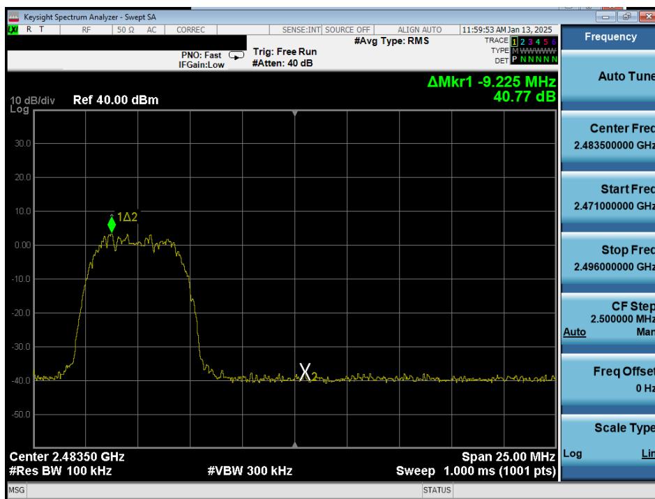
Plot 7-68. Band Edge Plot Antenna 1a (Bluetooth (HDR8), ePA – Ch. 73)
