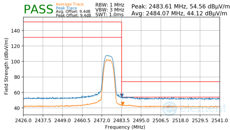
Plot 7-88. Radiated Restricted Upper Band Edge Measurement Antenna 3a
