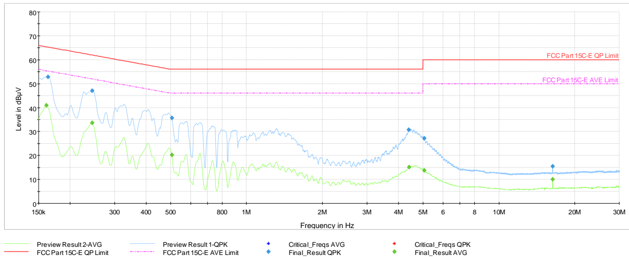
Plot 7-98. AC Line Conducted Plot with Bluetooth HDR Tx BF (L1, 4Mbps ePA - Ch.38 with AC/DC Adapter via USB-C cable with wire charger)
