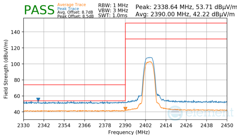
Plot 7-90. Radiated Restricted Lower Band Edge Measurement Antenna 1a
