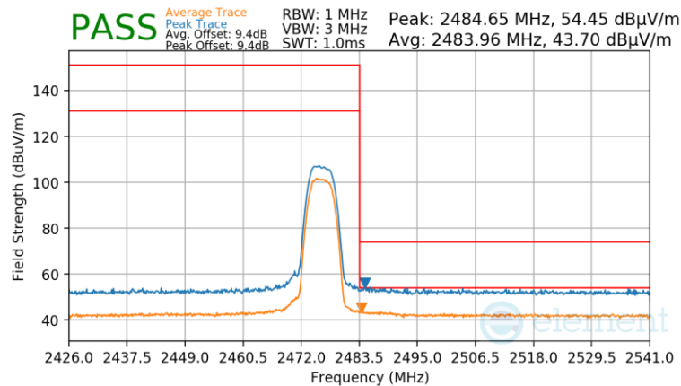
Plot 7-92. Radiated Restricted Upper Band Edge Measurement Antenna 1a
