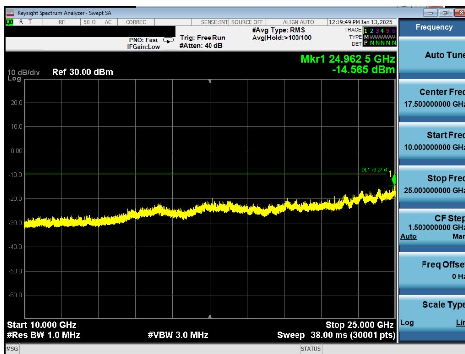
Plot 7-80. Conducted Spurious Plot Antenna 1a (Bluetooth (HDR4), 4 Mbps, ePA – Ch. 73)
