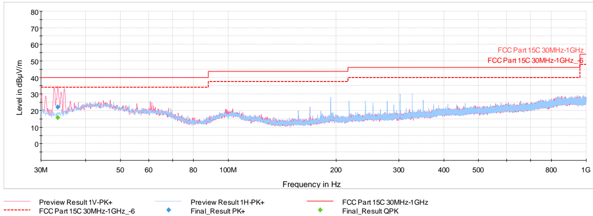
Plot 7-97. Radiated Spurious Emissions Below 1GHz TxBF (4Mbps, ePA – Ch.38 with AC/DC Adapter via USB-C cable with wire charger)
