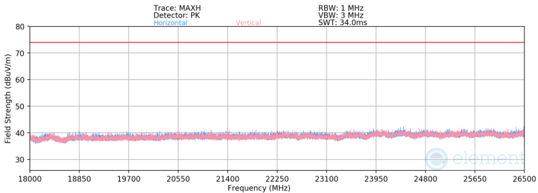
Plot 7-83. Radiated Spurious Emissions Above 18GHz TxBF (4Mbps, HDR4, ePA – Ch. 38)
