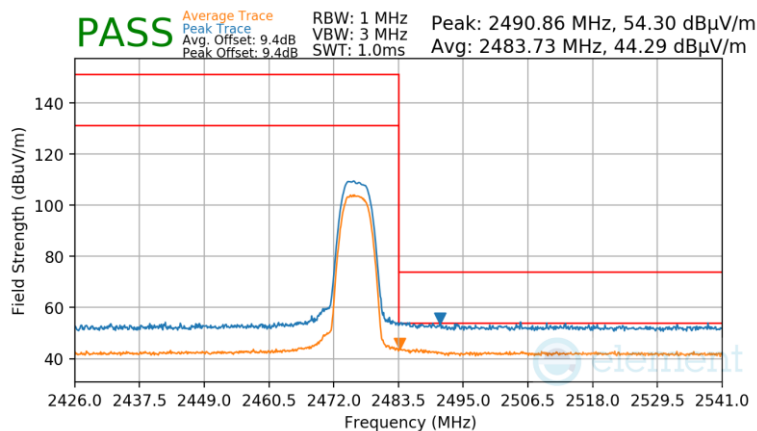
Plot 7-96. Radiated Restricted Upper Band Edge Measurement TxBF
