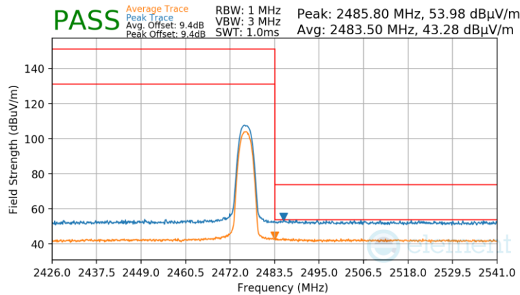
Plot 7-91. Radiated Restricted Upper Band Edge Measurement Antenna 1a
