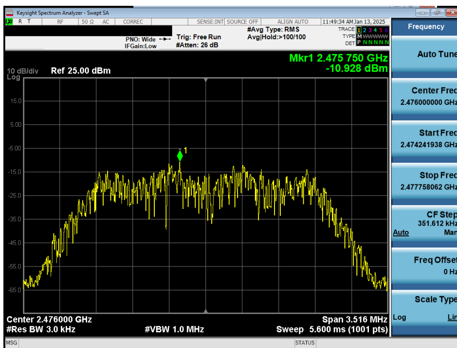
Plot 7-48. Power Spectral Density Plot TxBF Antenna 1a (Bluetooth (HDR4), 4Mbps, iPA – Ch. 73)
