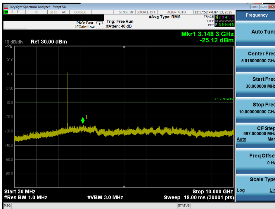
Plot 7-77. Conducted Spurious Plot Antenna 1a (Bluetooth (HDR4), 4 Mbps, ePA – Ch. 38)
