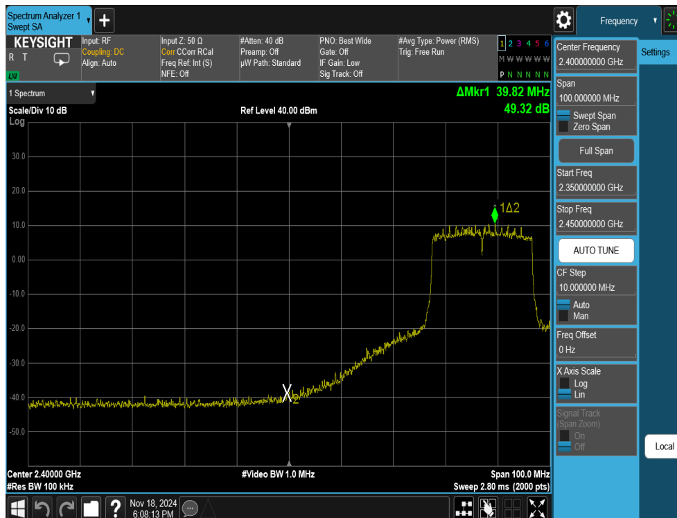
Plot 7-21. Band Edge Antenna 3a (802.11ax OFDMA – RU242 – Ch. 6(Low Channel))
