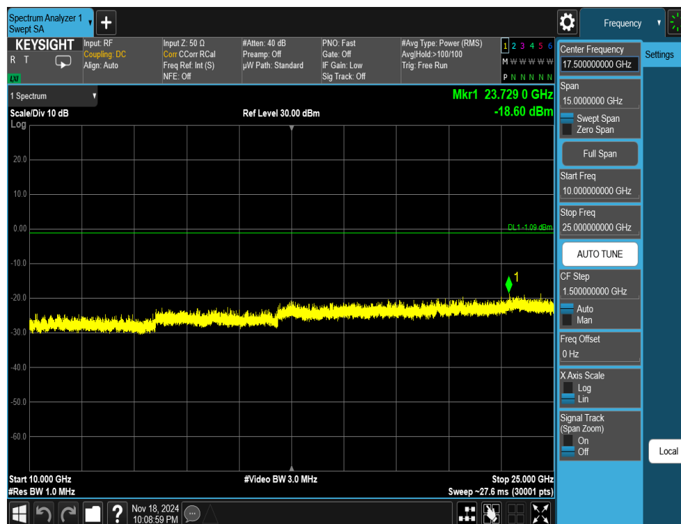
Plot 7-58. Conducted Spurious Plot Antenna 1a (802.11ax OFDMA – RU26 – Ch. 1)
