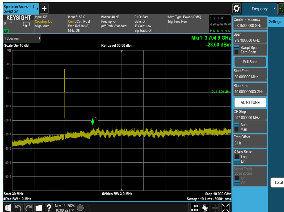
Plot 7-57. Conducted Spurious Plot Antenna 1a (802.11ax OFDMA – RU26 – Ch. 1)
