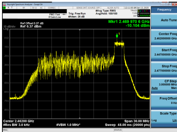
Plot 7-10. Power Spectral Density Plot Antenna 1a (802.11ax OFDMA – RU26 Index 8 – Ch. 11)
