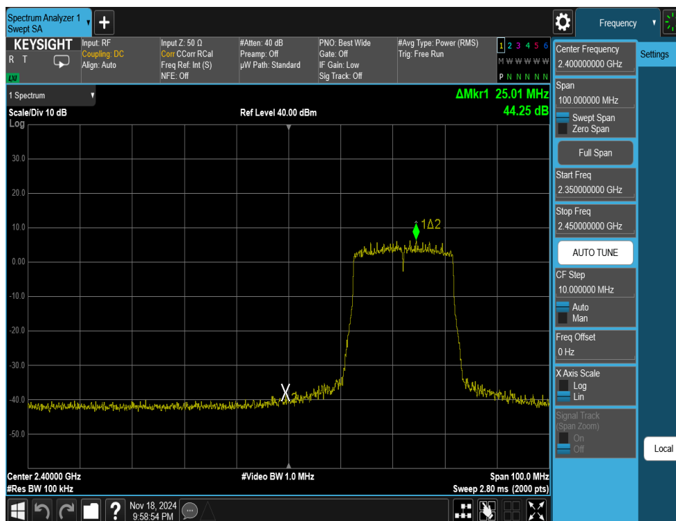
Plot 7-34. Band Edge Antenna 1a (802.11ax OFDMA – RU242 – Ch. 3)
