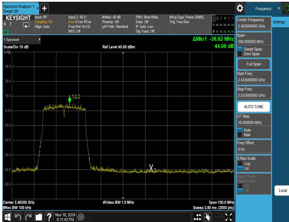
Plot 7-26. Band Edge Antenna 3a (802.11ax OFDMA – RU242 – Ch. 10)
