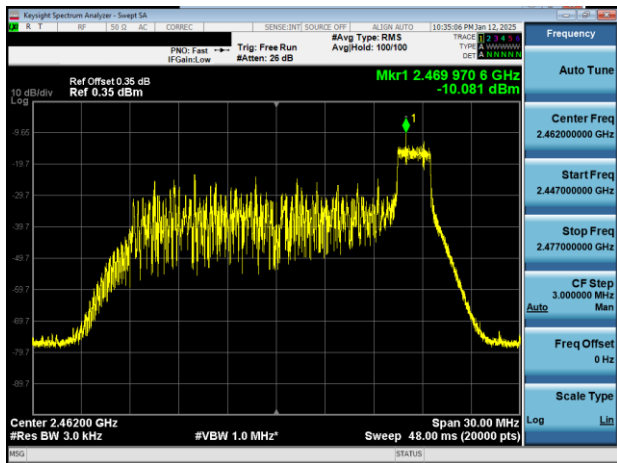
Plot 7-5. Power Spectral Density Plot Antenna 3a (802.11ax OFDMA – RU26 Index 8 – Ch. 11)
