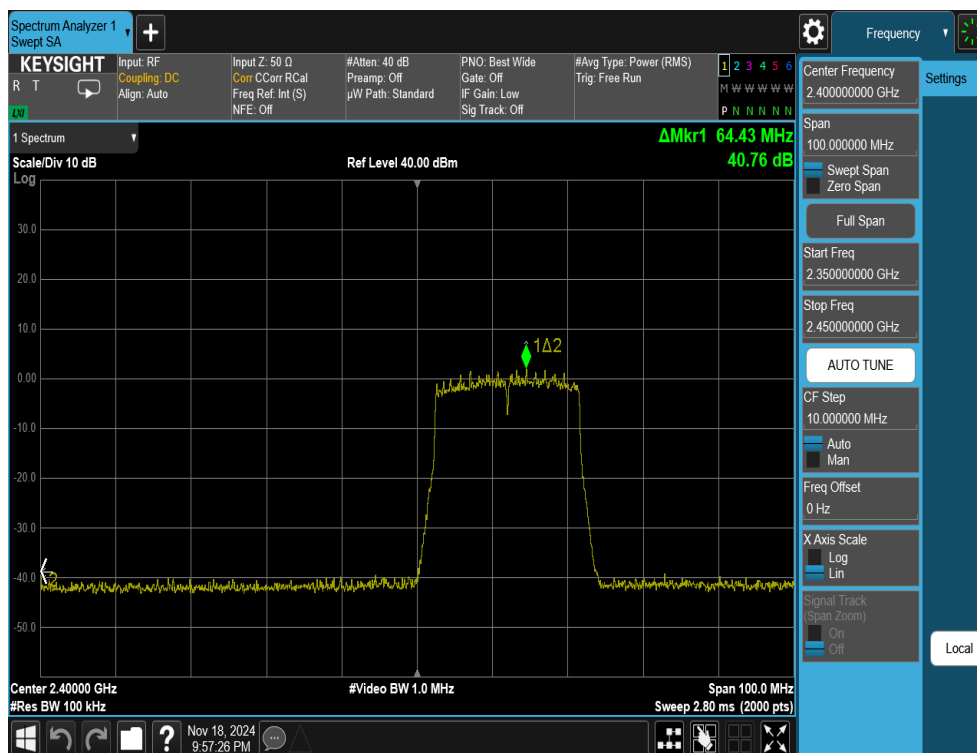
Plot 7-32. Band Edge Antenna 1a (802.11ax OFDMA – RU242 – Ch. 1)
