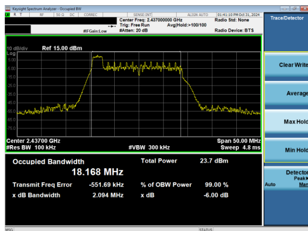
Plot 7-1. 6dB BW & 99% OBW Plot Antenna 3a (802.11ax OFDMA – RU26 Index 0 – Ch. 6)
