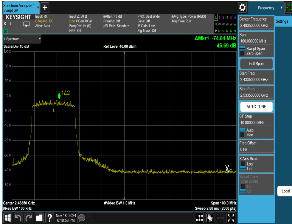
Plot 7-25. Band Edge Antenna 3a (802.11ax OFDMA – RU242 – Ch. 9)
