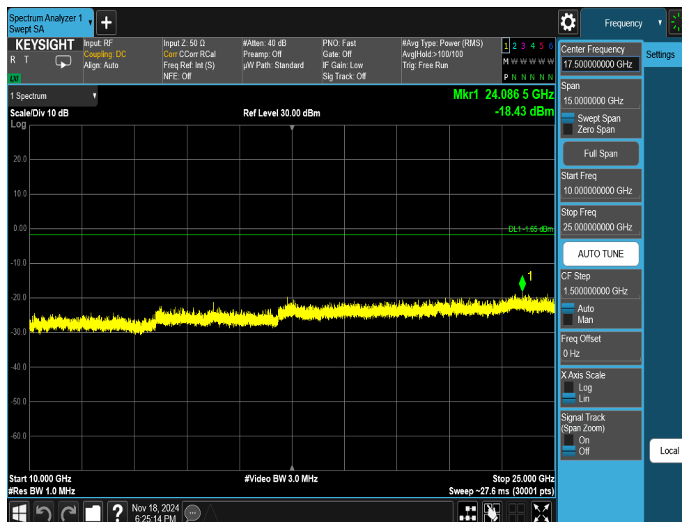
Plot 7-50. Conducted Spurious Plot Antenna 3a (802.11ax OFDMA – RU26 – Ch. 11)
