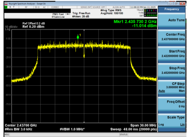
Plot 7-11. Power Spectral Density Plot Antenna 3a (802.11ax OFDMA – RU242 – Ch. 6)
