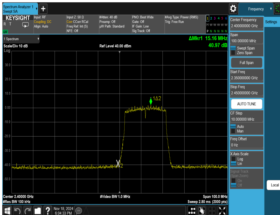
Plot 7-16. Band Edge Antenna 3a (802.11ax OFDMA – RU242 – Ch. 1)
