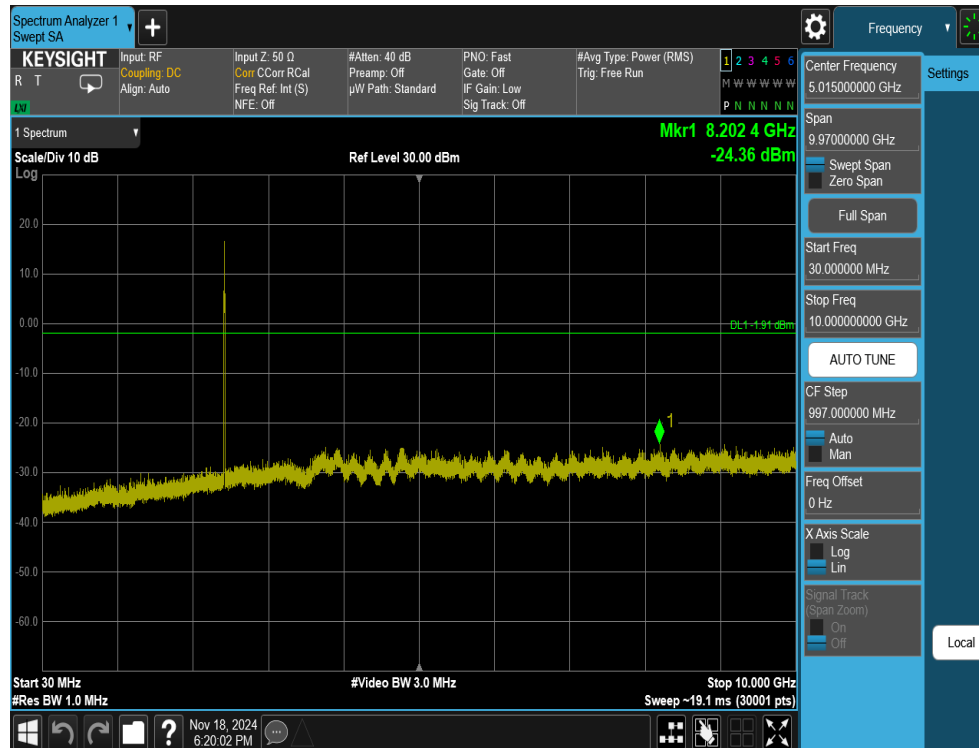
Plot 7-47. Conducted Spurious Plot Antenna 3a (802.11ax OFDMA – RU26 – Ch. 6)
