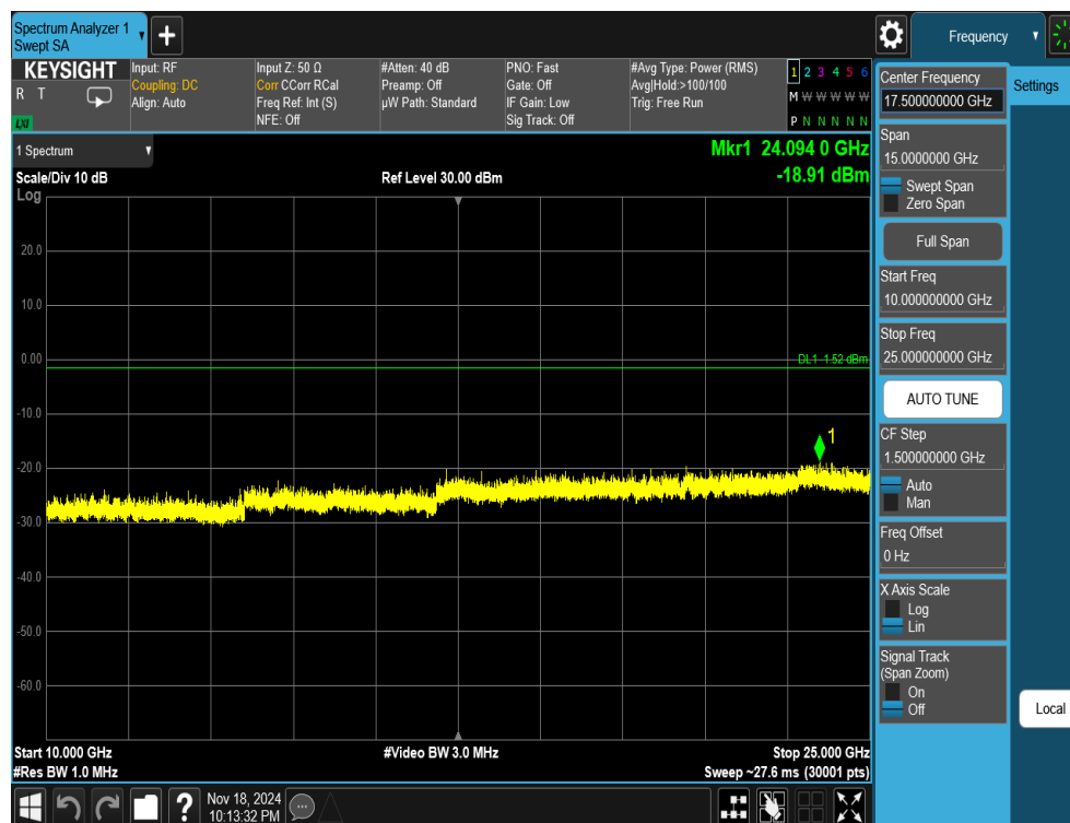
Plot 7-60. Conducted Spurious Plot Antenna 1a (802.11ax OFDMA – RU26 – Ch. 6)
