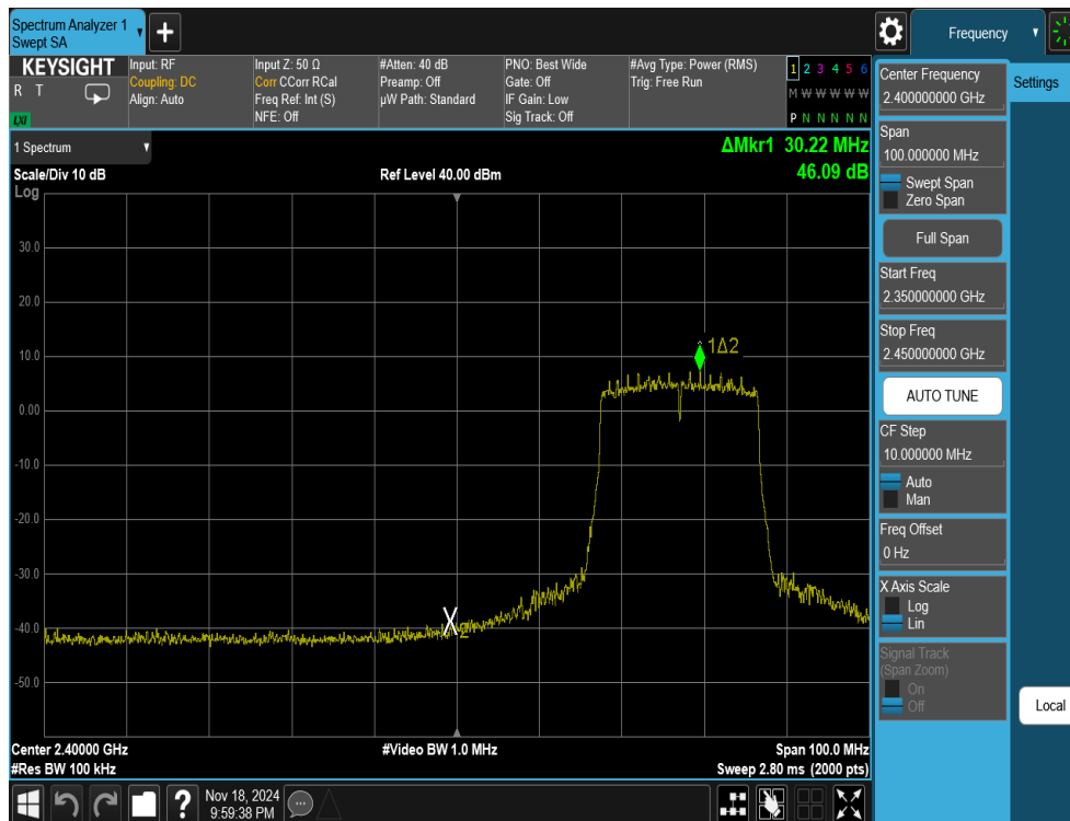
Plot 7-35. Band Edge Antenna 1a (802.11ax OFDMA – RU242 – Ch. 4)
