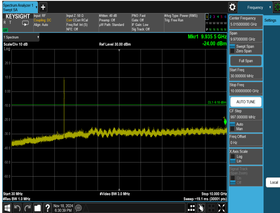
Plot 7-55. Conducted Spurious Plot Antenna 3a (802.11ax OFDMA – RU242 – Ch. 11)
