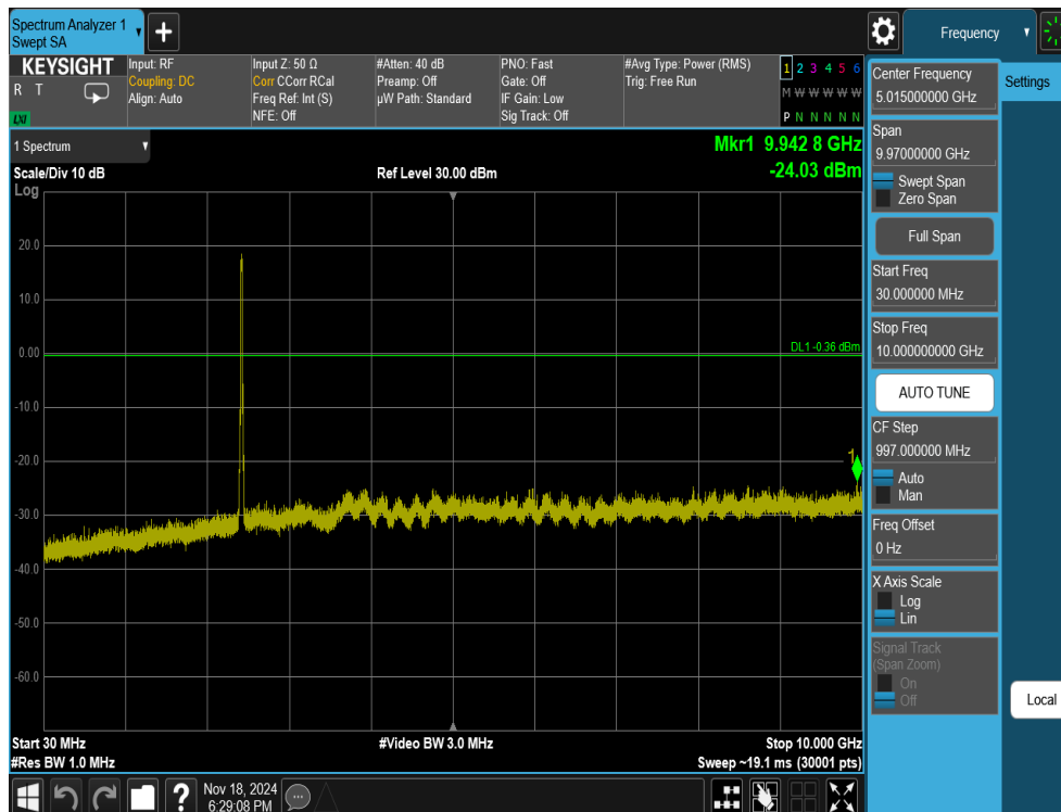
Plot 7-53. Conducted Spurious Plot Antenna 3a (802.11ax OFDMA – RU242 – Ch. 6)
