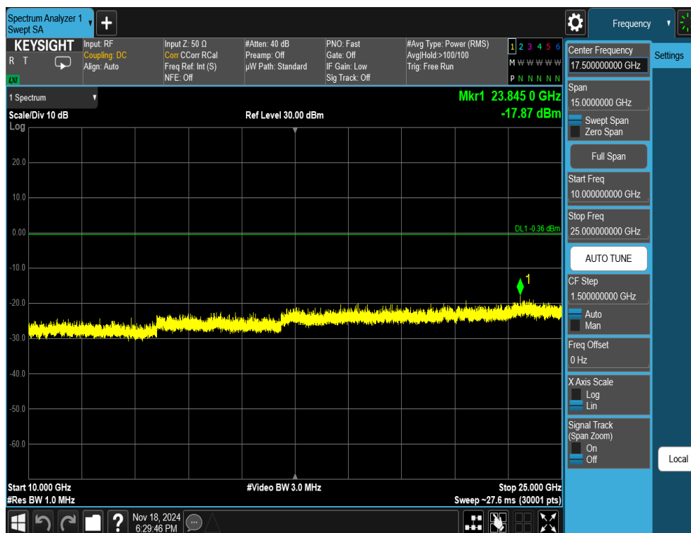
Plot 7-54. Conducted Spurious Plot Antenna 3a (802.11ax OFDMA – RU242 – Ch. 6)
