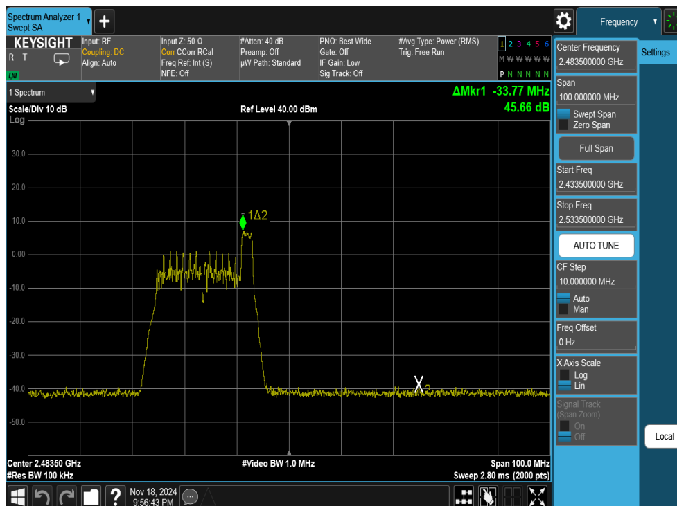
Plot 7-31. Band Edge Antenna 1a (802.11ax OFDMA – RU26 Index 8 – Ch. 12)
