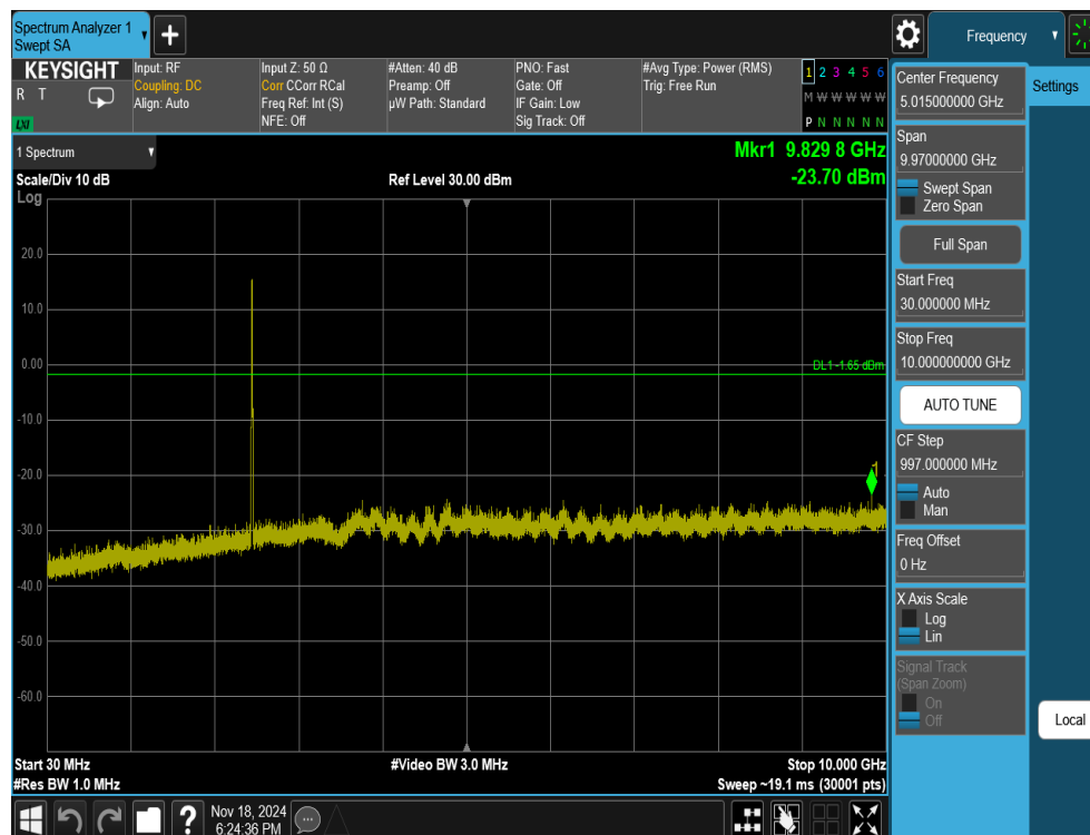
Plot 7-49. Conducted Spurious Plot Antenna 3a (802.11ax OFDMA – RU26 – Ch. 11)
