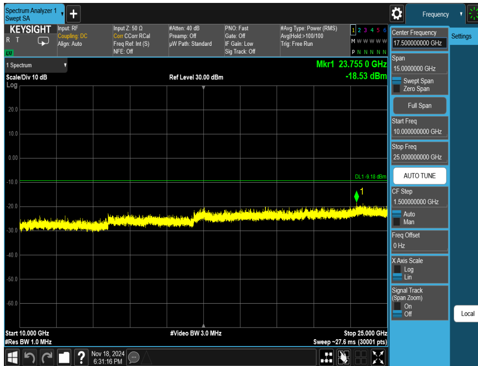
Plot 7-56. Conducted Spurious Plot Antenna 3a (802.11ax OFDMA – RU242 – Ch. 11)
