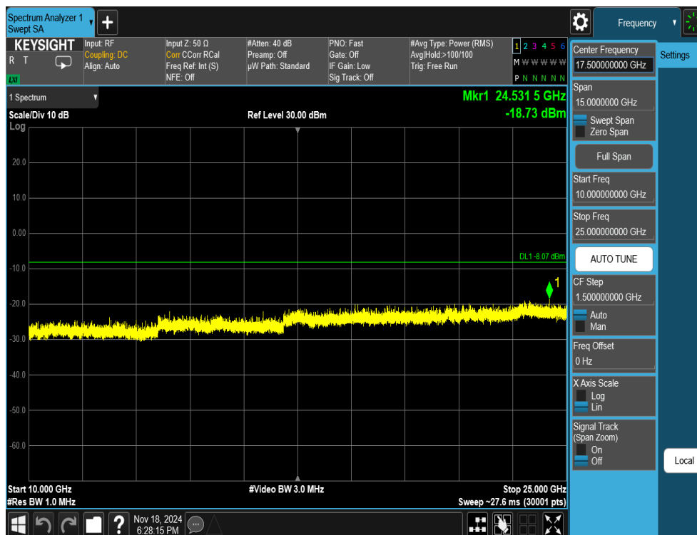
Plot 7-52. Conducted Spurious Plot Antenna 3a (802.11ax OFDMA – RU242 – Ch. 1)
