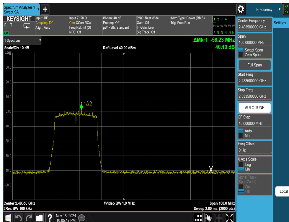
Plot 7-43. Band Edge Antenna 1a (802.11ax OFDMA – RU242 – Ch. 11)
