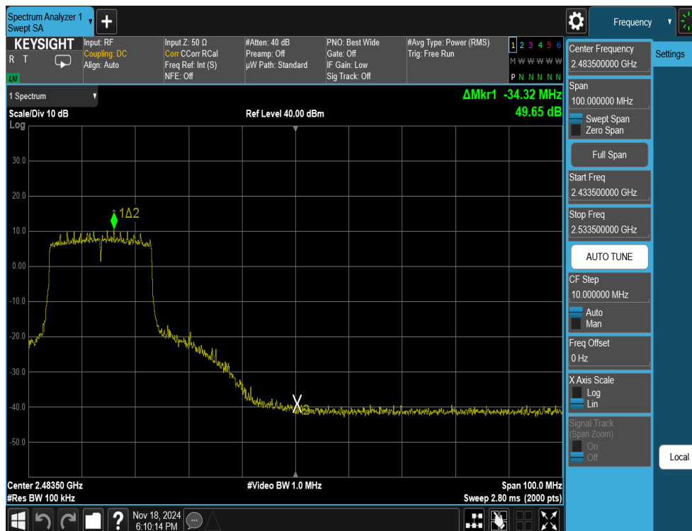
Plot 7-24. Band Edge Antenna 3a (802.11ax OFDMA – RU242 – Ch. 8)
