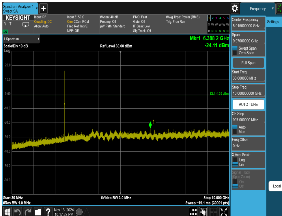
Plot 7-61. Conducted Spurious Plot Antenna 1a (802.11ax OFDMA – RU26 – Ch. 11)
