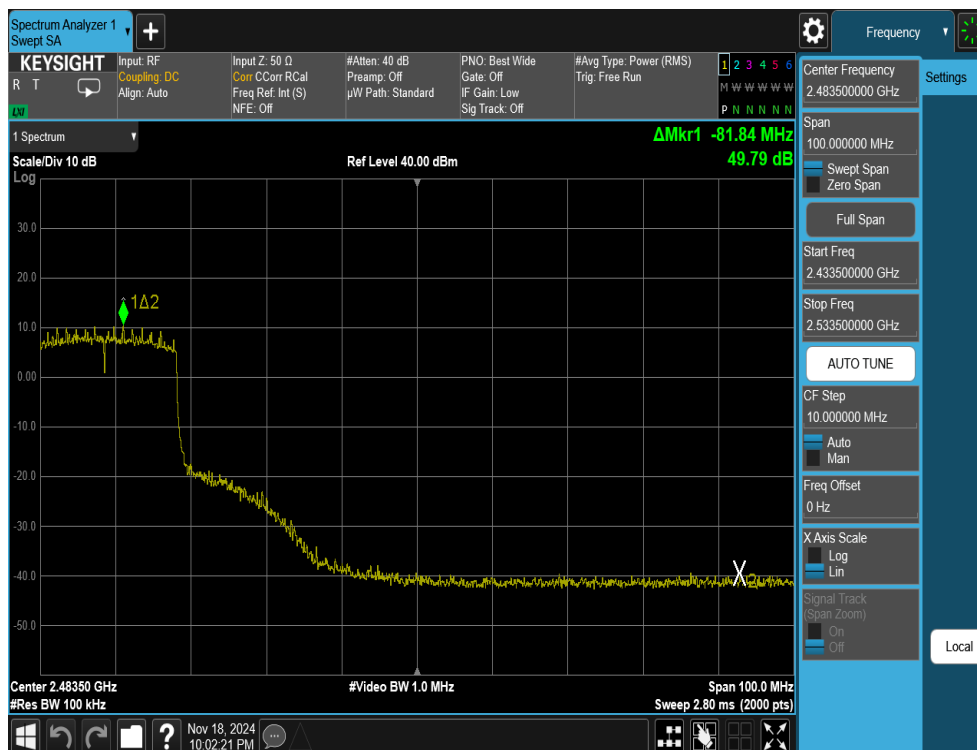
Plot 7-39. Band Edge Antenna 1a (802.11ax OFDMA – RU242 – Ch. 7)
