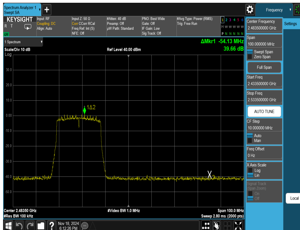
Plot 7-27. Band Edge Antenna 3a (802.11ax OFDMA – RU242 – Ch. 11)
