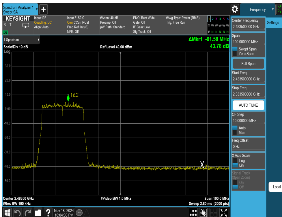
Plot 7-42. Band Edge Antenna 1a (802.11ax OFDMA – RU242 – Ch. 10)
