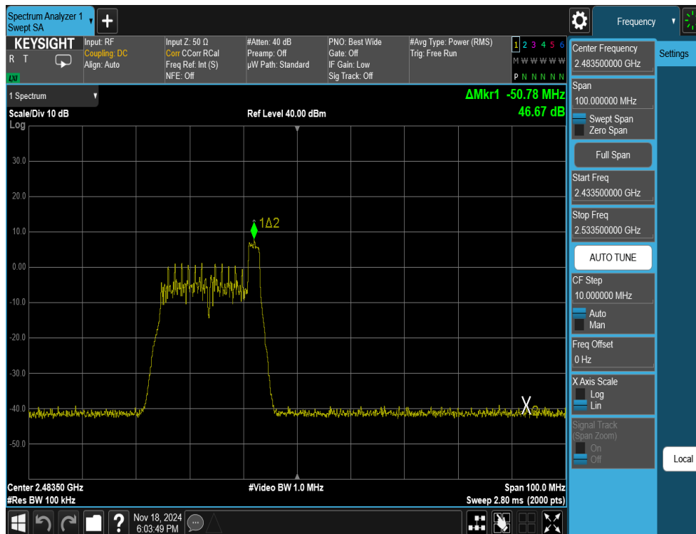
Plot 7-15. Band Edge Antenna 3a (802.11ax OFDMA – RU26 Index 8 – Ch. 12)
