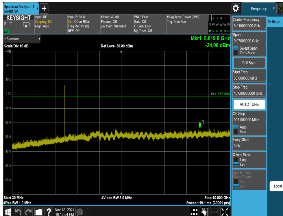
Plot 7-59. Conducted Spurious Plot Antenna 1a (802.11ax OFDMA – RU26 – Ch. 6)
