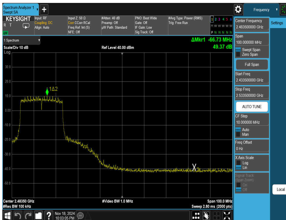
Plot 7-40. Band Edge Antenna 1a (802.11ax OFDMA – RU242 – Ch. 8)
