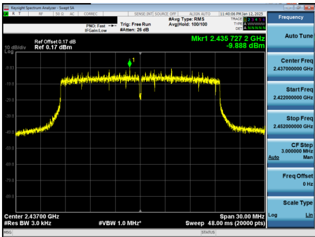
Plot 7-8. Power Spectral Density Plot Antenna 1a (802.11ax OFDMA – RU242 – Ch. 6)
