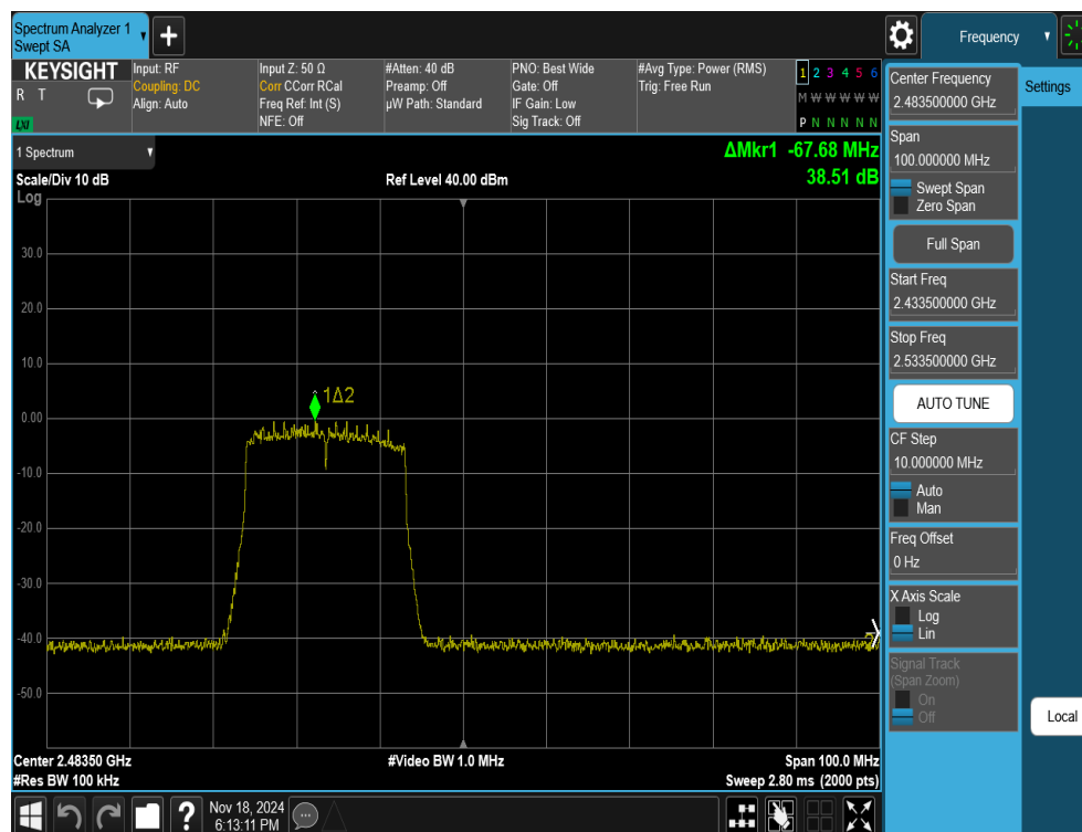
Plot 7-28. Band Edge Antenna 3a (802.11ax OFDMA – RU242 – Ch. 12)
