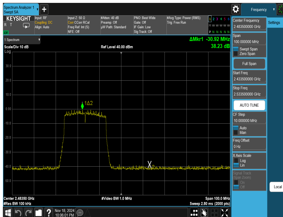
Plot 7-44. Band Edge Antenna 1a (802.11ax OFDMA – RU242 – Ch. 12)
