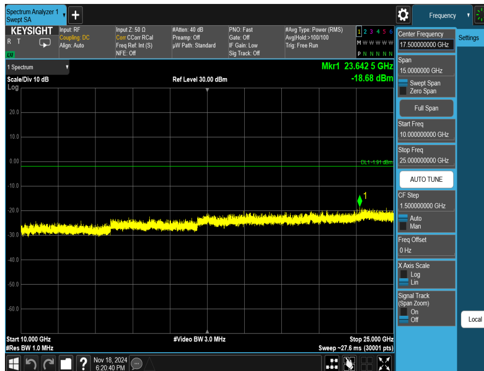
Plot 7-48. Conducted Spurious Plot Antenna 3a (802.11ax OFDMA – RU26 – Ch. 6)
