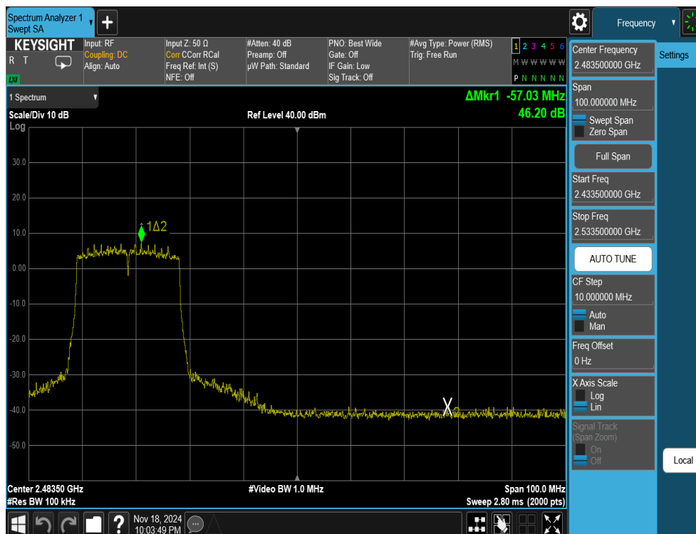
Plot 7-41. Band Edge Antenna 1a (802.11ax OFDMA – RU242 – Ch. 9)
