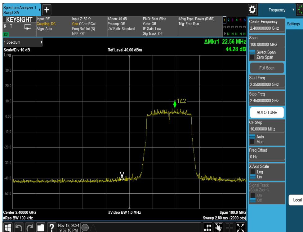
Plot 7-33. Band Edge Antenna 1a (802.11ax OFDMA – RU242 – Ch. 2)
