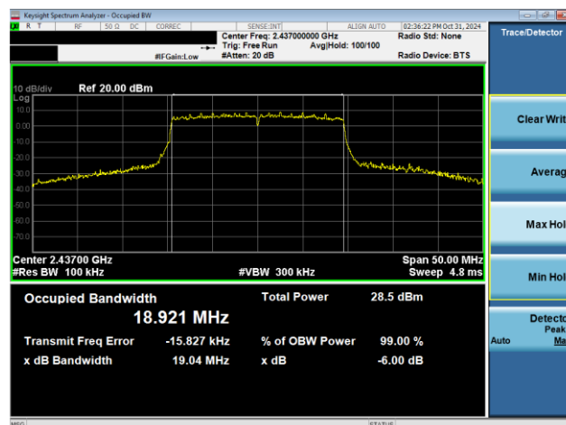
Plot 7-4. 6dB BW & 99% OBW Plot Antenna 1a (802.11ax OFDMA – RU242 – Ch. 6)
