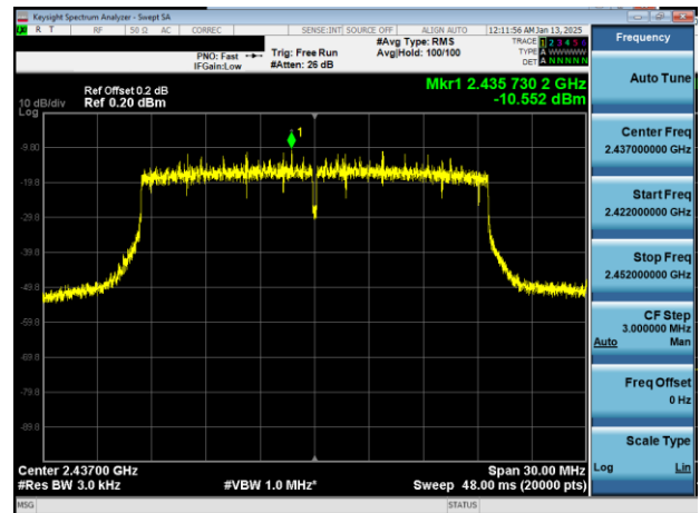
Plot 7-12. Power Spectral Density Plot Antenna 1a (802.11ax OFDMA – RU242 – Ch. 6)
