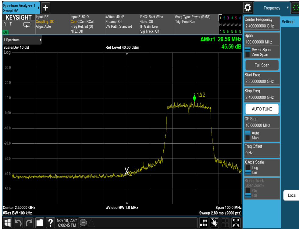
Plot 7-19. Band Edge Antenna 3a (802.11ax OFDMA – RU242 – Ch. 4)
