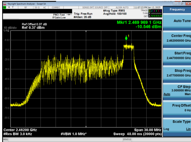
Plot 7-9. Power Spectral Density Plot Antenna 3a (802.11ax OFDMA – RU26 Index 8 – Ch. 11)
