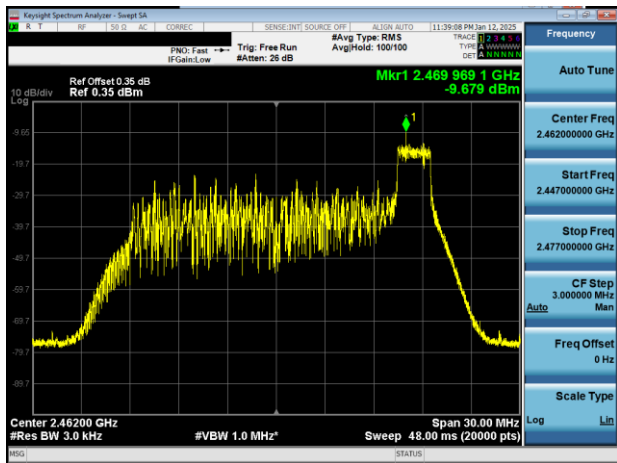
Plot 7-7. Power Spectral Density Plot Antenna 1a (802.11ax OFDMA – RU26 Index 8 – Ch. 11)
