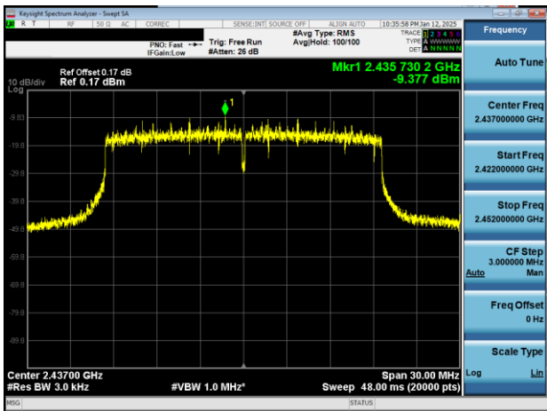
Plot 7-6. Power Spectral Density Plot Antenna 3a (802.11ax OFDMA – RU242 – Ch. 6)
