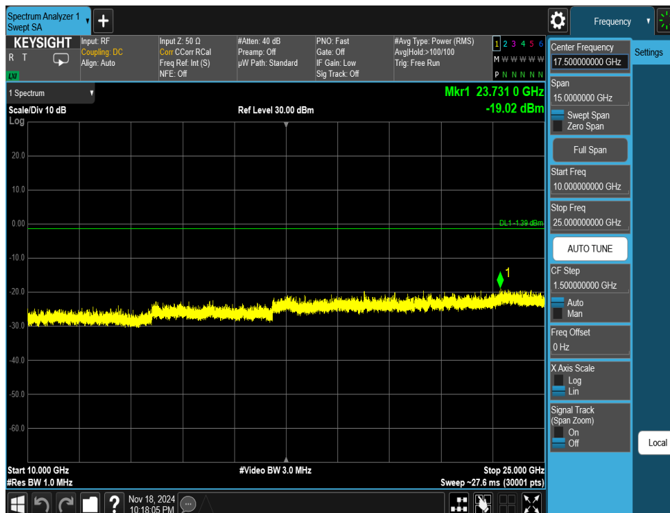
Plot 7-62. Conducted Spurious Plot Antenna 1a (802.11ax OFDMA – RU26 – Ch. 11)
