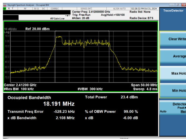
Plot 7-3. 6dB BW & 99% OBW Antenna 1a (802.11ax OFDMA – RU26 Index 0 – Ch. 1)
