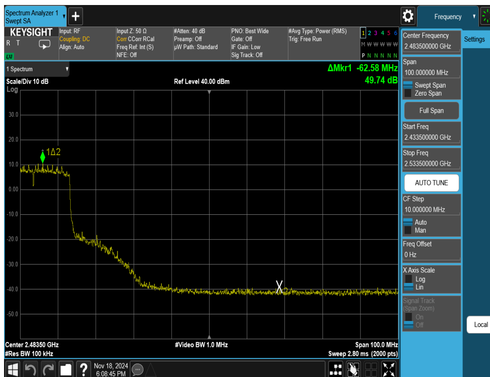
Plot 7-22. Band Edge Antenna 3a (802.11ax OFDMA – RU242 – Ch. 6(High Channel))
