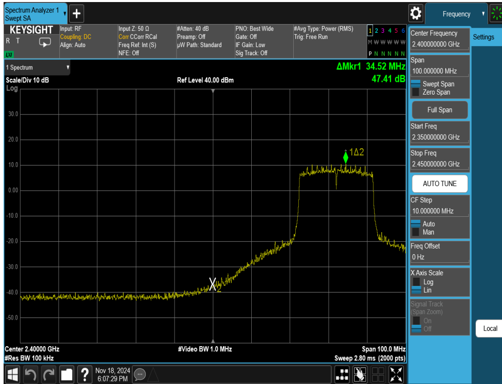
Plot 7-20. Band Edge Antenna 3a (802.11ax OFDMA – RU242 – Ch. 5)
