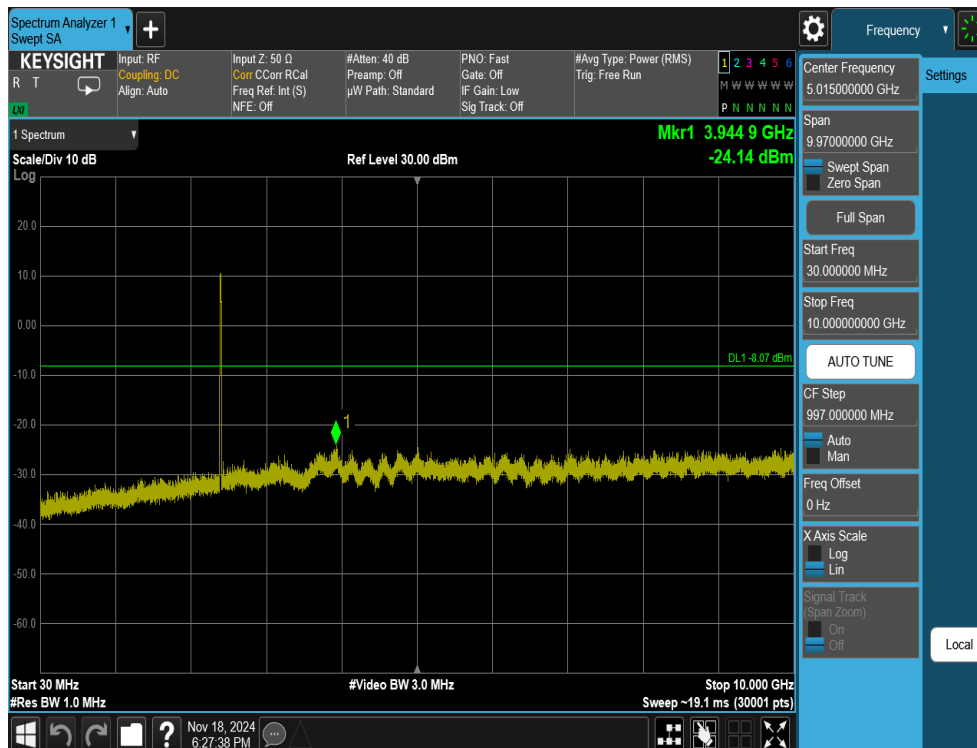
Plot 7-51. Conducted Spurious Plot Antenna 3a (802.11ax OFDMA – RU242 – Ch. 1)
