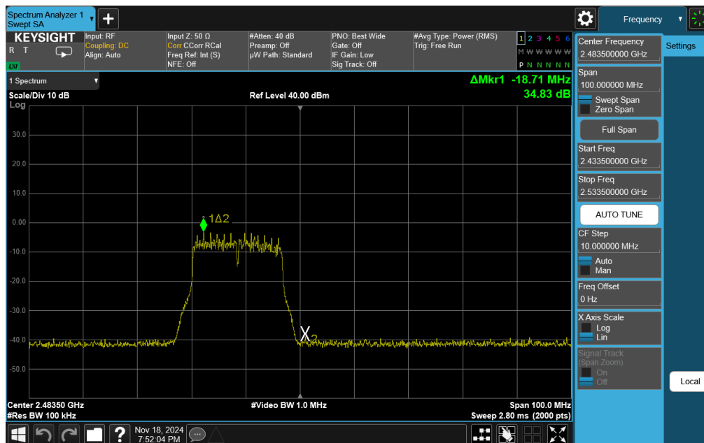
Plot 7-40. Band Edge Plot Antenna 3a (802.11g – Ch. 13)
