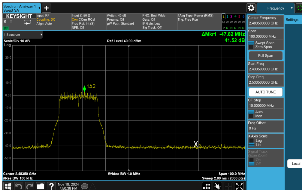
Plot 7-38. Band Edge Plot Antenna 3a (802.11g - Ch. 11)
