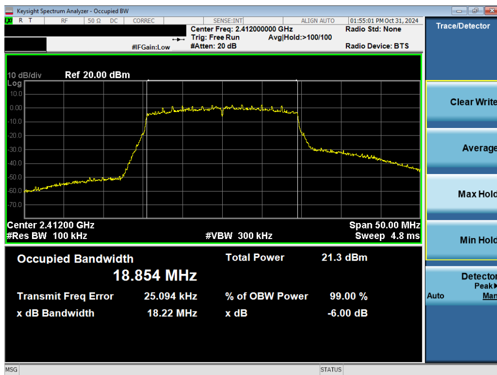
Plot 7-4. 6 dB BW and 99% OBW Plot Antenna 3a (802.11axSU – Ch. 1)
