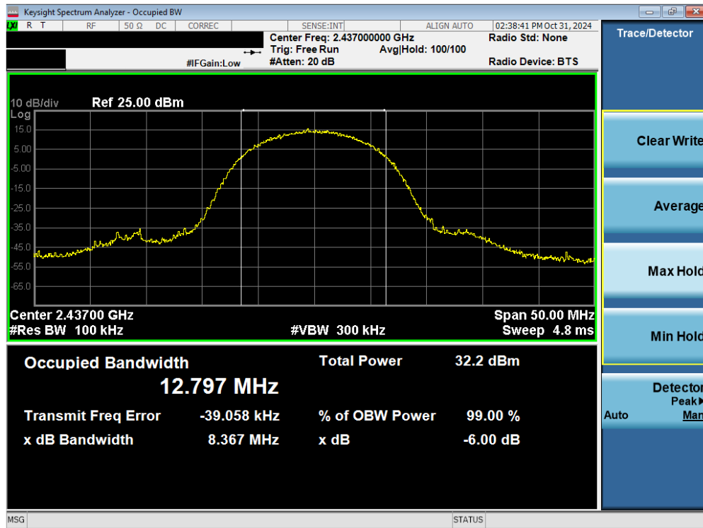
Plot 7-5. 6 dB BW and 99% OBW Plot Antenna 1a (802.11b – Ch. 6)
