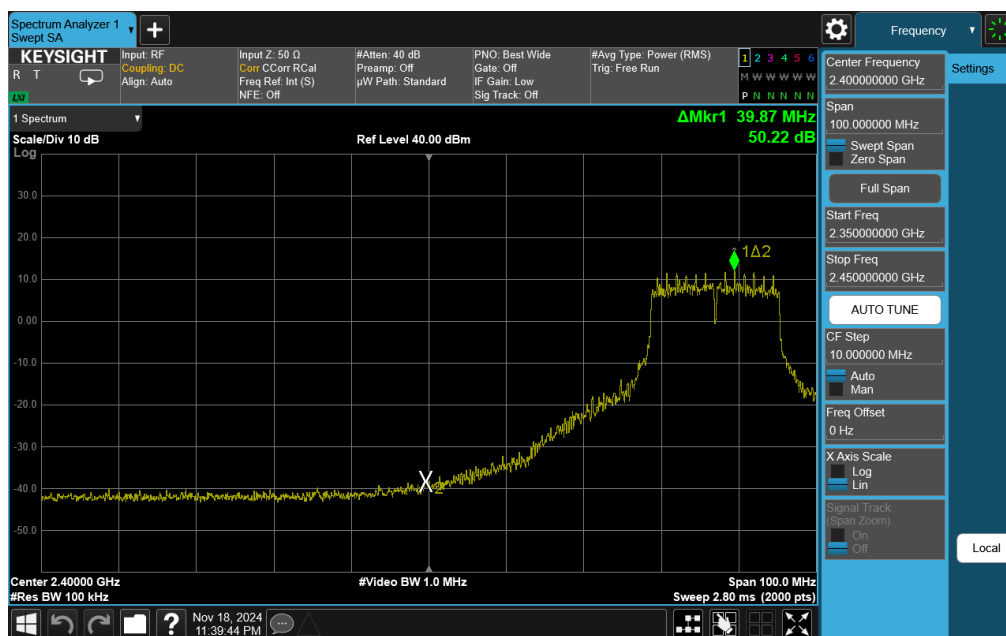
Plot 7-77. Band Edge Plot Antenna 1a (802.11g – Ch. 6-Low)
