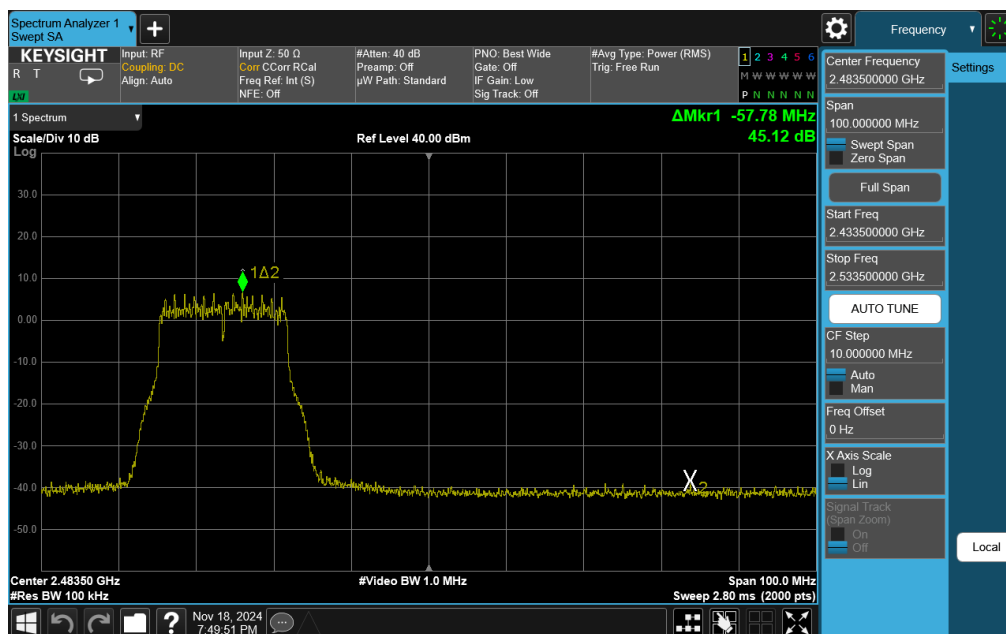
Plot 7-37. Band Edge Plot Antenna 3a (802.11g - Ch. 10)
