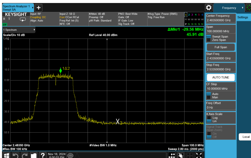
Plot 7-51. Band Edge Plot Antenna 3a (802.11n (2.4GHz) – Ch. 10)
