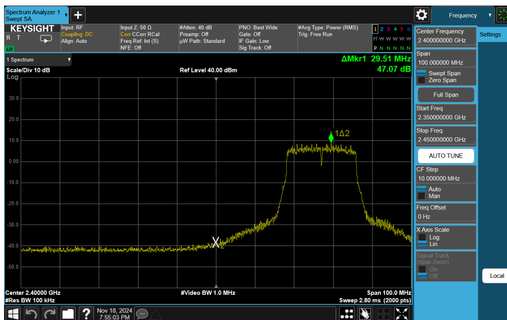
Plot 7-44. Band Edge Plot Antenna 3a (802.11n (2.4GHz) – Ch. 4)
