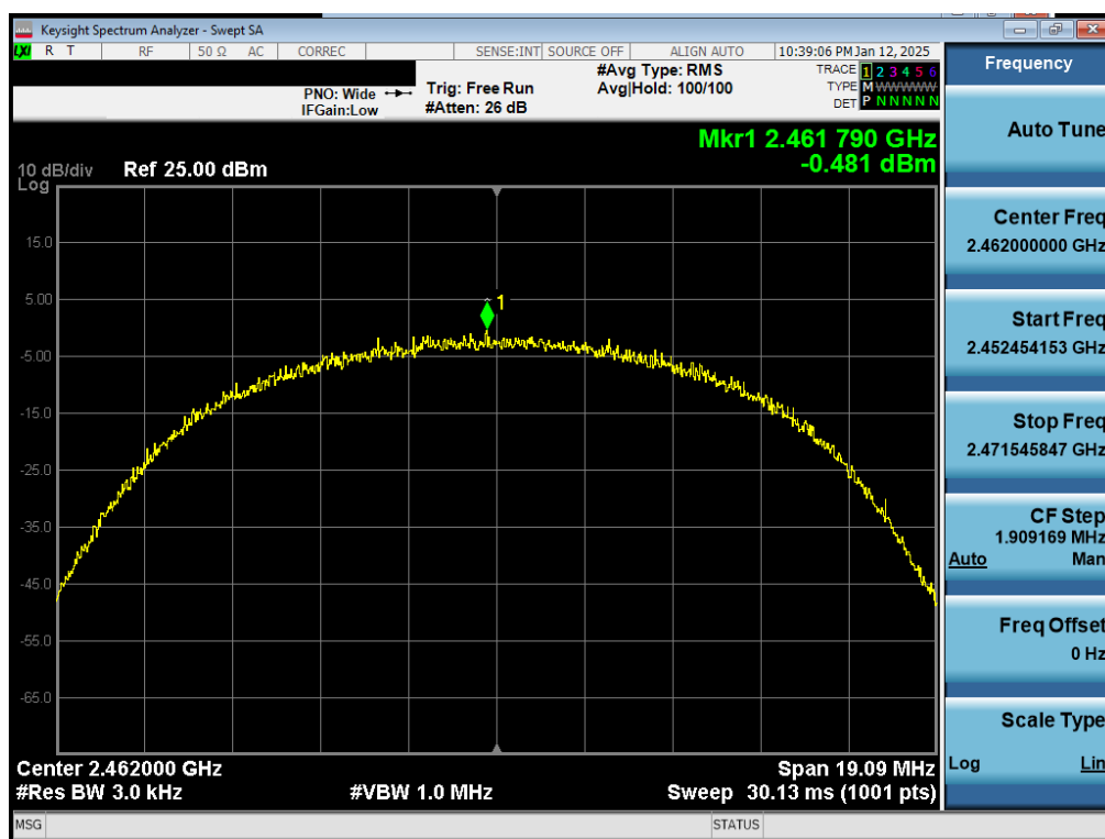
Plot 7-9. Power Spectral Density Plot Antenna 3a (802.11b – Ch. 11)
