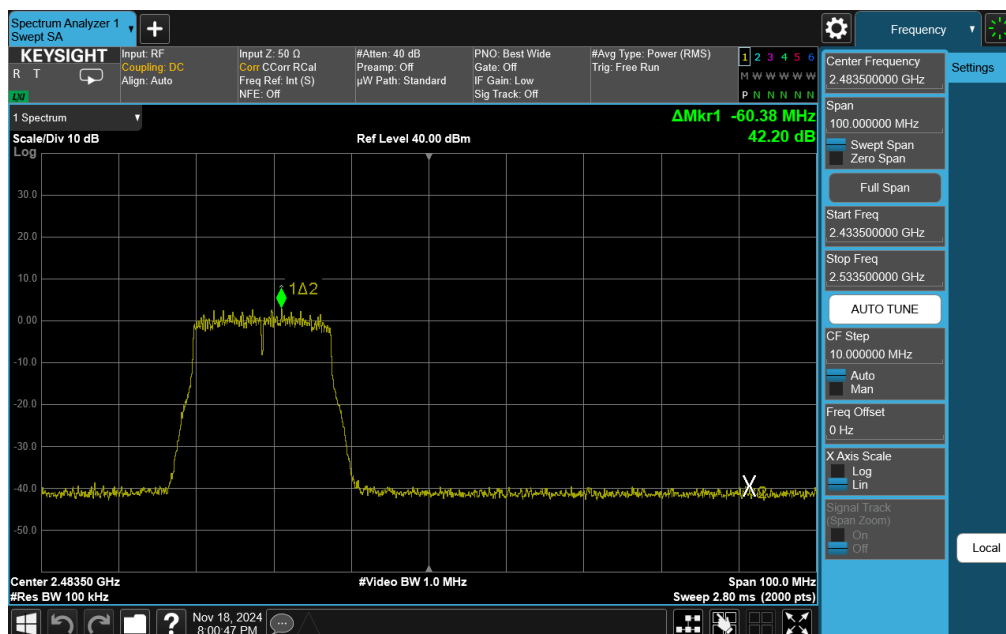
Plot 7-52. Band Edge Plot Antenna 3a (802.11n (2.4GHz) – Ch. 11)
