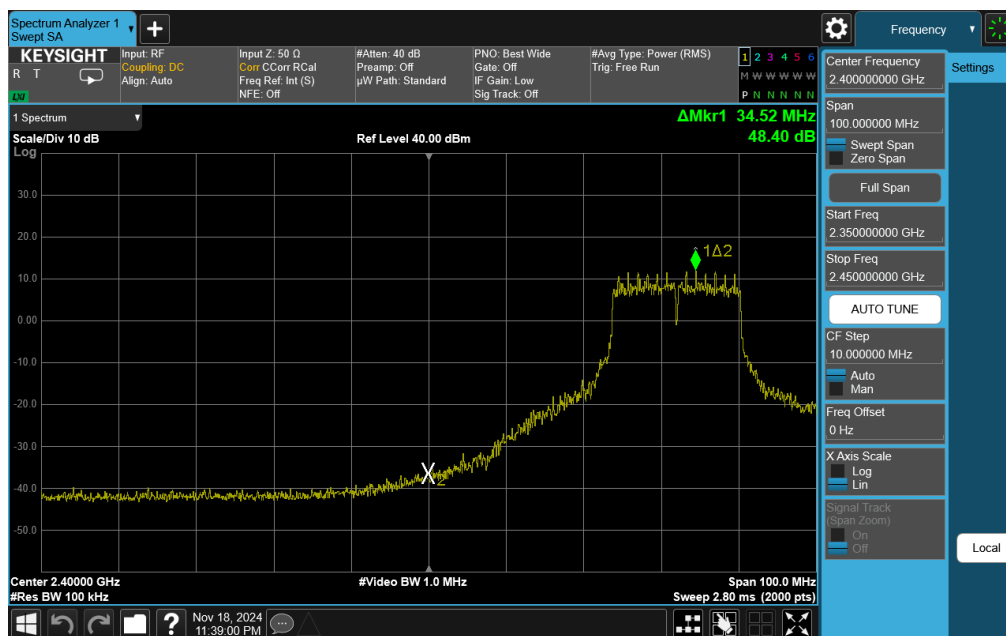
Plot 7-76. Band Edge Plot Antenna 1a (802.11g – Ch. 5)
