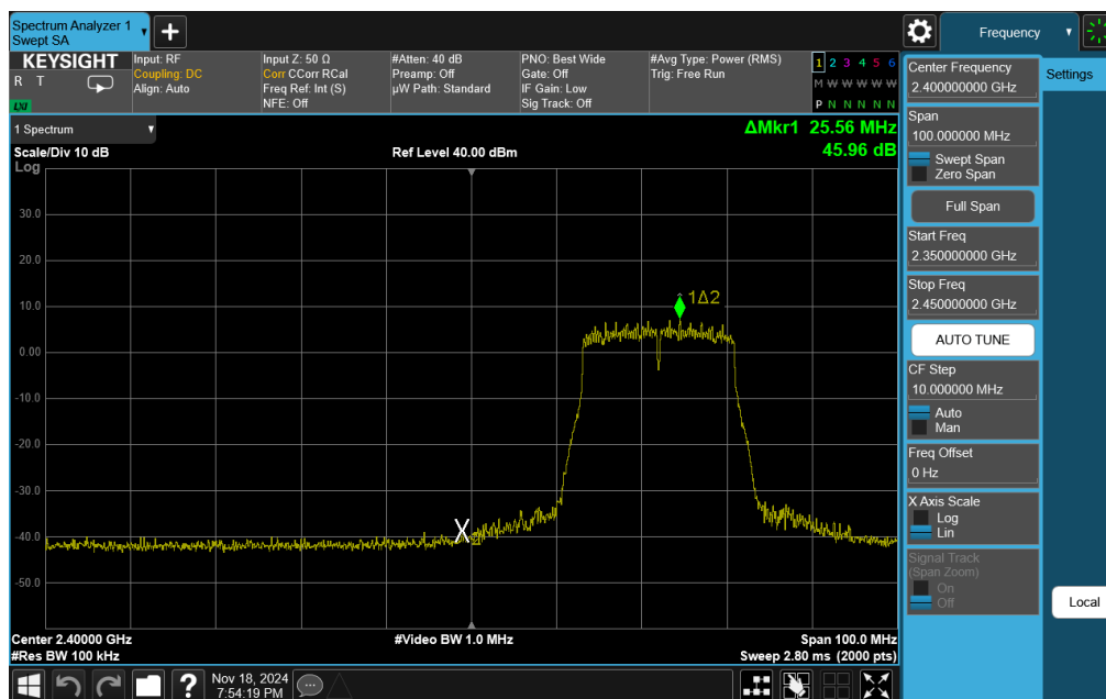
Plot 7-43. Band Edge Plot Antenna 3a (802.11n (2.4GHz) – Ch. 3)
