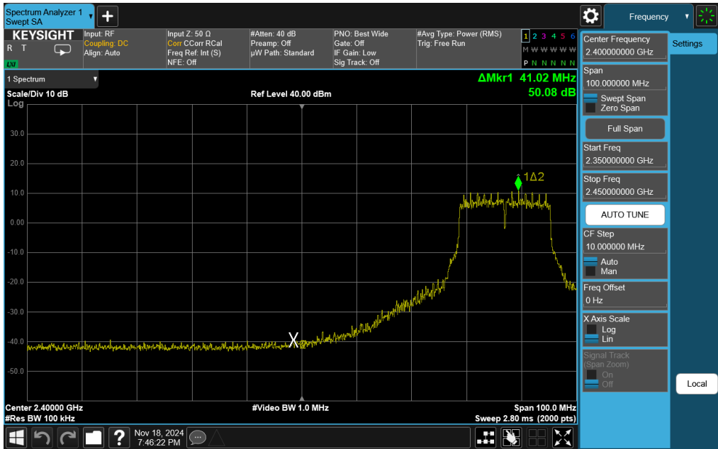
Plot 7-32. Band Edge Plot Antenna 3a (802.11g – Ch. 6-Low)
