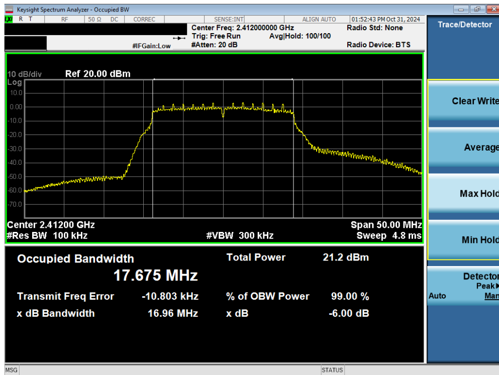
Plot 7-3. 6 dB BW and 99% OBW Plot Antenna 3a (802.11n – Ch. 1)
