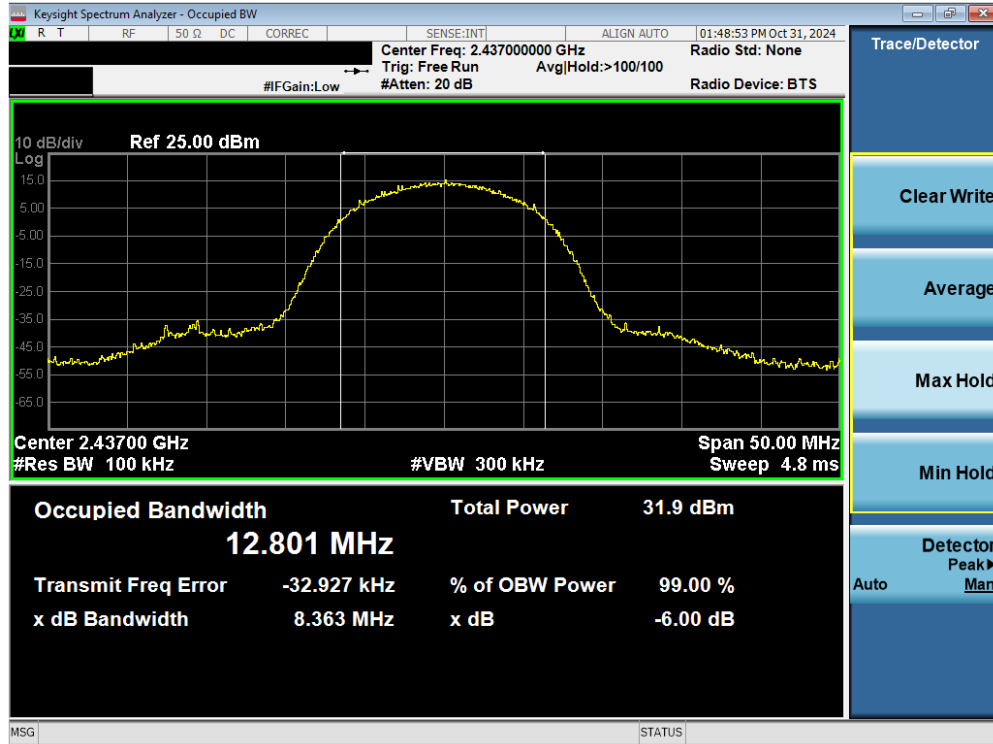
Plot 7-1. 6 dB BW and 99% OBW Plot Antenna 3a (802.11b – Ch. 6)
