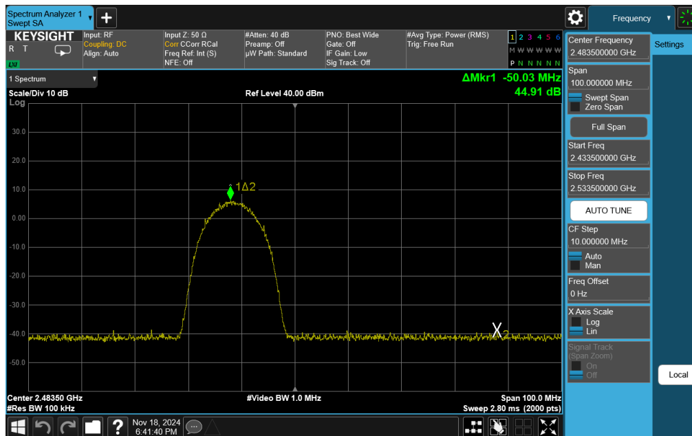
Plot 7-26. Band Edge Plot Antenna 3a (802.11b – Ch. 13)
