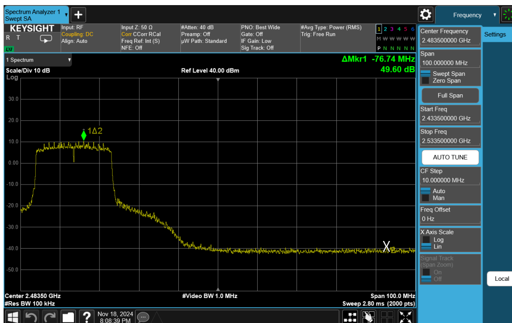
Plot 7-63. Band Edge Plot Antenna 3a (802.11ax (SU - 2.4GHz) – Ch. 8)
