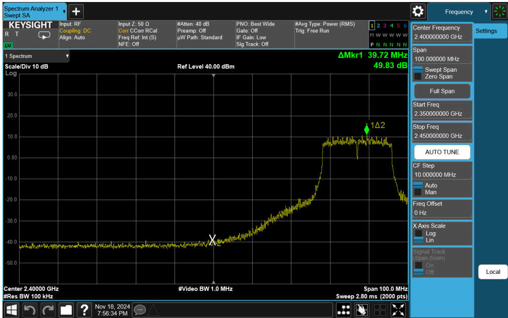
Plot 7-46. Band Edge Plot Antenna 3a (802.11n (2.4GHz) – Ch. 6-Low)
