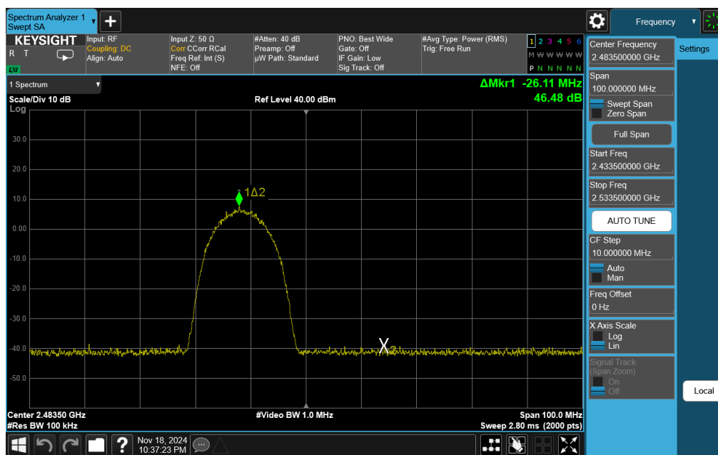
Plot 7-71. Band Edge Plot Antenna 1a (802.11b – Ch. 13)
