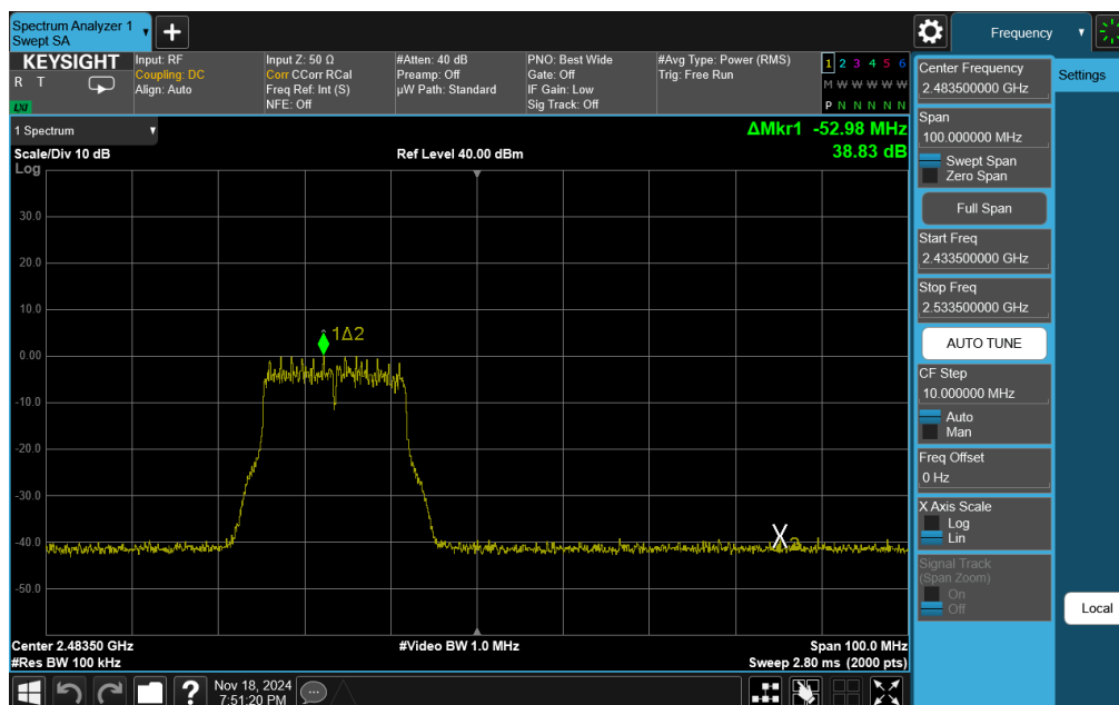
Plot 7-39. Band Edge Plot Antenna 3a (802.11g – Ch. 12)
