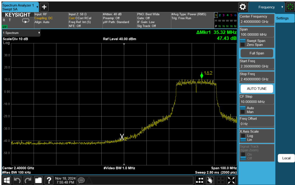
Plot 7-45. Band Edge Plot Antenna 3a (802.11n (2.4GHz) – Ch. 5)
