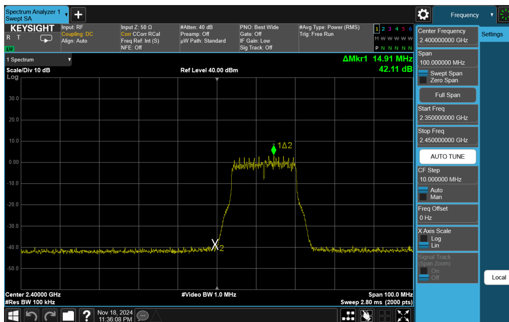
Plot 7-72. Band Edge Plot Antenna 1a (802.11g – Ch. 1)
