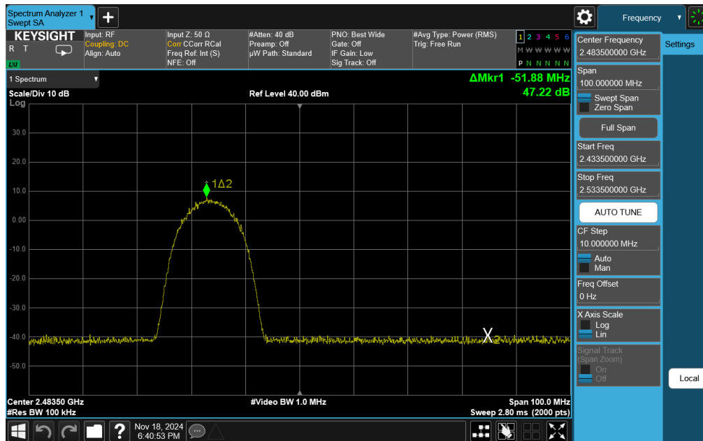
Plot 7-25. Band Edge Plot Antenna 3a (802.11b – Ch. 12)
