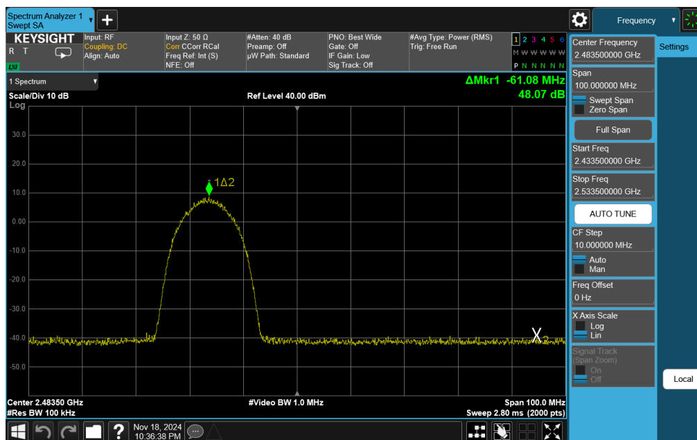
Plot 7-70. Band Edge Plot Antenna 1a (802.11b – Ch. 12)
