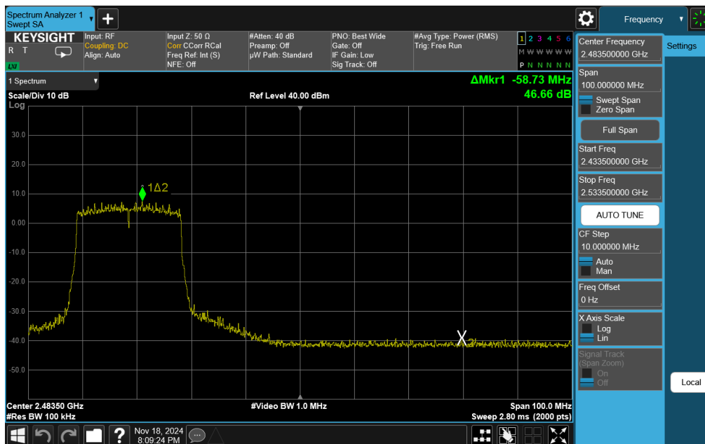
Plot 7-64. Band Edge Plot Antenna 3a (802.11ax (SU - 2.4GHz) – Ch. 9)
