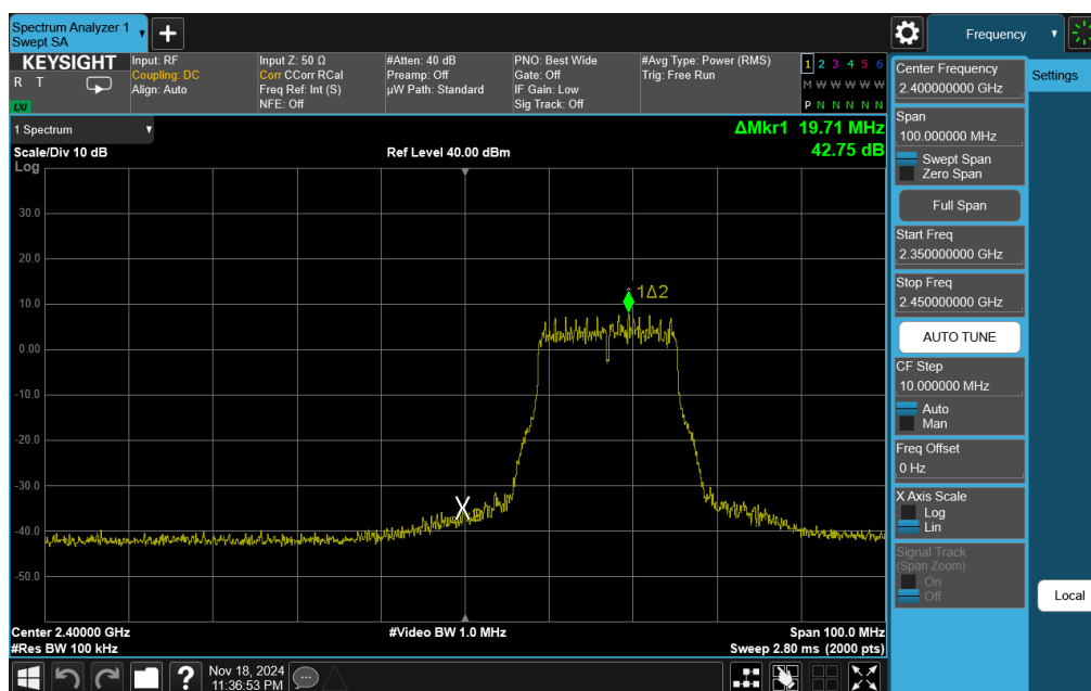
Plot 7-73. Band Edge Plot Antenna 1a (802.11g – Ch. 2)
