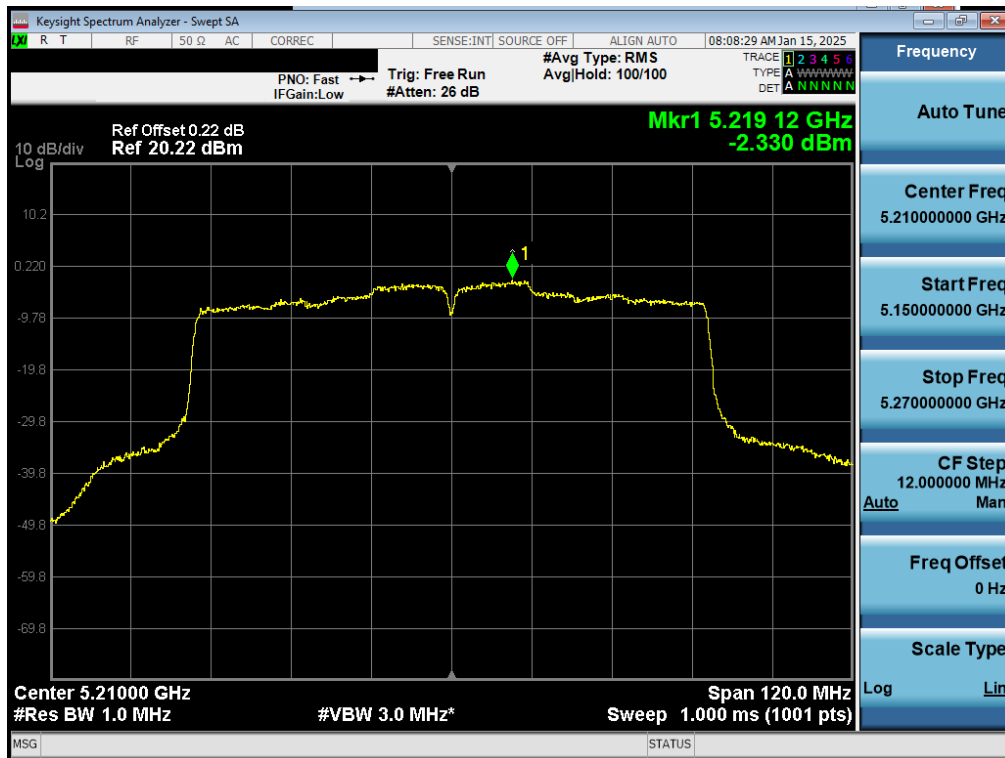
Plot 7-81. ISED PSD SDM Primary Antenna 3a (80MHz BW 11ac – Ch.42)
