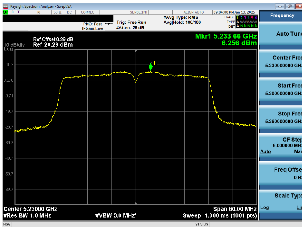
Plot 7-67. PSD CDD Diversity Antenna 1b (40MHz BW 802.11n – Ch. 46)
