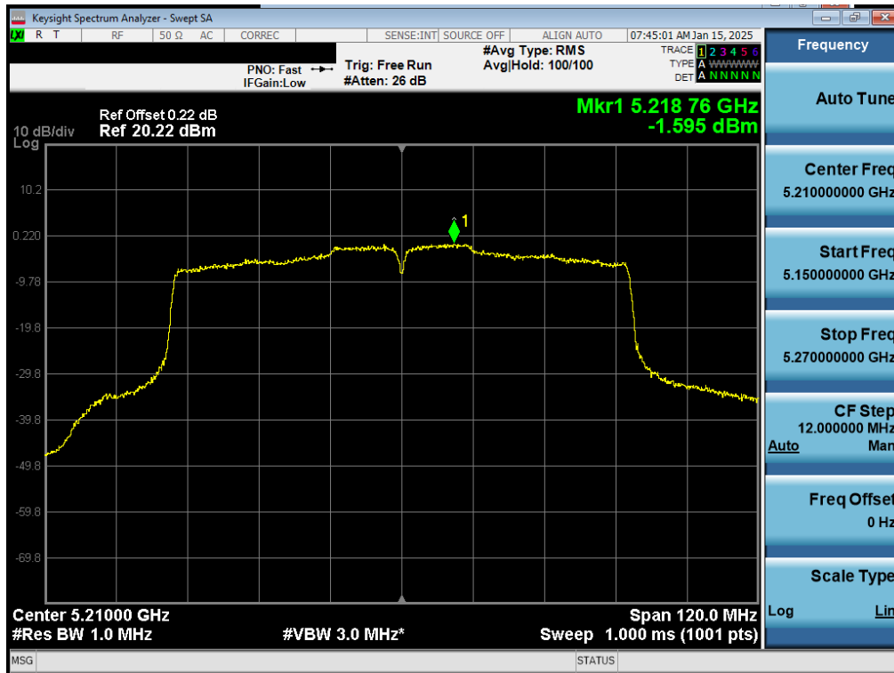
Plot 7-45. ISED PSD Antenna 1b (80MHz BW 11ac – Ch.42)
