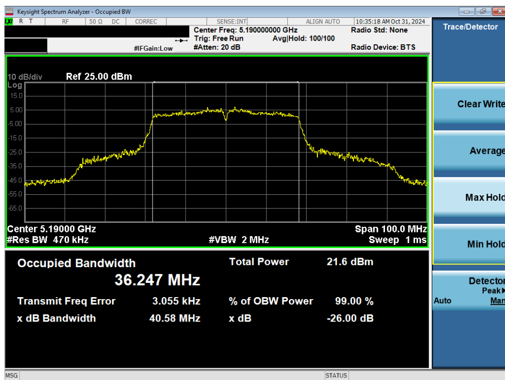
Plot 7-8. 26dB BW & 99% OBW Antenna 1b (40MHz BW 802.11n – Ch. 38)
