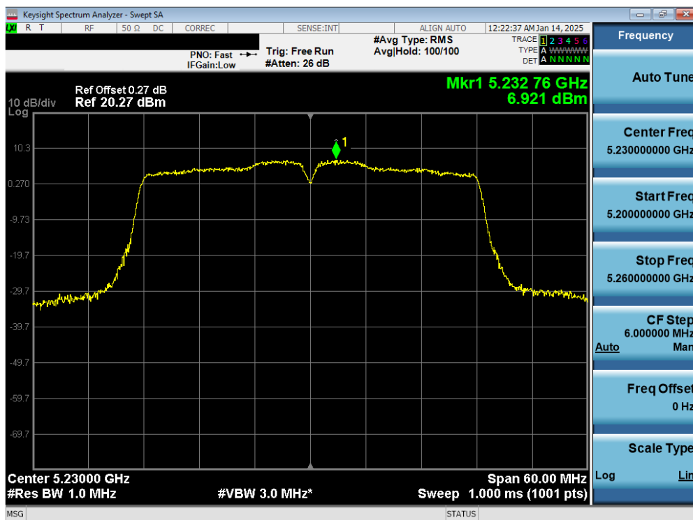
Plot 7-26. ISED PSD Antenna 3c (40MHz BW 11n – Ch.46)
