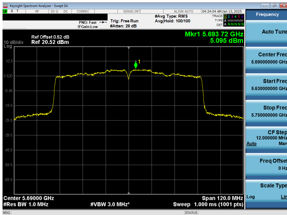
Plot 7-50. PSD CDD Primary Antenna 3c (80MHz BW 802.11ac – Ch. 138)
