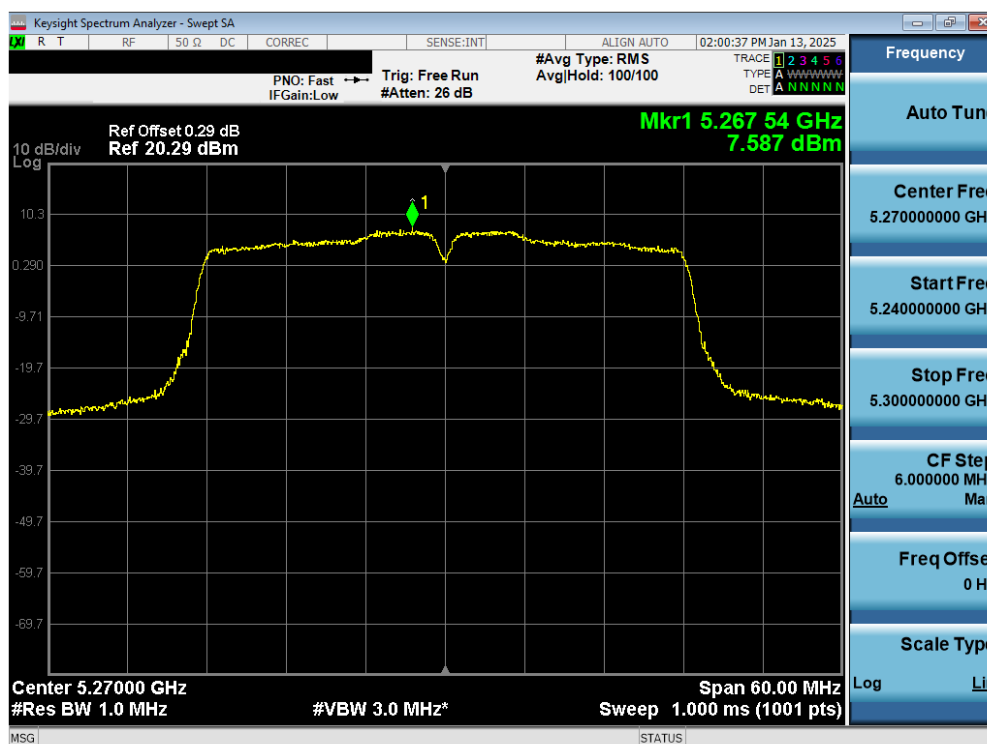
Plot 7-49. PSD CDD Primary Antenna 3a (40MHz BW 802.11n – Ch. 54)
