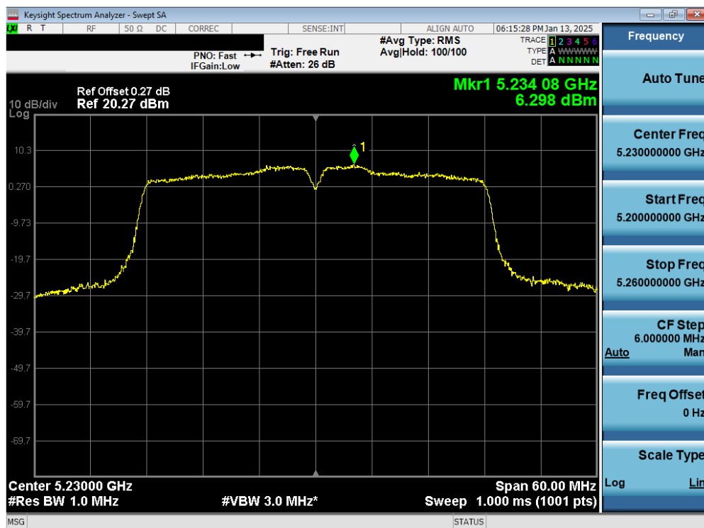
Plot 7-38. PSD Antenna 1b (40MHz BW 802.11n – Ch. 46)
