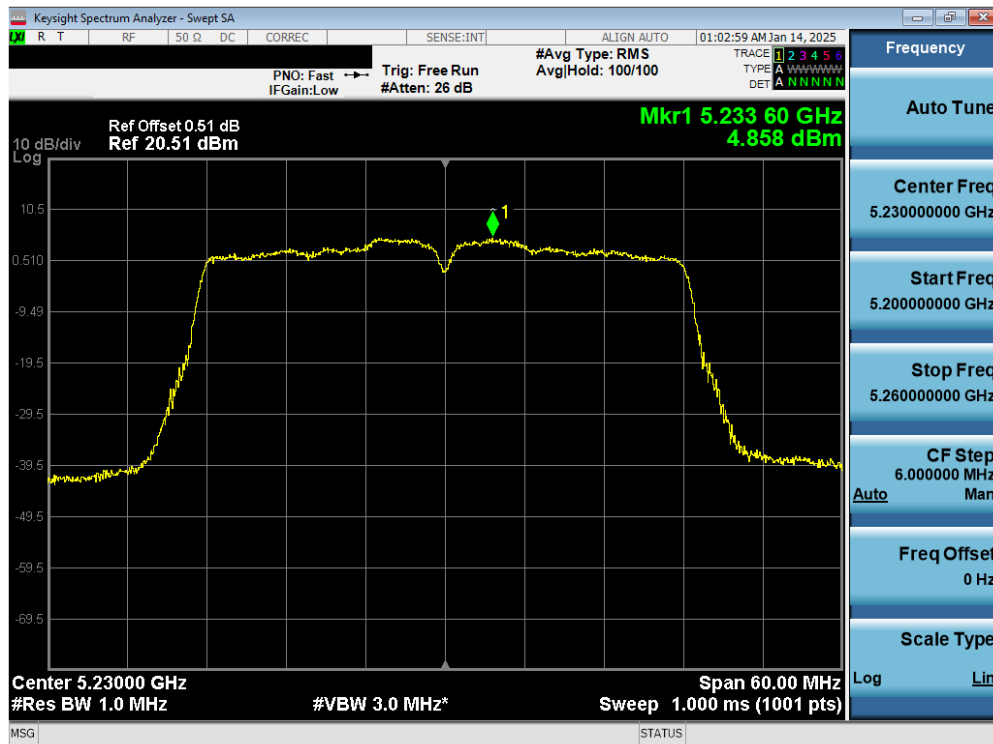
Plot 7-78. ISED PSD SDM Primary Antenna 3c (40MHz BW 11n – Ch.46)
