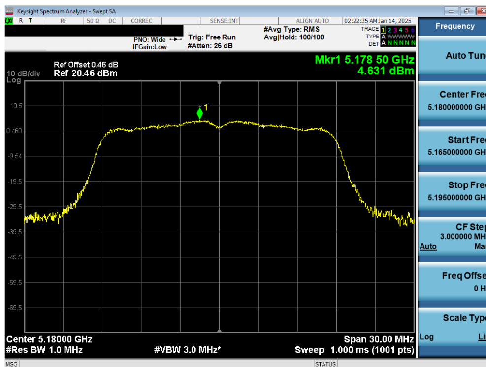
Plot 7-59. ISED PSD SDM Primary Antenna 3a (20MHz BW 11n – Ch.36)
