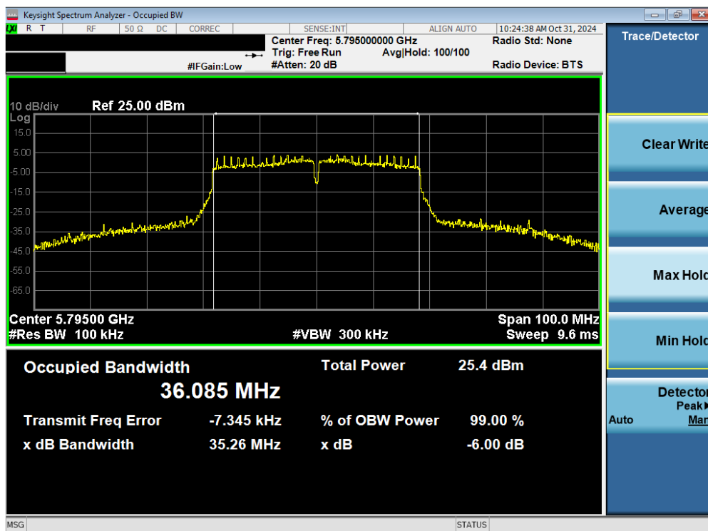
Plot 7-17. 6dB BW & 99% OBW Antenna 1b (40MHz BW 802.11n – Ch. 159)
