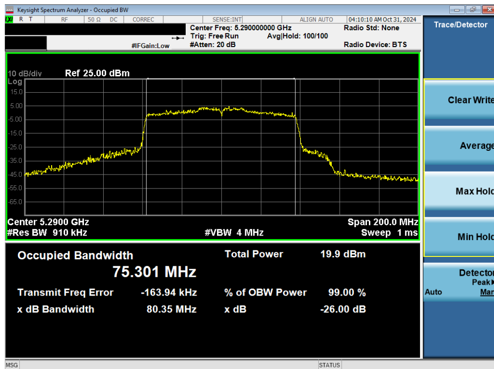
Plot 7-6. 26dB BW & 99% OBW Antenna 3a (80MHz BW 802.11ac – Ch. 58)
