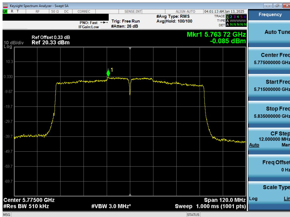
Plot 7-74. PSD CDD Diversity Antenna 3c (80MHz BW 802.11ac – Ch. 155)
