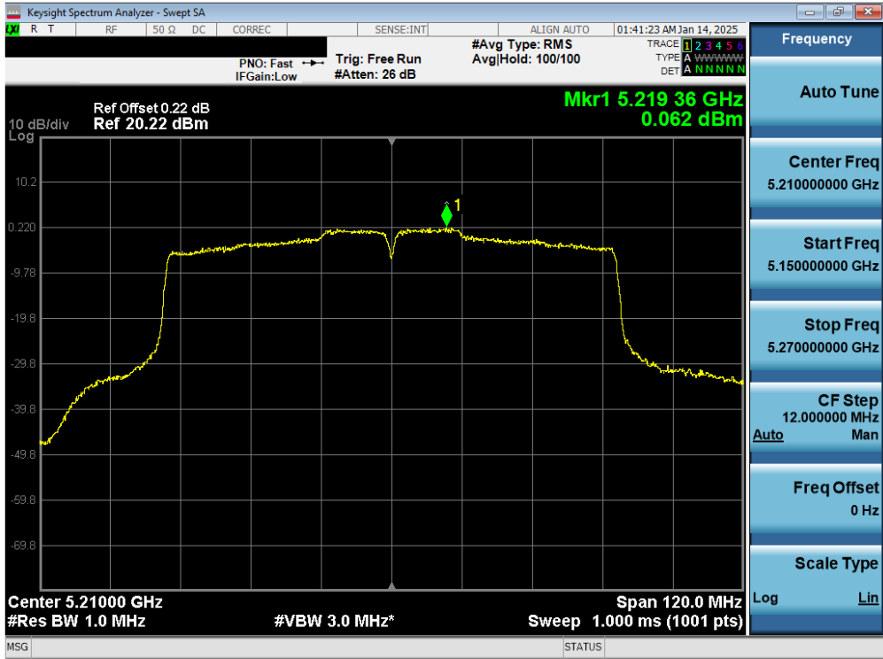
Plot 7-36. ISED PSD Antenna 3a (80MHz BW 11ac – Ch.42)
