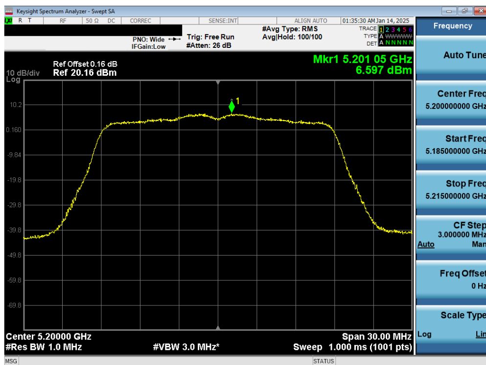
Plot 7-34. ISED PSD Antenna 3a (20MHz BW 11n – Ch.40)
