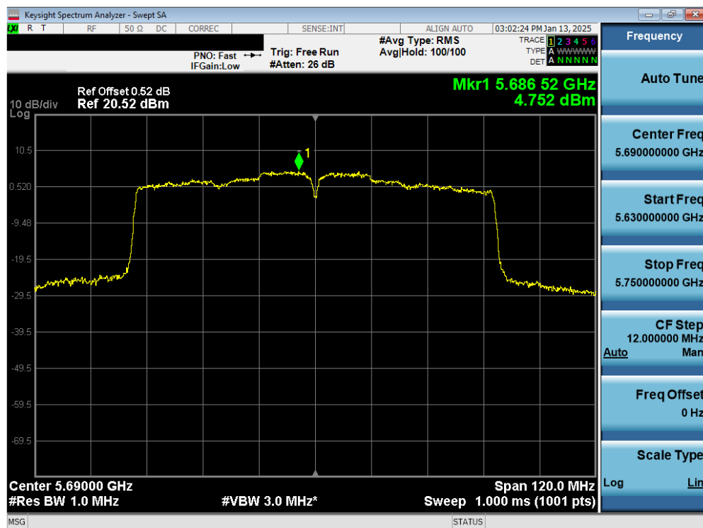
Plot 7-51. PSD CDD Primary Antenna 3a (80MHz BW 802.11ac – Ch. 138)
