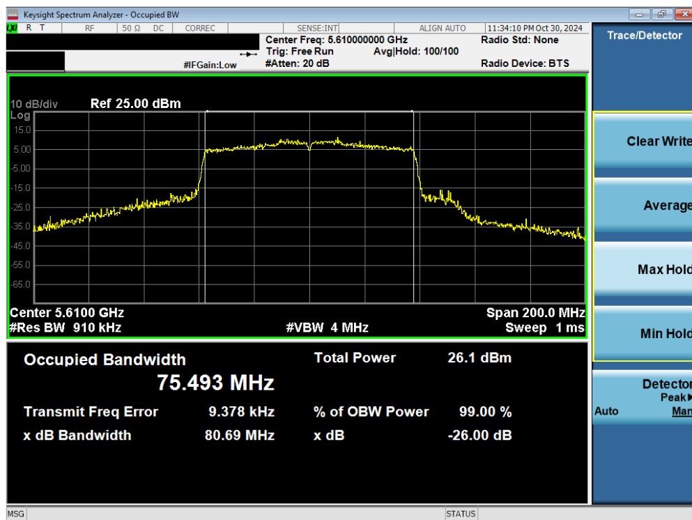
Plot 7-3. 26dB BW & 99% OBW Antenna 3c (80MHz BW 802.11ac – Ch. 122)
