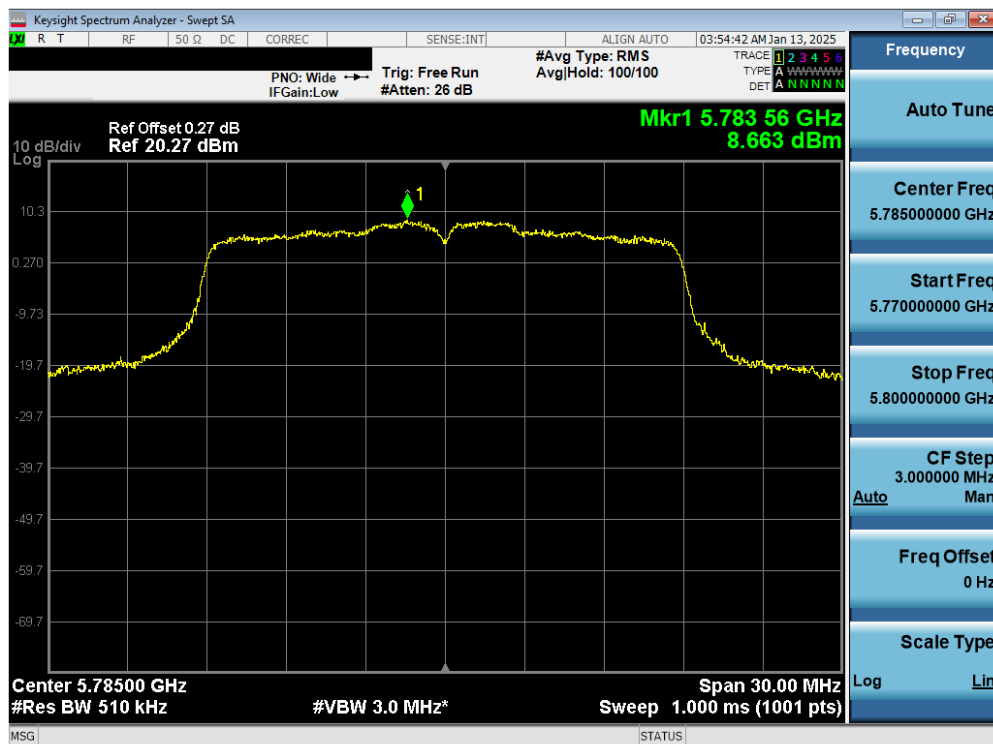
Plot 7-70. PSD CDD Diversity Antenna 3c (20MHz BW 802.11n – Ch. 157)
