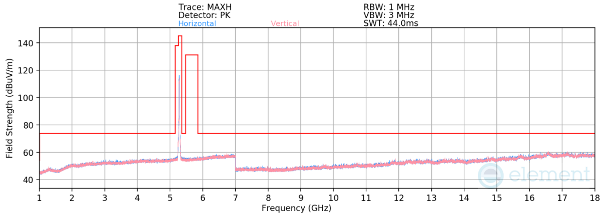
Plot 7-87. Radiated Spurious Emissions above 1GHz CDD Primary (802.11n – Ch. 56)
