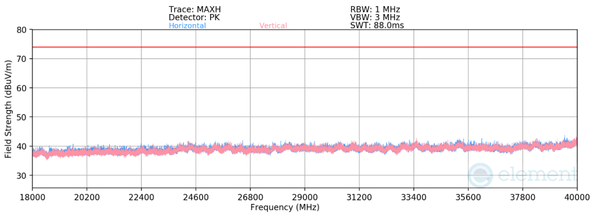
Plot 7-84. Radiated Spurious Emissions above 18GHz CDD Primary (802.11n – Ch. 40)
