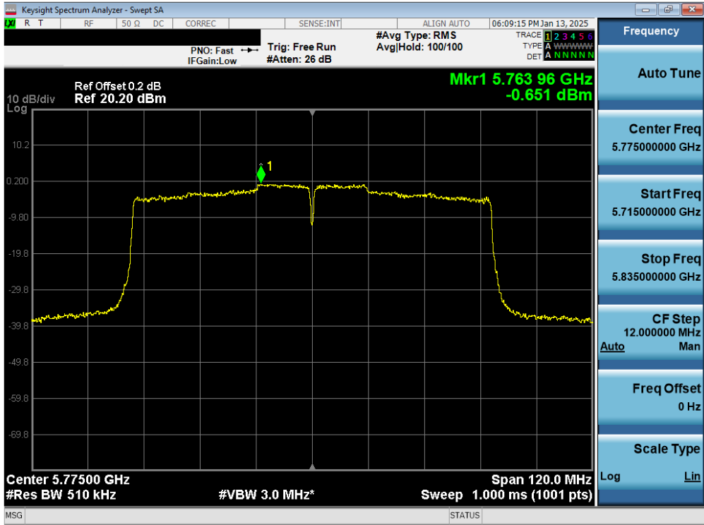
Plot 7-42. PSD Antenna 1b (80MHz BW 802.11ac – Ch. 155)
