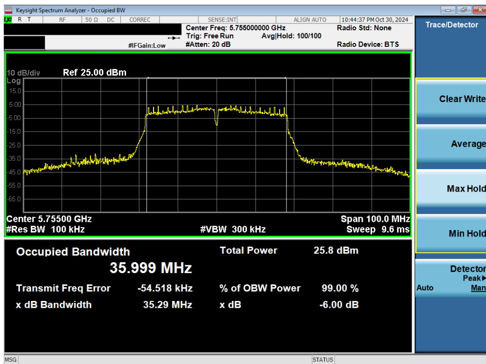
Plot 7-11. 6dB BW & 99% OBW Antenna 3c (40MHz BW 802.11n – Ch. 151)
