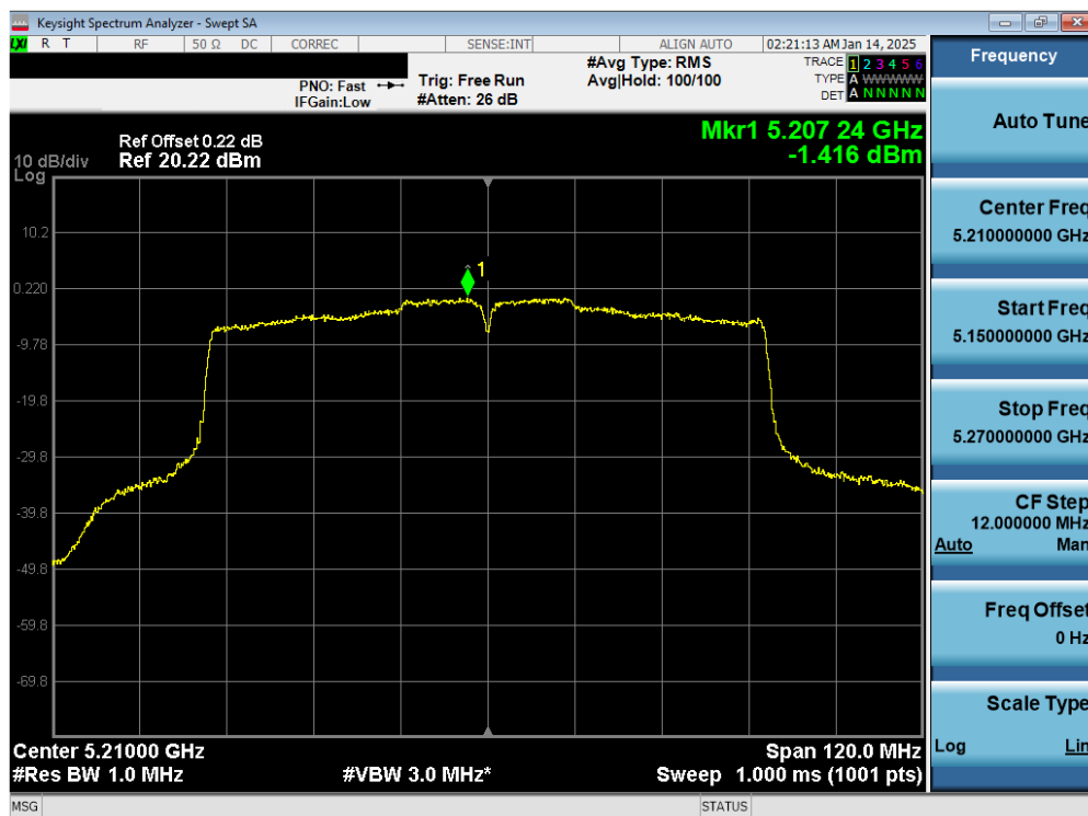
Plot 7-63. ISED PSD SDM Primary Antenna 3a (80MHz BW 11ac – Ch.42)
