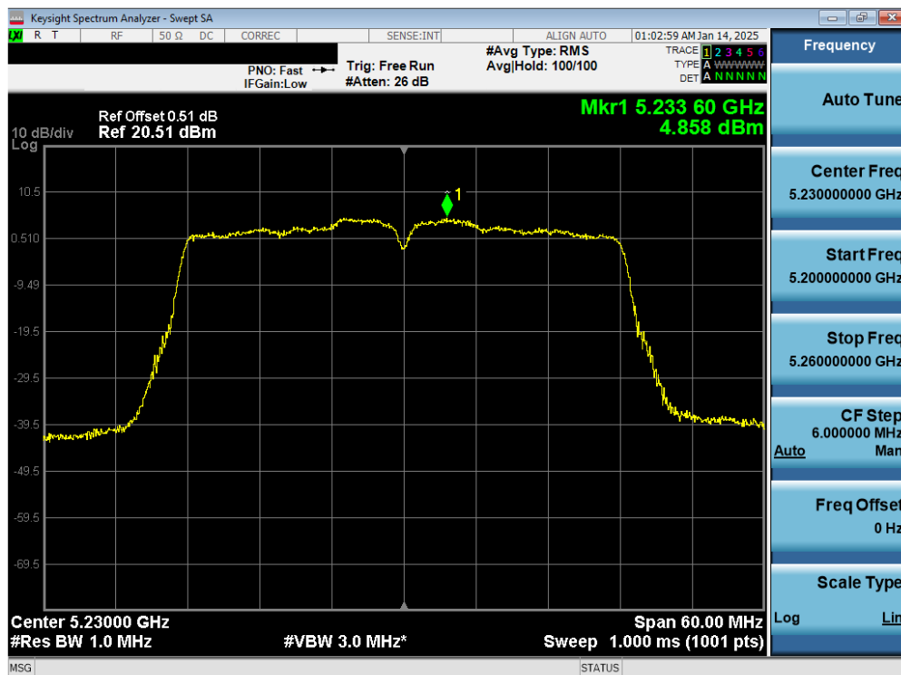
Plot 7-60. ISED PSD SDM Primary Antenna 3c (40MHz BW 11n – Ch.46)
