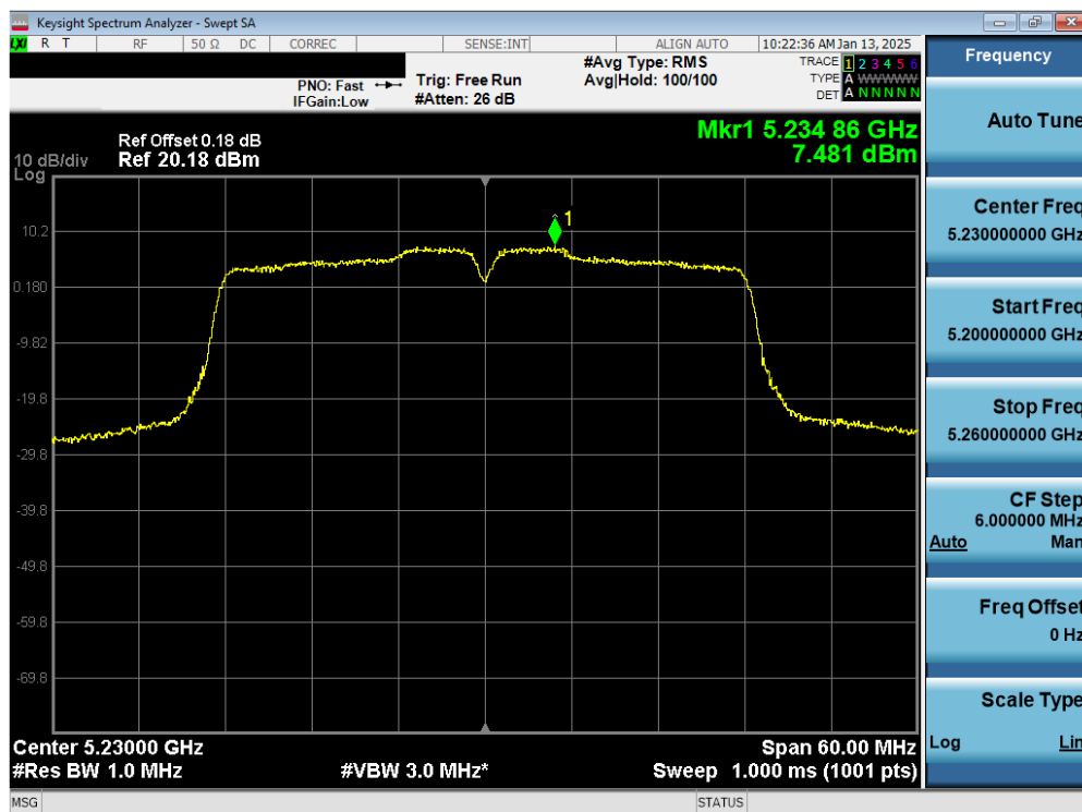
Plot 7-29. PSD Antenna 3a (40MHz BW 802.11n – Ch. 46)
