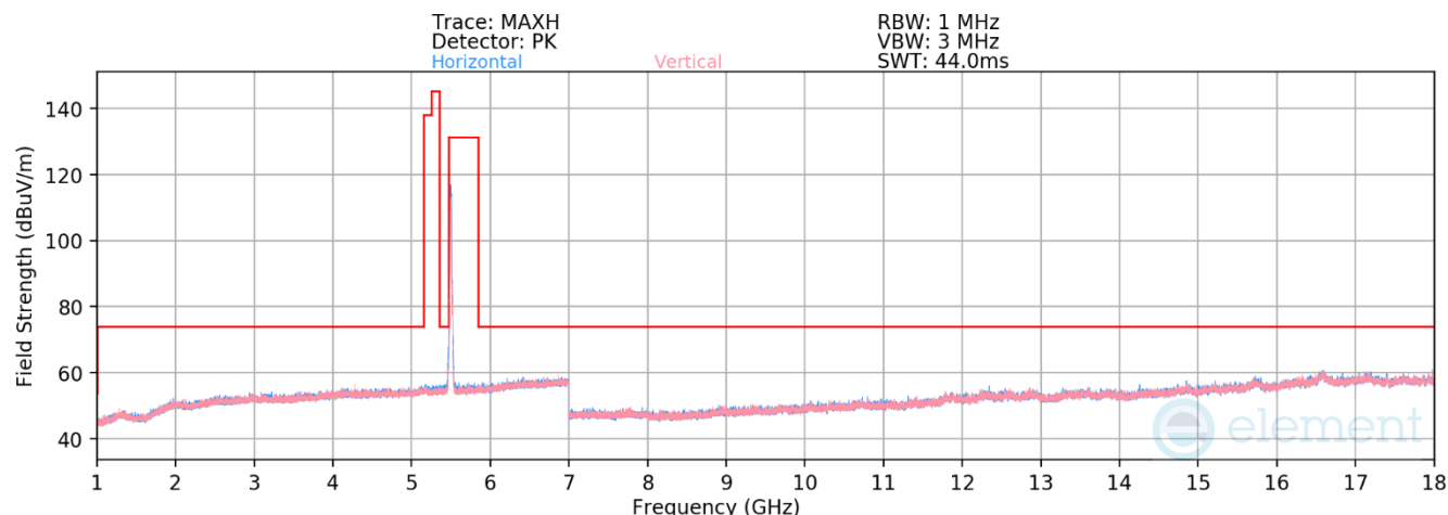
Plot 7-90. Radiated Spurious Emissions above 1GHz CDD Primary (802.11n – Ch. 100)
