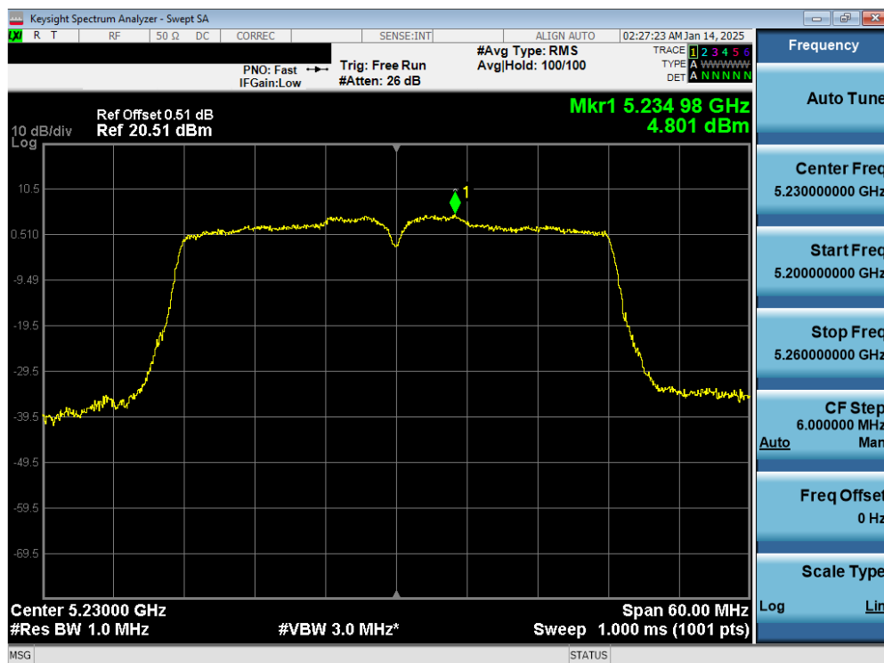
Plot 7-61. ISED PSD SDM Primary Antenna 3a (40MHz BW 11n – Ch.46)
