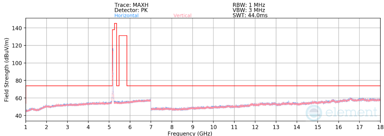
Plot 7-82. Radiated Spurious Emissions above 1GHz CDD Primary (802.11n – Ch. 36)
