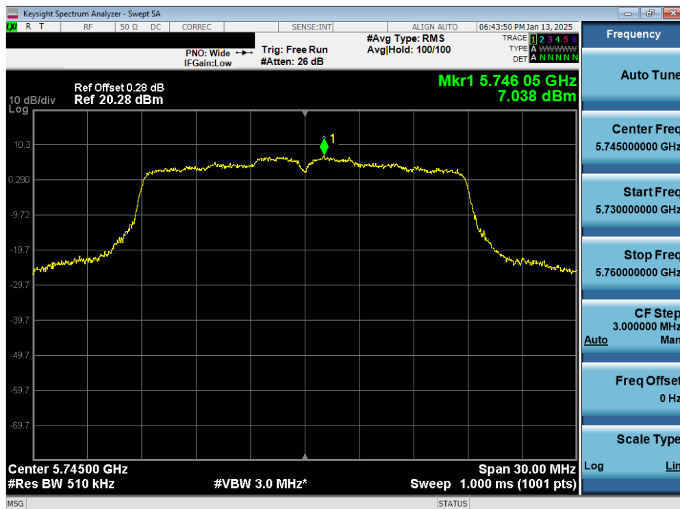
Plot 7-40. PSD Antenna 1b (20MHz BW 802.11n – Ch. 149)
