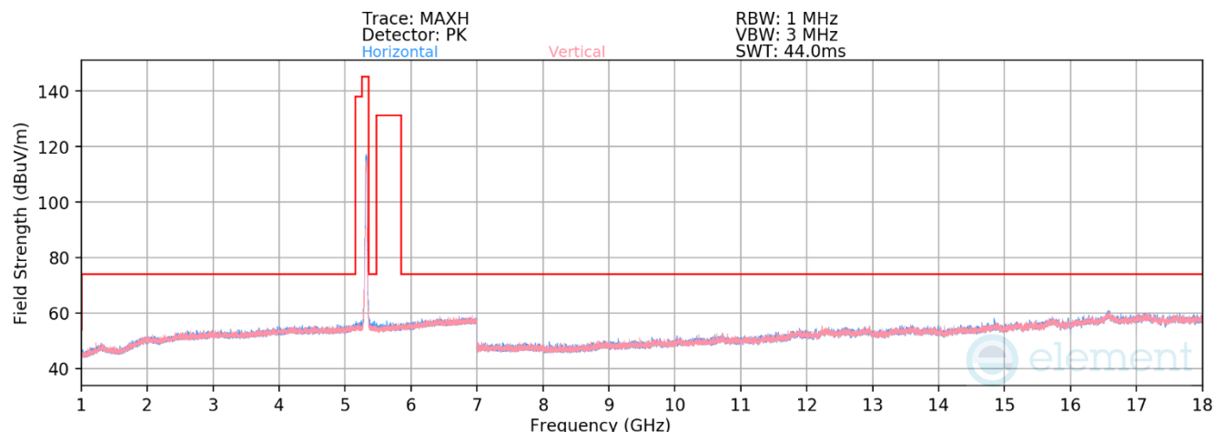
Plot 7-89. Radiated Spurious Emissions above 1GHz CDD Primary (802.11n – Ch. 64)
