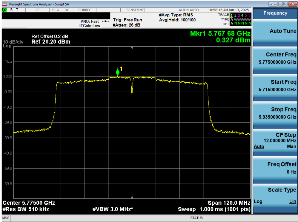
Plot 7-33. PSD Antenna 3a (80MHz BW 802.11ac – Ch. 155)
