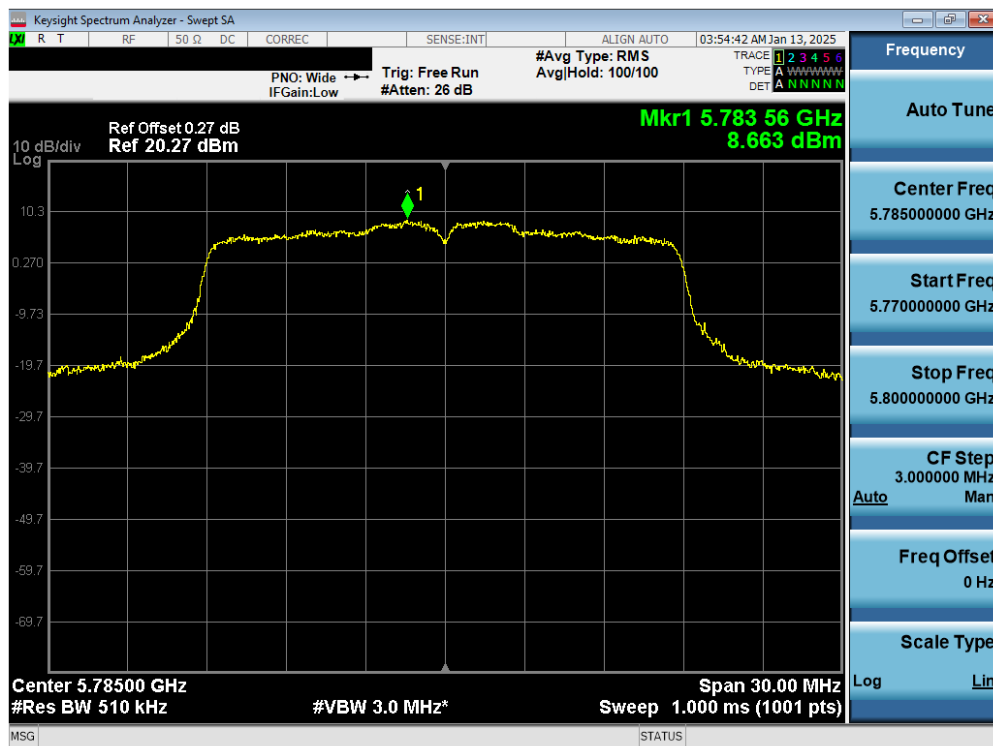
Plot 7-52. PSD CDD Primary Antenna 3c (20MHz BW 802.11n – Ch. 157)
