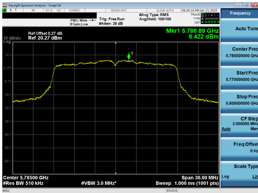
Plot 7-71. PSD CDD Diversity Antenna 1b (20MHz BW 802.11n – Ch. 157)
