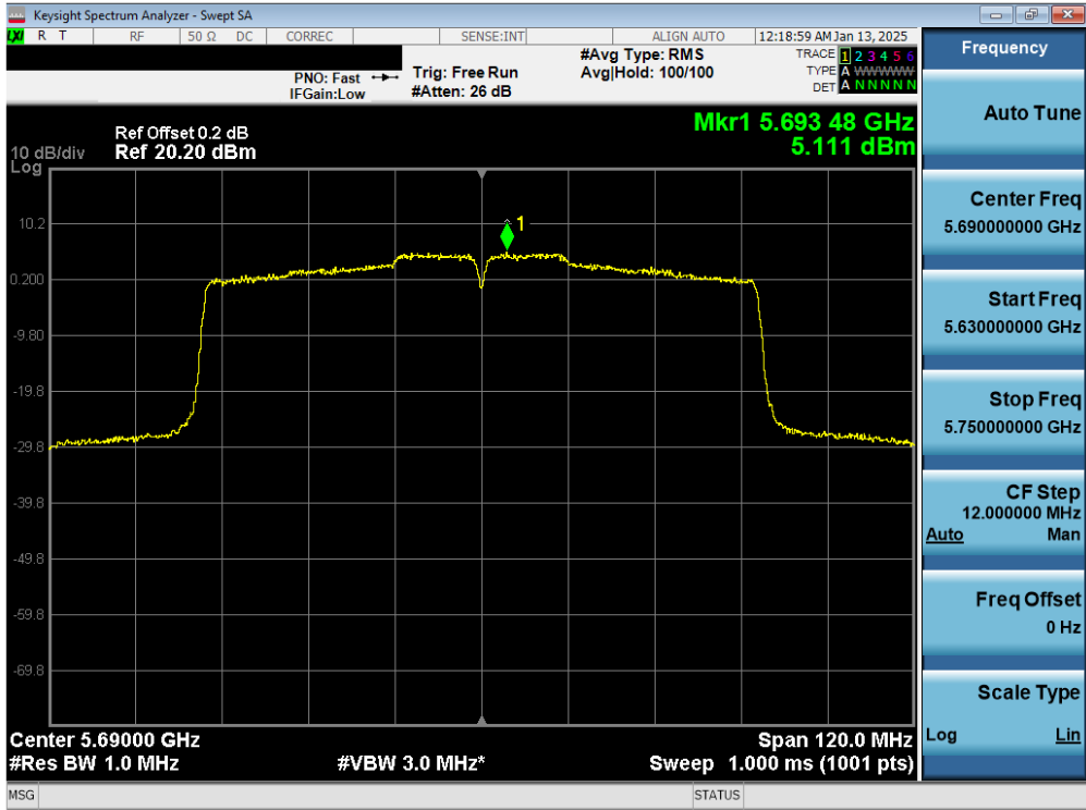
Plot 7-21. PSD Antenna 3c (80MHz BW 802.11ac – Ch. 138)
