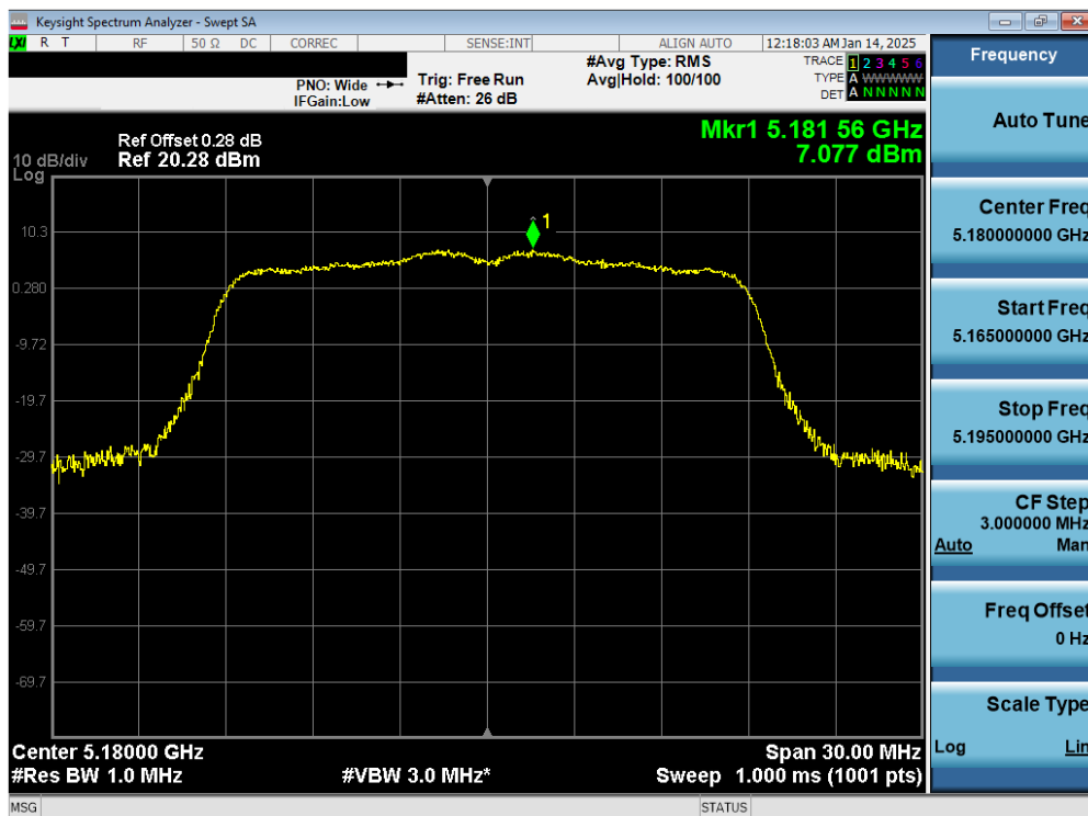
Plot 7-25. ISED PSD Antenna 3c (20MHz BW 11n – Ch.36)
