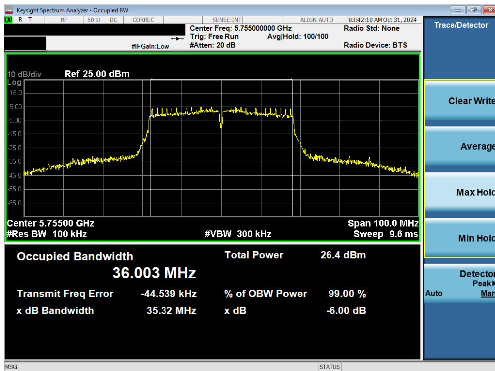
Plot 7-14. 6dB BW & 99% OBW Antenna 3a (40MHz BW 802.11n – Ch. 151)
