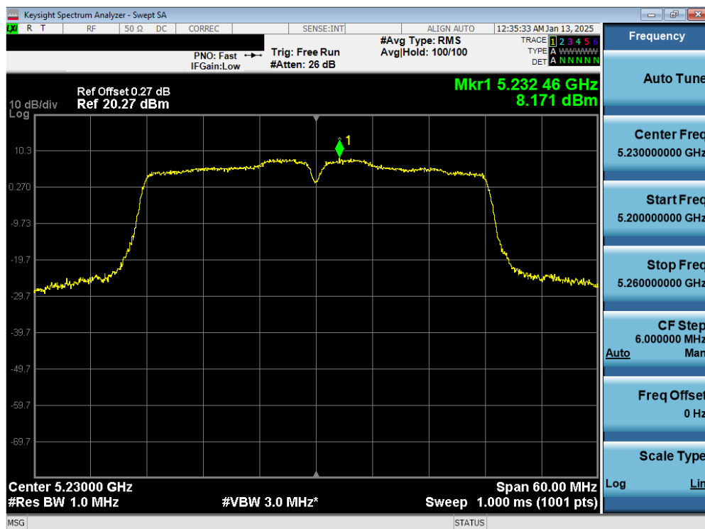
Plot 7-20. PSD Antenna 3c (40MHz BW 802.11n – Ch. 46)
