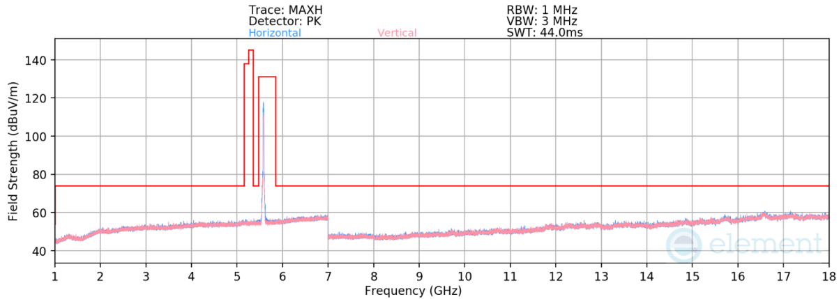
Plot 7-91. Radiated Spurious Emissions above 1GHz CDD Primary (802.11n – Ch. 116)
