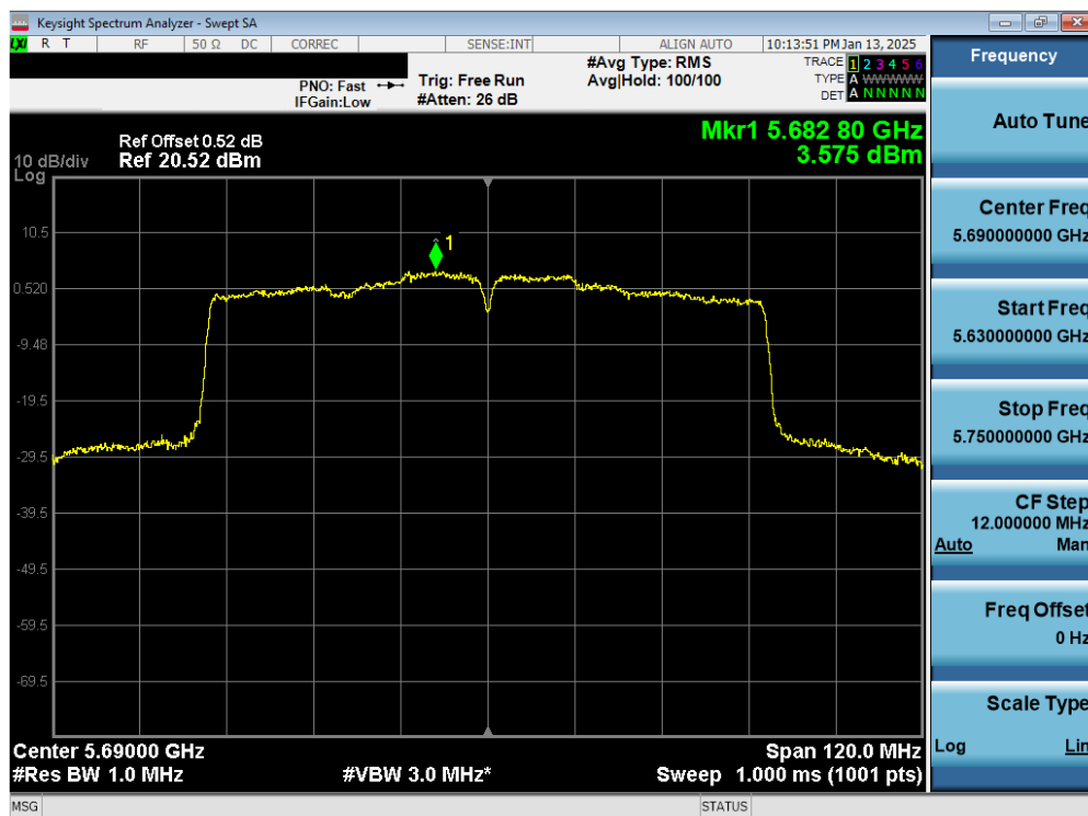
Plot 7-69. PSD CDD Diversity Antenna 1b (80MHz BW 802.11ac – Ch. 138)
