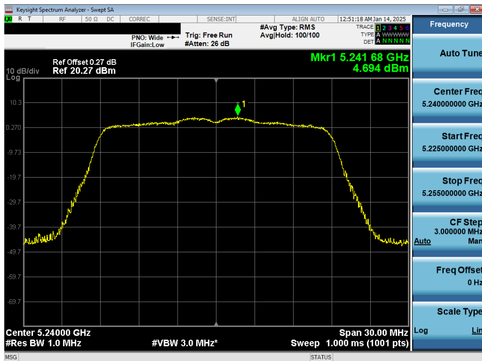
Plot 7-76. ISED PSD SDM Diversity Antenna 3c (20MHz BW 11n – Ch.48)
