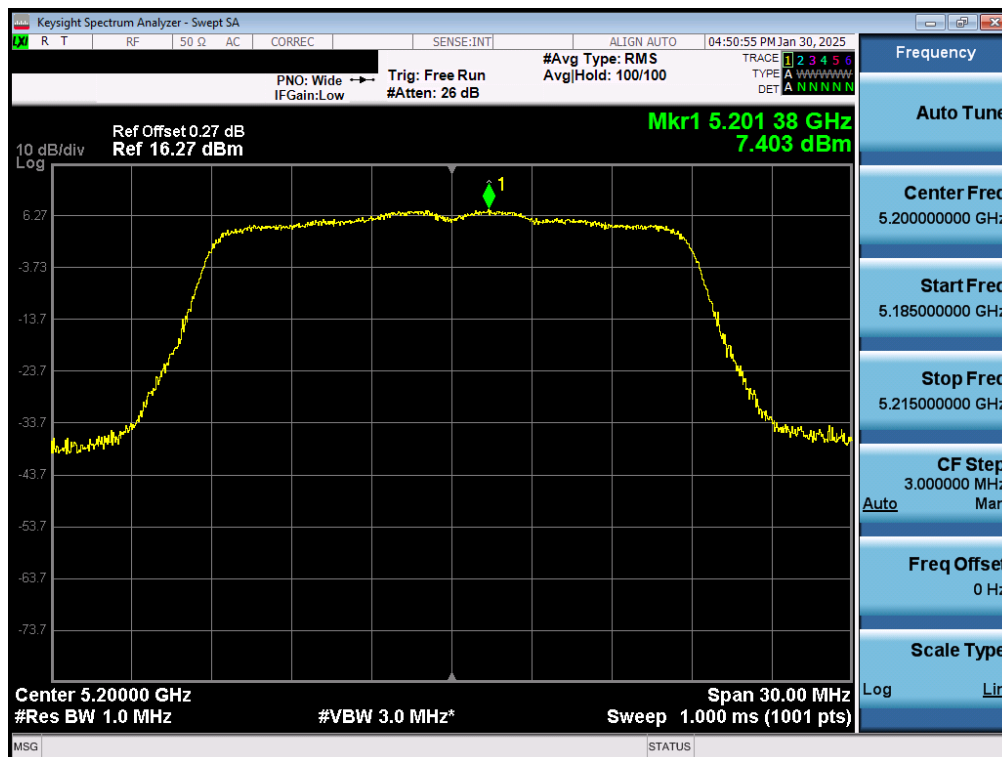
Plot 7-47. PSD CDD Primary Antenna 3a (20MHz BW 802.11n – Ch. 40)
