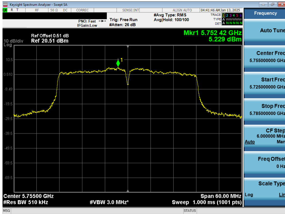
Plot 7-54. PSD CDD Primary Antenna 3c (40MHz BW 802.11n – Ch. 151)
