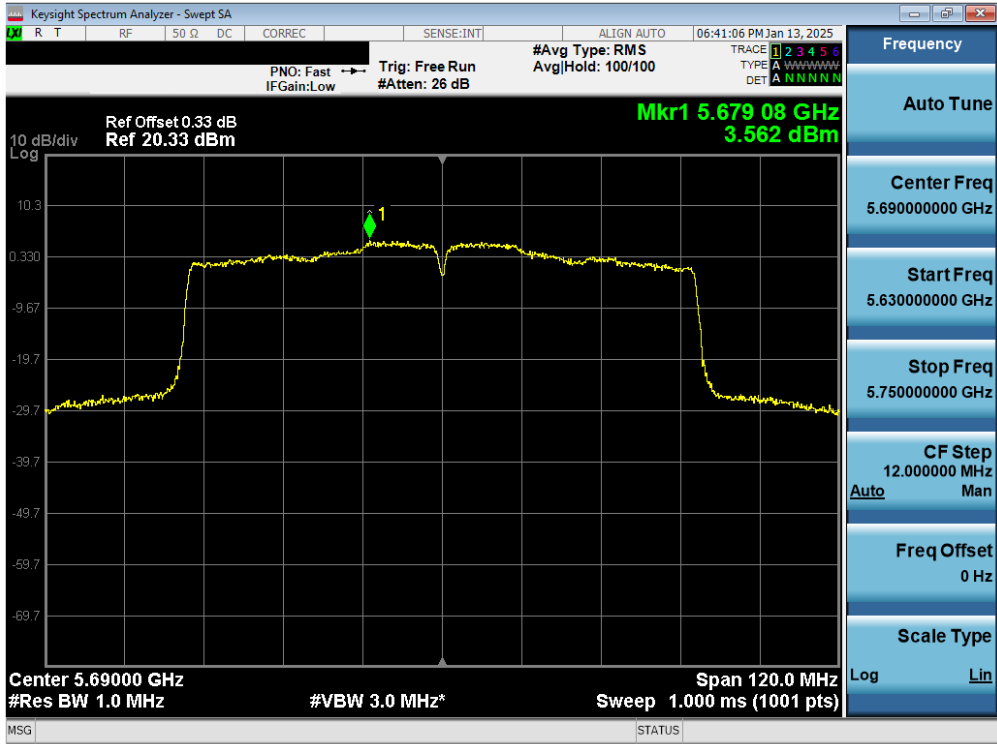
Plot 7-39. PSD Antenna 1b (80MHz BW 802.11ac – Ch. 138)
