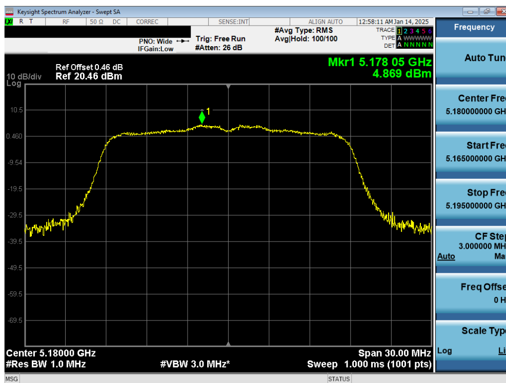
Plot 7-58. ISED PSD SDM Primary Antenna 3c (20MHz BW 11n – Ch.36)
