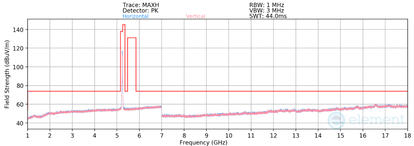
Plot 7-85. Radiated Spurious Emissions above 1GHz CDD Primary (802.11n – Ch. 48)
