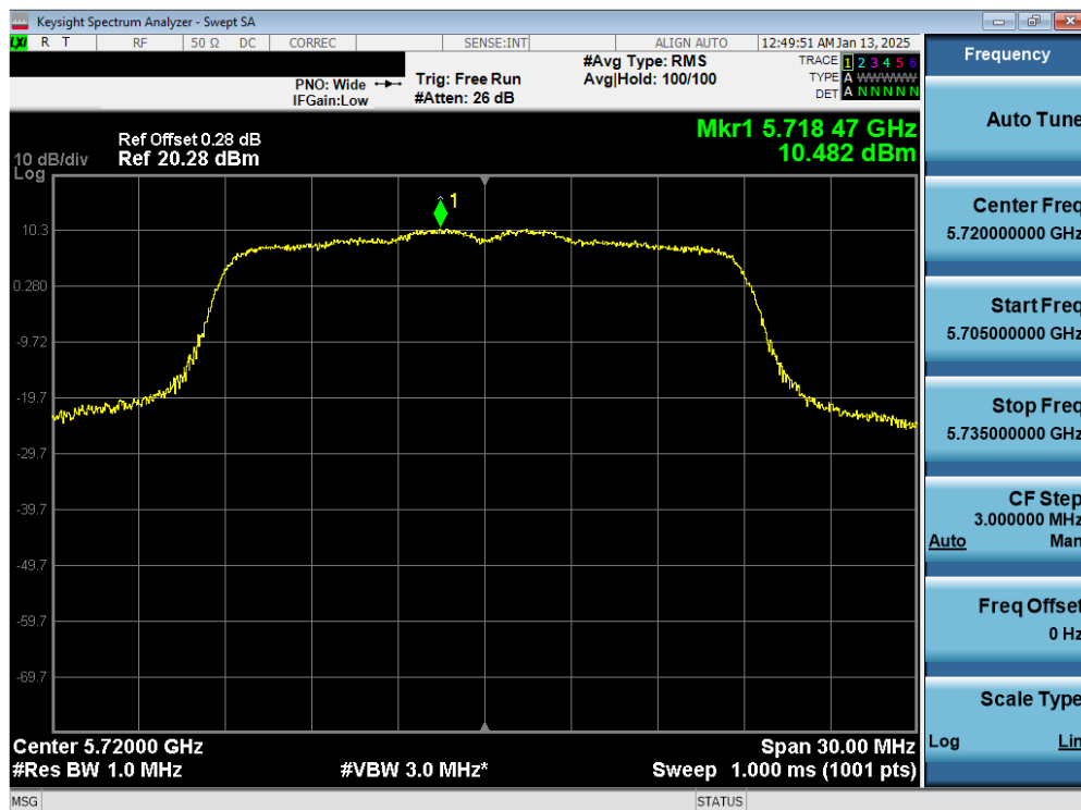
Plot 7-19. PSD Antenna 3c (20MHz BW 802.11n – Ch.144)
