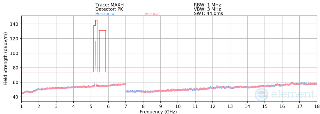
Plot 7-86. Radiated Spurious Emissions above 1GHz CDD Primary (802.11n – Ch. 52)
