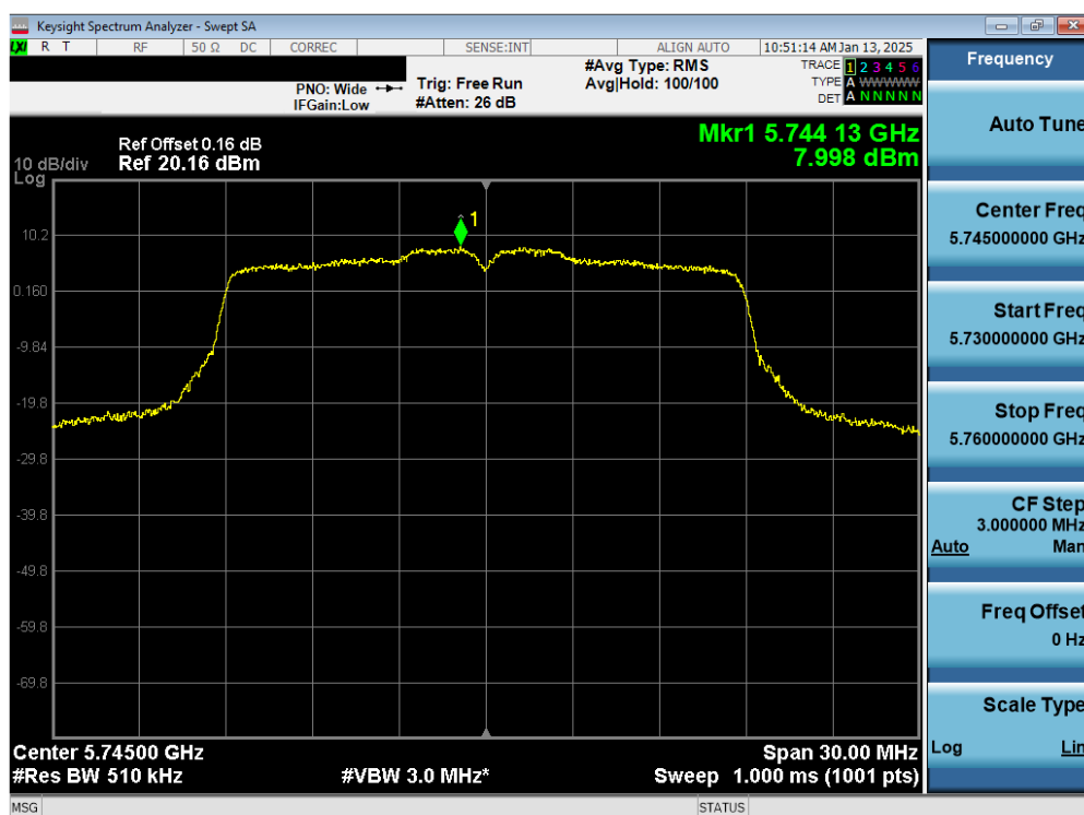
Plot 7-31. PSD Antenna 3a (20MHz BW 802.11n – Ch. 149)
