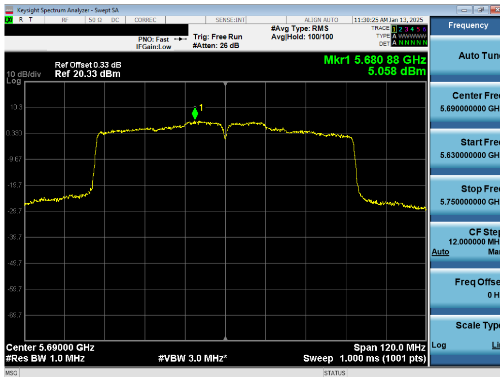
Plot 7-30. PSD Antenna 3a (80MHz BW 802.11ac – Ch. 138)
