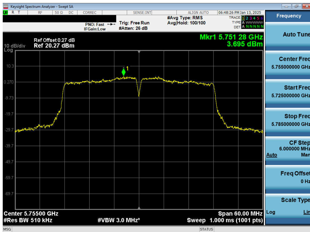
Plot 7-41. PSD Antenna 1b (40MHz BW 802.11n – Ch. 151)
