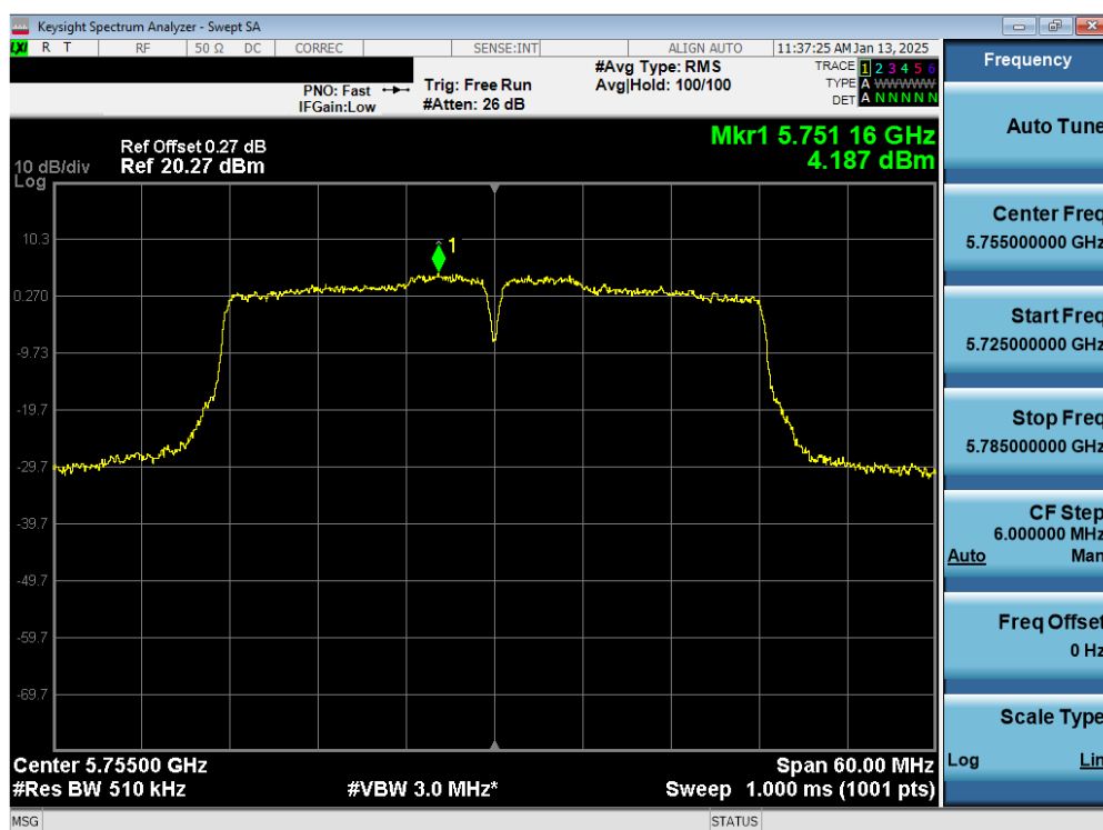
Plot 7-32. PSD Antenna 3a (40MHz BW 802.11n – Ch. 151)
