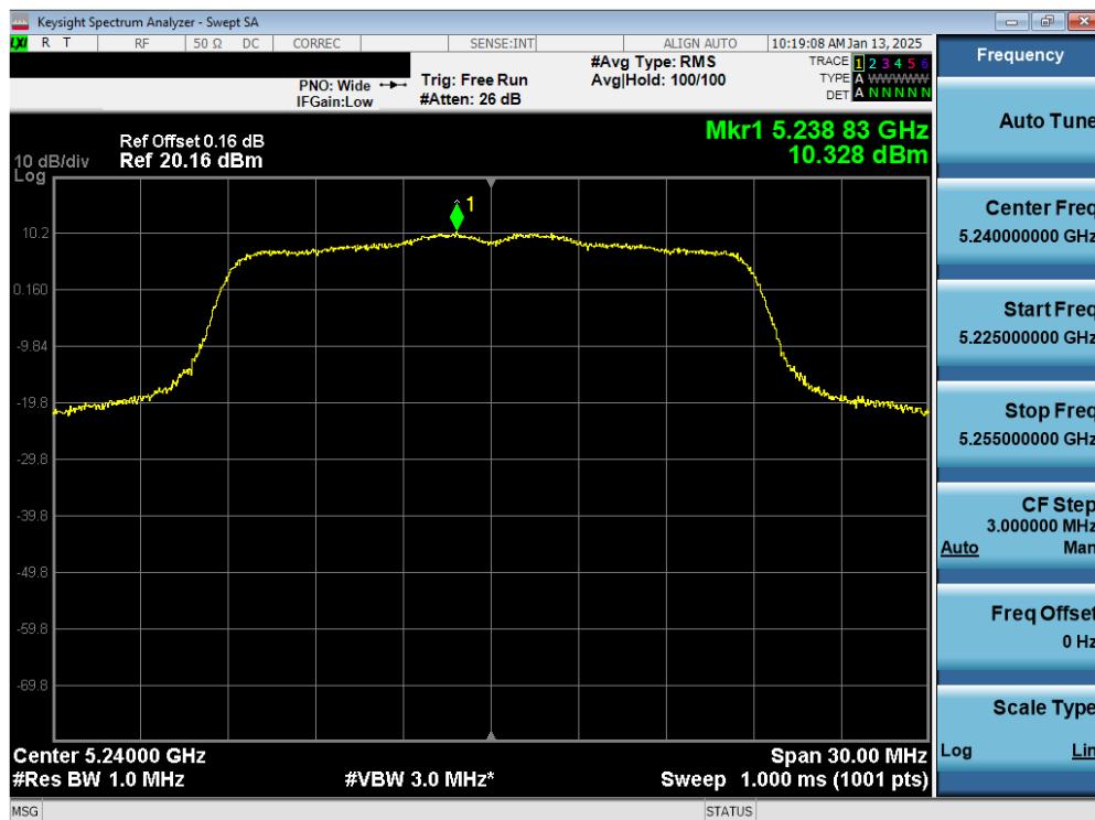
Plot 7-28. PSD Antenna 3a (20MHz BW 802.11n – Ch.48)
