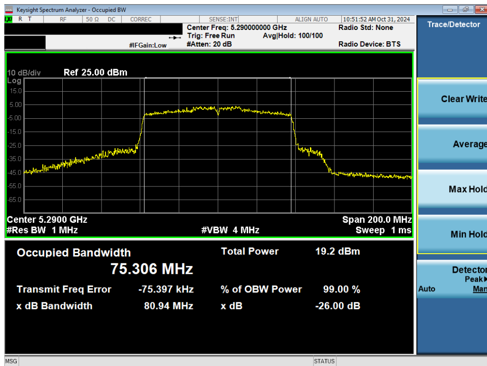
Plot 7-9. 26dB BW & 99% OBW Antenna 1b (80MHz BW 802.11ac – Ch. 58)
