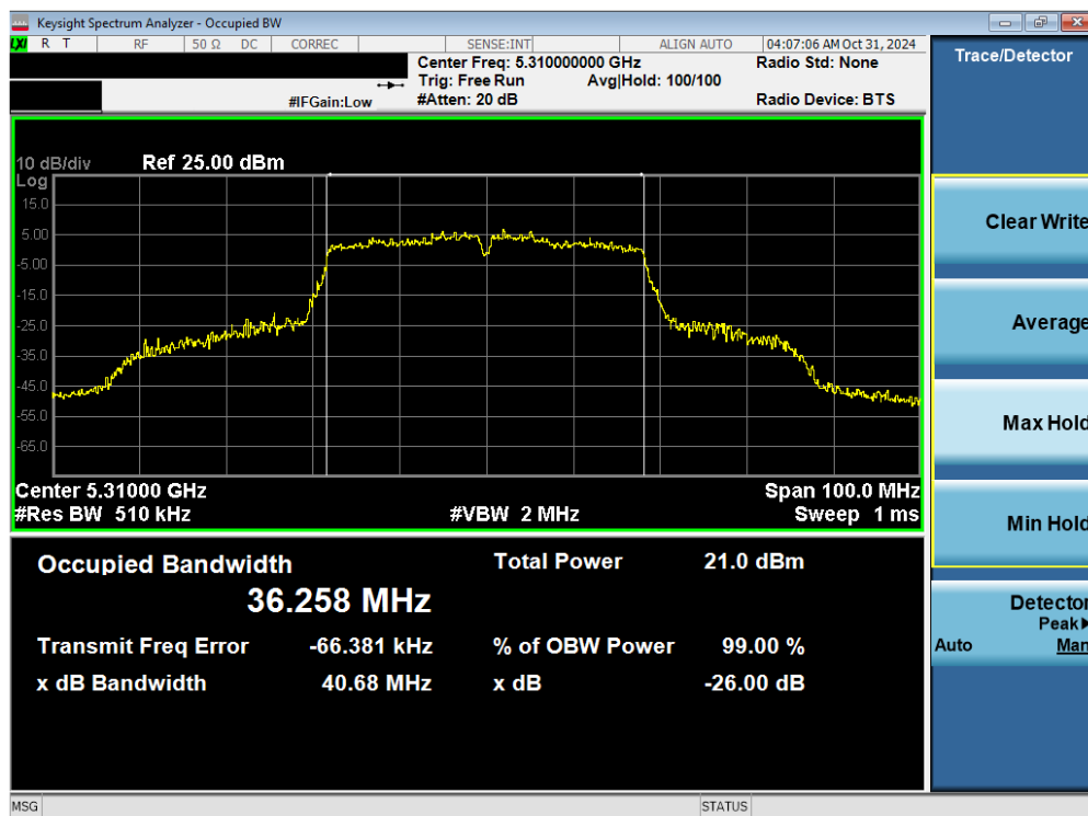
Plot 7-5. 26dB BW & 99% OBW Antenna 3a (40MHz BW 802.11n – Ch. 62)
