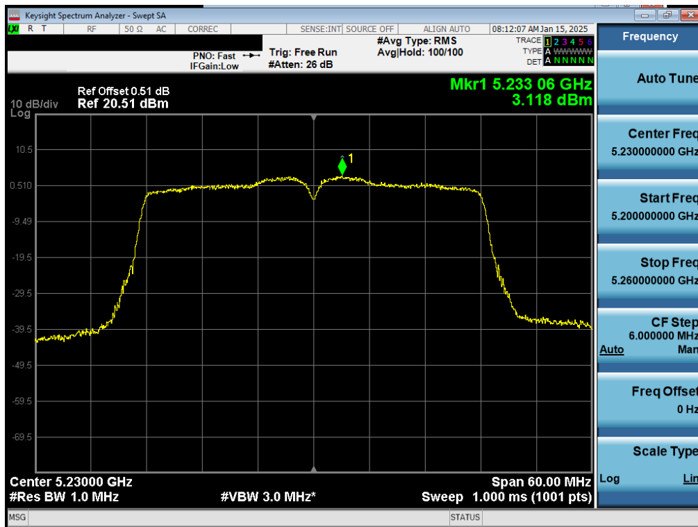
Plot 7-79. ISED PSD SDM Primary Antenna 3a (40MHz BW 11n – Ch.46)
