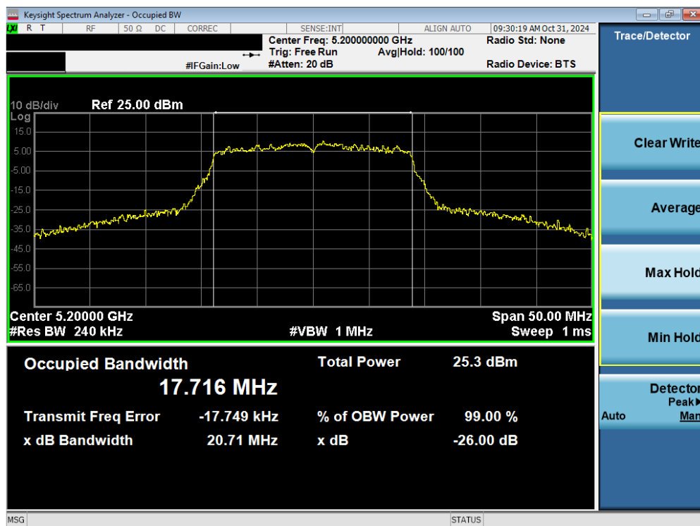
Plot 7-7. 26dB BW & 99% OBW Antenna 1b (20MHz BW 802.11n – Ch. 40)
