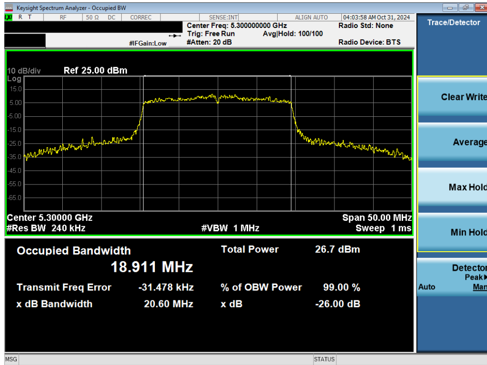
Plot 7-4. 26dB BW & 99% OBW Antenna 3a (20MHz BW 802.11ax (SU) – Ch. 60)
