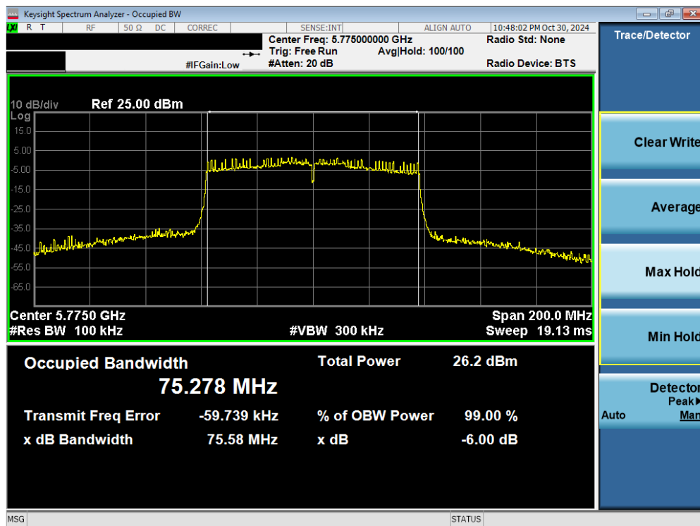
Plot 7-12. 6dB BW & 99% OBW Antenna 3c (80MHz BW 802.11ac – Ch. 155)
