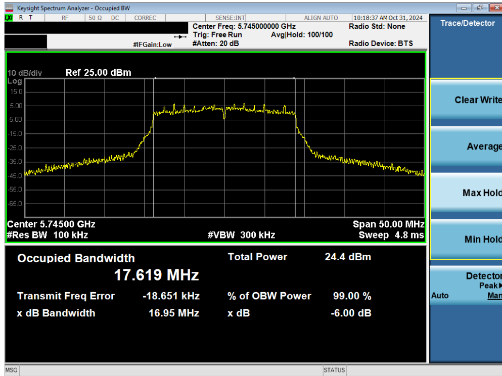
Plot 7-16. 6dB BW & 99% OBW Antenna 1b (20MHz BW 802.11n – Ch. 149)
