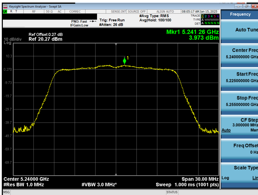
Plot 7-77. ISED PSD SDM Diversity Antenna 1b (20MHz BW 11n – Ch.48)
