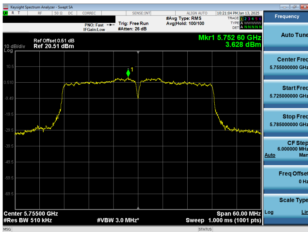
Plot 7-73. PSD CDD Diversity Antenna 1b (40MHz BW 802.11n – Ch. 151)
