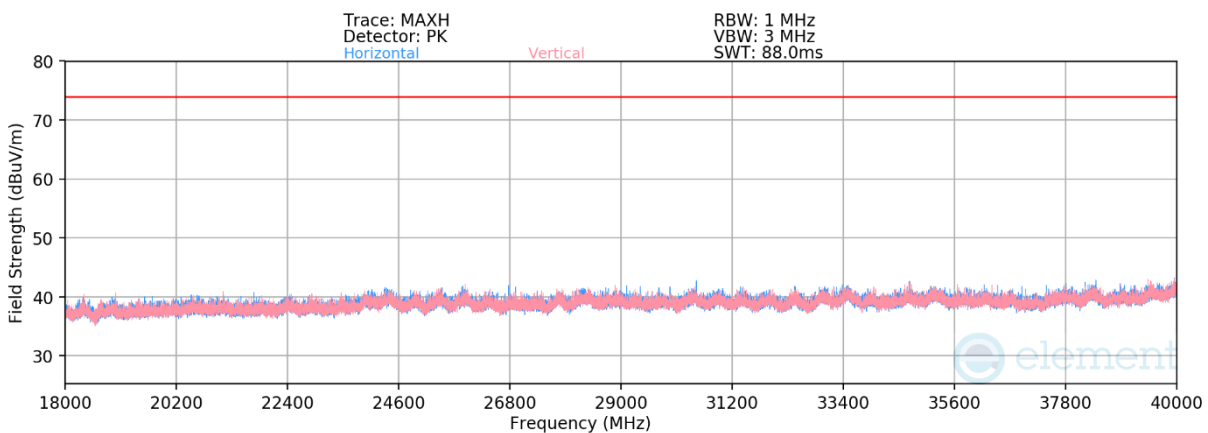
Plot 7-92. Radiated Spurious Emissions above 18GHz CDD Primary (802.11n – Ch. 116)
