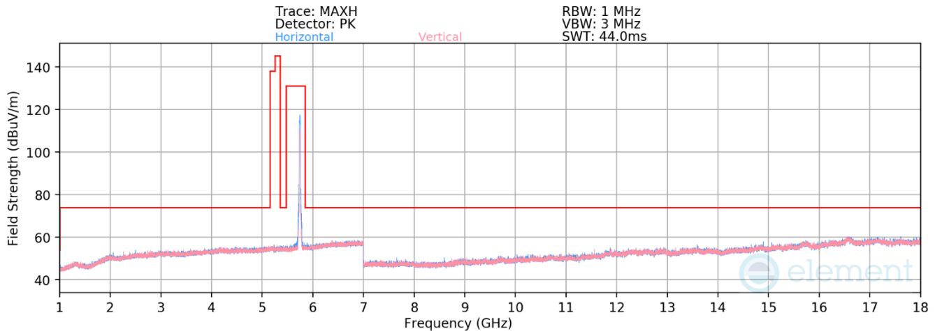
Plot 7-94. Radiated Spurious Emissions above 1GHz CDD Primary (802.11n – Ch. 149)
