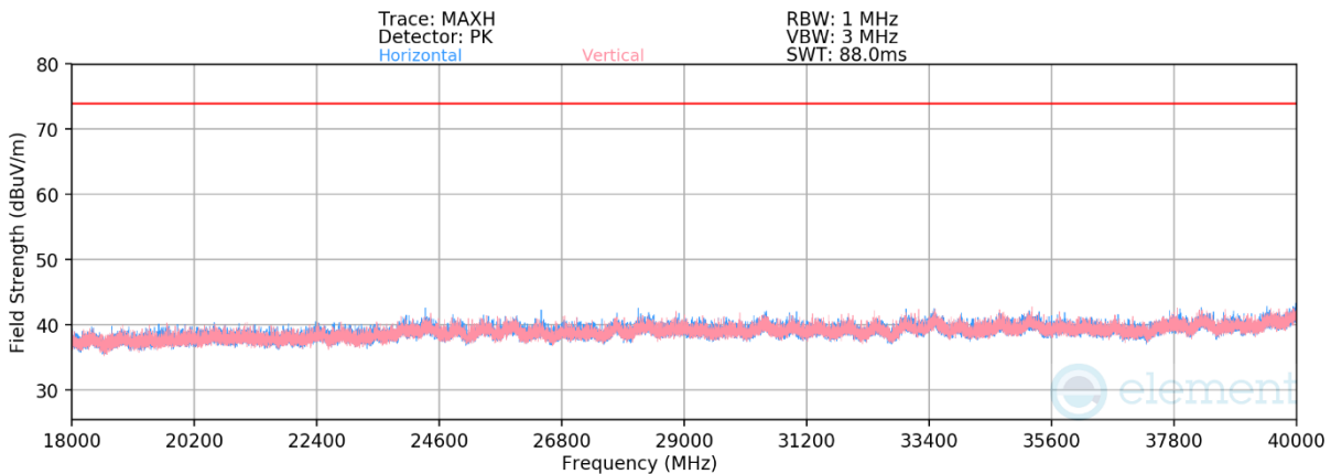
Plot 7-88. Radiated Spurious Emissions above 18GHz CDD Primary (802.11n – Ch. 56)
