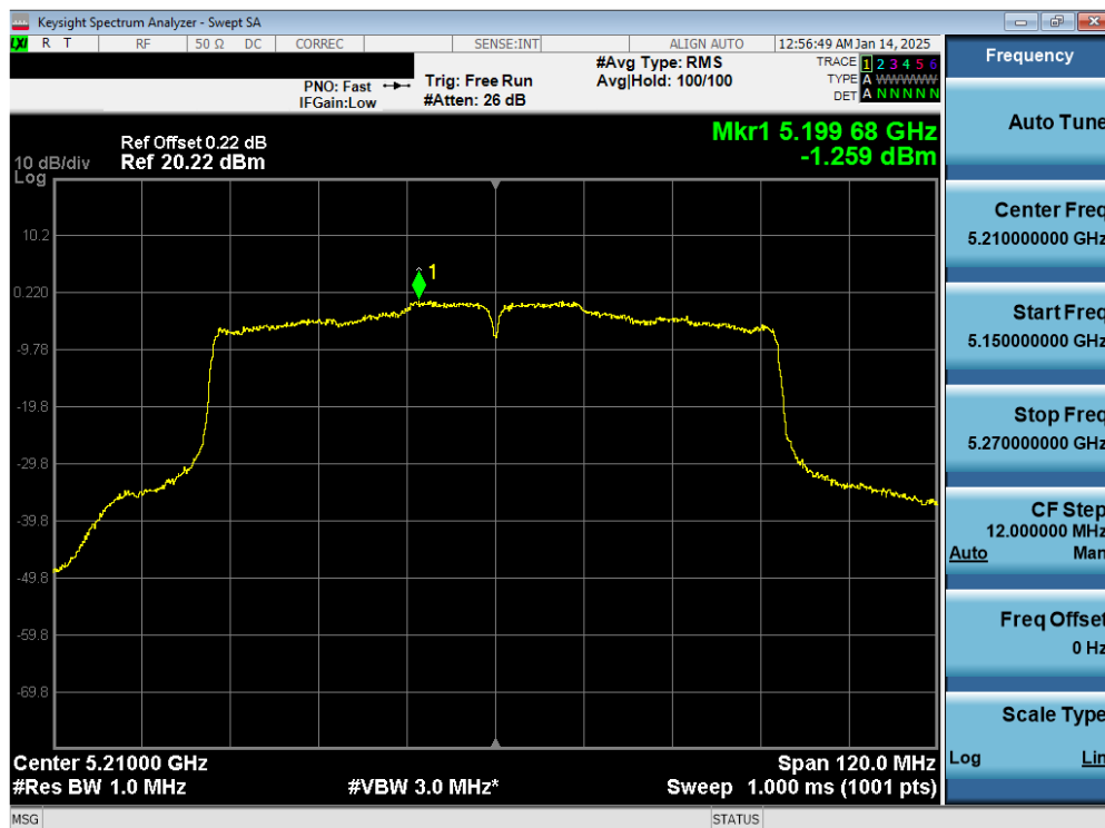
Plot 7-62. ISED PSD SDM Primary Antenna 3c (80MHz BW 11ac – Ch.42)
