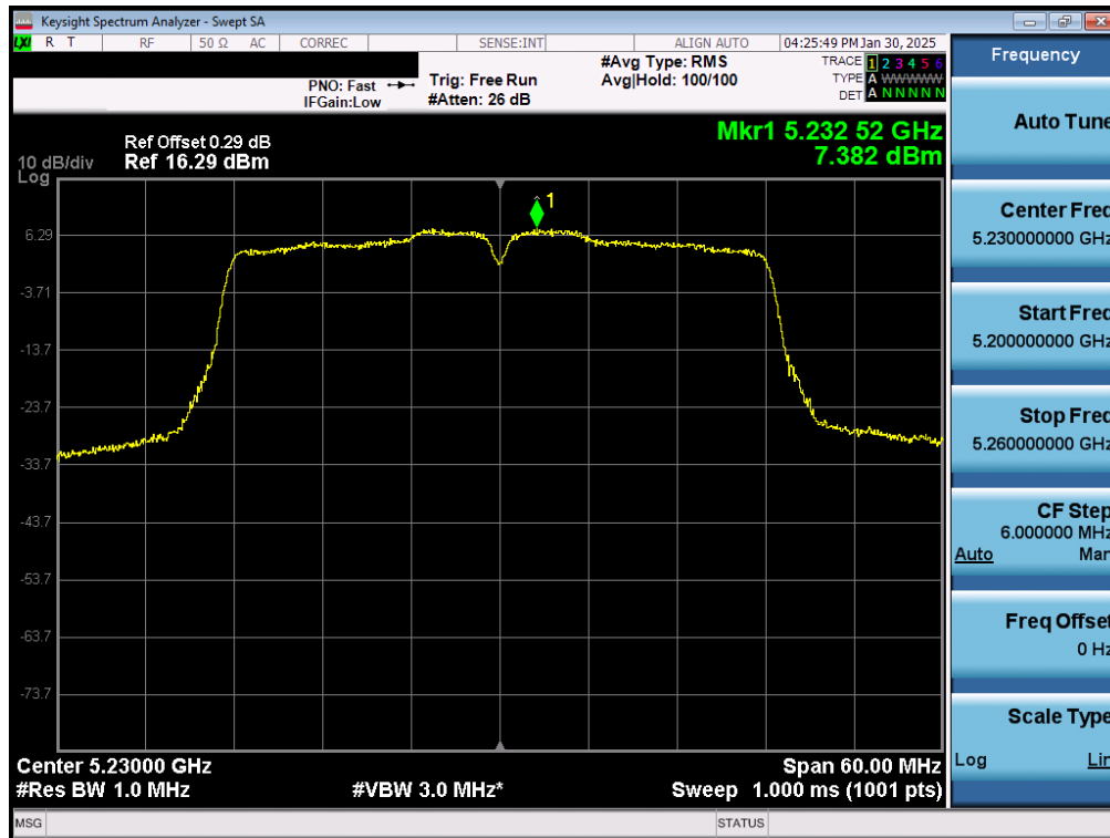
Plot 7-66. PSD CDD Diversity Antenna 3c (40MHz BW 802.11n – Ch. 46)
