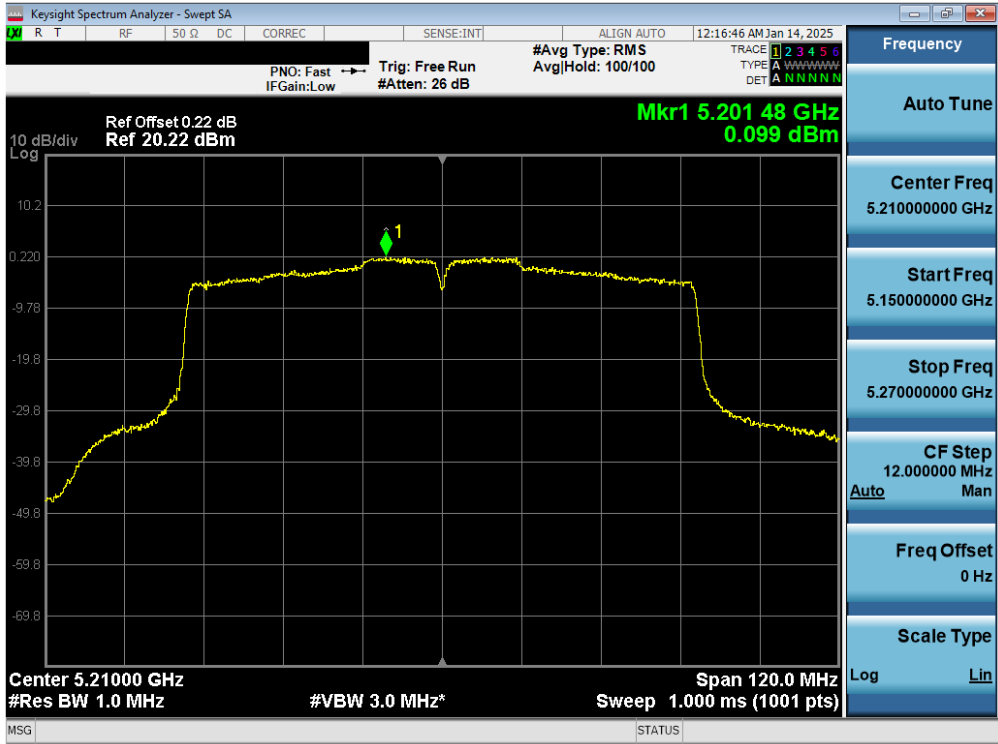
Plot 7-27. ISED PSD Antenna 3c (80MHz BW 11ac – Ch.42)
