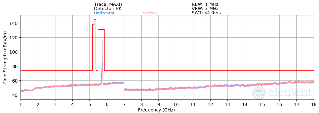
Plot 7-93. Radiated Spurious Emissions above 1GHz CDD Primary (802.11n – Ch. 144)
