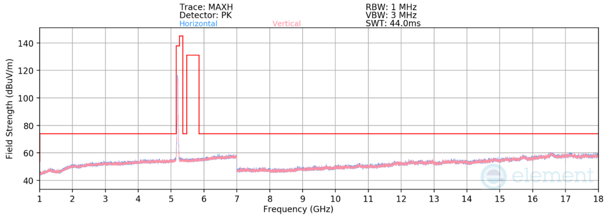
Plot 7-83. Radiated Spurious Emissions above 1GHz CDD Primary (802.11n – Ch. 40)
