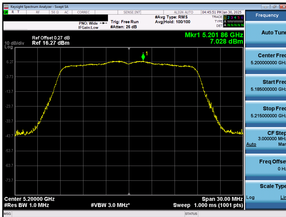
Plot 7-64. PSD CDD Diversity Antenna 3c (20MHz BW 802.11n – Ch. 40)
