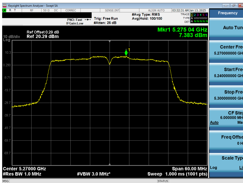
Plot 7-48. PSD CDD Primary Antenna 3c (40MHz BW 802.11n – Ch. 54)
