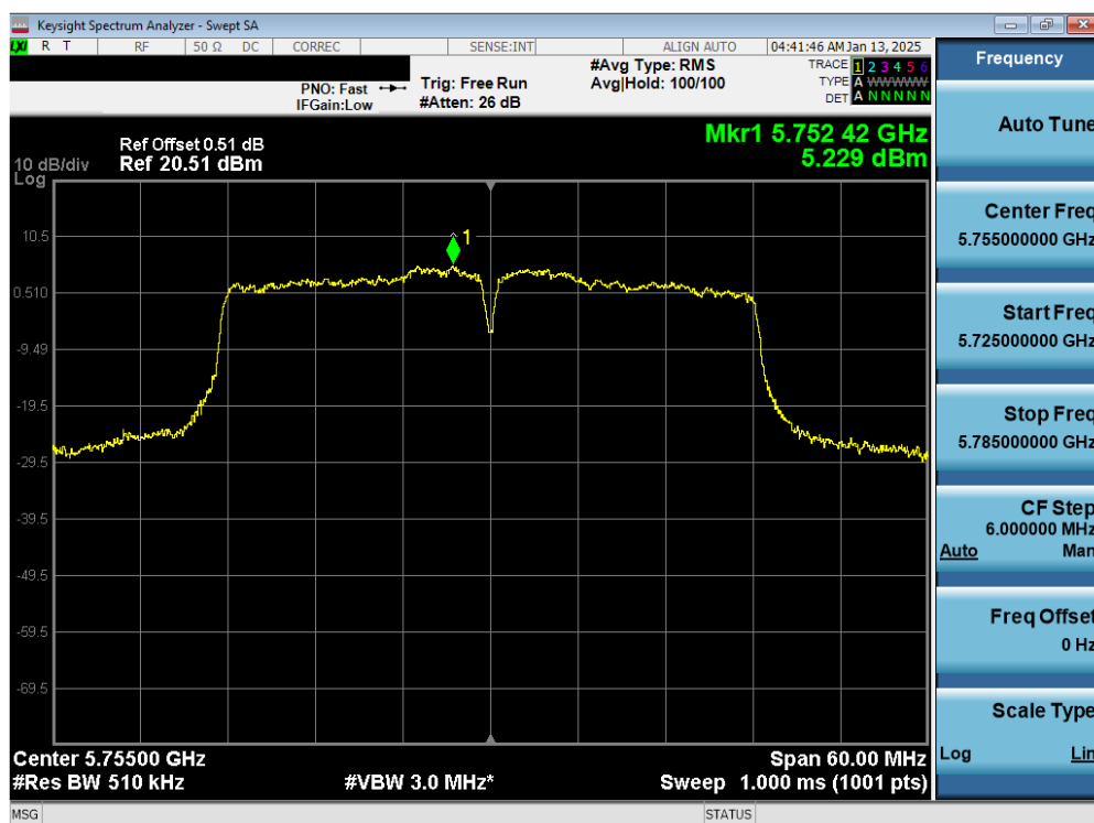
Plot 7-72. PSD CDD Diversity Antenna 3c (40MHz BW 802.11n – Ch. 151)
