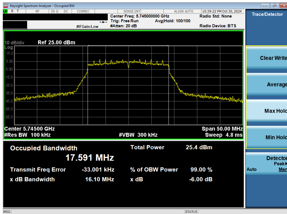
Plot 7-10. 6dB BW & 99% OBW Antenna 3c (20MHz BW 802.11n – Ch. 149)
