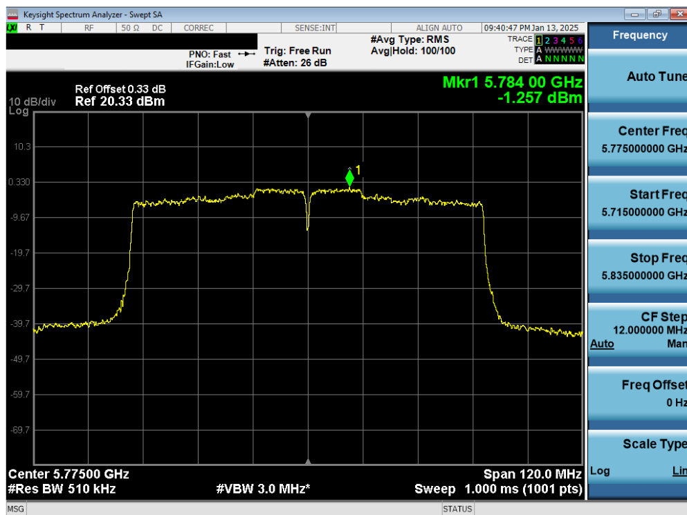
Plot 7-75. PSD CDD Diversity Antenna 1b (80MHz BW 802.11ac – Ch. 155)
