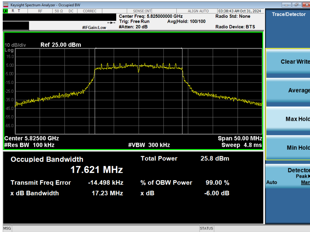
Plot 7-13. 6dB BW & 99% OBW Antenna 3a (20MHz BW 802.11n – Ch. 165)
