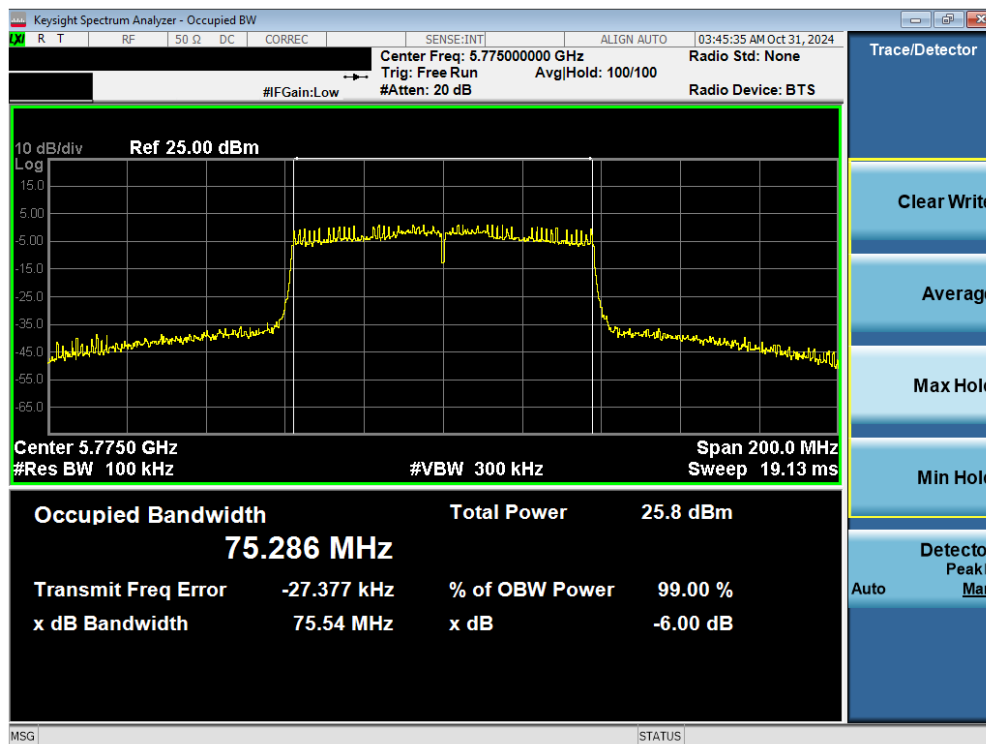
Plot 7-15. 6dB BW & 99% OBW Antenna 3a (80MHz BW 802.11ac – Ch. 155)
