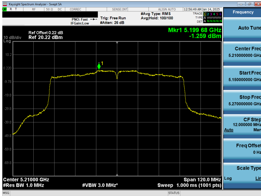
Plot 7-80. ISED PSD SDM Primary Antenna 3c (80MHz BW 11ac – Ch.42)
