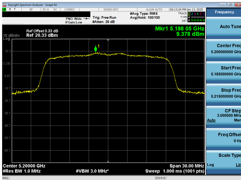
Plot 7-37. PSD Antenna 1b (20MHz BW 802.11ax (SU) – Ch.40)
