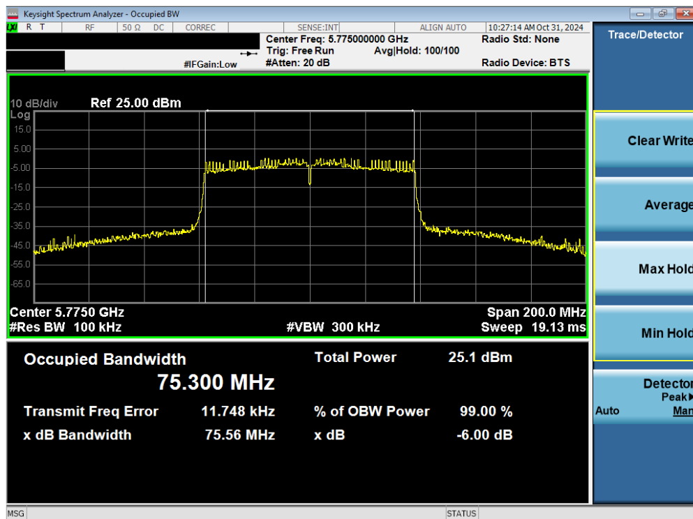
Plot 7-18. 6dB BW & 99% OBW Antenna 1b (80MHz BW 802.11ac – Ch. 155)
