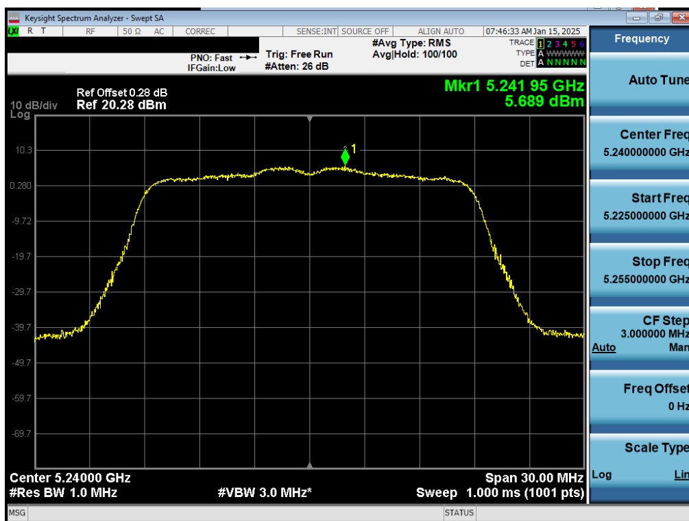
Plot 7-43. ISED PSD Antenna 1b (20MHz BW 11n – Ch.48)
