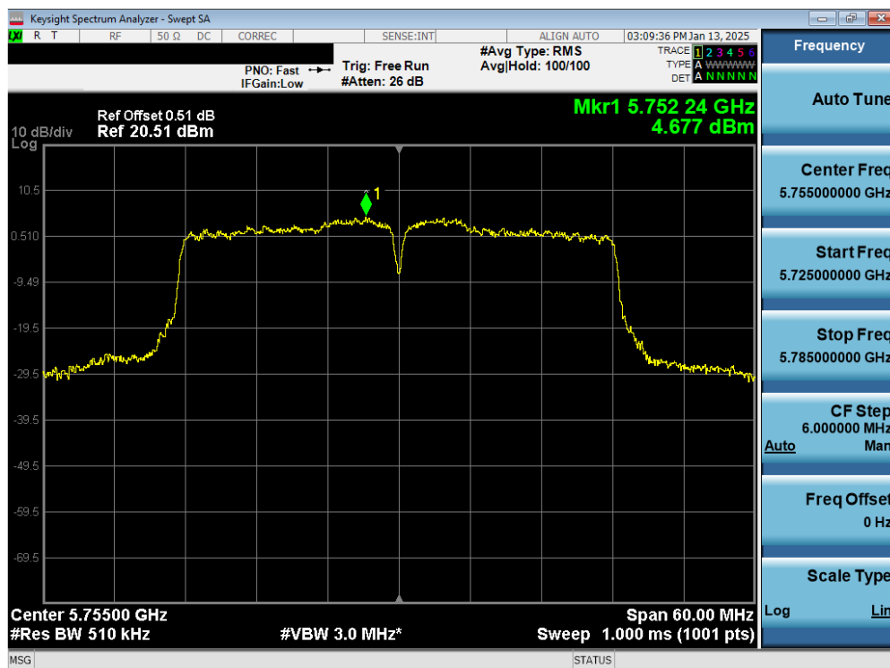
Plot 7-55. PSD CDD Primary Antenna 3a (40MHz BW 802.11n – Ch. 151)
