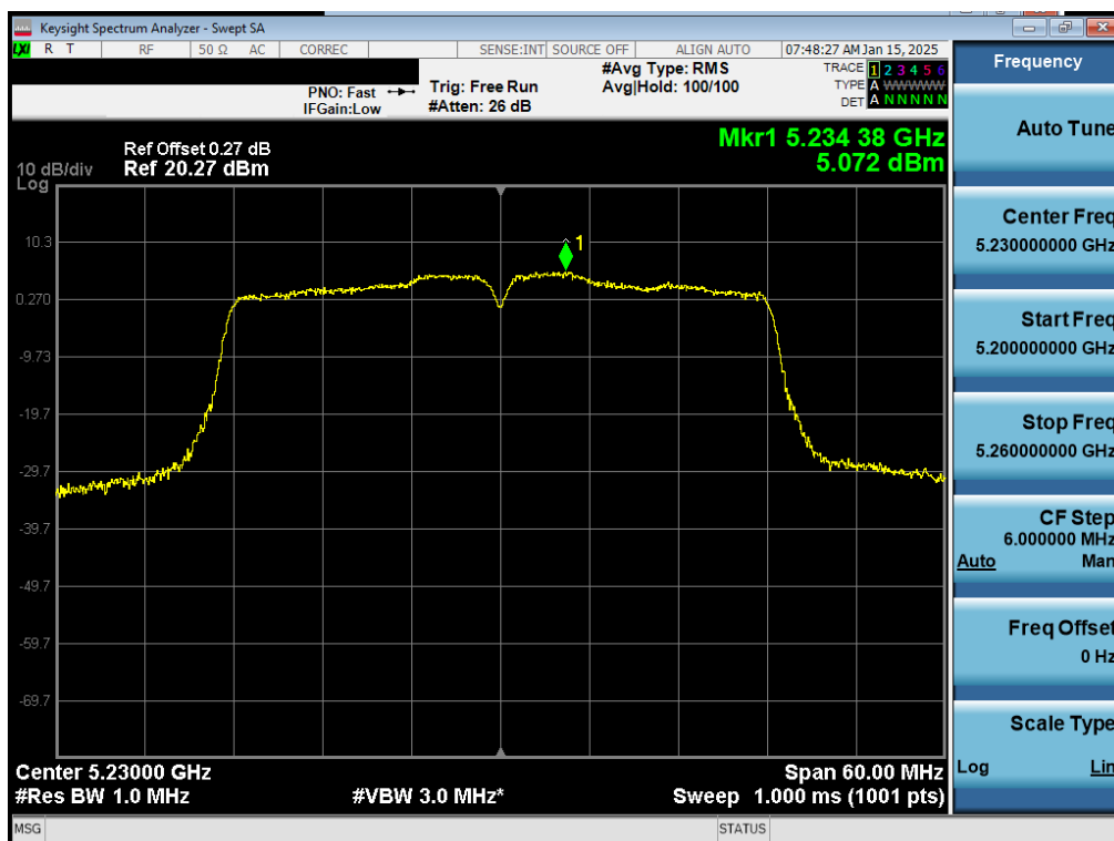
Plot 7-44. ISED PSD Antenna 1b (40MHz BW 11n – Ch.46)
