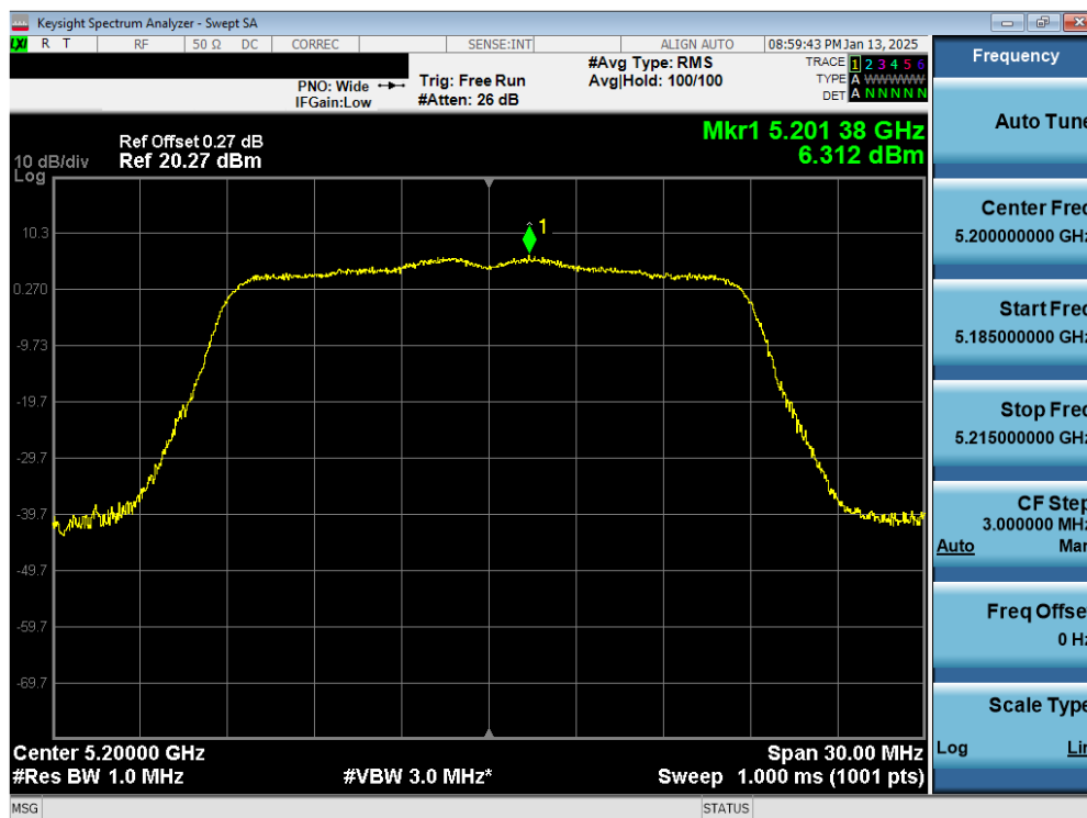
Plot 7-65. PSD CDD Diversity Antenna 1b (20MHz BW 802.11n – Ch. 40)
