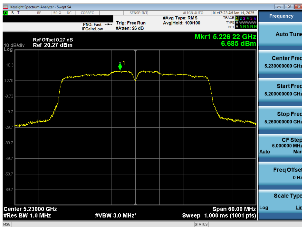
Plot 7-35. ISED PSD Antenna 3a (40MHz BW 11n – Ch.46)
