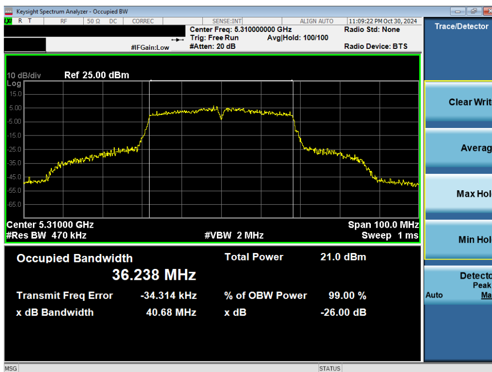
Plot 7-2. 26dB BW & 99% OBW Antenna 3c (40MHz BW 802.11n – Ch. 62)
