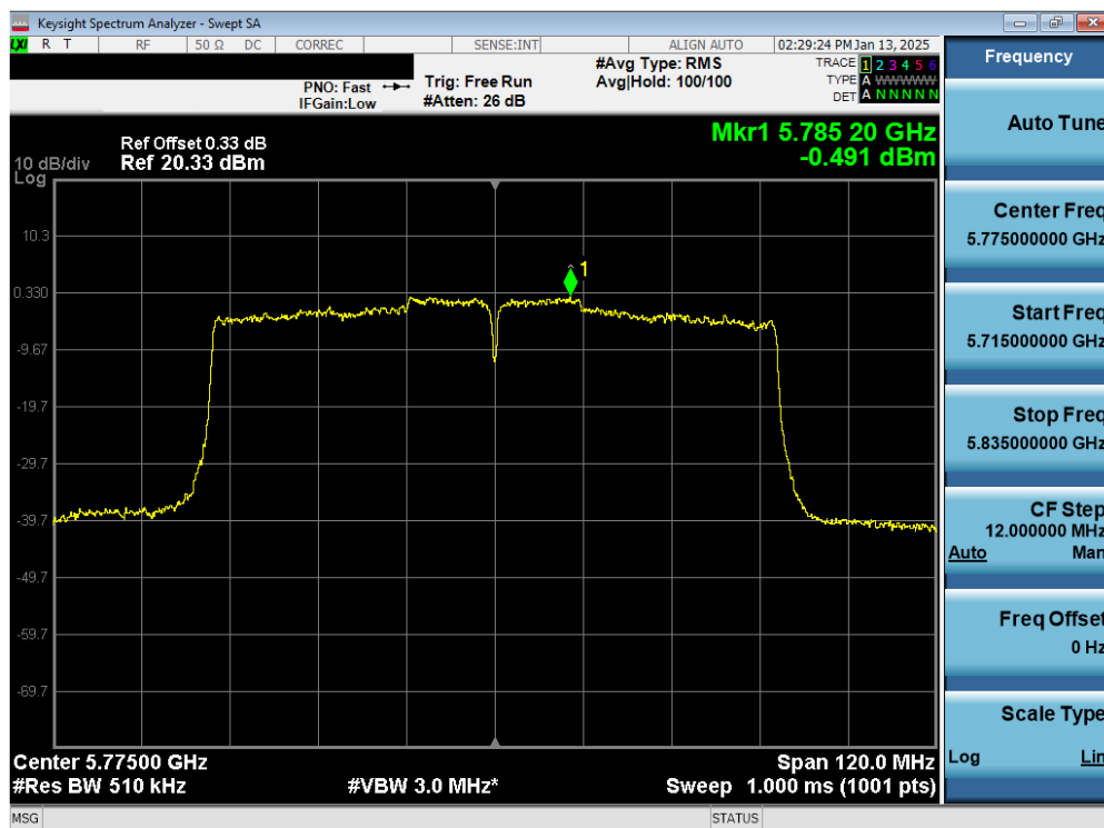
Plot 7-57. PSD CDD Primary Antenna 3a (80MHz BW 802.11ac – Ch. 155)
