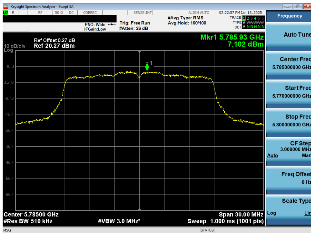
Plot 7-53. PSD CDD Primary Antenna 3a (20MHz BW 802.11n – Ch. 165)
