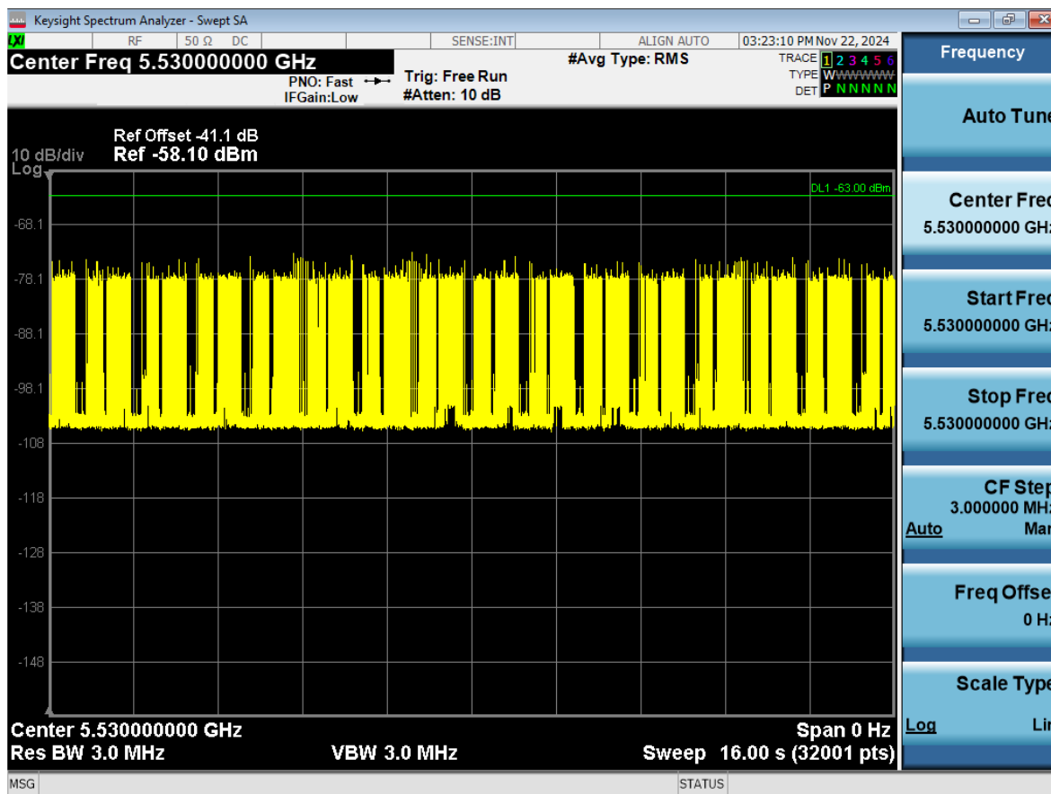
Figure 9-5. 5530MHz - Channel Loading - Mode 3 (80MHz)
