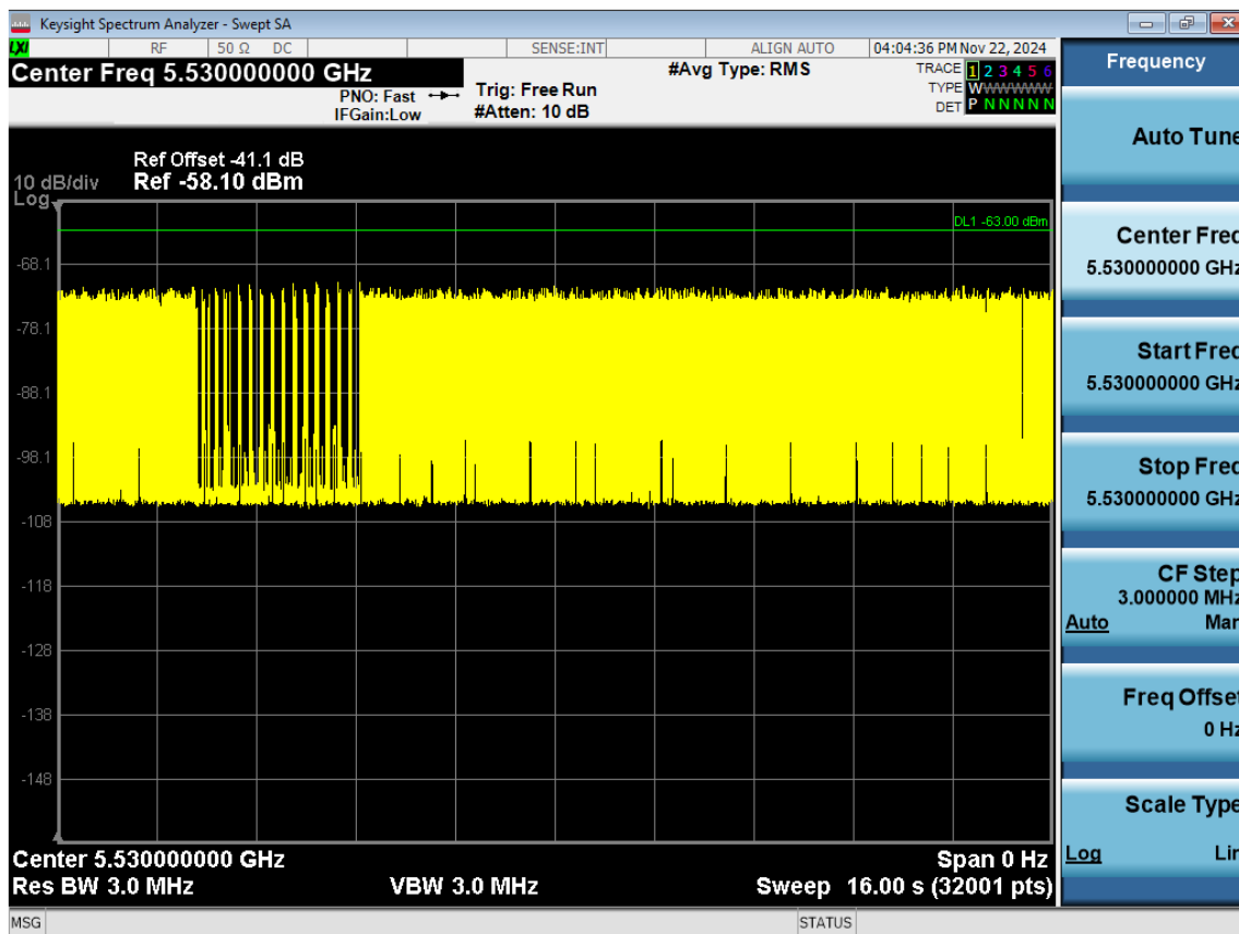
Figure 9-7. 5530 MHz - Channel Loading - Mode 4 (80MHz)
