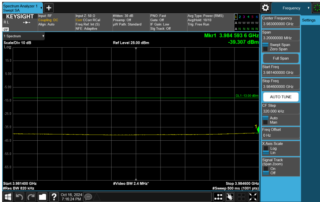
Plot 7-287. Upper ACP Plot (NR Band n77 C-Band - 80MHz DFT-s-OFDM \pi/2 BPSK – Full RB)
