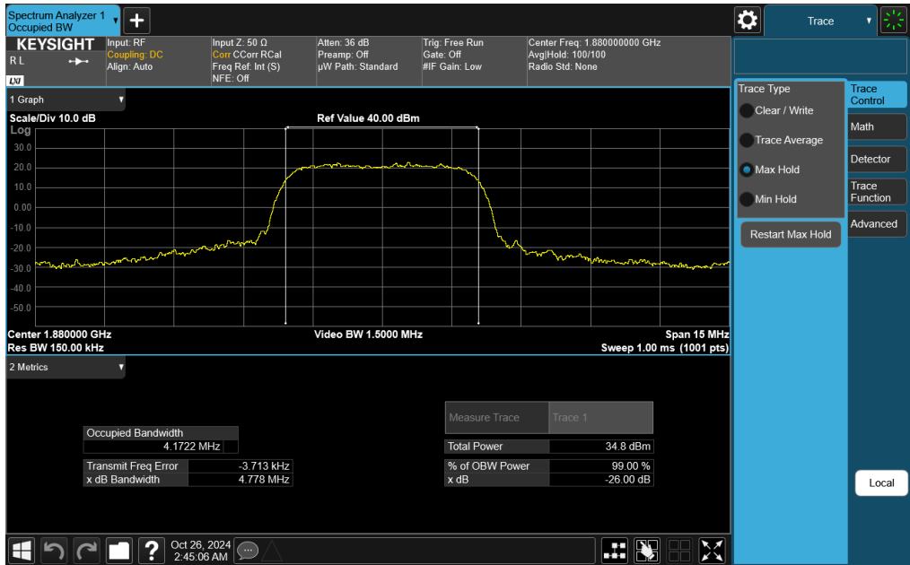
Plot 7-65. Occupied Bandwidth Plot (WCDMA, Ch. 9400)
