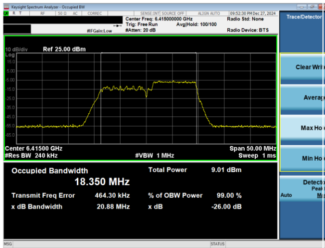
Plot 7-17. 26dB & 99% Bandwidth Plot Antenna WF2a (20MHz 802.11ax RU106 (UNII Band 5) – Ch. 93)
