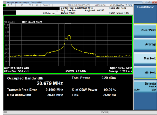
Plot 7-12. 26dB & 99% Bandwidth Plot Antenna WF7a (160MHz 802.11ax RU106 (UNII Band 7) – Ch. 143)
