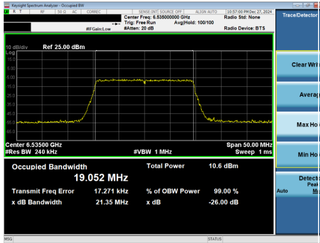
Plot 7-29. 26dB & 99% Bandwidth Plot Antenna WF2a (20MHz 802.11ax RU242 (UNII Band 7) – Ch. 117)
