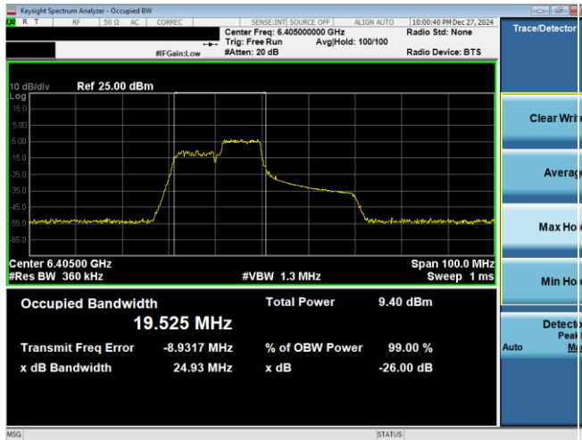
Plot 7-18. 26dB & 99% Bandwidth Plot Antenna WF2a (40MHz 802.11ax RU106 (UNII Band 5) – Ch. 91)
