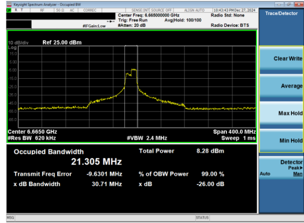
Plot 7-28. 26dB & 99% Bandwidth Plot Antenna WF2a (160MHz 802.11ax RU106 (UNII Band 7) – Ch. 143)
