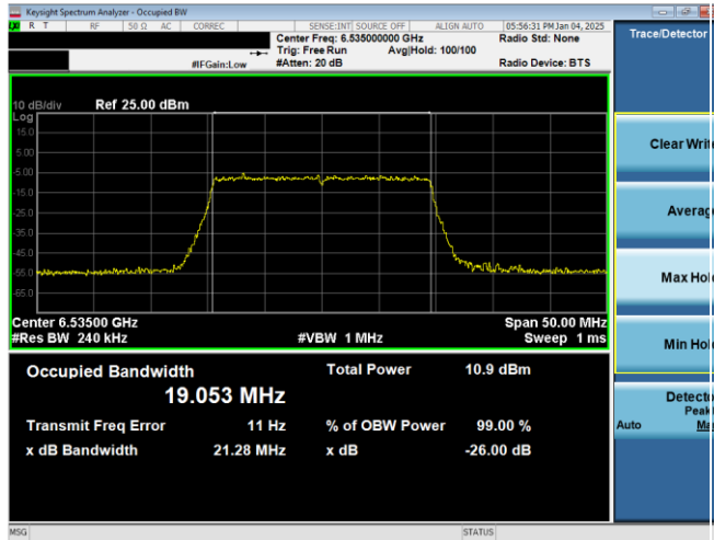
Plot 7-45. 26dB & 99% Bandwidth Plot Antenna WF7b (20MHz 802.11ax RU242 (UNII Band 7) – Ch. 117)
