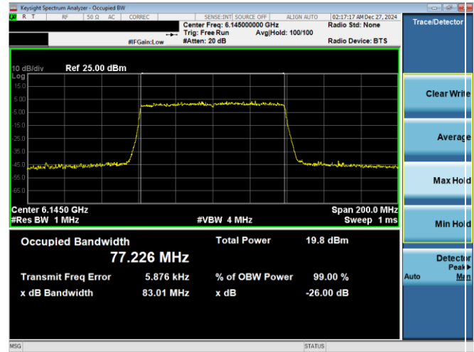
Plot 7-7. 26dB & 99% Bandwidth Plot Antenna WF7a (80MHz 802.11ax RU996 (UNII Band 5) – Ch. 39)
