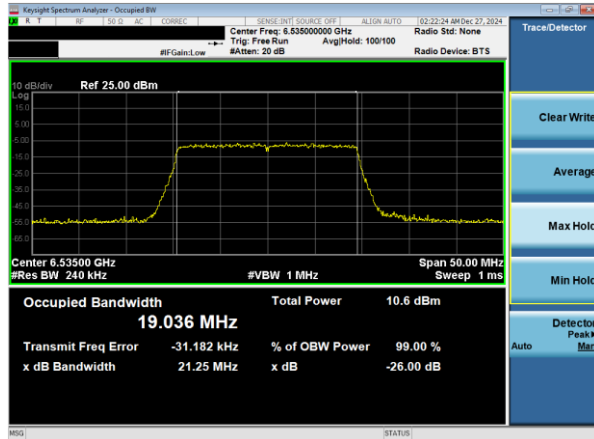
Plot 7-13. 26dB & 99% Bandwidth Plot Antenna WF7a (20MHz 802.11ax RU242 (UNII Band 7) – Ch. 117)
