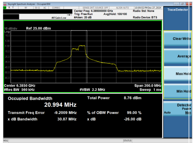
Plot 7-19. 26dB & 99% Bandwidth Plot Antenna WF2a (80MHz 802.11ax RU106 (UNII Band 5) – Ch. 87)
