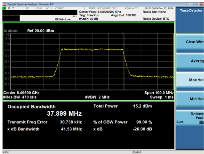
Plot 7-22. 26dB & 99% Bandwidth Plot Antenna WF2a (40MHz 802.11ax RU484 (UNII Band 5) – Ch. 91)
