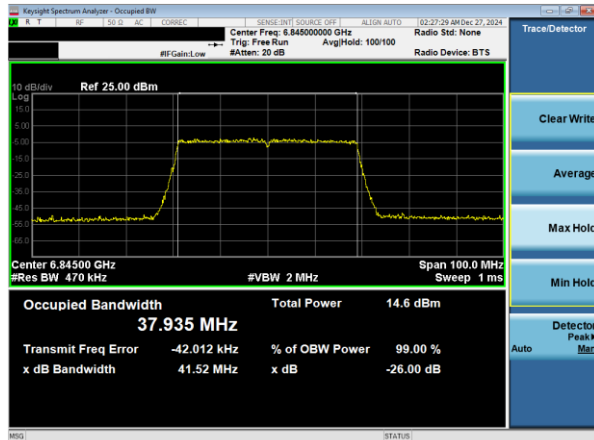
Plot 7-14. 26dB & 99% Bandwidth Plot Antenna WF7a (40MHz 802.11ax RU484 (UNII Band 7) – Ch. 179)
