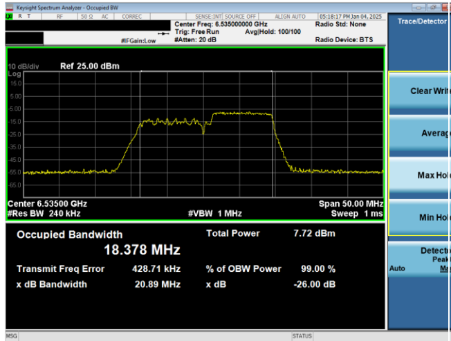
Plot 7-41. 26dB & 99% Bandwidth Plot Antenna WF7b (20MHz 802.11ax RU106 (UNII Band 7) – Ch. 117)
