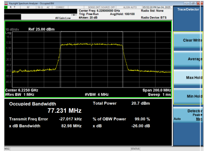
Plot 7-39. 26dB & 99% Bandwidth Plot Antenna WF7b (80MHz 802.11ax RU996 (UNII Band 5) – Ch. 55)
