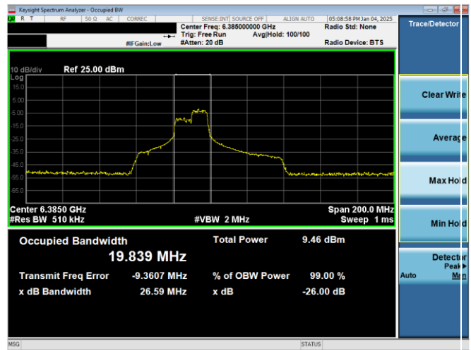
Plot 7-35. 26dB & 99% Bandwidth Plot Antenna WF7b (80MHz 802.11ax RU106 (UNII Band 5) – Ch. 87)
