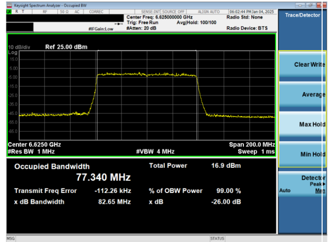
Plot 7-47. 26dB & 99% Bandwidth Plot Antenna WF7b (80MHz 802.11ax RU996 (UNII Band 7) – Ch. 135)
