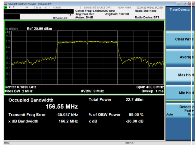
Plot 7-8. 26dB & 99% Bandwidth Plot Antenna WF7a (160MHz 802.11ax RU996x2 (UNII Band 5) – Ch. 47)
