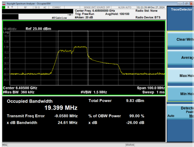
Plot 7-2. 26dB & 99% Bandwidth Plot Antenna WF7a (40MHz 802.11ax RU106 (UNII Band 5) - Ch. 91)
