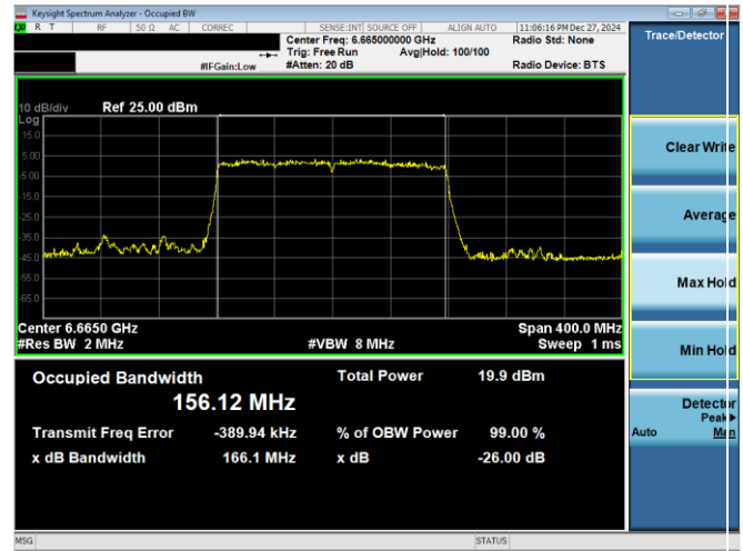
Plot 7-32. 26dB & 99% Bandwidth Plot Antenna WF2a (160MHz 802.11ax RU996x2 (UNII Band 7) – Ch. 143)
