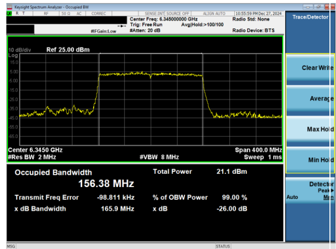
Plot 7-24. 26dB & 99% Bandwidth Plot Antenna WF2a (160MHz 802.11ax RU996x2 (UNII Band 5) – Ch. 79)
