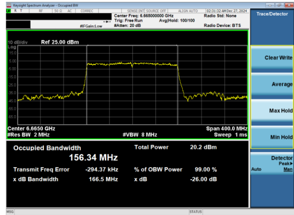
Plot 7-16. 26dB & 99% Bandwidth Plot Antenna WF7a (160MHz 802.11ax RU996x2 (UNII Band 7) – Ch. 143)
