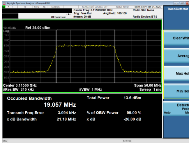
Plot 7-37. 26dB & 99% Bandwidth Plot Antenna WF7b (20MHz 802.11ax RU242 (UNII Band 5) – Ch. 33)
