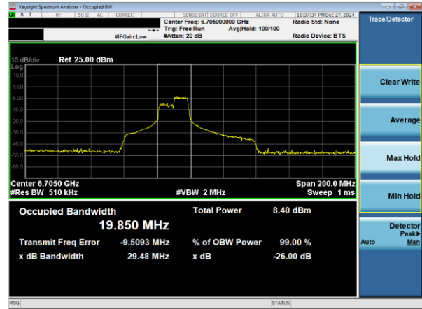
Plot 7-27. 26dB & 99% Bandwidth Plot Antenna WF2a (80MHz 802.11ax RU106 (UNII Band 7) – Ch. 151)
