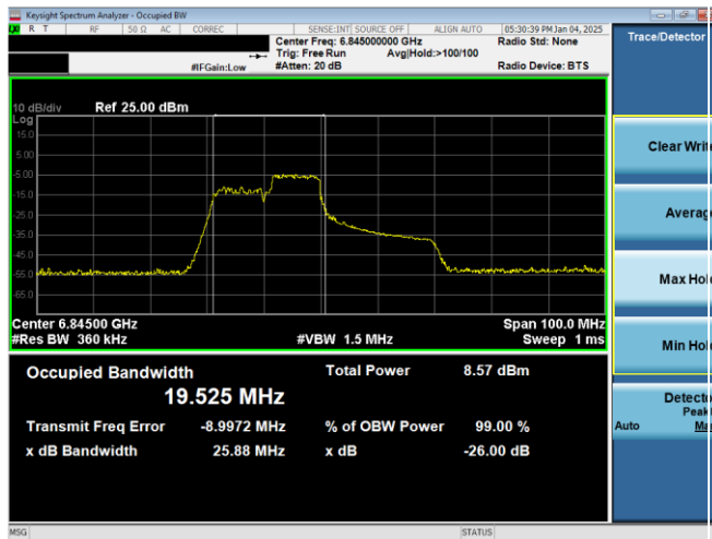
Plot 7-42. 26dB & 99% Bandwidth Plot Antenna WF7b (40MHz 802.11ax RU106 (UNII Band 7) – Ch. 179)
