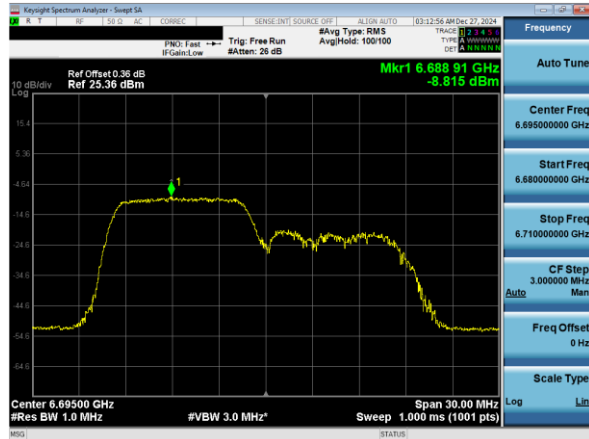
Plot 7-57. PSD Plot Antenna WF7a (20MHz 802.11ax RU106 (UNII Band 7) – Ch. 149)
