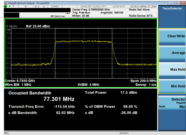
Plot 7-15. 26dB & 99% Bandwidth Plot Antenna WF7a (80MHz 802.11ax RU996 (UNII Band 7) – Ch. 167)
