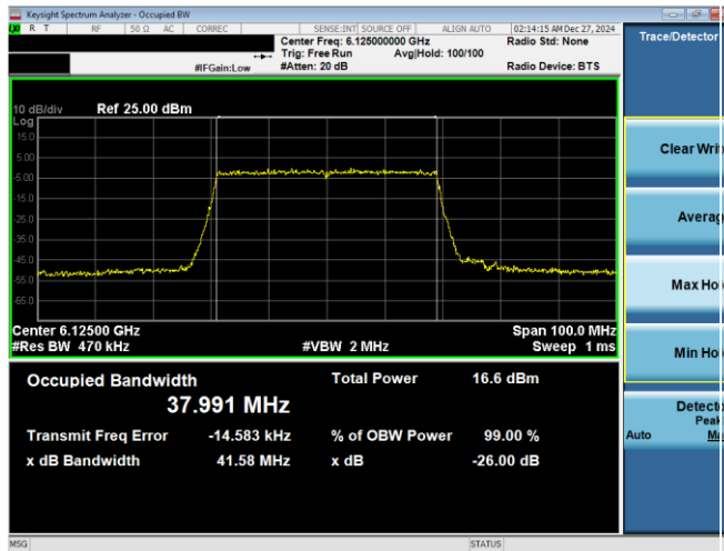
Plot 7-6. 26dB & 99% Bandwidth Plot Antenna WF7a (40MHz 802.11ax RU484 (UNII Band 5) – Ch. 35)
