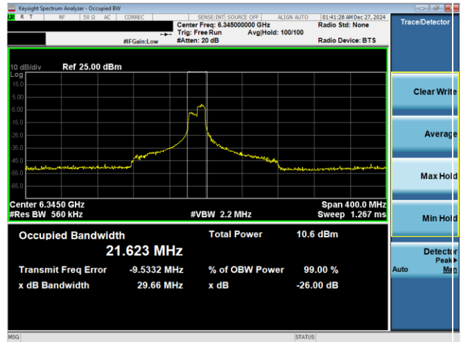
Plot 7-4. 26dB & 99% Bandwidth Plot Antenna WF7a (160MHz 802.11ax RU106 (UNII Band 5) - Ch. 79)
