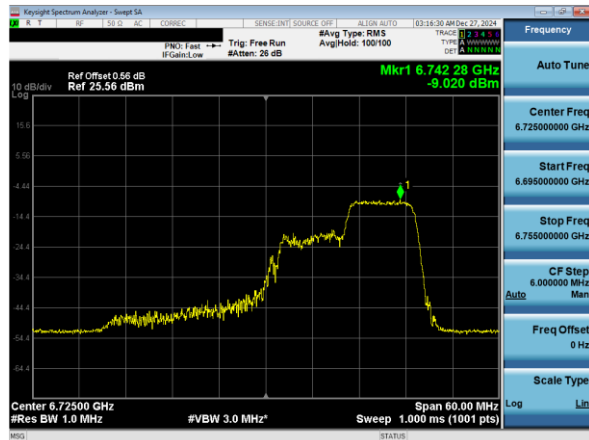
Plot 7-58. PSD Plot Antenna WF7a (40MHz 802.11ax RU106 (UNII Band 7) – Ch. 155)
