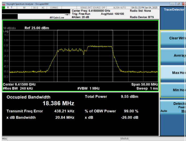
Plot 7-33. 26dB & 99% Bandwidth Plot Antenna WF7b (20MHz 802.11ax RU106 (UNII Band 5) – Ch. 93)
