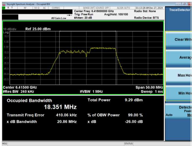
Plot 7-1. 26dB & 99% Bandwidth Plot Antenna WF7a (20MHz 802.11ax RU106 (UNII Band 5) - Ch. 93)
