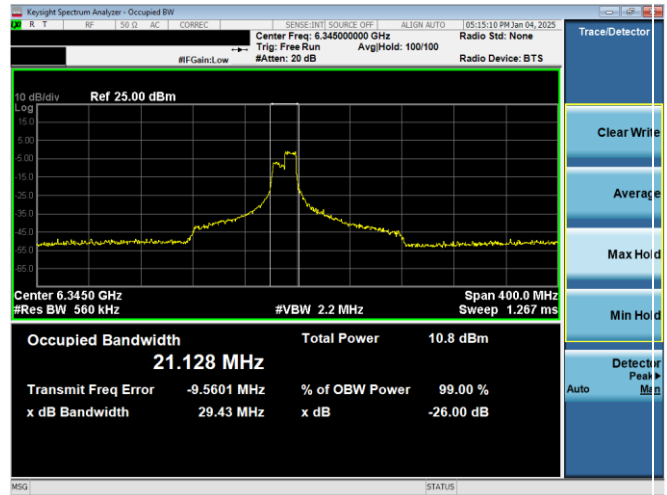
Plot 7-36. 26dB & 99% Bandwidth Plot Antenna WF7b (160MHz 802.11ax RU106 (UNII Band 5) – Ch. 79)
