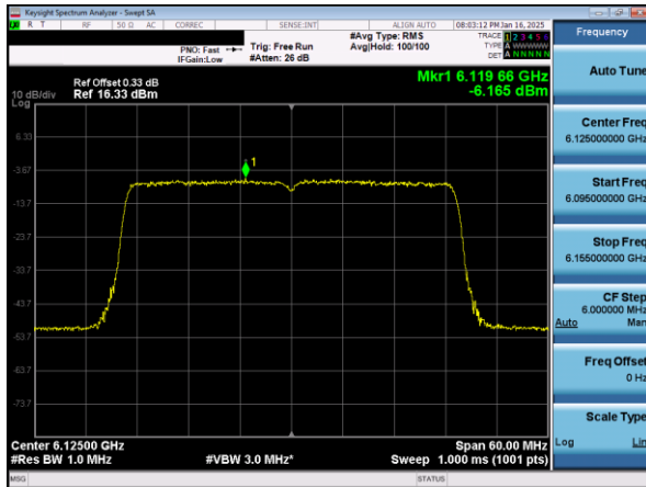
Plot 7-54. PSD Plot Antenna WF7a (40MHz 802.11ax RU484 (UNII Band 5) – Ch. 35)
