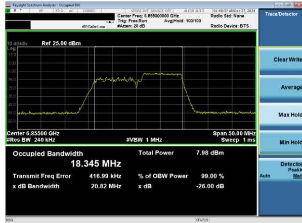
Plot 7-9. 26dB & 99% Bandwidth Plot Antenna WF7a (20MHz 802.11ax RU106 (UNII Band 7) – Ch. 181)
