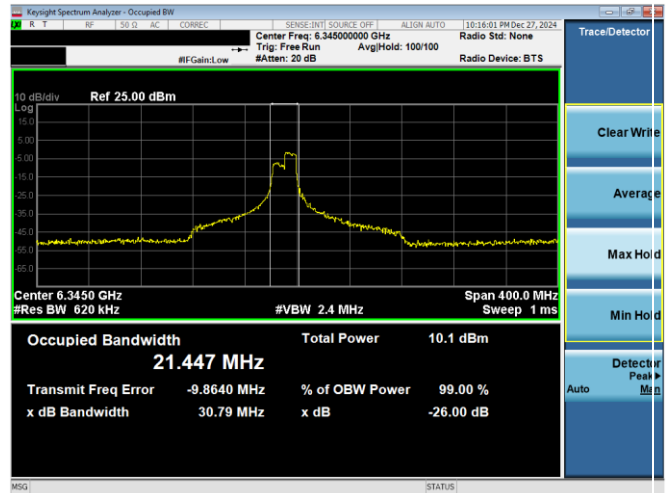
Plot 7-20. 26dB & 99% Bandwidth Plot Antenna WF2a (160MHz 802.11ax RU106 (UNII Band 5) – Ch. 79)
