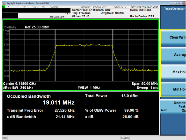
Plot 7-21. 26dB & 99% Bandwidth Plot Antenna WF2a (20MHz 802.11ax RU242 (UNII Band 5) – Ch. 33)
