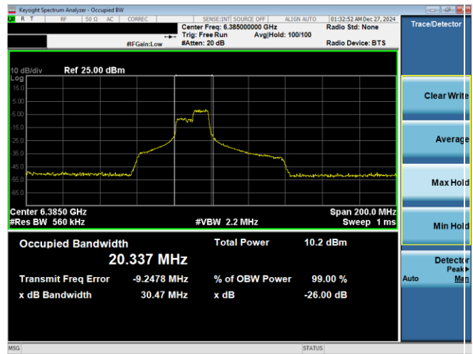
Plot 7-3. 26dB & 99% Bandwidth Plot Antenna WF7a (80MHz 802.11ax RU106 (UNII Band 5) - Ch. 87)
