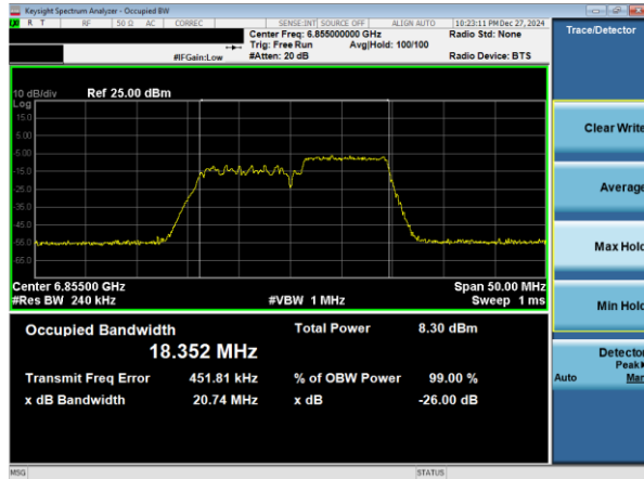
Plot 7-25. 26dB & 99% Bandwidth Plot Antenna WF2a (20MHz 802.11ax RU106 (UNII Band 7) – Ch. 181)
