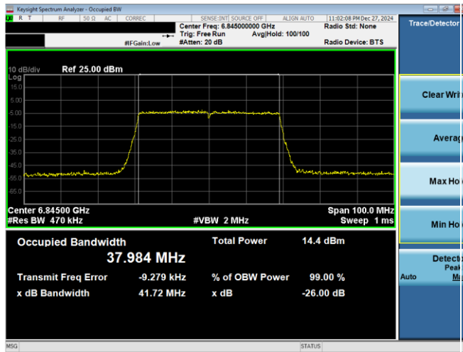
Plot 7-30. 26dB & 99% Bandwidth Plot Antenna WF2a (40MHz 802.11ax RU484 (UNII Band 7) – Ch. 179)
