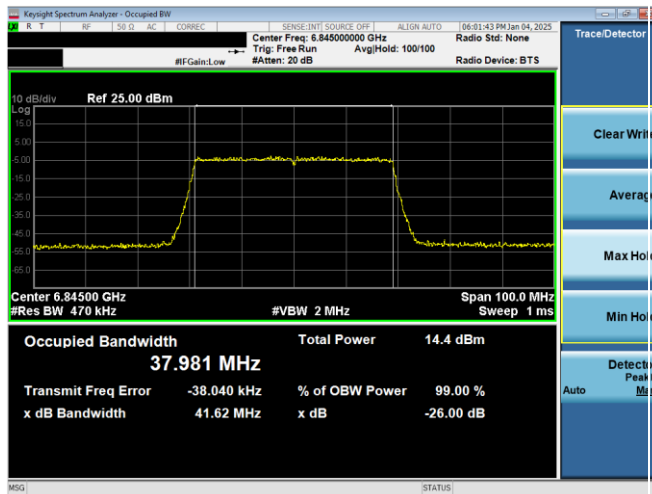
Plot 7-46. 26dB & 99% Bandwidth Plot Antenna WF7b (40MHz 802.11ax RU484 (UNII Band 7) – Ch. 179)
