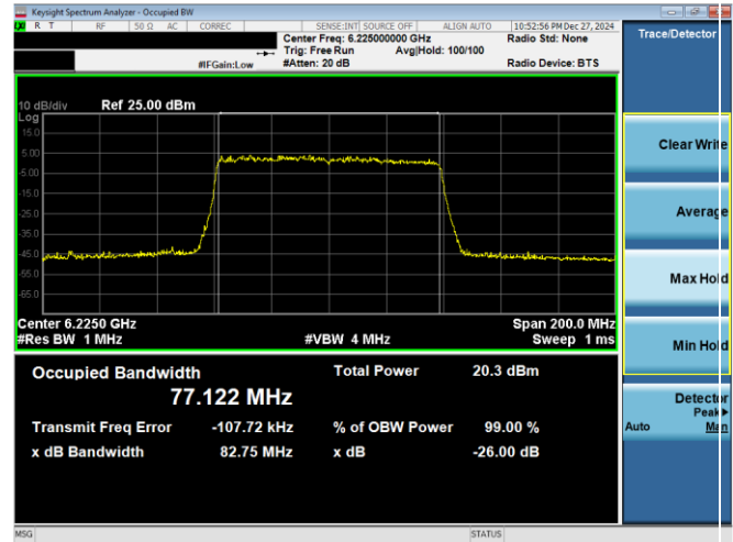
Plot 7-23. 26dB & 99% Bandwidth Plot Antenna WF2a (80MHz 802.11ax RU996 (UNII Band 5) – Ch. 55)
