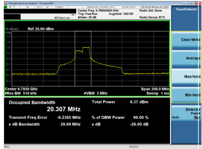
Plot 7-43. 26dB & 99% Bandwidth Plot Antenna WF7b (80MHz 802.11ax RU106 (UNII Band 7) – Ch. 167)
