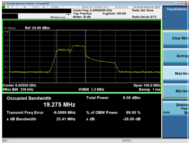
Plot 7-34. 26dB & 99% Bandwidth Plot Antenna WF7b (40MHz 802.11ax RU106 (UNII Band 5) – Ch. 91)
