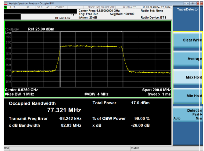
Plot 7-31. 26dB & 99% Bandwidth Plot Antenna WF2a (80MHz 802.11ax RU996 (UNII Band 7) – Ch. 135)
