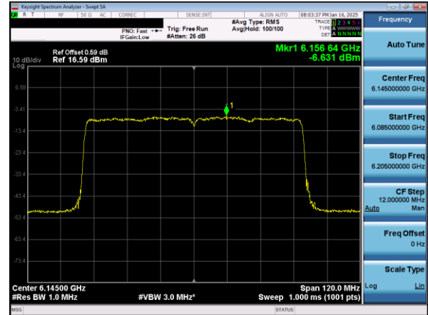
Plot 7-55. PSD Plot Antenna WF7a (80MHz 802.11ax RU996 (UNII Band 5) – Ch. 39)
