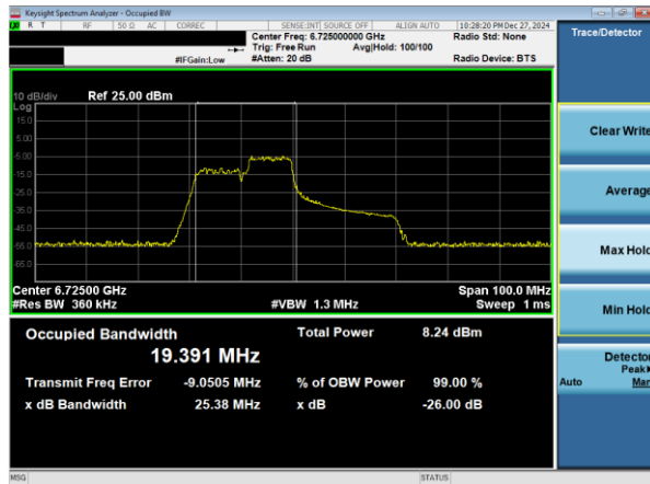
Plot 7-26. 26dB & 99% Bandwidth Plot Antenna WF2a (40MHz 802.11ax RU106 (UNII Band 7) – Ch. 155)
