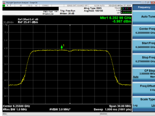
Plot 7-53. PSD Plot Antenna WF7a (20MHz 802.11ax RU242 (UNII Band 5) – Ch. 61)
