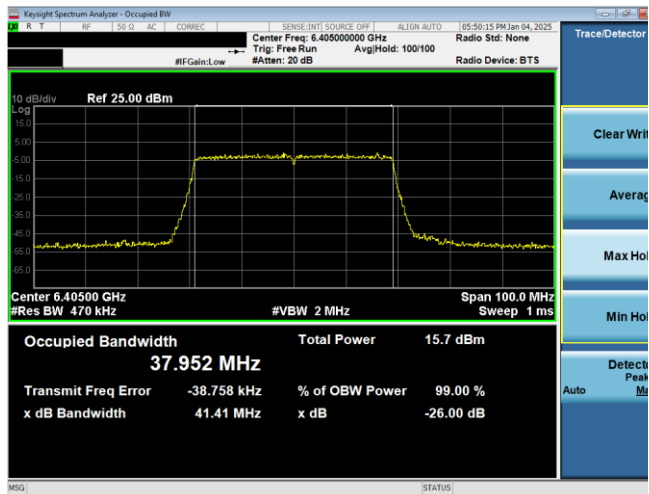
Plot 7-38. 26dB & 99% Bandwidth Plot Antenna WF7b (40MHz 802.11ax RU484 (UNII Band 5) – Ch. 91)
