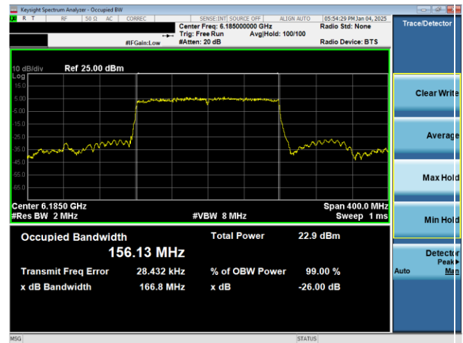
Plot 7-40. 26dB & 99% Bandwidth Plot Antenna WF7b (160MHz 802.11ax RU996x2 (UNII Band 5) – Ch. 47)
