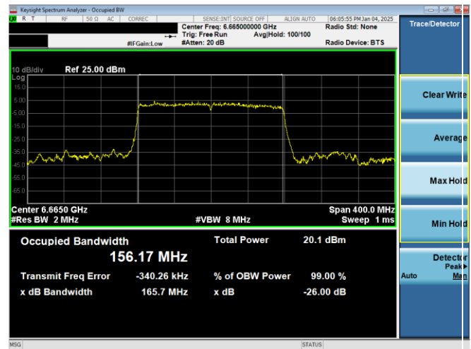
Plot 7-48. 26dB & 99% Bandwidth Plot Antenna WF7b (160MHz 802.11ax RU996x2 (UNII Band 7) – Ch. 143)
