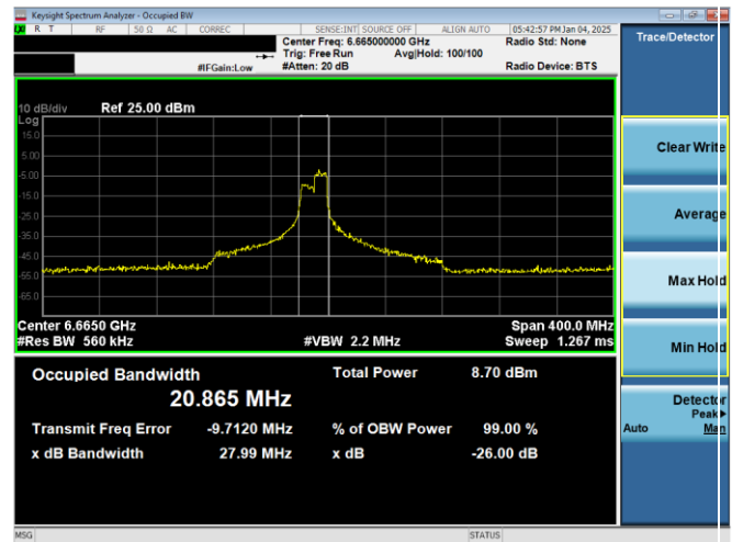
Plot 7-44. 26dB & 99% Bandwidth Plot Antenna WF7b (160MHz 802.11ax RU106 (UNII Band 7) – Ch. 143)
