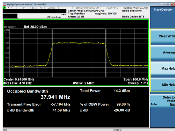
Plot 7-6. 26dB & 99% Bandwidth Plot Antenna WF7a (40MHz) 802.11ax (UNII Band 7) - Ch. 179)
