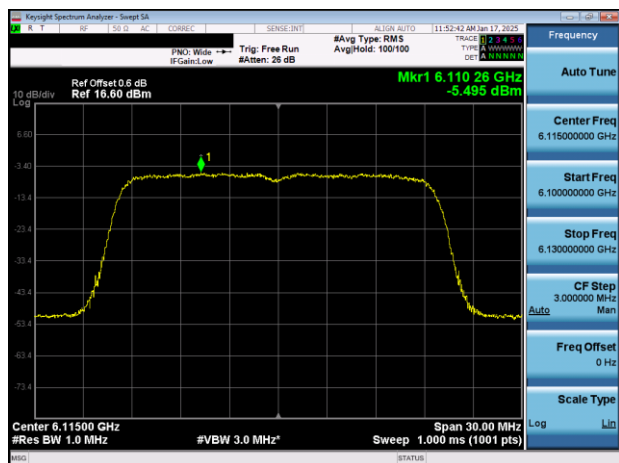
Plot 7-41. PSD Plot Antenna WF7b (20MHz 802.11ax (UNII Band 5) – Ch. 33)
