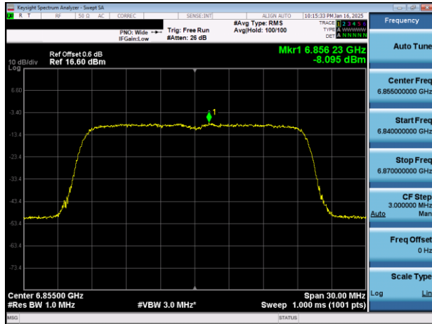
Plot 7-29. PSD Plot Antenna WF7a (20MHz 802.11ax (UNII Band 7) – Ch. 181)– Ch. 181)
