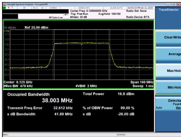
Plot 7-10. 26dB & 99% Bandwidth Plot Antenna WF2a (40MHz 802.11ax (UNII Band 5) – Ch. 35)
