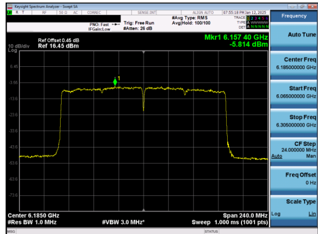
Plot 7-36. PSD Plot Antenna WF2a (160MHz 802.11ax (UNII Band 5) – Ch. 47)
