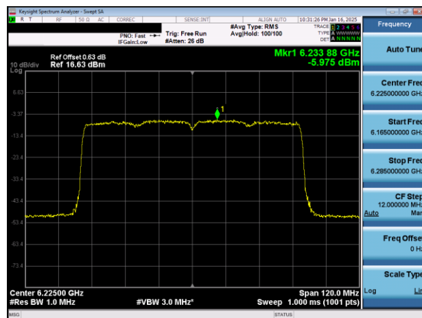
Plot 7-43. PSD Plot Antenna WF7b (80MHz 802.11ax (UNII Band 5) – Ch. 55)
