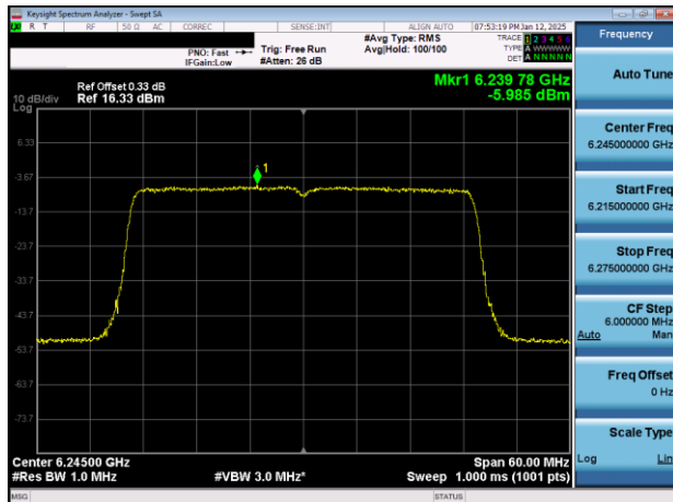
Plot 7-34. PSD Plot Antenna WF2a (40MHz 802.11ax (UNII Band 5) – Ch. 59)
