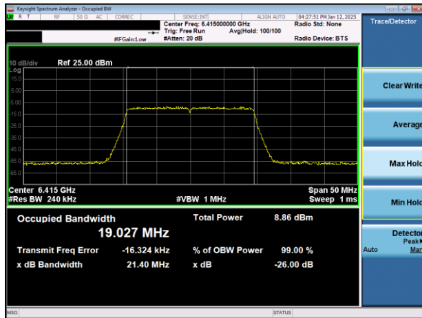
Plot 7-1. 26dB & 99% Bandwidth Plot Antenna WF7a (20MHz 802.11ax (UNII Band 5) – Ch. 93)
