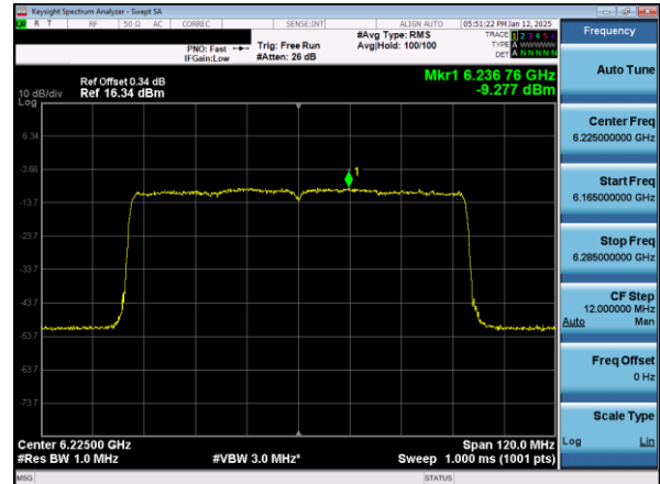
Plot 7-53. Power Spectral Density Plot SDM Primary Antenna WF7a (80MHz 802.11ax (UNII Band 5) – Ch. 55)
