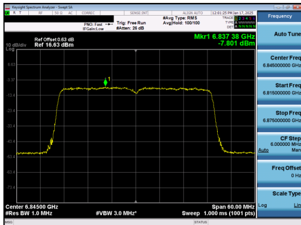
Plot 7-46. PSD Plot Antenna WF7b (40MHz 802.11ax (UNII Band 7) – Ch. 179)
