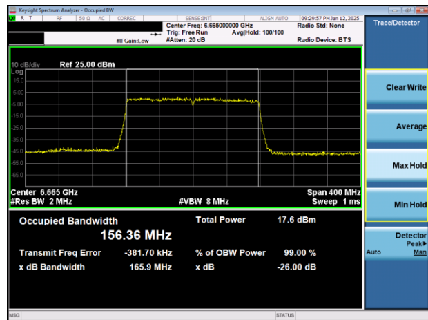
Plot 7-24. 26dB & 99% Bandwidth Plot Antenna WF7b (160MHz 802.11ax (UNII Band 7) – Ch. 143)
