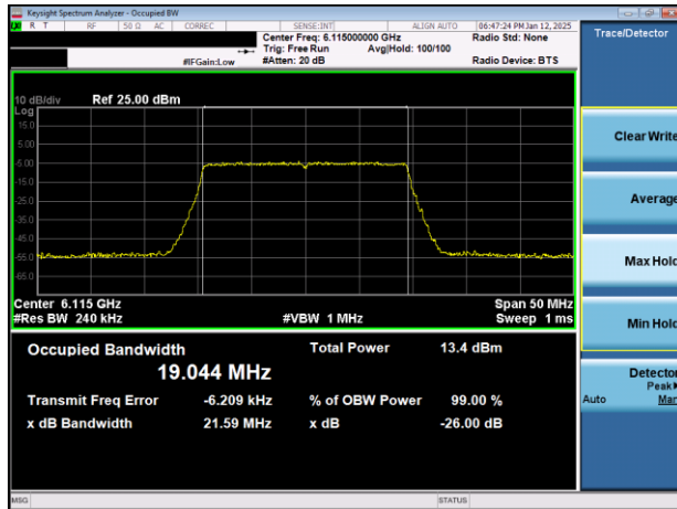
Plot 7-9. 26dB & 99% Bandwidth Plot Antenna WF2a (20MHz 802.11ax (UNII Band 5) – Ch. 33)
