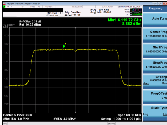
Plot 7-51. Power Spectral Density Plot SDM Primary Antenna WF7a (40MHz 802.11ax (UNII Band 5) – Ch. 35)
