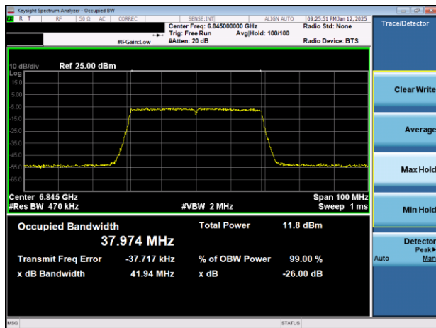
Plot 7-22. 26dB & 99% Bandwidth Plot Antenna WF7b (40MHz 802.11ax (UNII Band 7) – Ch. 179)
