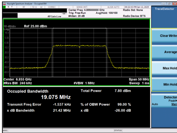
Plot 7-21. 26dB & 99% Bandwidth Plot Antenna WF7b (20MHz 802.11ax (UNII Band 7) – Ch. 181)
