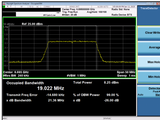
Plot 7-5. 26dB & 99% Bandwidth Plot Antenna WF7a (20MHz) 802.11ax (UNII Band 7) - Ch. 149)
