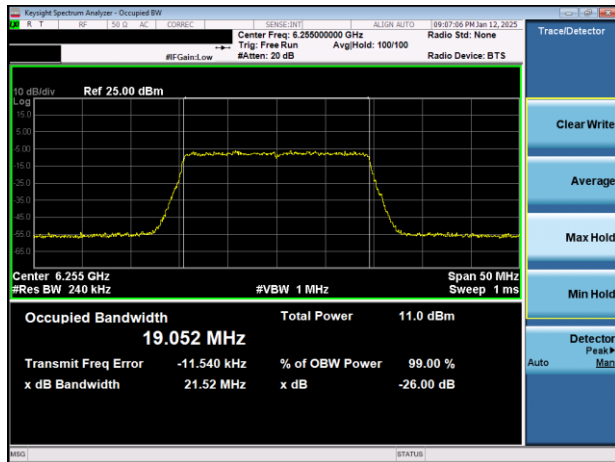
Plot 7-17. 26dB & 99% Bandwidth Plot Antenna WF7b (20MHz 802.11ax (UNII Band 5) – Ch. 61)
