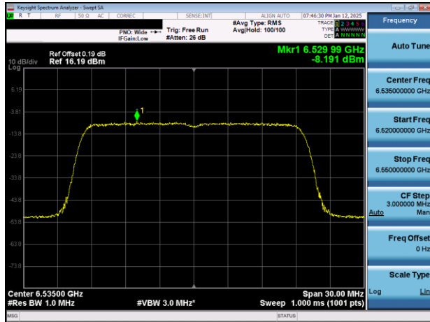
Plot 7-37. PSD Plot Antenna WF2a (20MHz 802.11ax (UNII Band 7) – Ch. 117)
