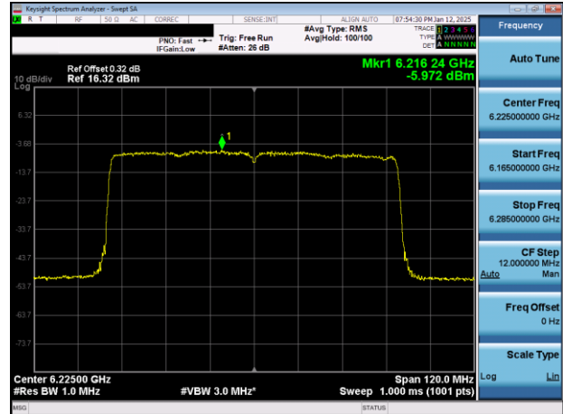
Plot 7-35. PSD Plot Antenna WF2a (80MHz 802.11ax (UNII Band 5) – Ch. 55)
