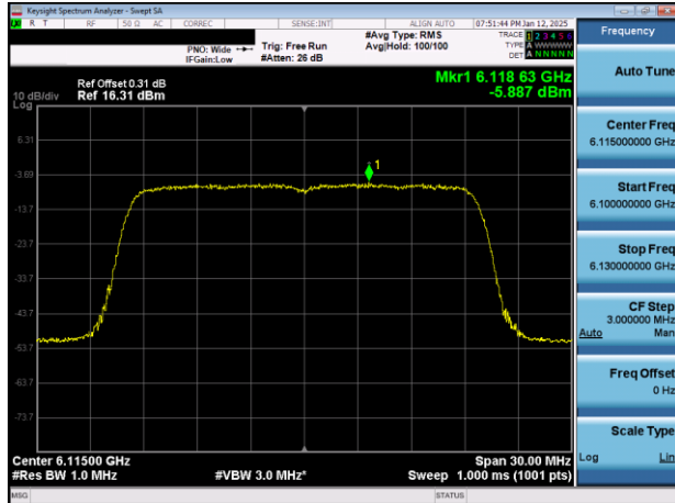
Plot 7-33. PSD Plot Antenna WF2a (20MHz 802.11ax (UNII Band 5) – Ch. 33)
