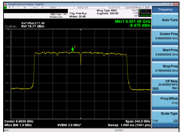
Plot 7-48. PSD Plot Antenna WF7b (160MHz 802.11ax (UNII Band 7) – Ch. 143)
