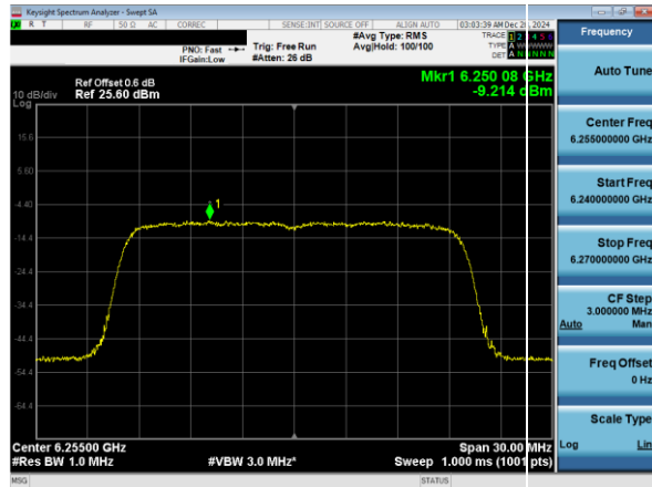
Plot 7-50. Power Spectral Density Plot SDM Primary Antenna WF2a (20MHz 802.11ax (UNII Band 5) – Ch.61)
