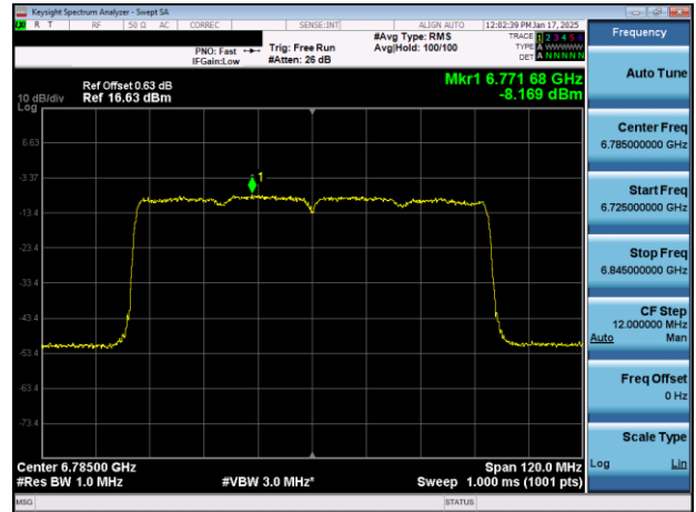
Plot 7-47. PSD Plot Antenna WF7b (80MHz 802.11ax (UNII Band 7) – Ch. 167)
