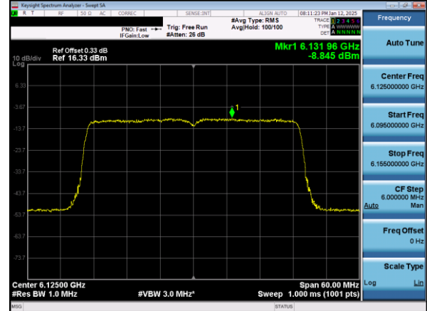
Plot 7-52. Power Spectral Density Plot SDM Primary Antenna WF2a (40MHz 802.11ax (UNII Band 5) – Ch. 35)
