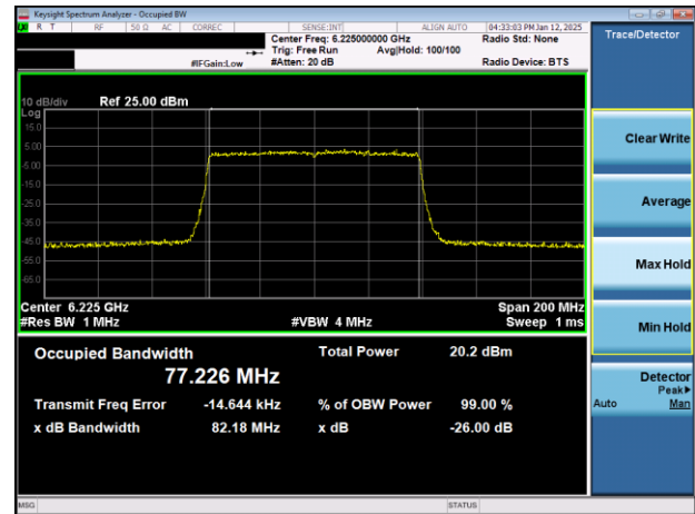
Plot 7-3. 26dB & 99% Bandwidth Plot Antenna WF7a (80MHz 802.11ax (UNII Band 5) – Ch. 55)
