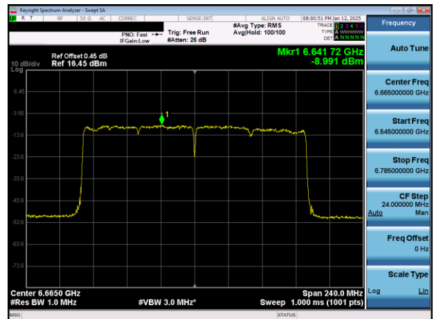
Plot 7-40. PSD Plot Antenna WF2a (160MHz 802.11ax (UNII Band 7) – Ch. 143)
