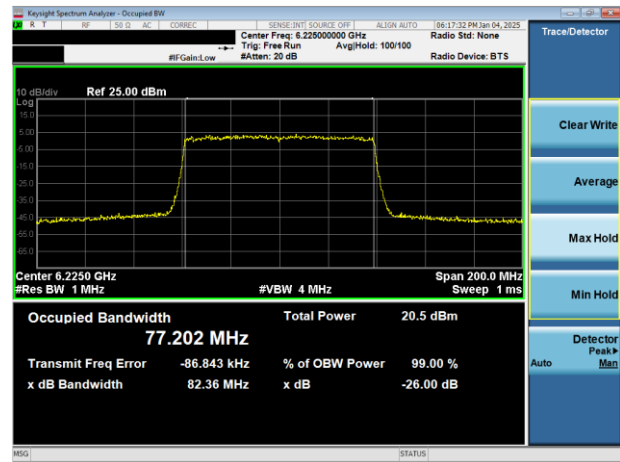
Plot 7-19. 26dB & 99% Bandwidth Plot Antenna WF7b (80MHz 802.11ax (UNII Band 5) – Ch. 55)
