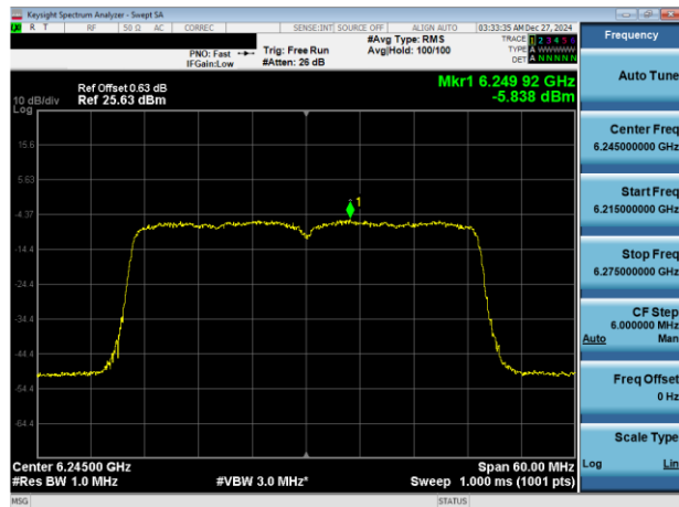
Plot 7-26. PSD Plot Antenna WF7a (40MHz 802.11ax (UNII Band 5) – Ch. 59)
