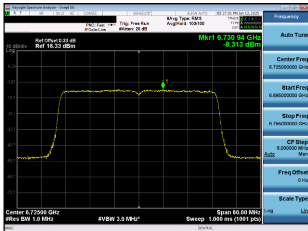
Plot 7-30. PSD Plot Antenna WF7a (40MHz 802.11ax (UNII Band 7) – Ch. 155)
