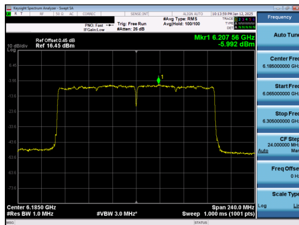
Plot 7-44. PSD Plot Antenna WF7b (160MHz 802.11ax (UNII Band 5) Ch. 47)
