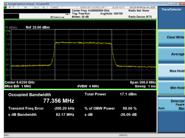
Plot 7-23. 26dB & 99% Bandwidth Plot Antenna WF7b (80MHz 802.11ax (UNII Band 7) – Ch. 135)
