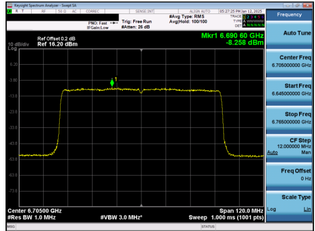
Plot 7-31. PSD Plot Antenna WF7a (80MHz 802.11ax (UNII Band 7) – Ch. 151)
