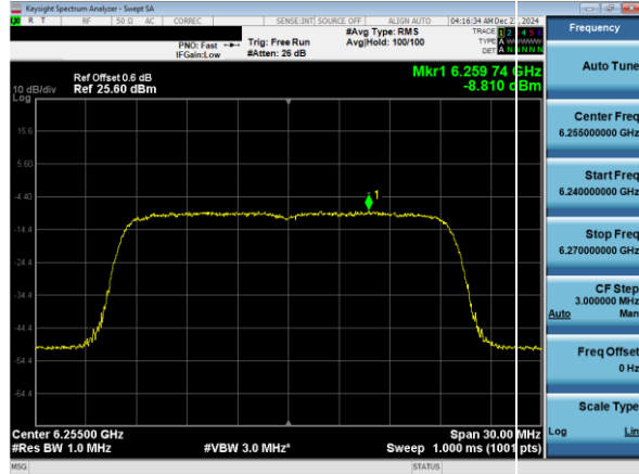
Plot 7-49. Power Spectral Density Plot SDM Primary Antenna WF7a (20MHz 802.11ax (UNII Band 5) – Ch.61)
