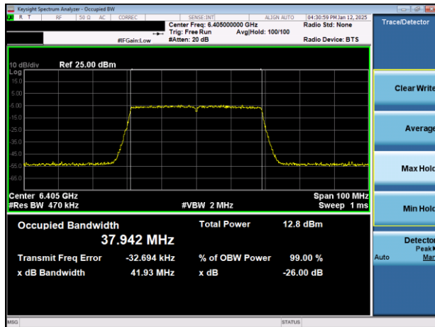
Plot 7-2. 26dB & 99% Bandwidth Plot Antenna WF7a (40MHz 802.11ax (UNII Band 5) – Ch. 91)
