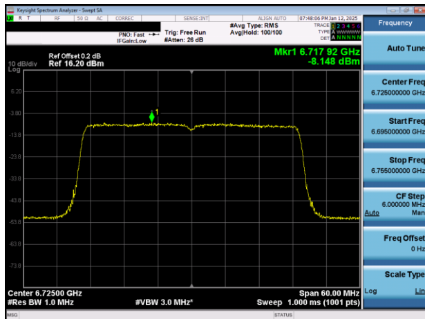
Plot 7-38. PSD Plot Antenna WF2a (40MHz 802.11ax (UNII Band 7) – Ch. 155)
