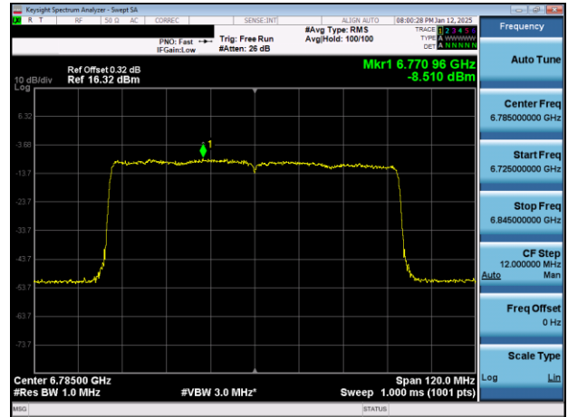
Plot 7-39. PSD Plot Antenna WF2a (80MHz 802.11ax (UNII Band 7) – Ch. 167)
