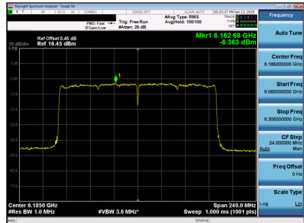
Plot 7-28. PSD Plot Antenna WF7a (160MHz 802.11ax (UNII Band 5) – Ch. 47)
