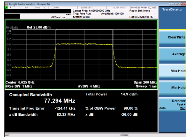
Plot 7-7. 26dB & 99% Bandwidth Plot Antenna WF7a (80MHz) 802.11ax (UNII Band 7) - Ch. 135)
