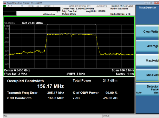
Plot 7-20. 26dB & 99% Bandwidth Plot Antenna WF7b (160MHz 802.11ax (UNII Band 5) – Ch. 79)
