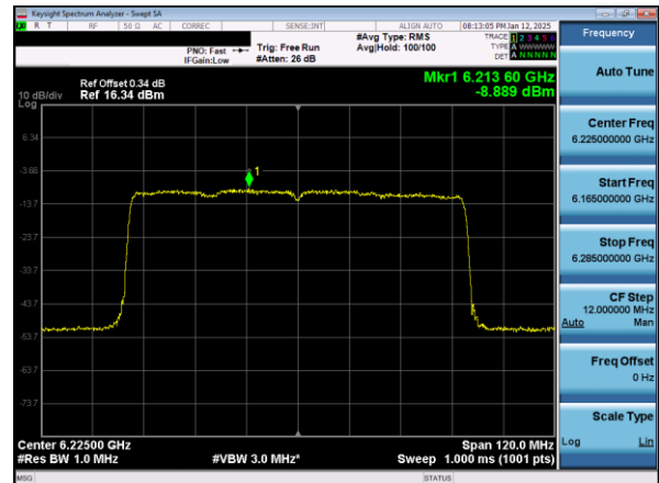
Plot 7-54. Power Spectral Density Plot SDM Primary Antenna WF2a (80MHz 802.11ax (UNII Band 5) – Ch. 55)
