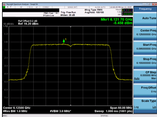
Plot 7-42. PSD Plot Antenna WF7b (40MHz 802.11ax (UNII Band 5) – Ch. 35)
