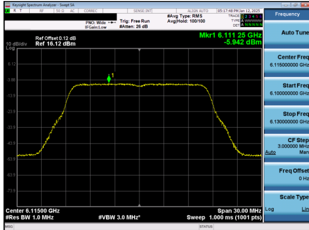
Plot 7-25. PSD Plot Antenna WF7a (20MHz 802.11a (UNII Band 5) – Ch. 33)
