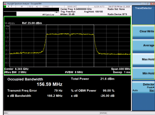
Plot 7-12. 26dB & 99% Bandwidth Plot Antenna WF2a (160MHz 802.11ax (UNII Band 5) – Ch. 79)
