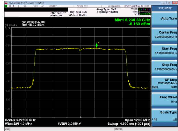
Plot 7-27. PSD Plot Antenna WF7a (80MHz 802.11ax (UNII Band 5) – Ch. 55)
