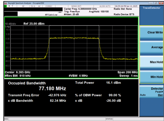
Plot 7-11. 26dB & 99% Bandwidth Plot Antenna WF2a (80MHz 802.11ax (UNII Band 5) – Ch. 87)
