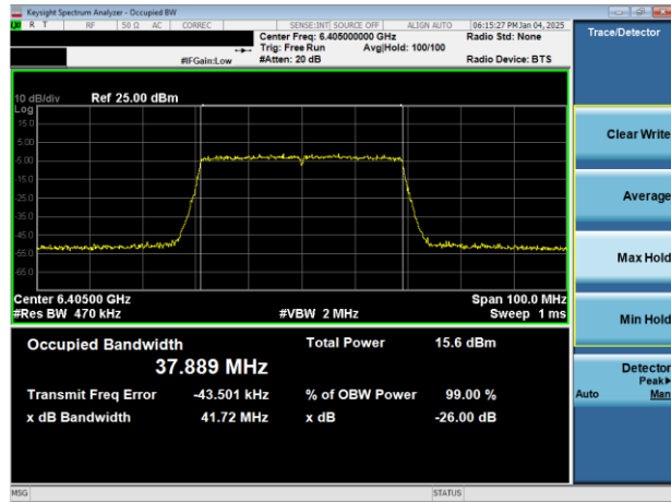
Plot 7-18. 26dB & 99% Bandwidth Plot Antenna WF7b (40MHz 802.11ax (UNII Band 5) – Ch. 91)
