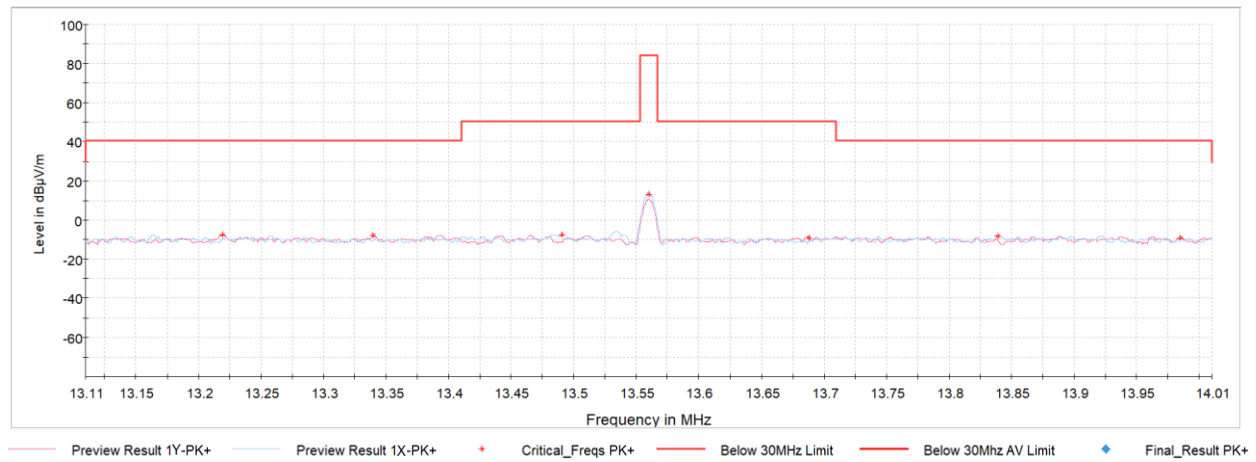
Plot 7-1. In Band Radiated Spurious Emissions (Charging Rate 2.6C, with AC/DC Adapter)
