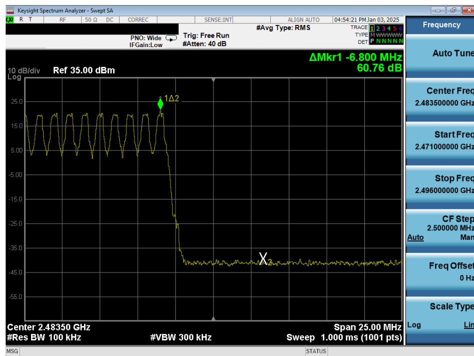
Plot 7-16. Band Edge Plot Antenna WF7b (Bluetooth with Hopping Enabled, GFSK, ePA)
