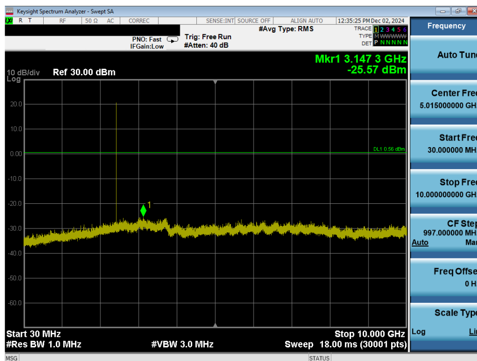
Plot 7-53. Conducted Spurious Plot Antenna WF2b (Bluetooth, GFSK, ePA – Ch. 39)
