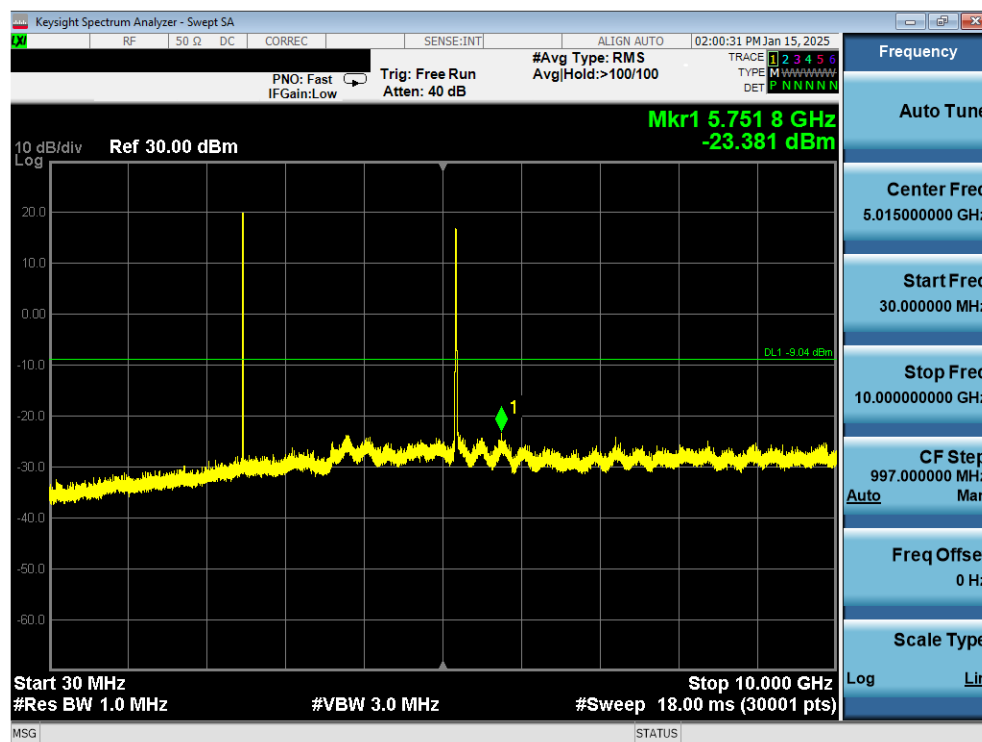
Plot 7-57. Conducted Simultaneous Tx Spurious Plots Antenna WF7b (Bluetooth + UNII)
