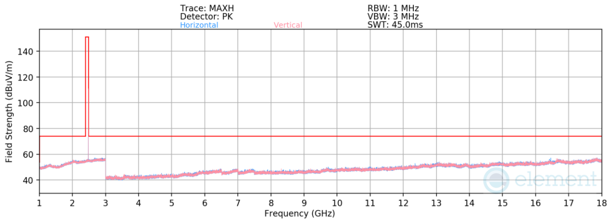
Plot 7-62. Radiated Spurious Emissions above 1GHz TxBF (BT GFSK ePA – Ch. 78)
