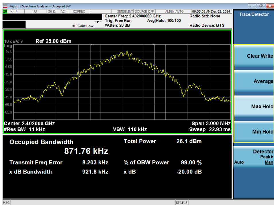
Plot 7-1. 20dB BW and 99% OBW Plot Antenna WF7b (Bluetooth, GFSK, ePA – Ch. 0)
