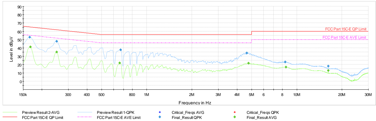
Plot 7-79. AC Line-Conducted Test Plot TxBF (L1, GFSK ePA – Ch.39, with AC/DC Adapter)
