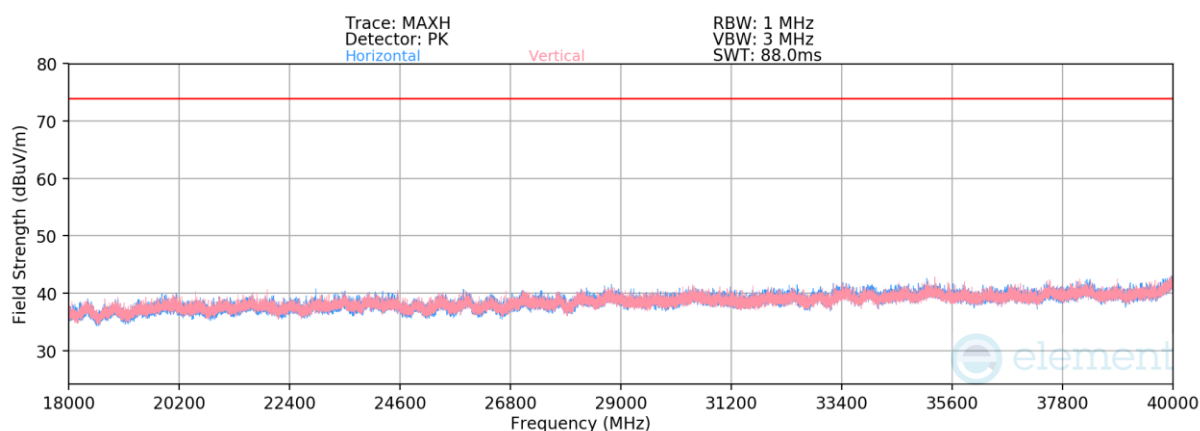
Plot 7-64. Radiated Spurious Emissions – Simultaneous Transmission Above 18GHz
