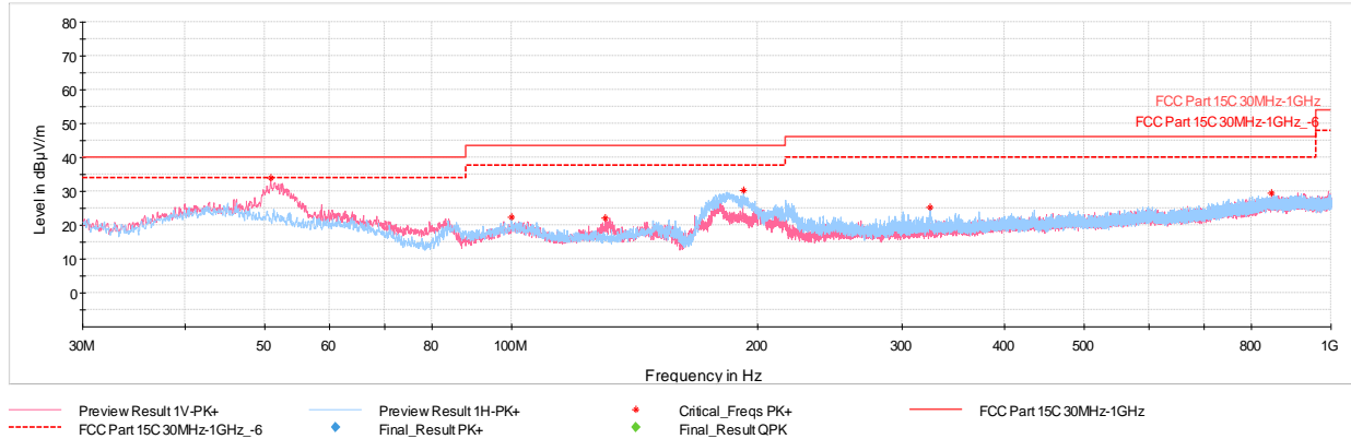
Plot 7-78. Radiated Spurious Emissions – Simultaneous Transmission Below 1GHz (with AC/DC Adapter)
