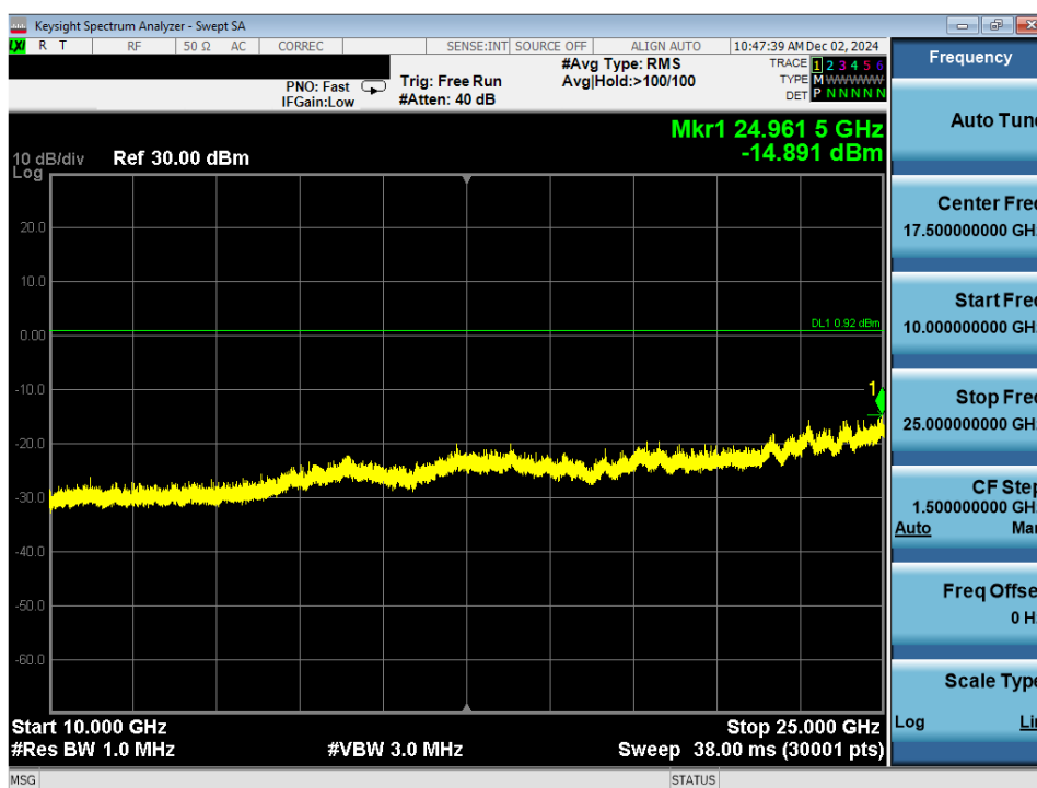
Plot 7-50. Conducted Spurious Plot Antenna WF7b (Bluetooth, GFSK, ePA – Ch. 78)
