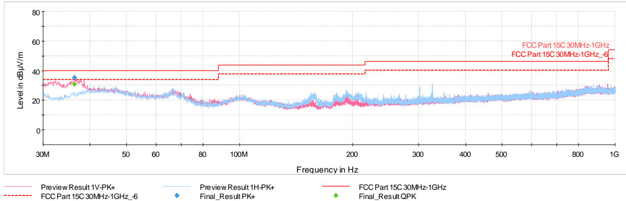
Plot 7-77. Radiated Spurious Emissions Below 1GHz TxBF (GFSK ePA – Ch.39, with AC/DC Adapter)
