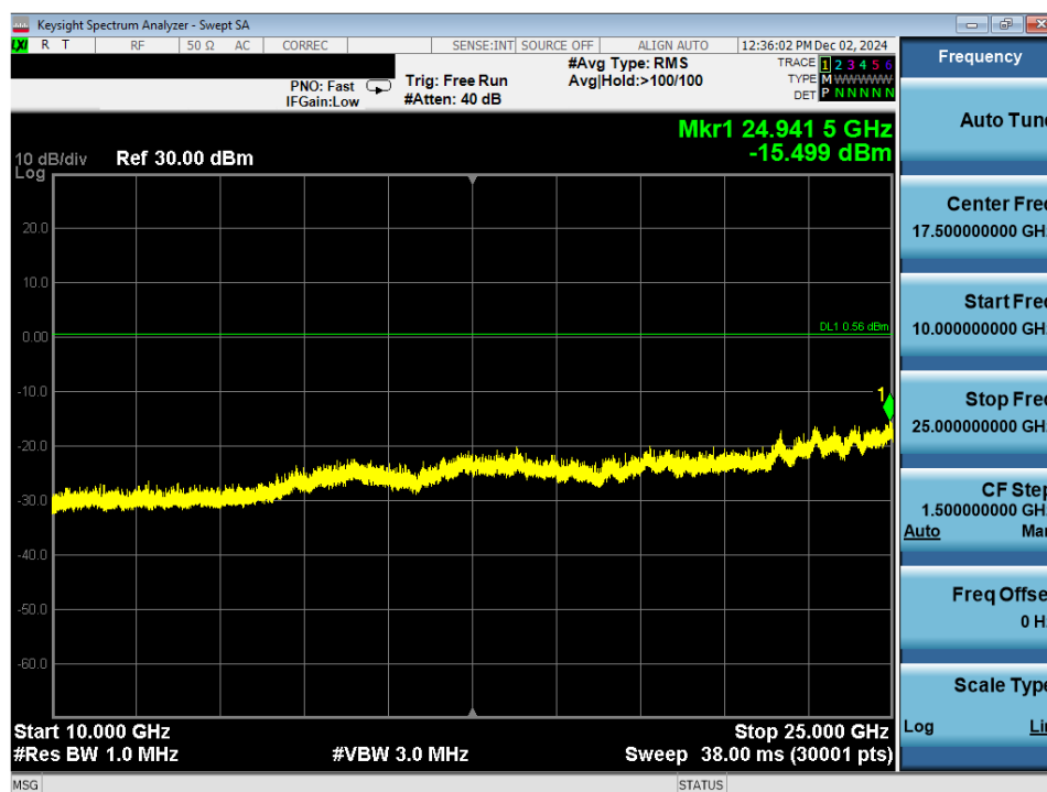
Plot 7-54. Conducted Spurious Plot Antenna WF2b (Bluetooth, GFSK, ePA Ch. 39)
