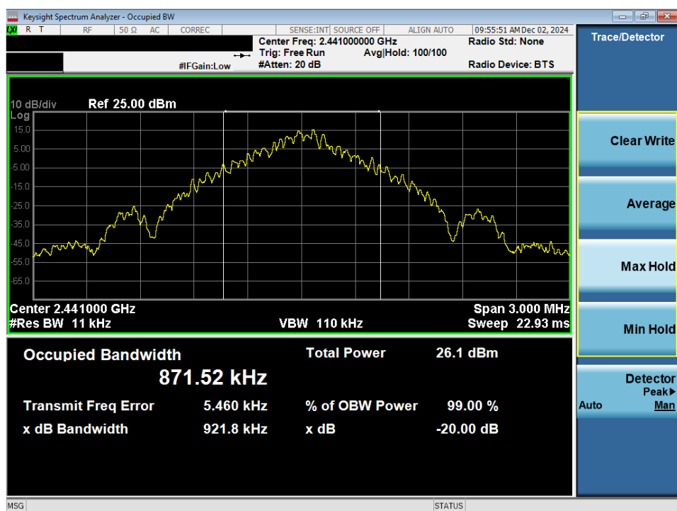
Plot 7-2. 20dB BW and 99% OBW Plot Antenna WF7b (Bluetooth, GFSK, ePA – Ch. 39)
