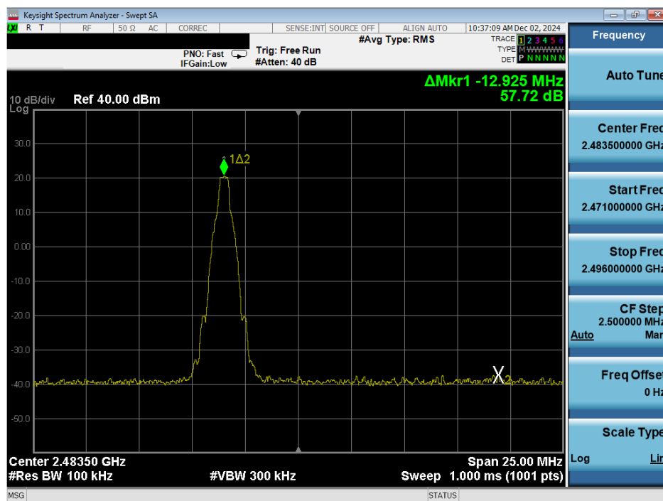
Plot 7-14. Band Edge Plot Antenna WF7b (Bluetooth with Hopping Disabled, GFSK, ePA – Ch. 78)
