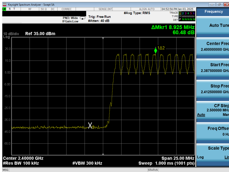
Plot 7-15. Band Edge Plot Antenna WF7b (Bluetooth with Hopping Enabled, GFSK, ePA)
