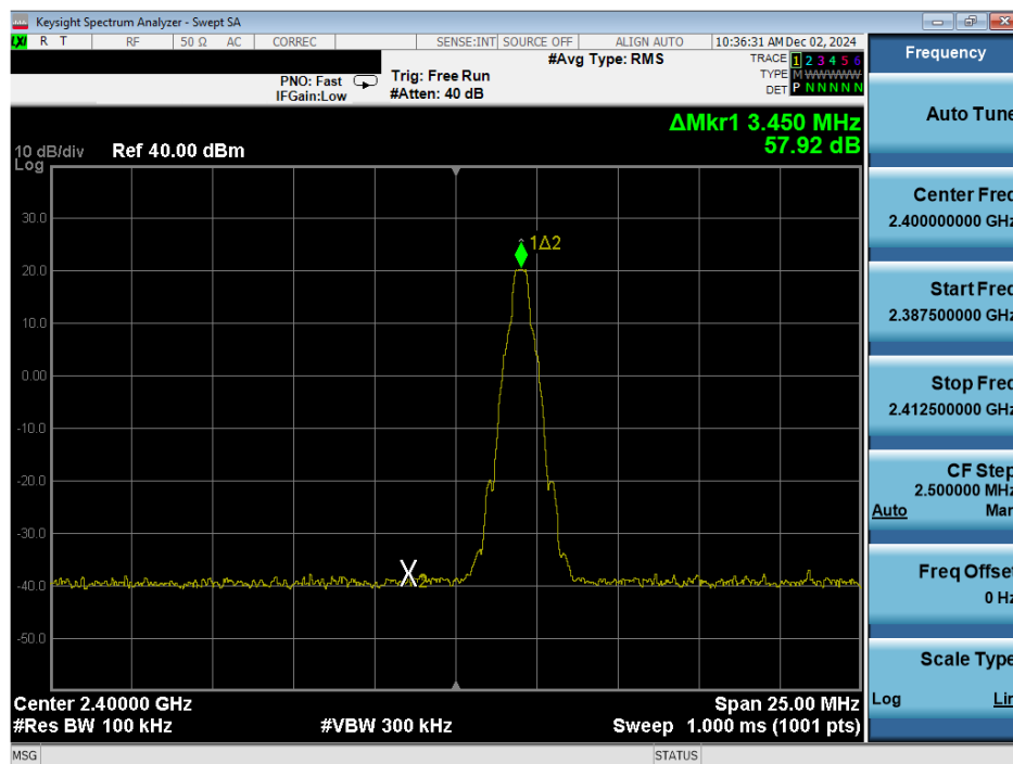
Plot 7-13. Band Edge Plot Antenna WF7b (Bluetooth with Hopping Disabled, GFSK, ePA – Ch. 0)
