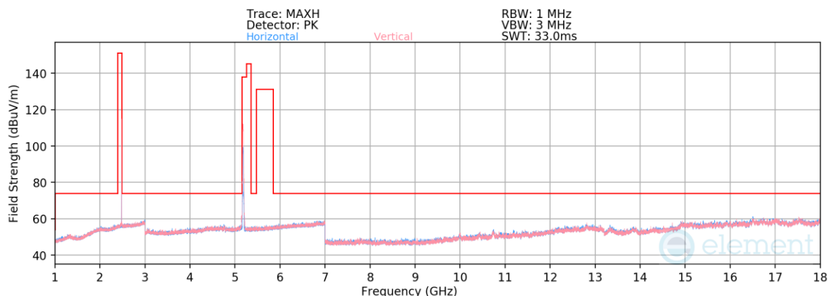
Plot 7-63. Radiated Spurious Emissions – Simultaneous Transmission Above 1GHz
